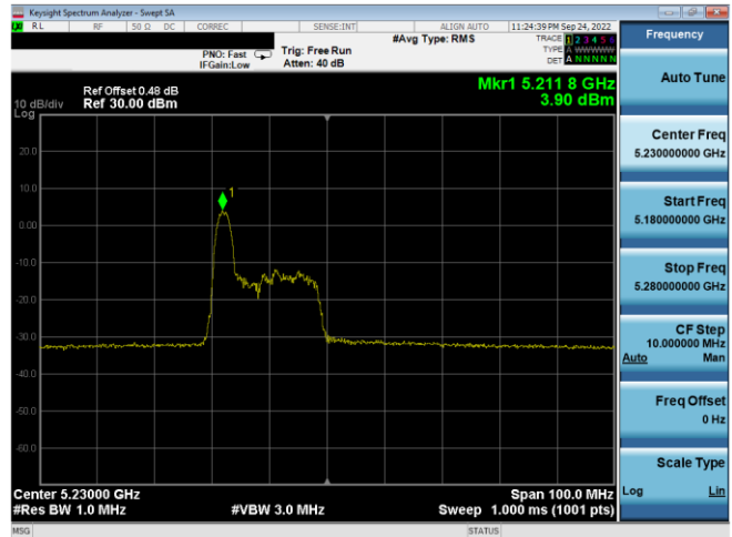
Plot 7-376. ISSED PSD SDM Antenna WF5B (40MHz BW 11ax index 0 - RU26 - Ch.46)
