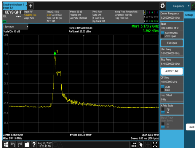
Plot 7-391. ISED PSD Antenna WF5T (20MHz BW 11ax Index 37 – RU52 – Ch.50(L))
