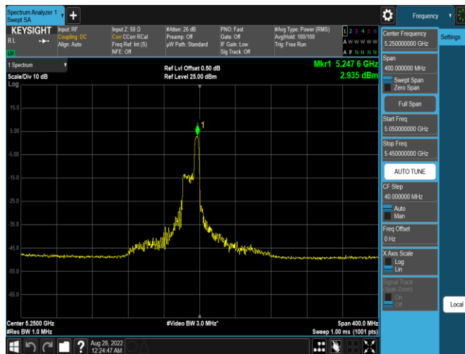
Plot 7-393. ISED PSD Antenna WF5T (20MHz BW 11ax Index 52 – RU52 – Ch.50(L))
