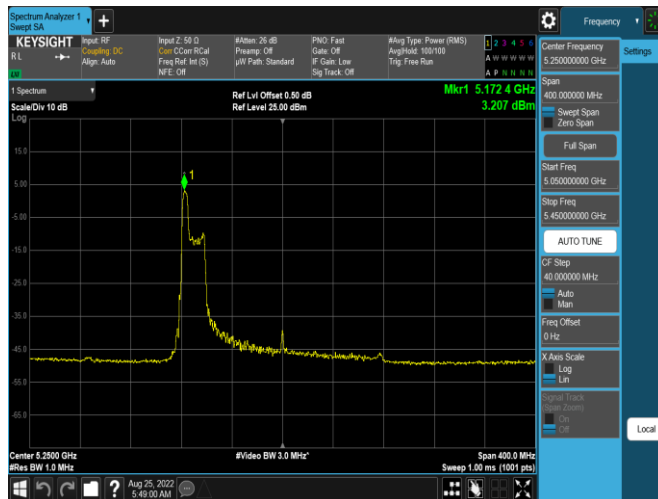
Plot 7-392. ISED PSD Antenna WF5B (20MHz BW 11ax Index 37 – RU52 – Ch.50(L))
