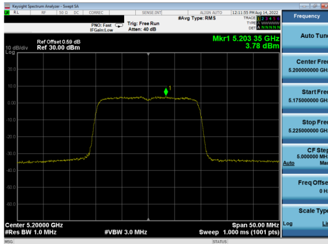
Plot 7-374. ISSED PSD SDM Antenna WF5B (20MHz BW 11ax- RU242 - Ch.40)
