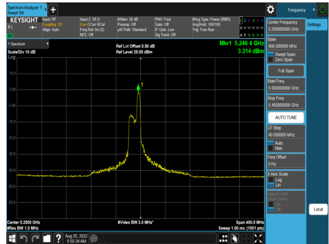
Plot 7-394. ISED PSD Antenna WF5B (20MHz BW 11ax Index 52 – RU52 – Ch.50(L))
