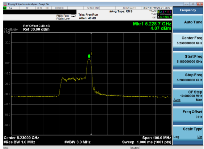
Plot 7-378. ISSED PSD SDM Antenna WF5B (40MHz BW 11ax Index 8 - RU26 - Ch.46)
