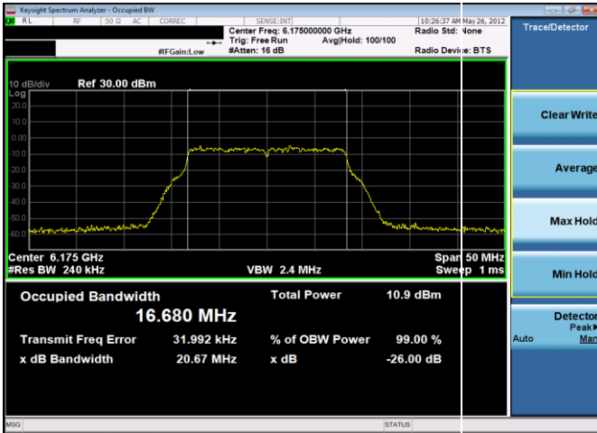
Plot 7-101. 26dB & 99% Bandwidth Plot Antenna 4a (20MHz 802.11a (UNII Band 5) – Ch. 45, MCS11)
