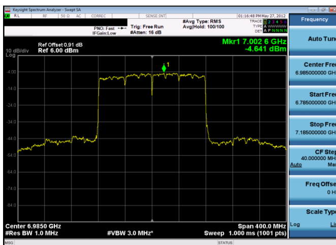
Plot 7-160. Power Spectral Density Plot Antenna 5b (160MHz 802.11ax (UNII Band 8) – Ch. 207, MCS4)
