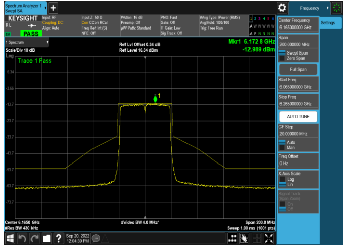
Plot 7-467. In-Band Emission Plot SDM Antenna 5b (40MHz 802.11ax (UNII Band 5) – Ch. 43, MCS2)
