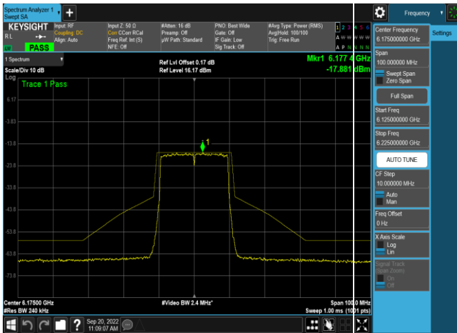
Plot 7-466. In-Band Emission Plot SDM Antenna 4a (20MHz 802.11ax (UNII Band 5) – Ch. 45, MCS2)
