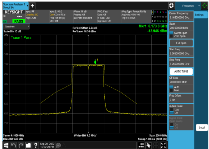
Plot 7-468. In-Band Emission Plot SDM Antenna 4a (40MHz 802.11ax (UNII Band 5) – Ch. 43, MCS2)
