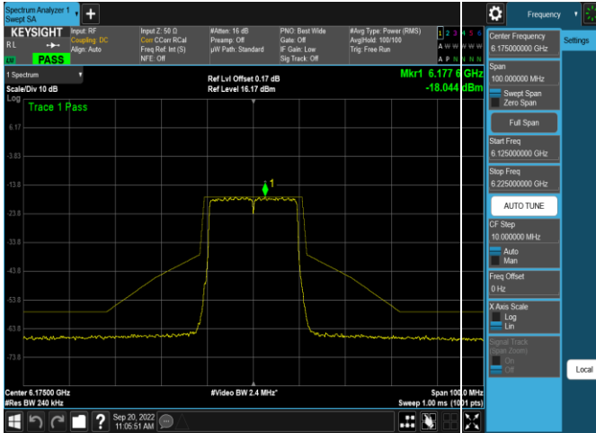
Plot 7-465. In-Band Emission Plot SDM Antenna 5b (20MHz 802.11ax (UNII Band 5) – Ch. 45, MCS2)
