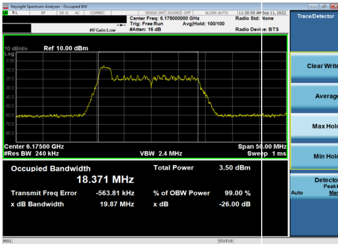
Plot 7-1. 26dB & 99% Bandwidth Plot Antenna 5b (20MHz 802.11ax RU26 (UNII Band 5) – Ch. 45)
