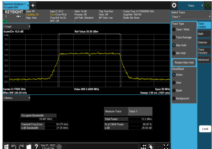
Plot 7-4. 26dB & 99% Bandwidth Plot Antenna 5b (20MHz 802.11ax RU242 (UNII Band 5) – Ch. 45)
