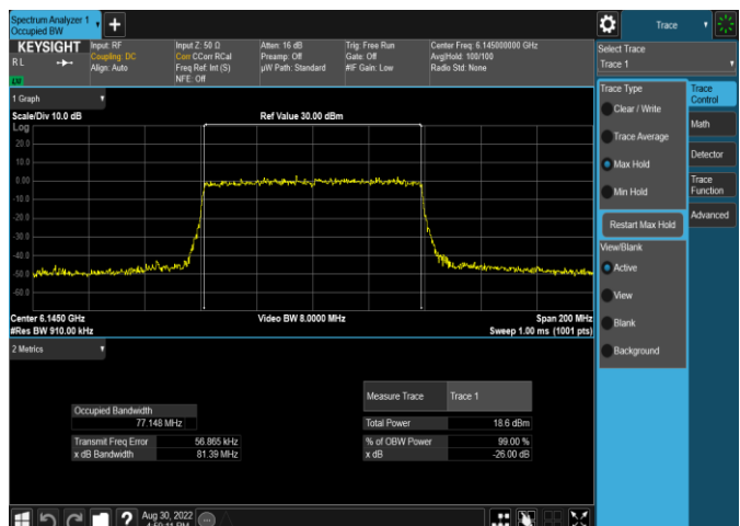
Plot 7-12. 26dB & 99% Bandwidth Plot Antenna 5b (80MHz 802.11ax RU996 (UNII Band 5) – Ch. 39)
