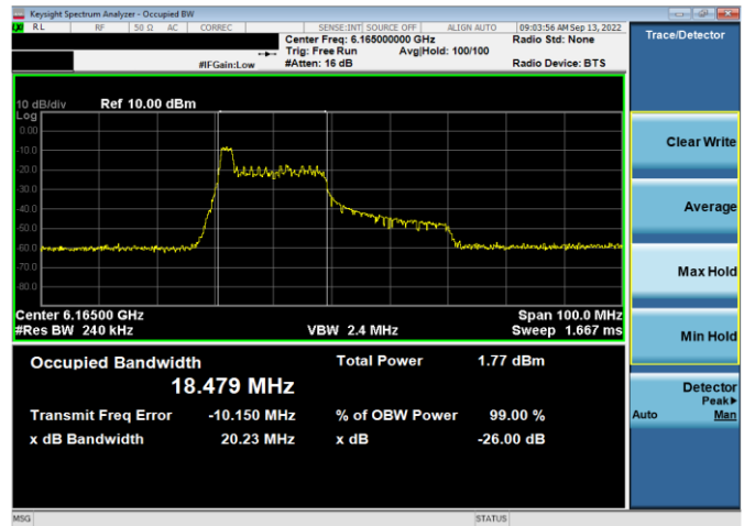
Plot 7-5. 26dB & 99% Bandwidth Plot Antenna 5b (40MHz 802.11ax RU26 (UNII Band 5) – Ch. 43)
