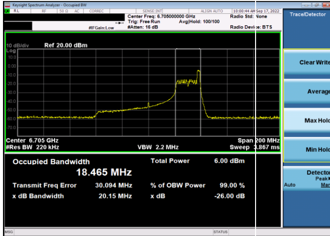
Plot 7-43. 26dB & 99% Bandwidth Plot Antenna 5b (80MHz 802.11ax RU26 (UNII Band 7) – Ch. 151)
