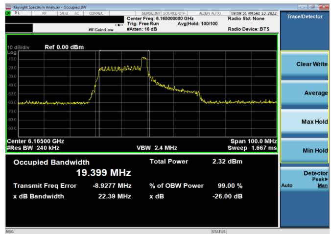
Plot 7-6. 26dB & 99% Bandwidth Plot Antenna 5b (40MHz 802.11ax RU26 (UNII Band 5) – Ch. 43)
