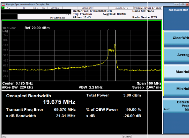
Plot 7-15. 26dB & 99% Bandwidth Plot Antenna 5b (160MHz 802.11ax RU26 (UNII Band 5) – Ch. 47)
