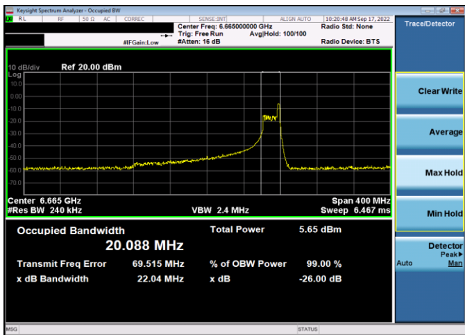
Plot 7-47. 26dB & 99% Bandwidth Plot Antenna 5b (160MHz 802.11ax RU26 (UNII Band 7) – Ch. 143)
