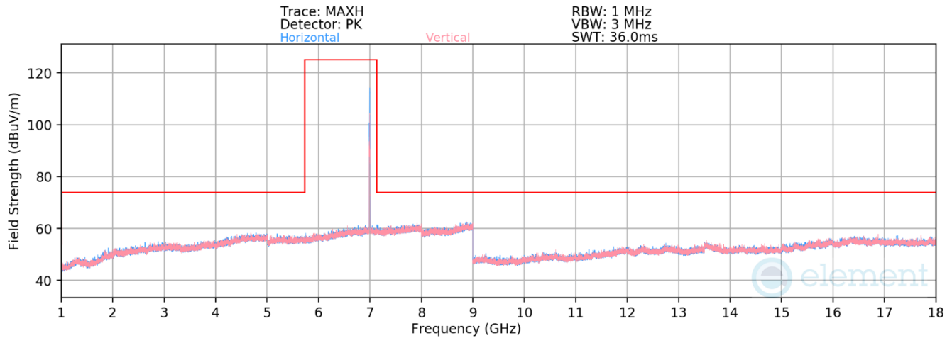
Plot 7-4. Radiated Spurious Emissions above 1GHz SDM (802.11ax – Ch. 209 – RU26)
