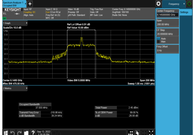
Plot 7-10. 26dB & 99% Bandwidth Plot Antenna 5b (80MHz 802.11ax RU26 (UNII Band 5) – Ch. 39)
