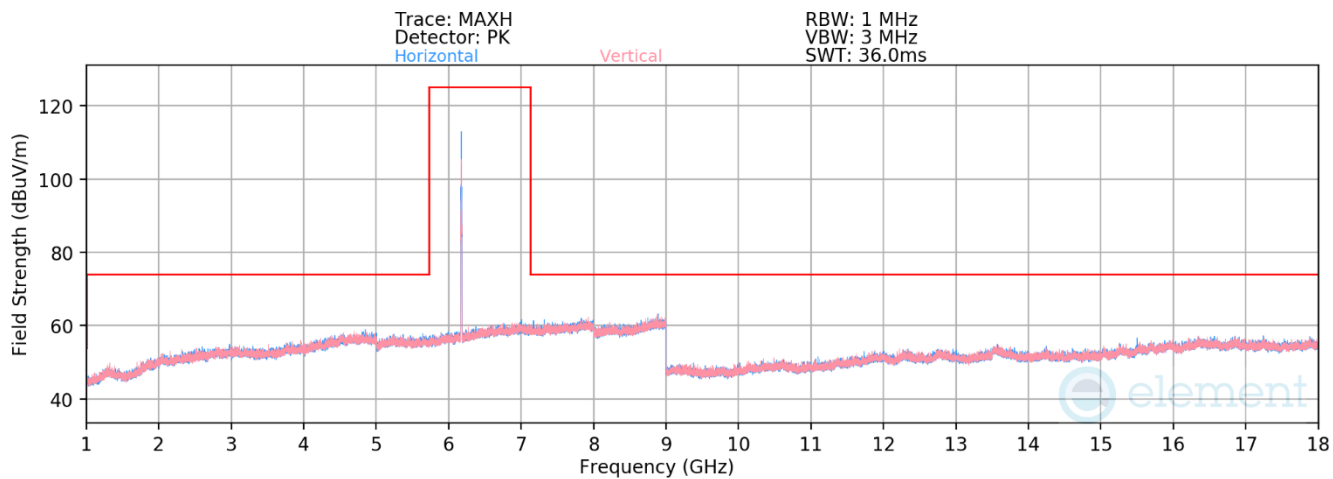
Plot 7-1. Radiated Spurious Emissions above 1GHz SDM (802.11ax – Ch. 45 – RU26)
