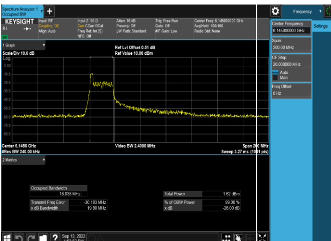
Plot 7-9. 26dB & 99% Bandwidth Plot Antenna 5b (80MHz 802.11ax RU26 (UNII Band 5) – Ch. 39)
