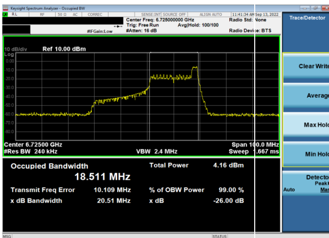
Plot 7-39. 26dB & 99% Bandwidth Plot Antenna 5b (40MHz 802.11ax RU26 (UNII Band 7) – Ch. 155)
