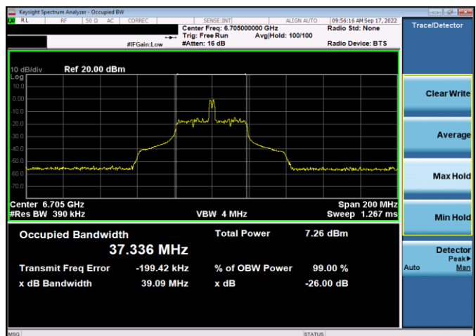
Plot 7-42. 26dB & 99% Bandwidth Plot Antenna 5b (80MHz 802.11ax RU26 (UNII Band 7) – Ch. 151)
