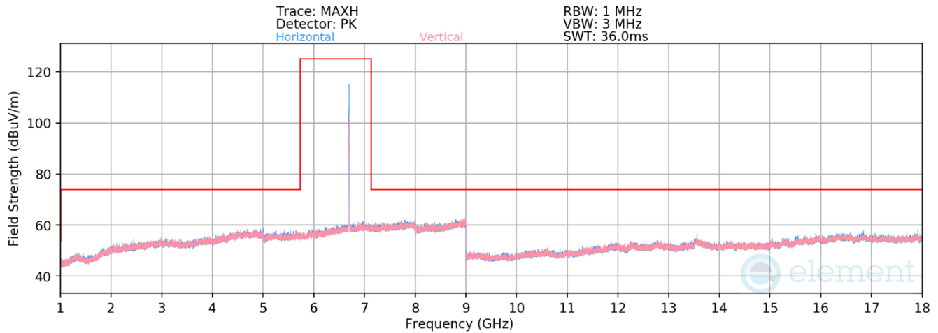
Plot 7-3. Radiated Spurious Emissions above 1GHz SDM (802.11ax – Ch. 149 – RU26)
