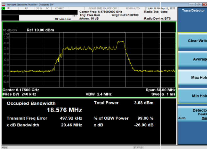
Plot 7-3. 26dB & 99% Bandwidth Plot Antenna 5b (20MHz 802.11ax RU26 (UNII Band 5) – Ch. 45)
