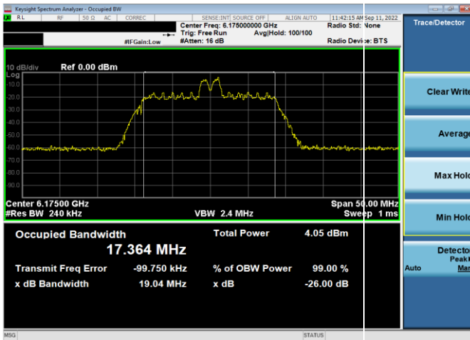
Plot 7-2. 26dB & 99% Bandwidth Plot Antenna 5b (20MHz 802.11ax RU26 (UNII Band 5) – Ch. 45)
