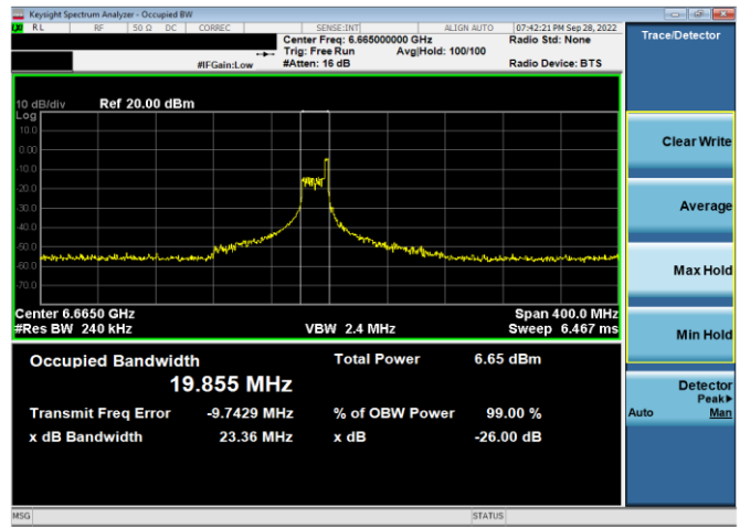
Plot 7-46. 26dB & 99% Bandwidth Plot Antenna 5b (160MHz 802.11ax RU26 (UNII Band 7) – Ch. 143)
