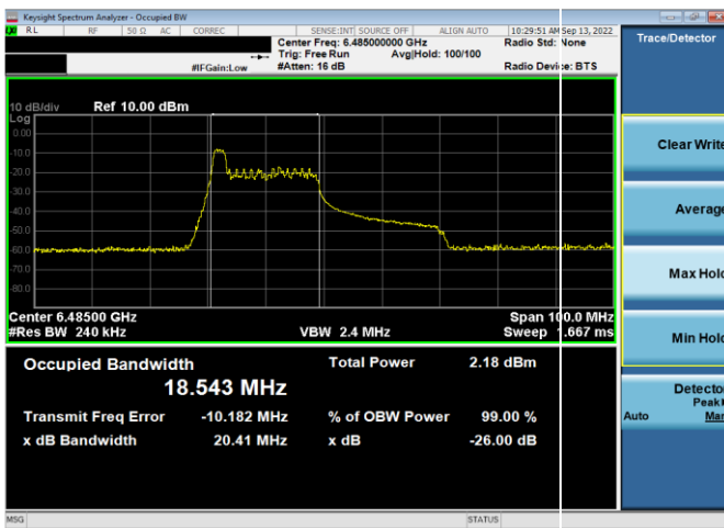
Plot 7-21. 26dB & 99% Bandwidth Plot Antenna 5b (40MHz 802.11ax RU26 (UNII Band 6) – Ch. 107)
