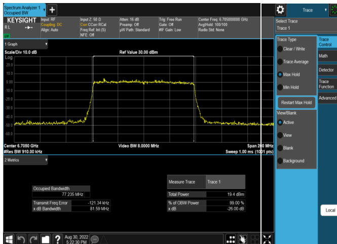
Plot 7-44. 26dB & 99% Bandwidth Plot Antenna 5b (80MHz 802.11ax RU996 (UNII Band 7) – Ch. 151)
