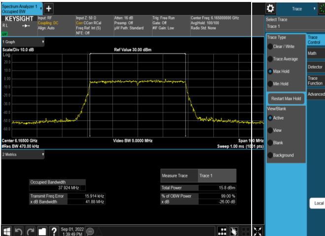
Plot 7-8. 26dB & 99% Bandwidth Plot Antenna 5b (40MHz 802.11ax RU484 (UNII Band 5) – Ch. 43)
