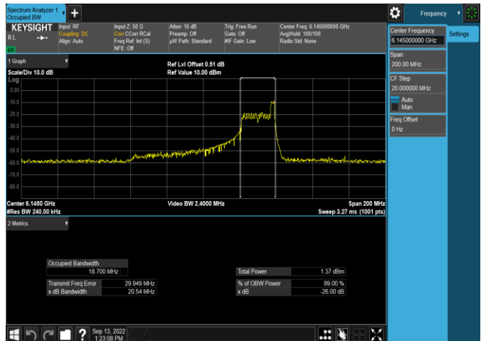
Plot 7-11. 26dB & 99% Bandwidth Plot Antenna 5b (80MHz 802.11ax RU26 (UNII Band 5) – Ch. 39)
