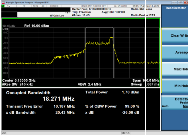
Plot 7-7. 26dB & 99% Bandwidth Plot Antenna 5b (40MHz 802.11ax RU26 (UNII Band 5) – Ch. 43)
