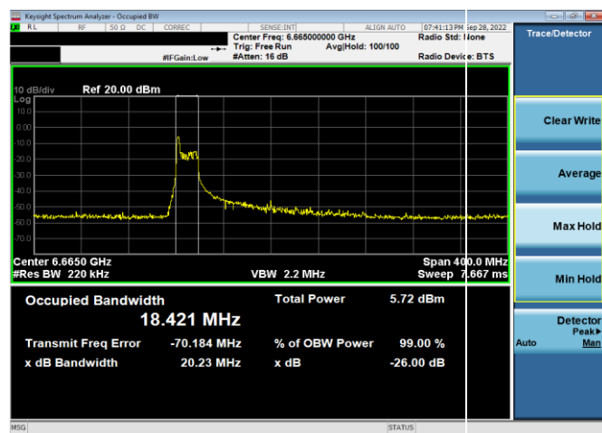
Plot 7-45. 26dB & 99% Bandwidth Plot Antenna 5b (160MHz 802.11ax RU26 (UNII Band 7) – Ch. 143)
