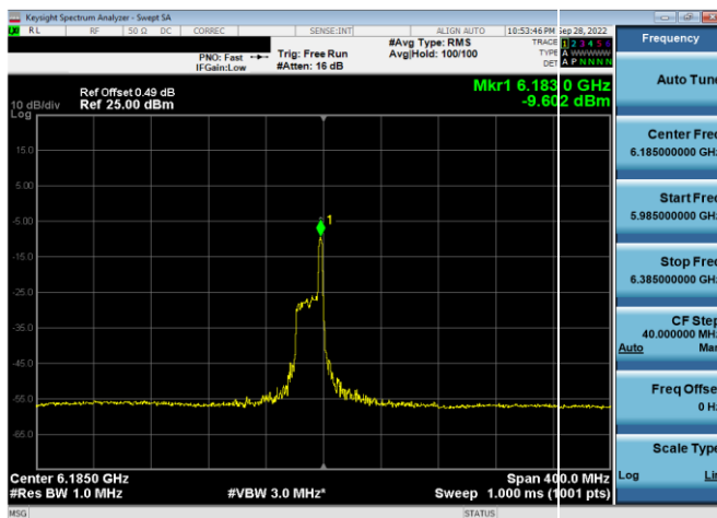
Plot 7-283. Power Spectral Density Plot SDM Antenna 5b (160MHz 802.11ax RU26 (UNII Band 5) – Ch. 47)
