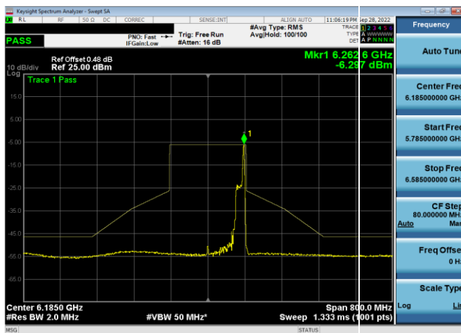
Plot 7-399. In-Band Emission Plot Antenna 5b (160MHz 802.11ax RU26 (UNII Band 5) – Ch. 47)
