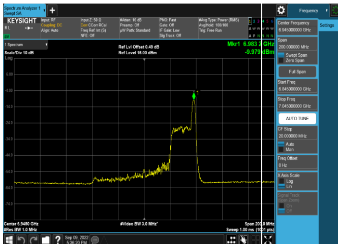
Plot 7-373. Power Spectral Density Plot SDM Antenna 5b (80MHz 802.11ax RU26 (UNII Band 8) – Ch. 199)
