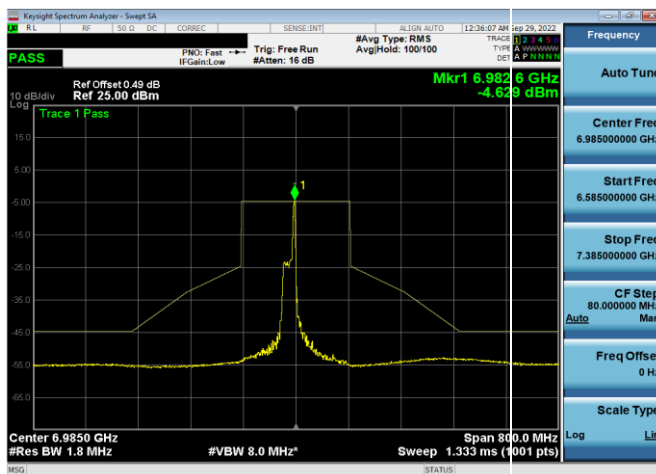
Plot 7-635. In-Band Emission Plot SDM Antenna 5b (160MHz 802.11ax RU26 (UNII Band 8) – Ch. 207)
