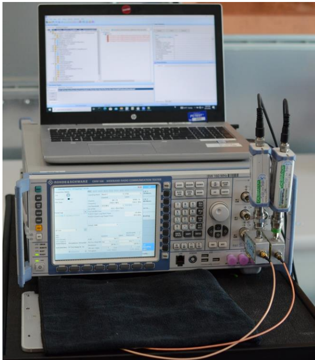
Test Setup Photo 5 – Conducted Test Setup (Figure 5-1c)
