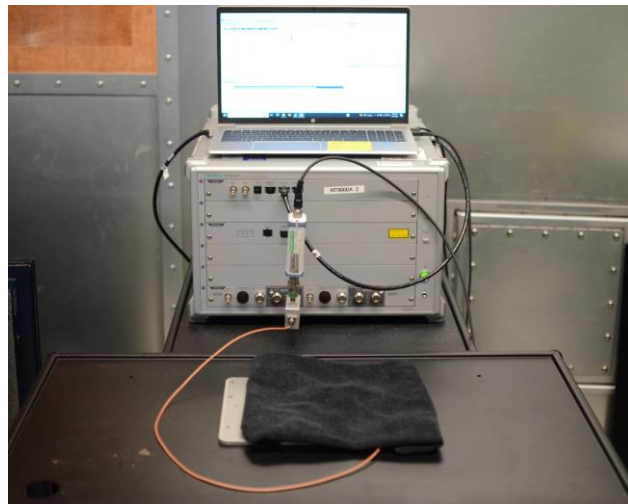
Test Setup Photo 2 – Conducted Test Setup (Figure 5-1a)
