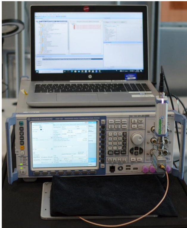
Test Setup Photo 1 – Conducted Test Setup (Figure 5-1a)
