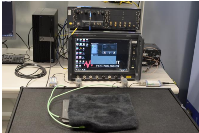
Test Setup Photo 6 – Conducted Test Setup (Figure 5-1c)
