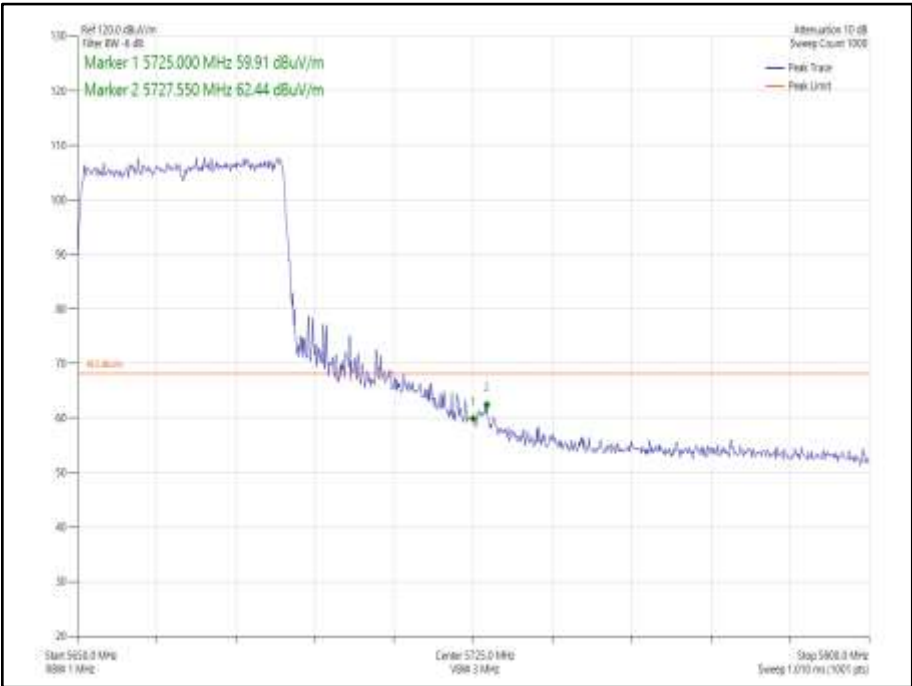
Figure 936 - 802.11ax HE40, Core 0, SU - 5670 MHz Band Edge Frequency 5725 MHz
