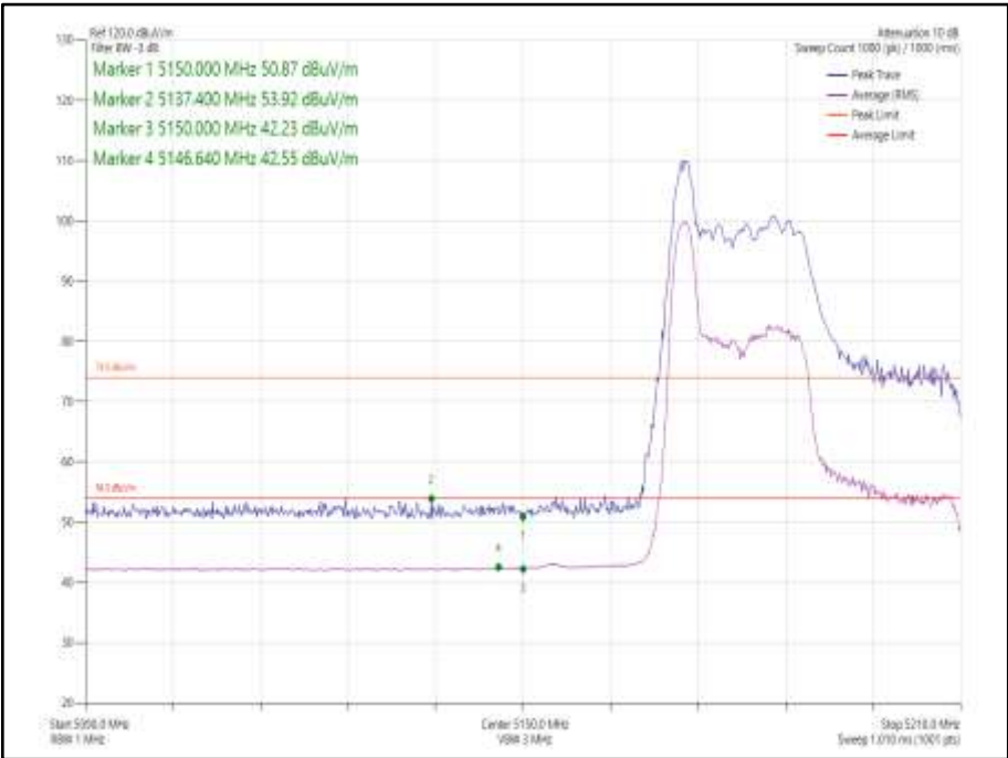
Figure 1044 - 802.11ax HE40 CDD, Cores 0-1, 26-0 - 5190 MHz Band Edge Frequency 5150 MHz
