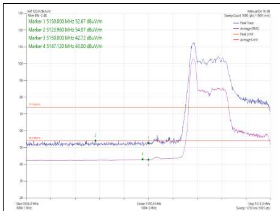
Figure 1046 - 802.11ax HE40 SDM, Cores 0-1, 26-0 - 5190 MHz Band Edge Frequency 5150 MHz
