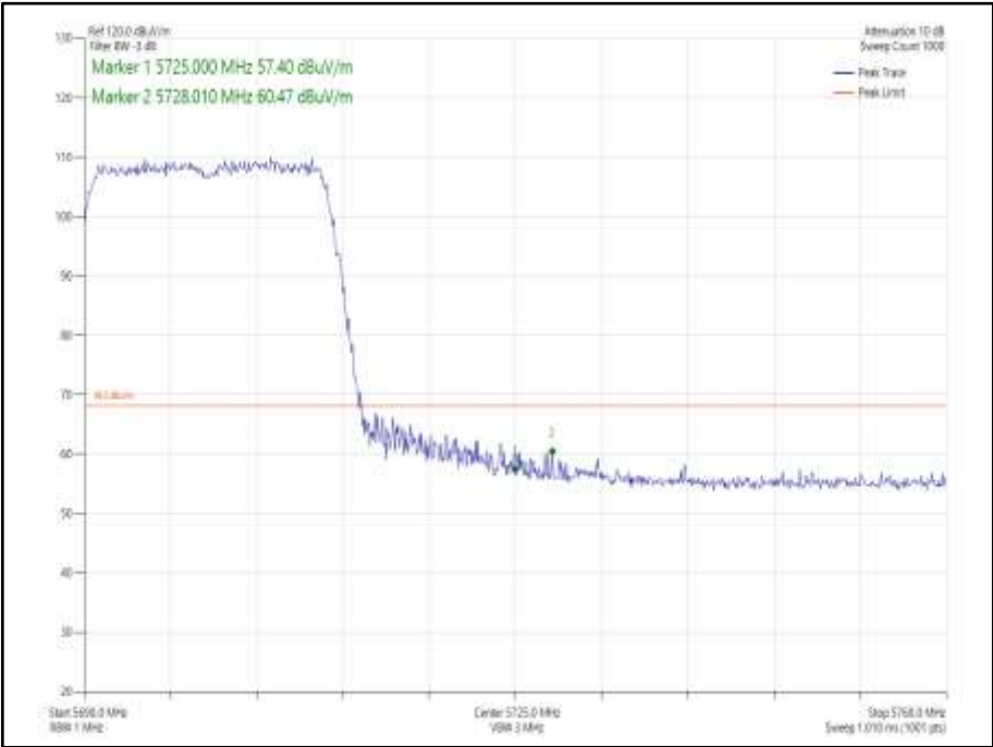
Figure 916 - 802.11ax HE20 SDM, Cores 0-1, SU - 5700 MHz Band Edge Frequency 5725 MHz
