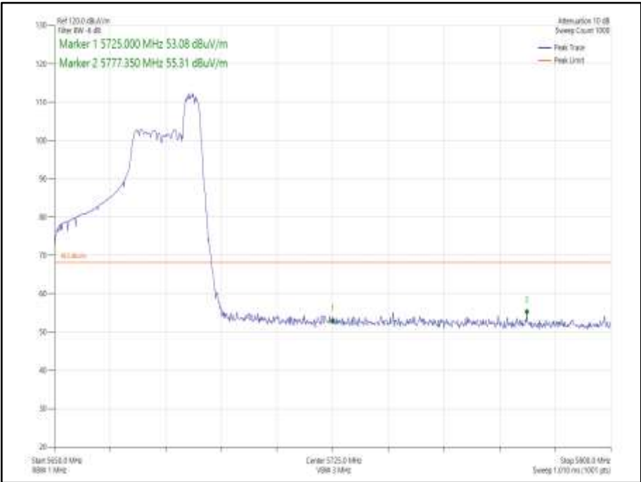
Figure 951 - 802.11ax HE40 CDD, Cores 0-1, 52-44 - 5670 MHz Band Edge Frequency 5725 MHz
