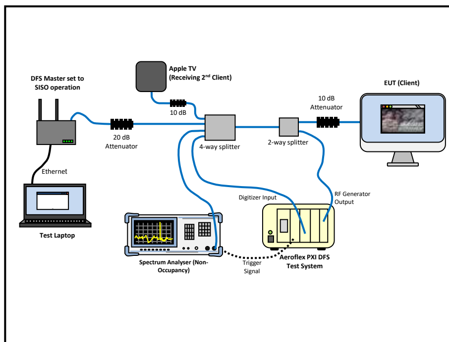
Figure 1149 - Test Equipment Setup Diagram for Client without Radar Detection with Injection at the Master – Client-to-Client Mode
