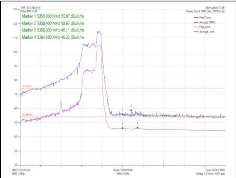
Figure 1079 - 802.11ax HE80 SDM, Cores 0-1, 26-36- 5290 MHz Band Edge Frequency 5350 MHz
