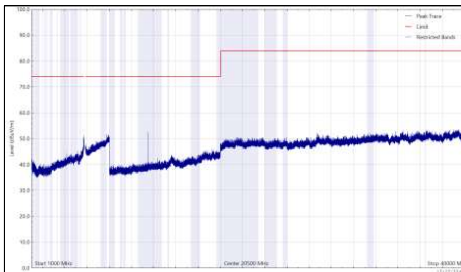
Figure 1133 - 5745 MHz (CH149), HE20, RU26-0, Core 0 + Core 1, 1 GHz to 40 GHz, Horizontal (Peak)
