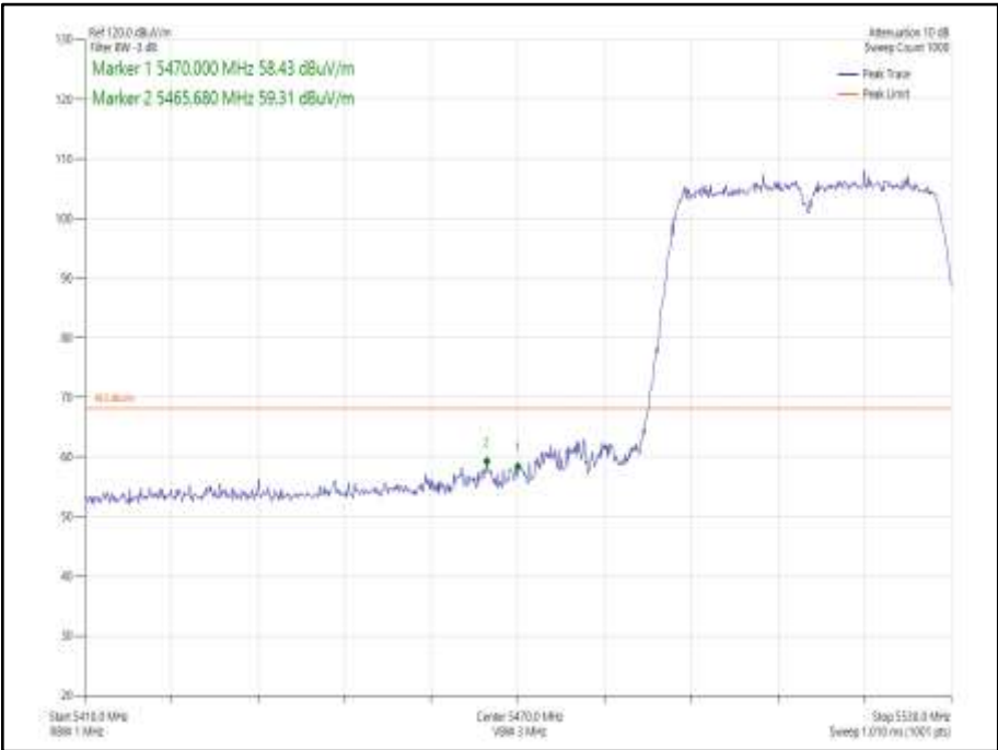
Figure 943 - 802.11n HT40 SDM, Cores 0-1 - 5510 MHz Band Edge Frequency 5470 MHz
