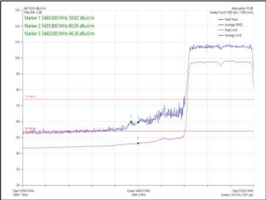
Figure 1039 - 802.11ax HE40, Core 0, SU - 5510 MHz Band Edge Frequency 5460 MHz
