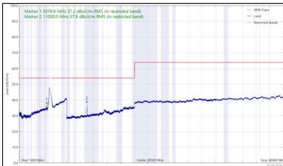
Figure 1098 - U-NII-2C - 5500 MHz (CH100), HT20, CDD, Core 0 + Core 1, 1 GHz to 40 GHz, Horizontal (RMS)
