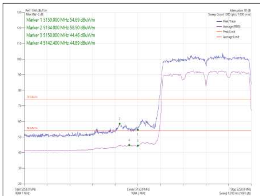
Figure 1069 - 802.11ac VHT80 SDM, Cores 0-1- 5210 MHz Band Edge Frequency 5150 MHz
