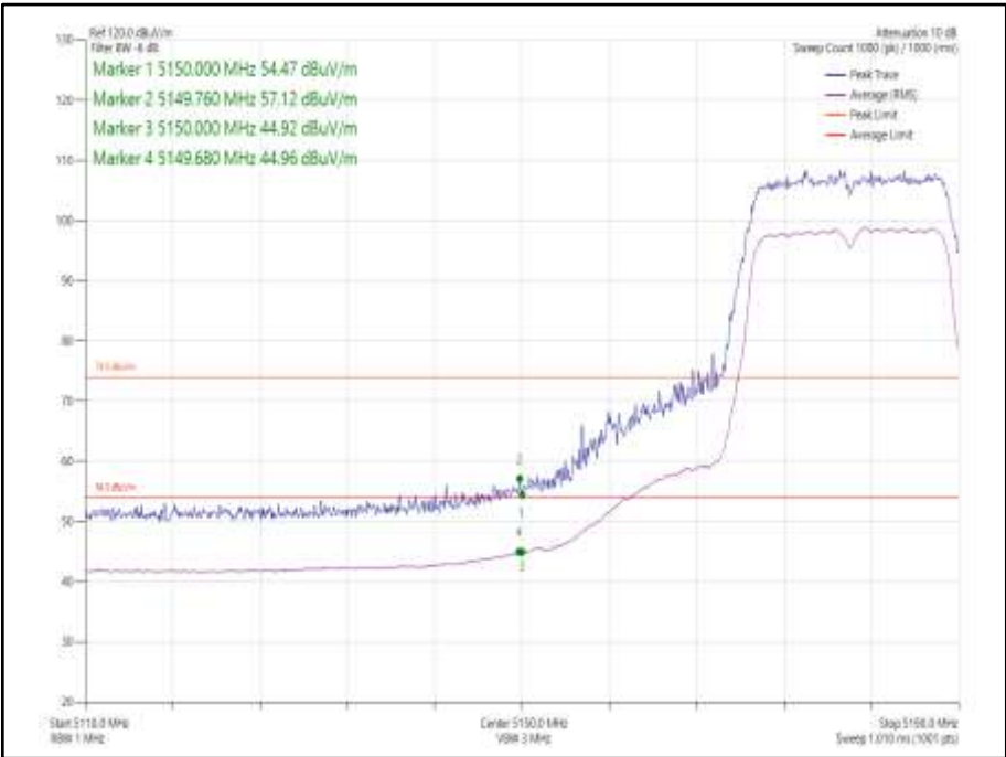
Figure 1015 - 802.11n HT20 SDM, Cores 0-1 - 5180 MHz Band Edge Frequency 5150 MHz
