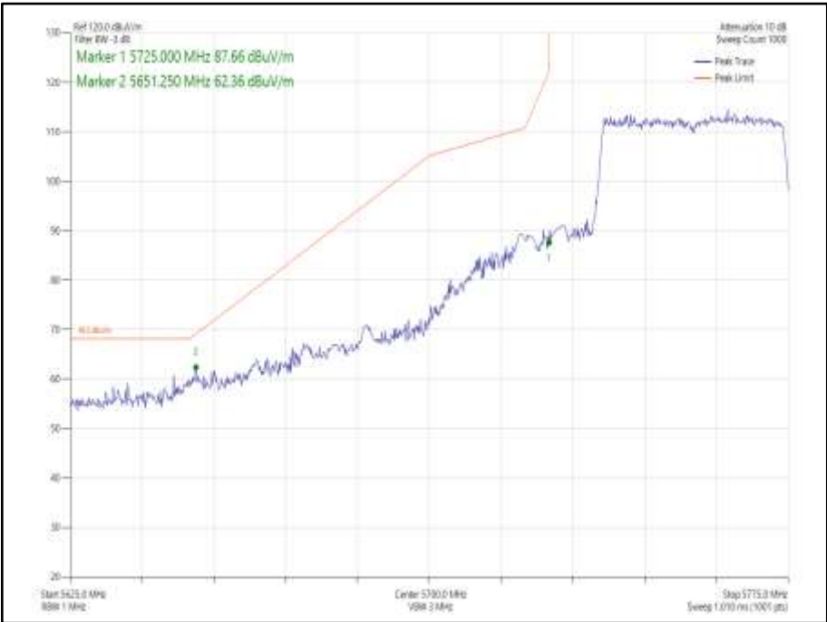
Figure 938 - 802.11ax HE40, Core 0, SU - 5755 MHz Band Edge Frequency 5725 MHz
