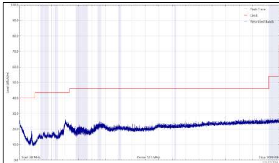
Figure 1112 - U-NII-3 - 5825 MHz (CH165), HT20, CDD, Core 0 + Core 1, 30 MHz to 1 GHz, Vertical (Peak)
