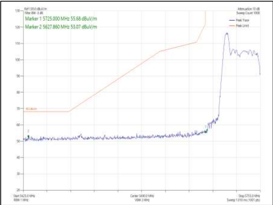
Figure 921 - 802.11ax HE20 CDD, Cores 0-1, 26-0 - 5745 MHz Band Edge Frequency 5725 MHz
