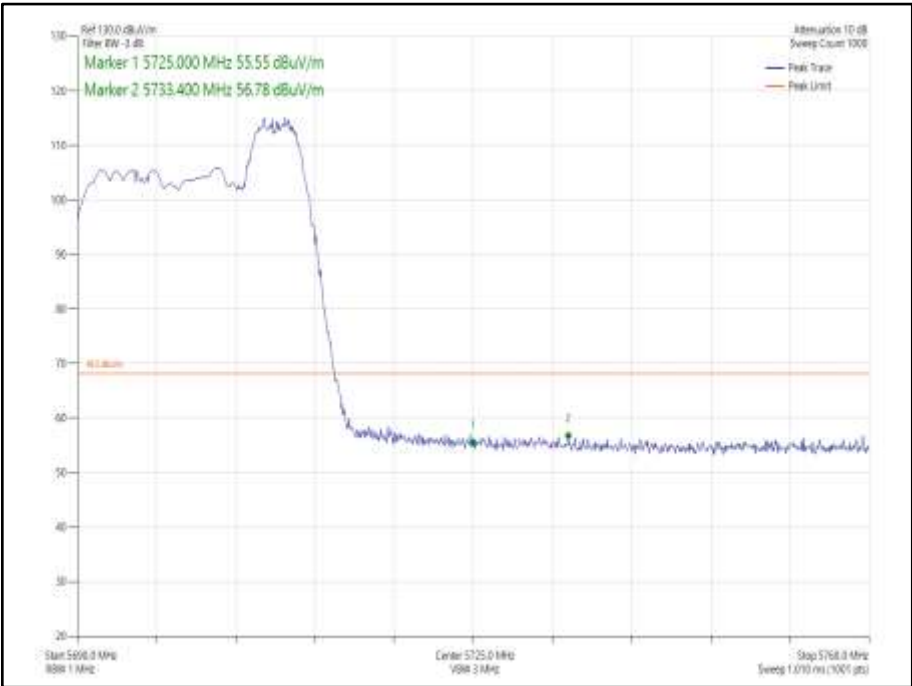
Figure 917 - 802.11ax HE20 SDM, Cores 0-1, 26-8 - 5700 MHz Band Edge Frequency 5725 MHz
