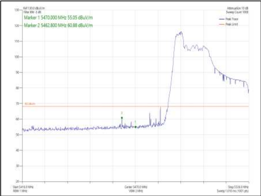
Figure 935 - 802.11ax HE40, Core 0, 26-0 - 5510 MHz Band Edge Frequency 5470 MHz
