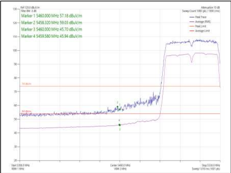
Figure 1038 - 802.11n HT40, Core 0 - 5510 MHz Band Edge Frequency 5460 MHz
