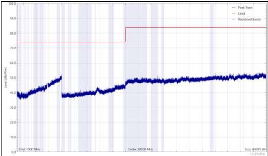
Figure 1135 - 5745 MHz (CH149), HE20, RU26-0, Core 0 + Core 1, 1 GHz to 40 GHz, Vertical (Peak)
