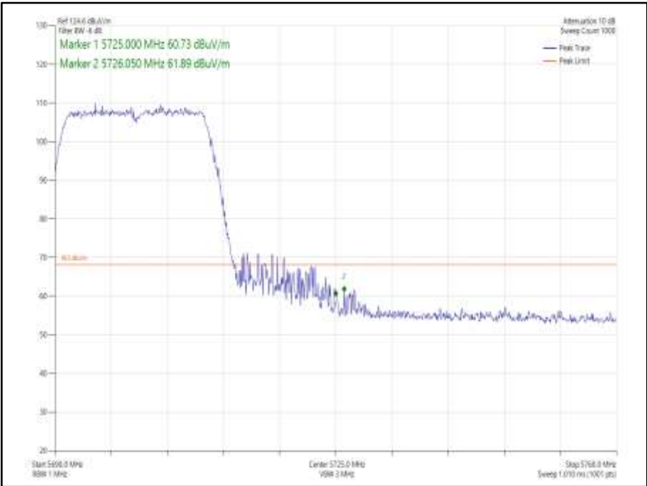
Figure 913 - 802.11n HT20 SDM, Cores 0-1 - 5700 MHz Band Edge Frequency 5725 MHz
