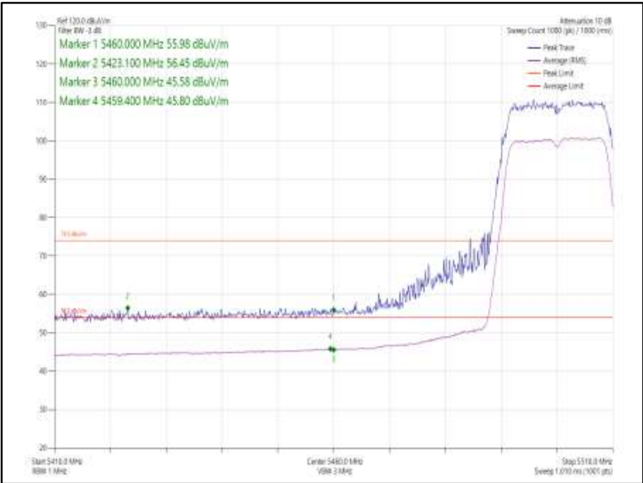
Figure 1027 - 802.11n HT20 SDM, Cores 0-1 - 5500 MHz Band Edge Frequency 5460 MHz
