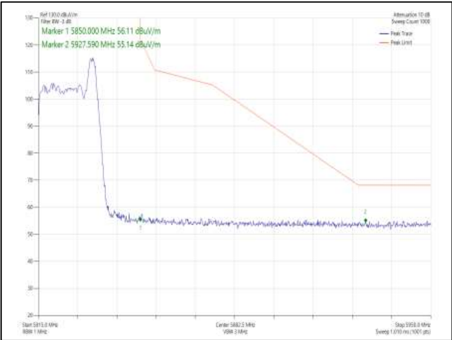
Figure 929 - 802.11ax HE20 SDM, Cores 0-1, 26-8 - 5825 MHz Band Edge Frequency 5850 MHz
