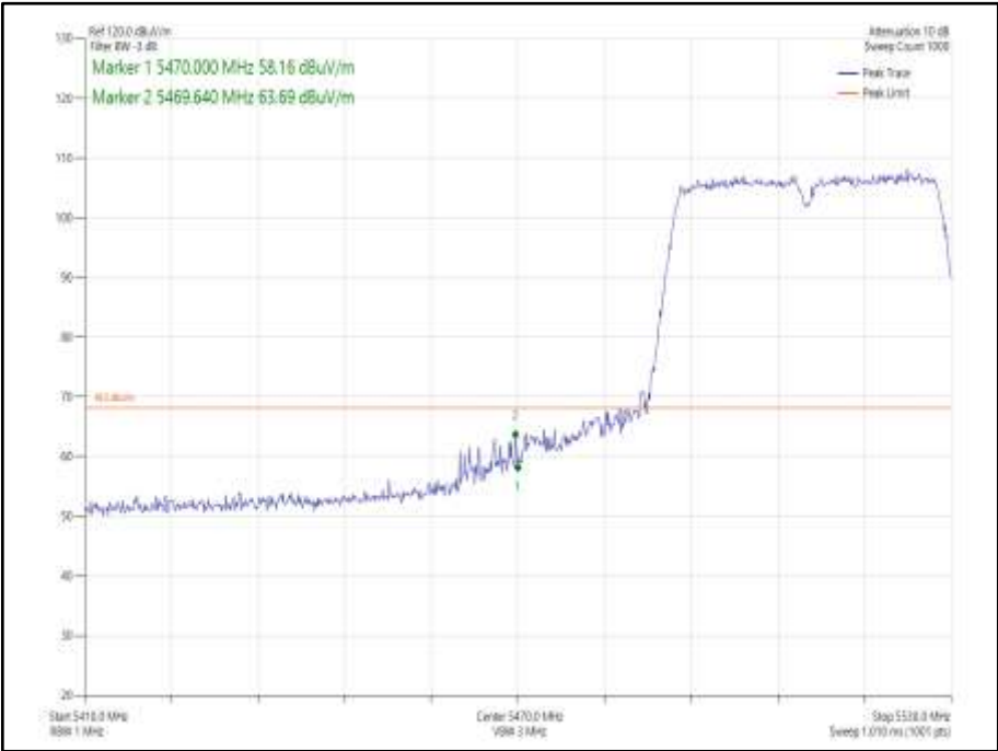
Figure 942 - 802.11n HT40 CDD, Cores 0-1 - 5510 MHz Band Edge Frequency 5470 MHz
