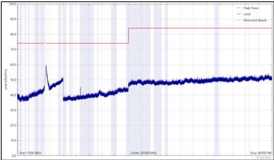
Figure 1093 - U-NII-2A - 5320 MHz (CH64), HT20, CDD, Core 0 + Core 1, 1 GHz to 40 GHz, Horizontal (Peak)
