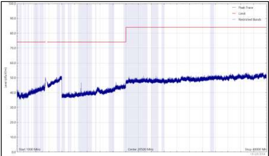
Figure 1099 - U-NII-2C - 5500 MHz (CH100), HT20, CDD, Core 0 + Core 1, 1 GHz to 40 GHz, Vertical (Peak)
