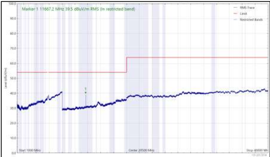
Figure 1142 - 5825 MHz (CH165), HE20, RU26-8, Core 0 + Core 1, 1 GHz to 40 GHz, Vertical (RMS)
