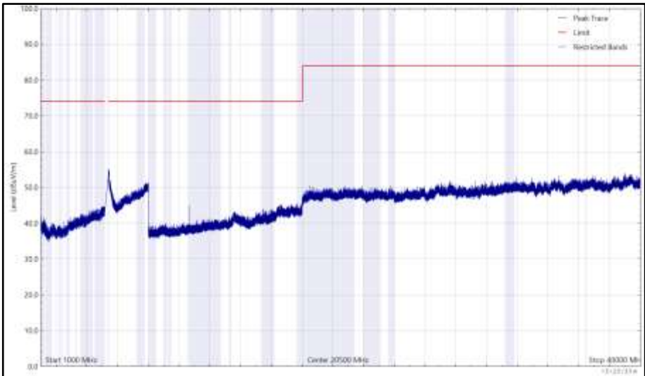
Figure 1121 - 5320 MHz (CH64), HE20, RU52-37, Core 0 + Core 1, 1 GHz to 40 GHz, Horizontal (Peak)
