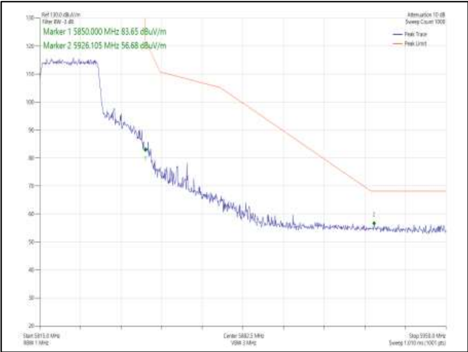
Figure 928 - 802.11ax HE20 SDM, Cores 0-1, SU - 5825 MHz Band Edge Frequency 5850 MHz
