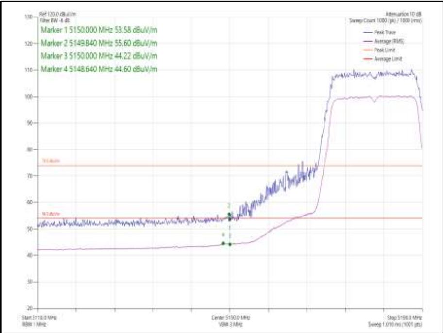
Figure 1014 - 802.11n HT20 CDD, Cores 0-1 - 5180 MHz Band Edge Frequency 5150 MHz
