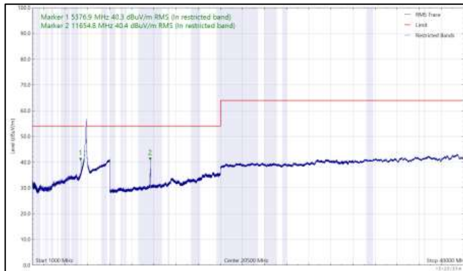
Figure 1111 - U-NII-3 - 5825 MHz (CH165), HT20, CDD, Core 0 + Core 1, 1 GHz to 40 GHz, Horizontal (RMS)
