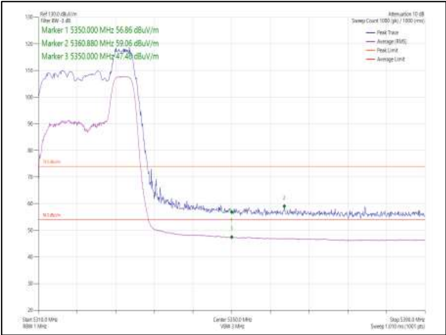
Figure 1009 - 802.11ax HE20, Core 0, 52-40 - 5320 MHz, Band Edge Frequency 5350 MHz
