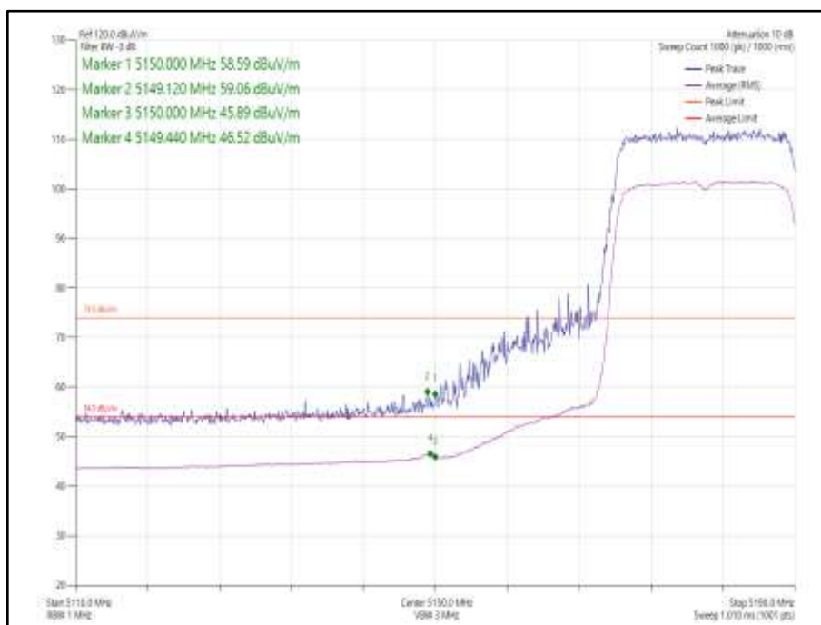
Figure 1018 - 802.11ax HE20 SDM, Cores 0-1, SU - 5180 MHz Band Edge Frequency 5150 MHz
