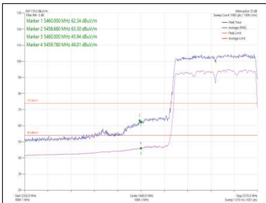
Figure 1080 - 802.11ac VHT80 CDD, Cores 0-1- 5530 MHz Band Edge Frequency 5460 MHz
