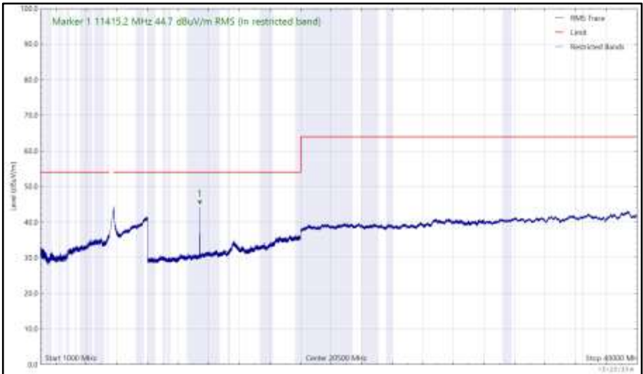
Figure 1132 - 5700 MHz (CH140), HE20, RU52-40, Core 0 + Core 1, 1 GHz to 40 GHz, Vertical (RMS)
