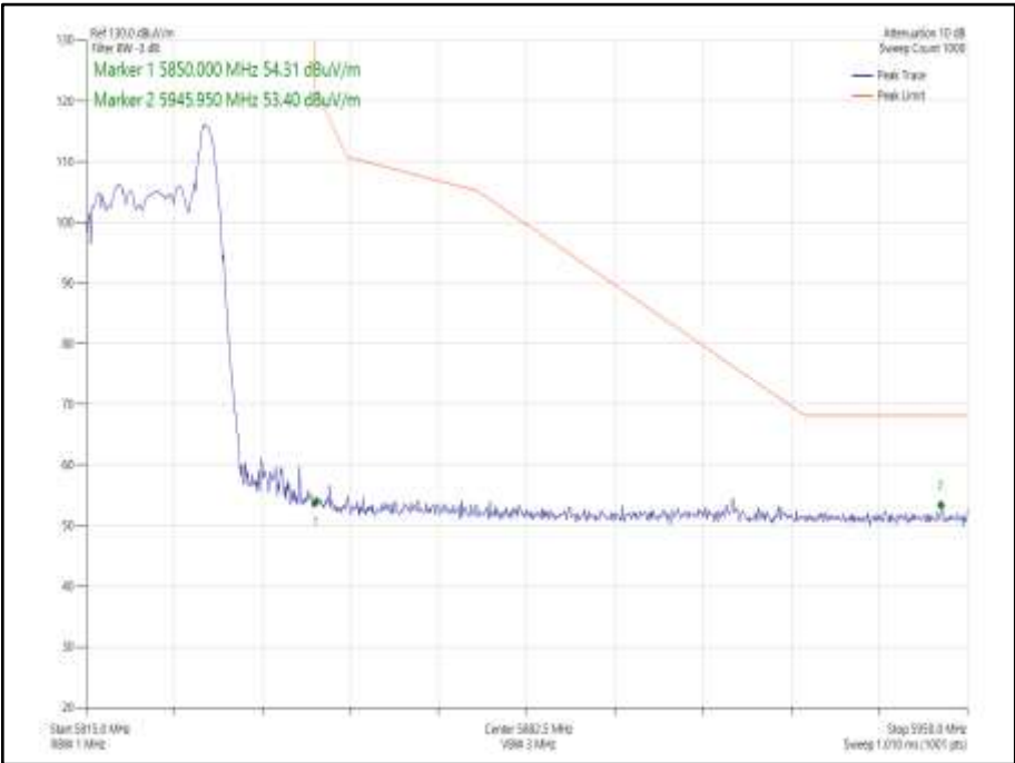
Figure 927 - 802.11ax HE20 CDD, Cores 0-1, 26-8 - 5825 MHz Band Edge Frequency 5850 MHz
