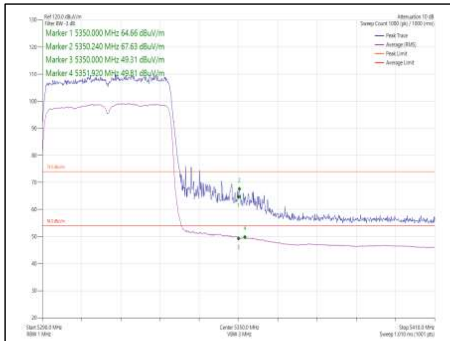
Figure 1051 - 802.11ax HE40 SDM, Cores 0-1, SU - 5310 MHz Band Edge Frequency 5350 MHz
