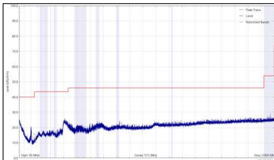
Figure 1140 - 5825 MHz (CH165), HE20, RU26-8, Core 0 + Core 1, 30 MHz to 1 GHz, Vertical (Peak)
