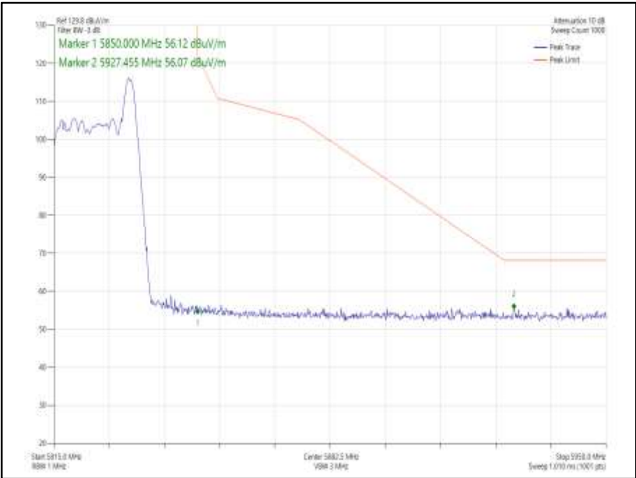
Figure 905 - 802.11ax HE20, Core 0, 26-8 - 5825 MHz Band Edge Frequency 5850 MHz
