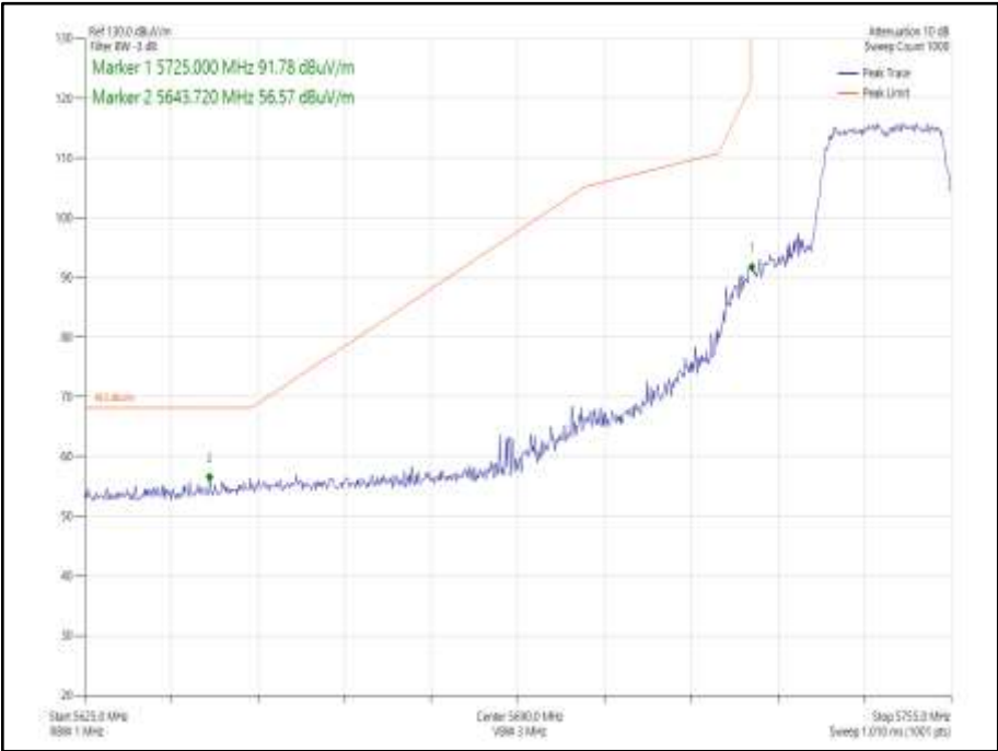
Figure 918 - 802.11n HT20 CDD, Cores 0-1 - 5745 MHz Band Edge Frequency 5725 MHz
