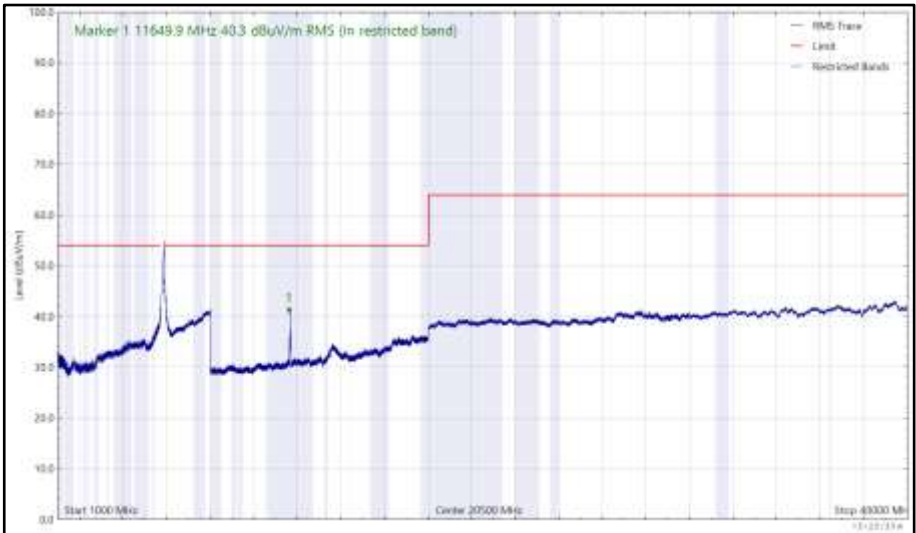
Figure 1114 - U-NII-3 - 5825 MHz (CH165), HT20, CDD, Core 0 + Core 1, 1 GHz to 40 GHz, Vertical (RMS)
