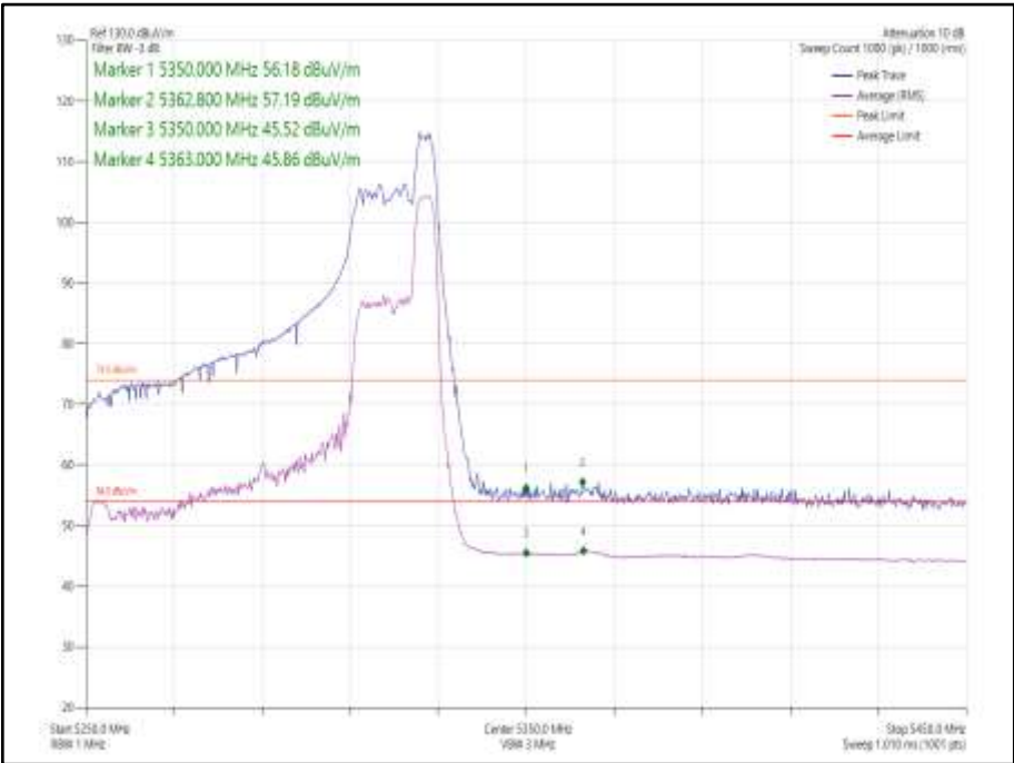
Figure 1065 - 802.11ax HE80, Core 0, 52-52 - 5290 MHz Band Edge Frequency 5350 MHz
