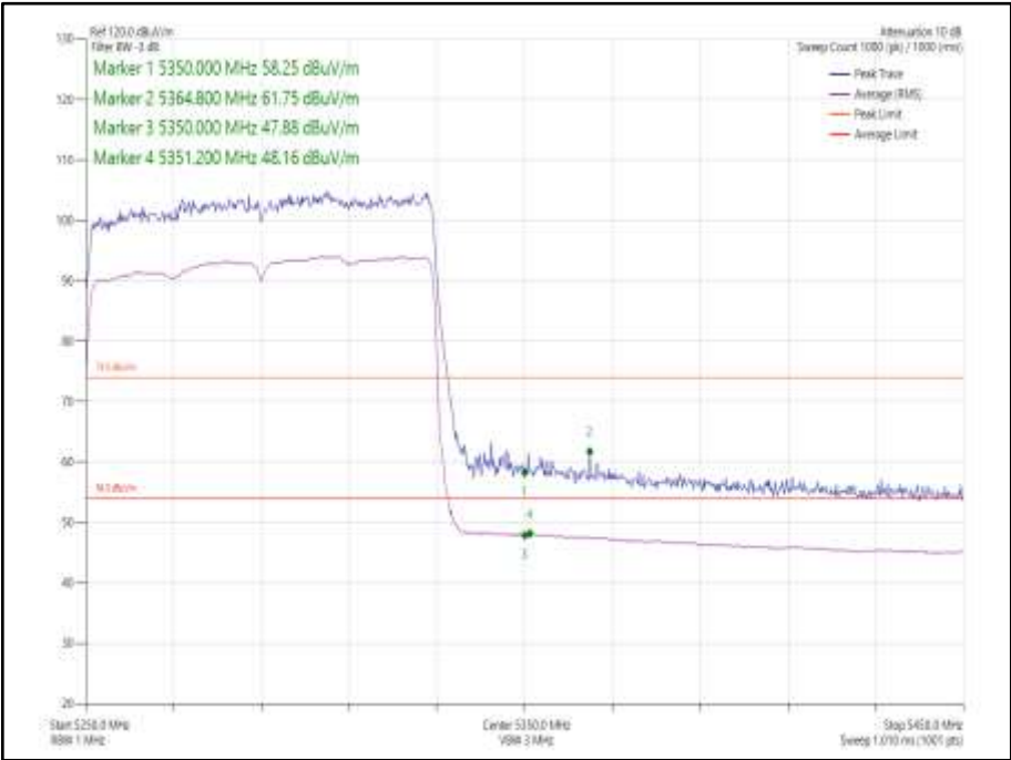
Figure 1064 - 802.11ax HE80, Core 0, SU - 5290 MHz Band Edge Frequency 5350 MHz
