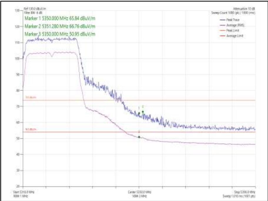
Figure 1021 - 802.11n HT20 SDM, Cores 0-1 - 5320 MHz Band Edge Frequency 5350 MHz
