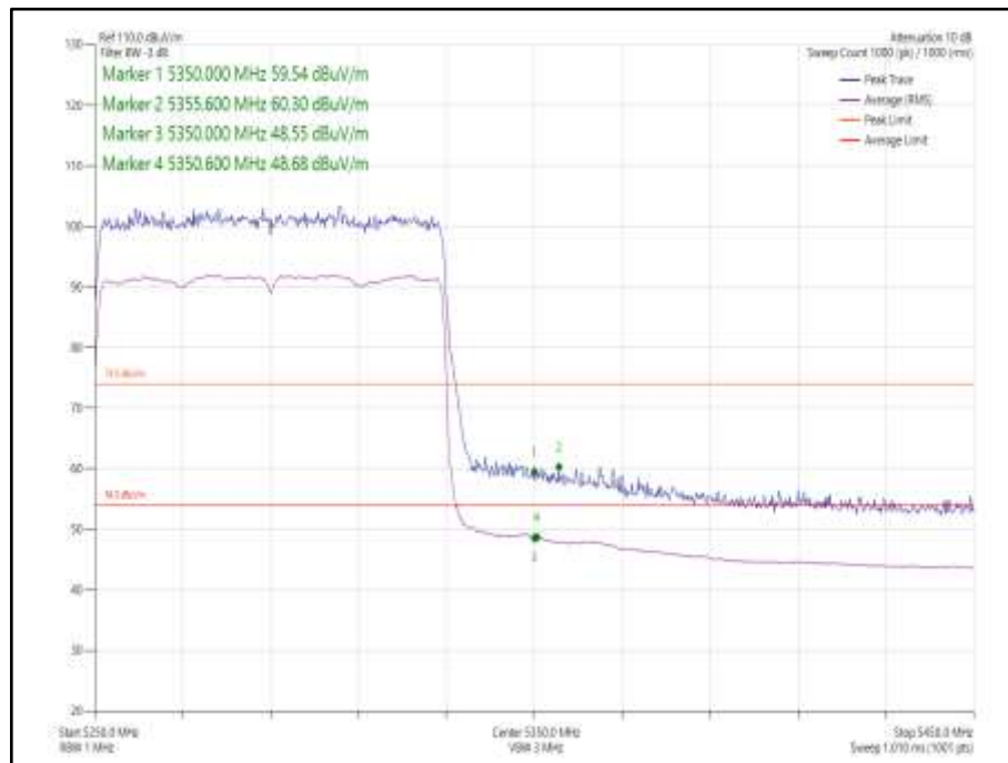
Figure 1076 - 802.11ax HE80 CDD, Cores 0-1, SU - 5290 MHz Band Edge Frequency 5350 MHz
