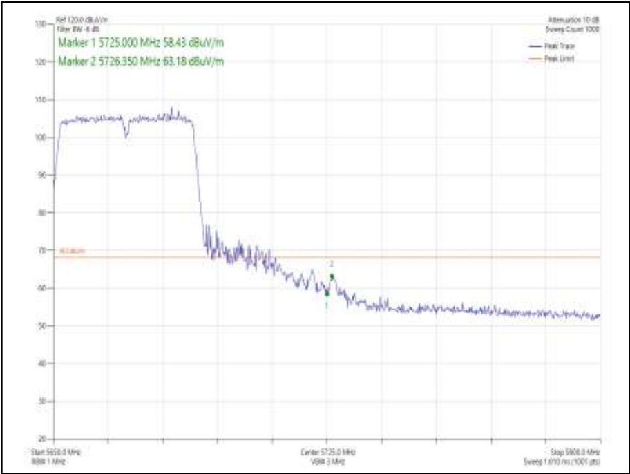
Figure 931 - 802.11n HT40, Core 0 - 5670 MHz Band Edge Frequency 5725 MHz
