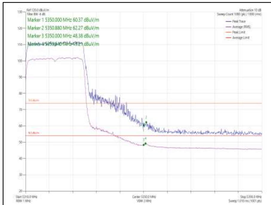
Figure 1022 - 802.11ax HE20 CDD, Cores 0-1, SU - 5320 MHz Band Edge Frequency 5350 MHz
