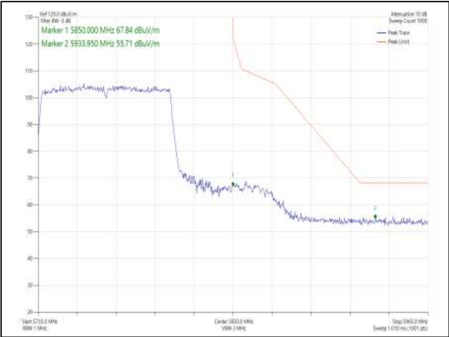
Figure 996 - 802.11ac VHT80 CDD, Cores 0-1 - 5775 MHz Band Edge Frequency 5850 MHz
