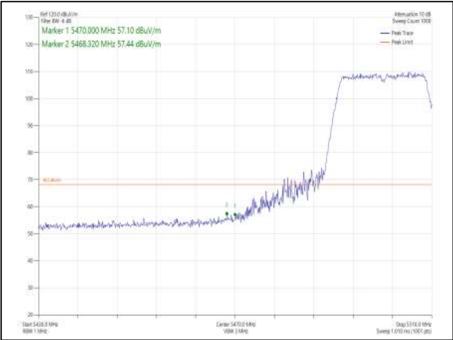
Figure 906 - 802.11n HT20 CDD, Cores 0-1 - 5500 MHz Band Edge Frequency 5470 MHz
