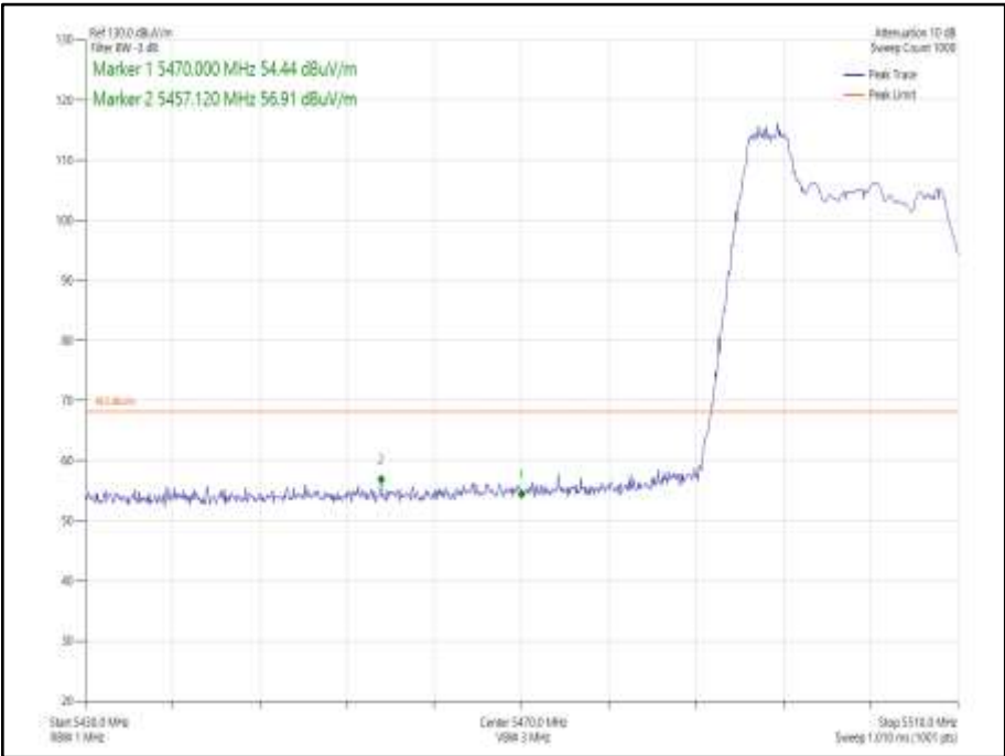
Figure 911 - 802.11ax HE20 SDM, Cores 0-1 52-37 - 5500 MHz Band Edge Frequency 5470 MHz
