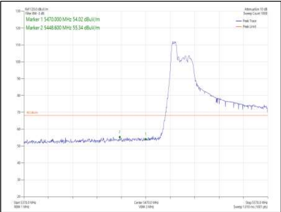
Figure 981 - 802.11ax HE80 CDD, Cores 0-1, 52-37- 5530 MHz Band Edge Frequency 5470 MHz
