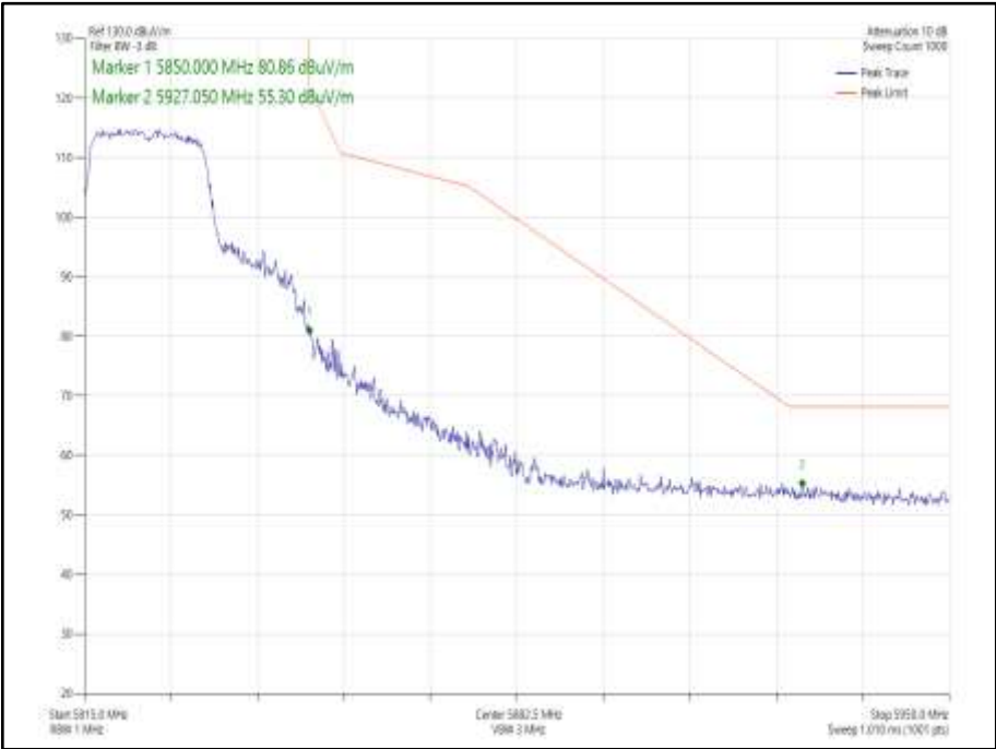
Figure 924 - 802.11n HT20 CDD, Cores 0-1 - 5825 MHz Band Edge Frequency 5850 MHz
