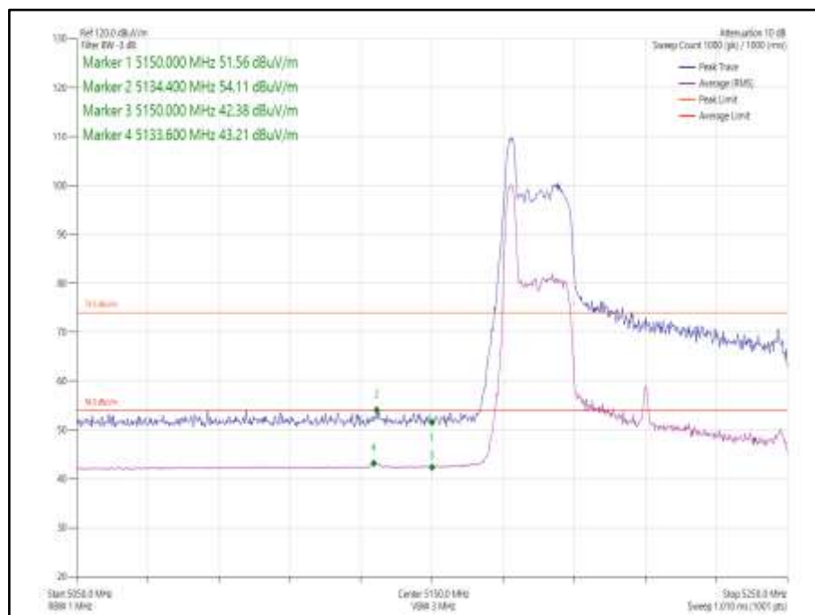
Figure 1071 - 802.11ax HE80 CDD, Cores 0-1, 26-0 - 5210 MHz Band Edge Frequency 5150 MHz
