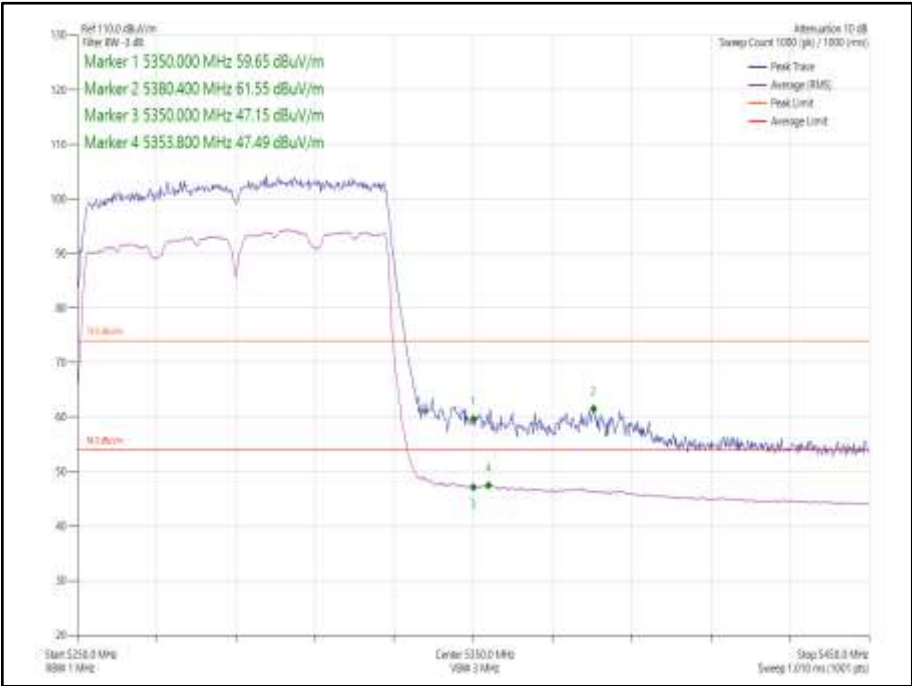
Figure 1060 - 802.11ac VHT80, Core 0 - 5290 MHz Band Edge Frequency 5350 MHz
