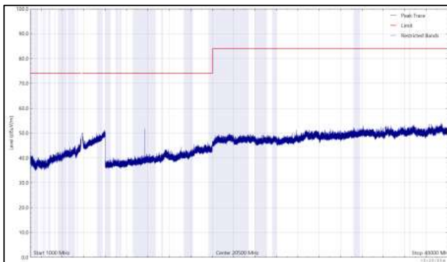
Figure 1138 - 5825 MHz (CH165), HE20, RU26-8, Core 0 + Core 1, 1 GHz to 40 GHz, Horizontal (Peak)
