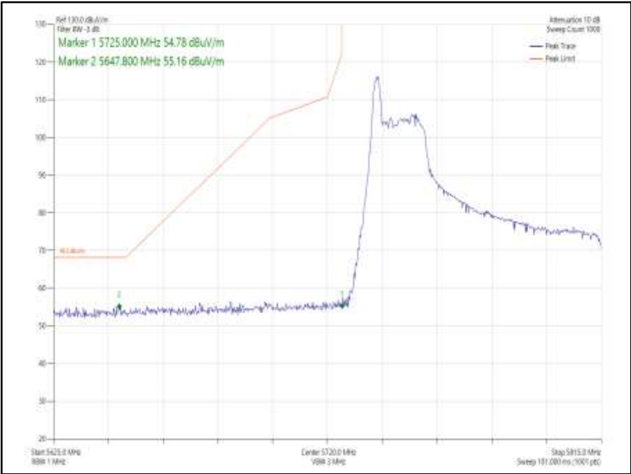
Figure 975 - 802.11ax HE80 Core 0 26-0 - 5775 MHz Band Edge Frequency 5725 MHz
