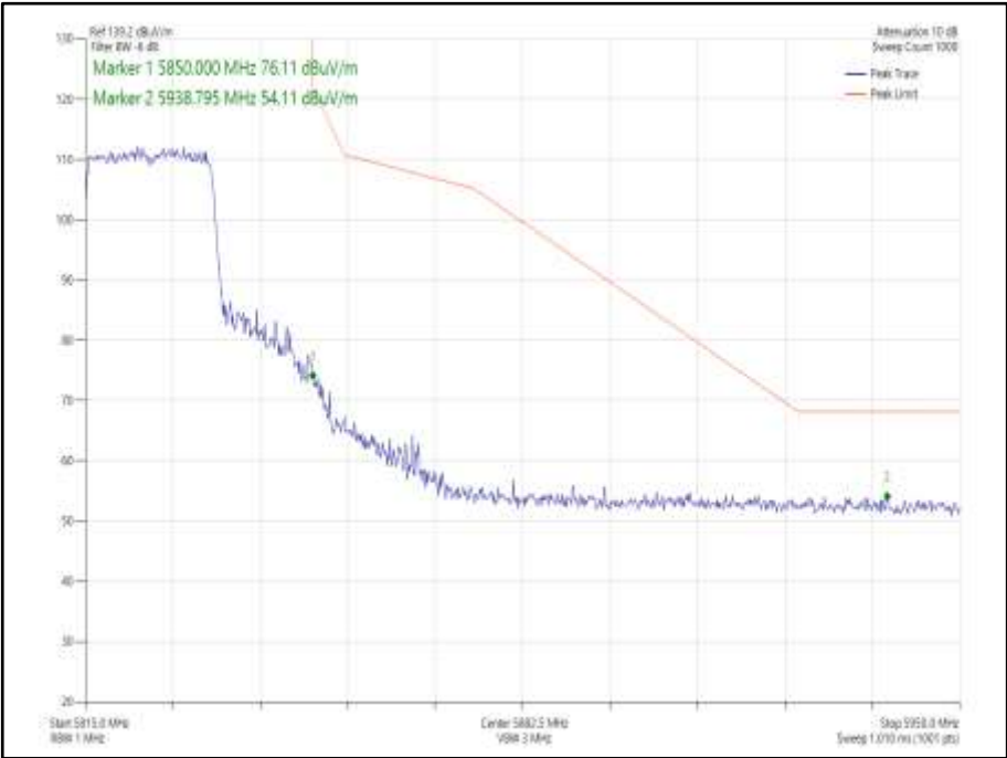
Figure 904 - 802.11ax HE20, Core 0, SU - 5825 MHz Band Edge Frequency 5850 MHz
