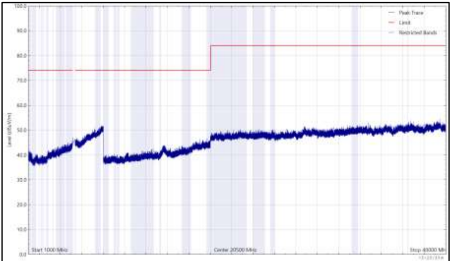
Figure 1119 - 5180 MHz (CH36), HE20, RU26-0, Core 0 + Core 1, 1 GHz to 40 GHz, Vertical (Peak)
