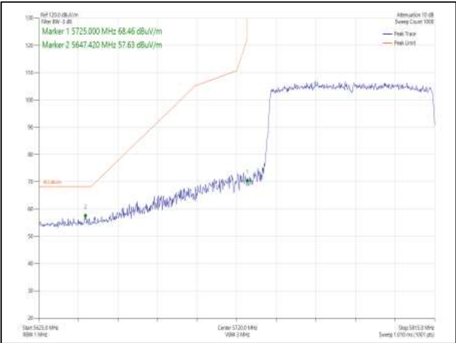
Figure 974 - 802.11ax HE80 Core 0 SU - 5775 MHz Band Edge Frequency 5725 MHz
