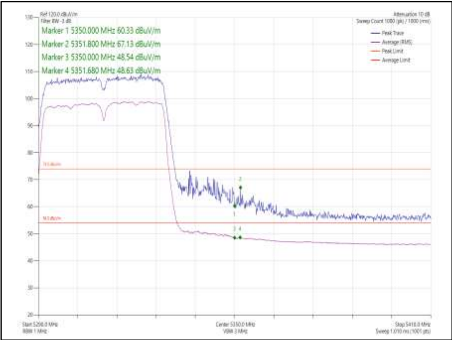
Figure 1047 - 802.11n HT40 CDD, Cores 0-1 - 5310 MHz Band Edge Frequency 5350 MHz
