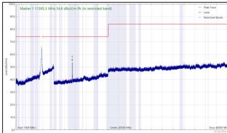
Figure 1101 - U-NII-2C - 5700 MHz (CH140), HT20, CDD, Core 0 + Core 1, 1 GHz to 40 GHz, Horizontal (Peak)
