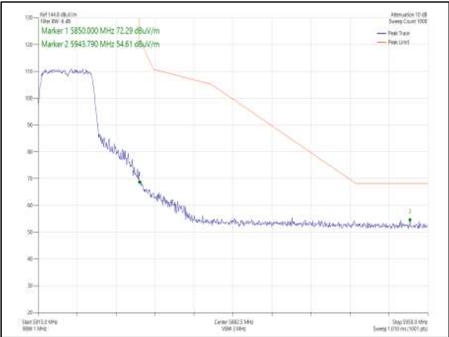
Figure 903 - 802.11n HT20, Core 0 - 5825 MHz Band Edge Frequency 5850 MHz
