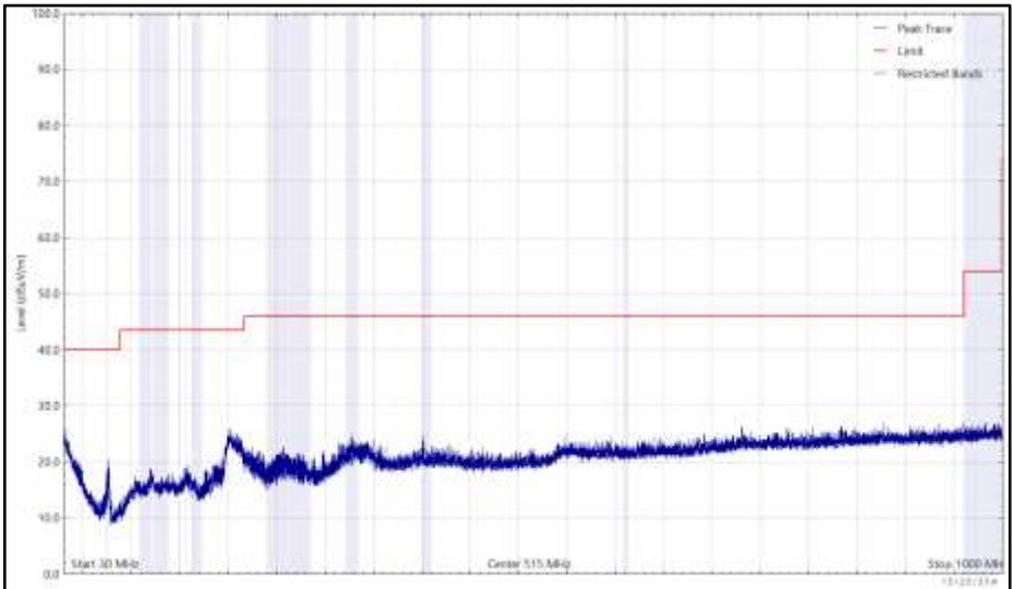
Figure 1118 - 5180 MHz (CH36), HE20, RU26-0, Core 0 + Core 1, 30 MHz to 1 GHz, Vertical (Peak)
