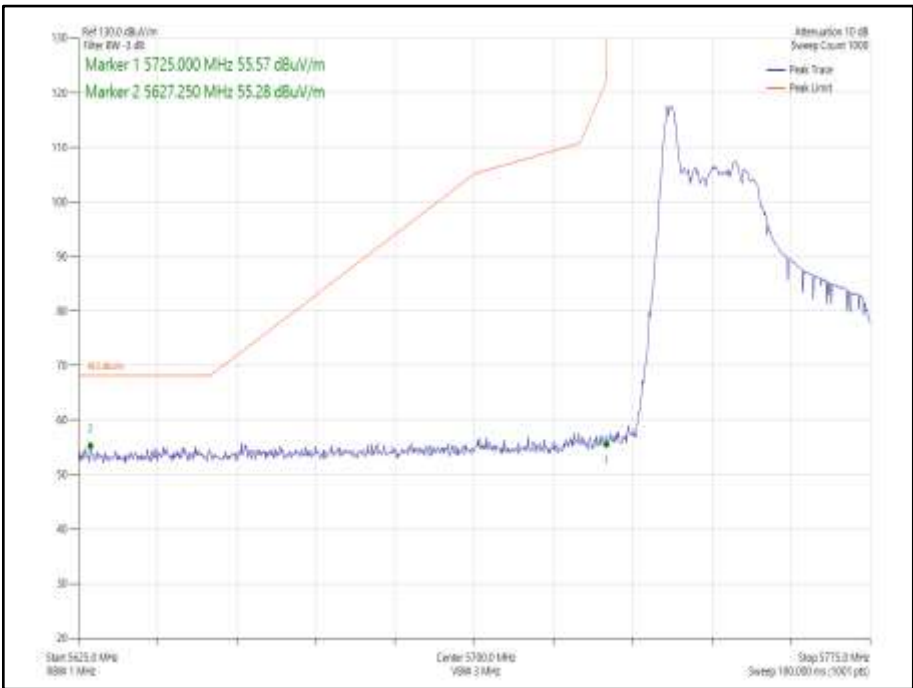
Figure 957 - 802.11ax HE40 CDD, Cores 0-1, 26-0 - 5755 MHz Band Edge Frequency 5725 MHz
