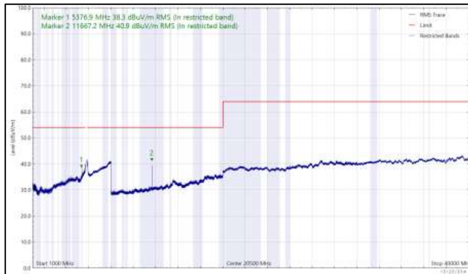
Figure 1139 - 5825 MHz (CH165), HE20, RU26-8, Core 0 + Core 1, 1 GHz to 40 GHz, Horizontal (RMS)
