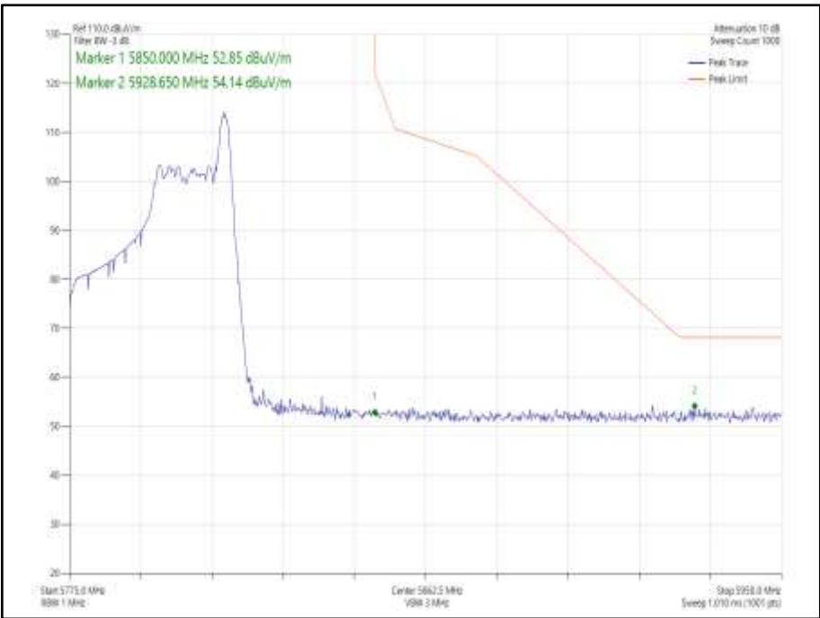
Figure 965 - 802.11ax HE40 SDM, Cores 0-1, 26-17 - 5795 MHz Band Edge Frequency 5850 MHz
