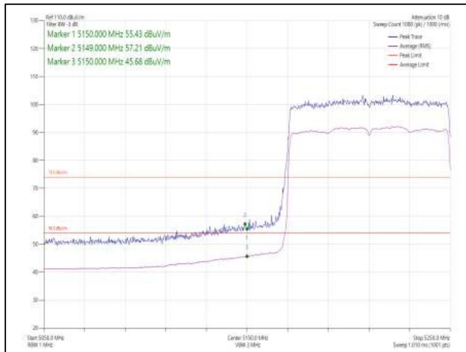
Figure 1070 - 802.11ax HE80 CDD, Cores 0-1, SU - 5210 MHz Band Edge Frequency 5150 MHz
