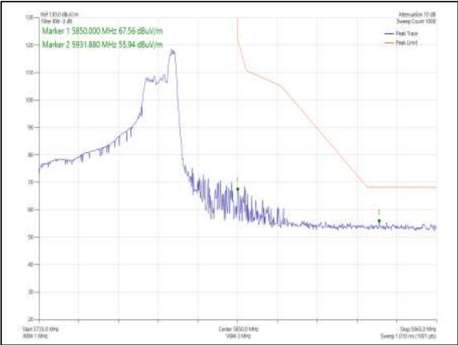
Figure 977 - 802.11ax HE80 Core 0 26-36 - 5775 MHz Band Edge Frequency 5850 MHz
