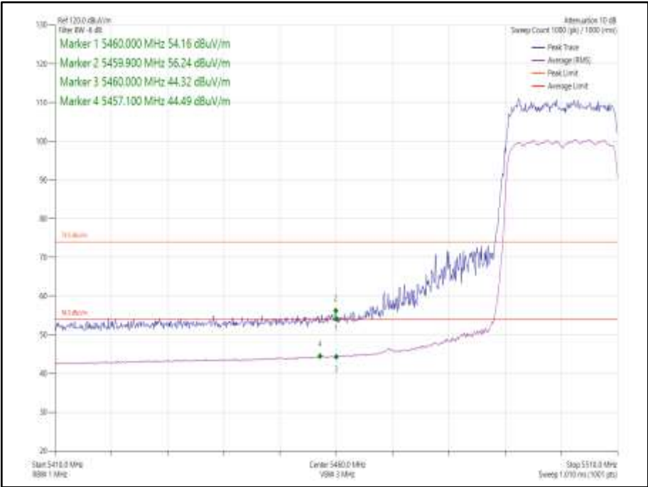
Figure 1028 - 802.11ax HE20 CDD, Cores 0-1, SU- 5500 MHz Band Edge Frequency 5460 MHz
