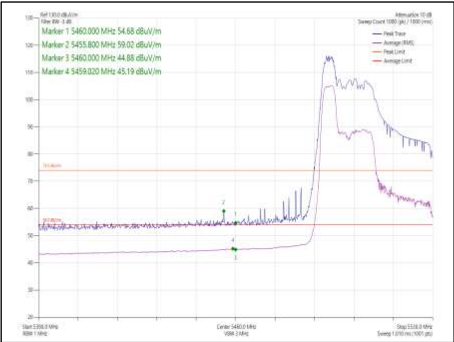
Figure 1040 - 802.11ax HE40, Core 0, 26-0- 5510 MHz Band Edge Frequency 5460 MHz
