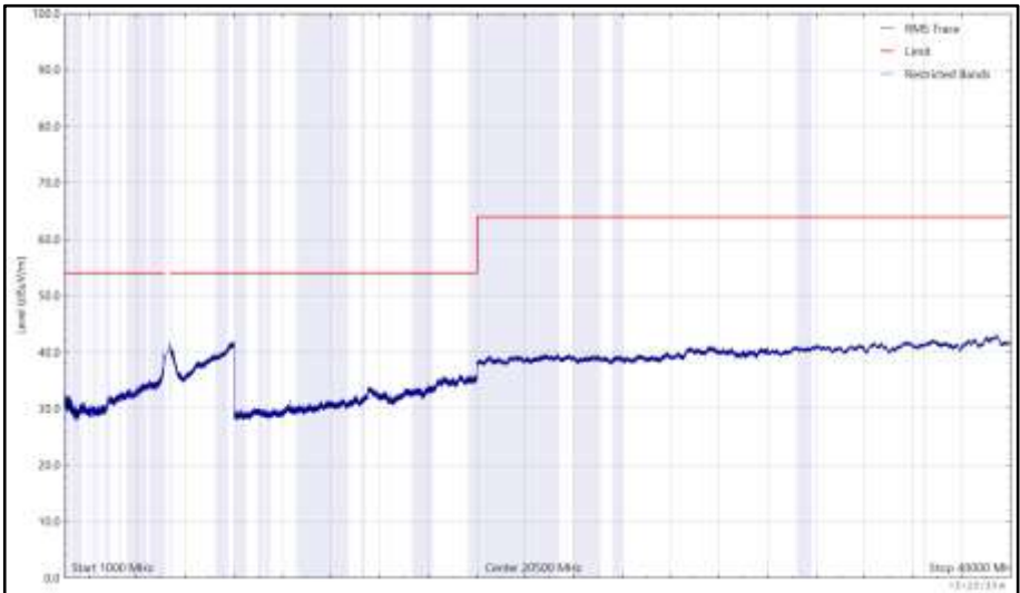
Figure 1117 - 5180 MHz (CH36), HE20, RU26-0, Core 0 + Core 1, 1 GHz to 40 GHz, Horizontal (RMS)
