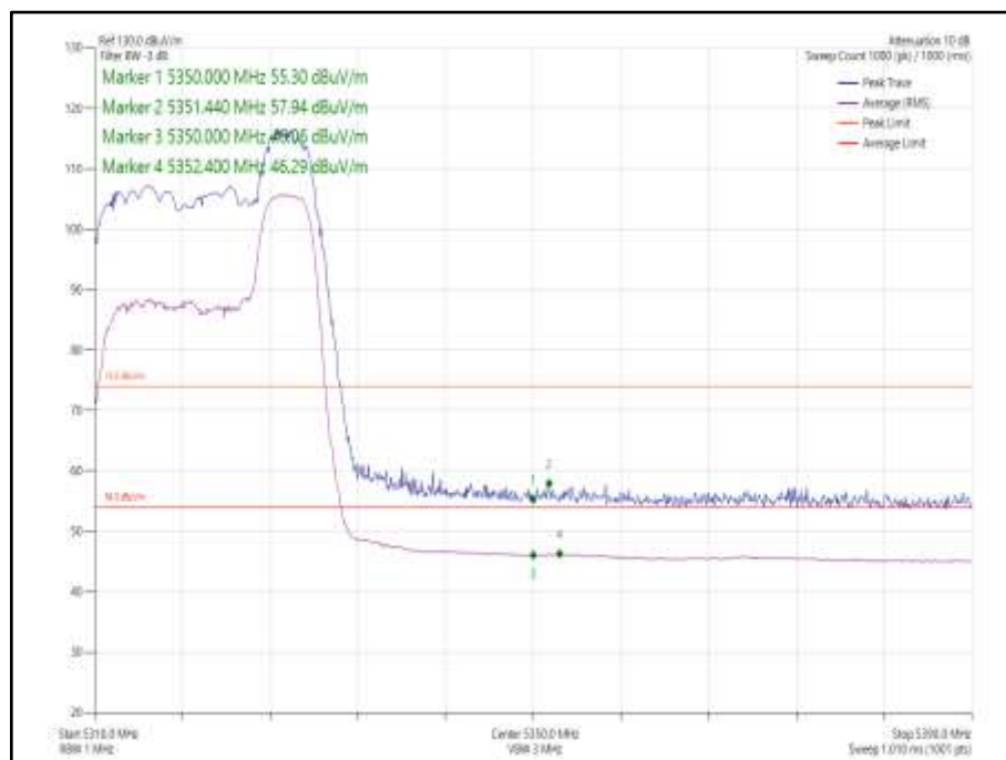
Figure 1025 - 802.11ax HE20 SDM, Cores 0-1, 52-40 - 5320 MHz Band Edge Frequency 5350 MHz
