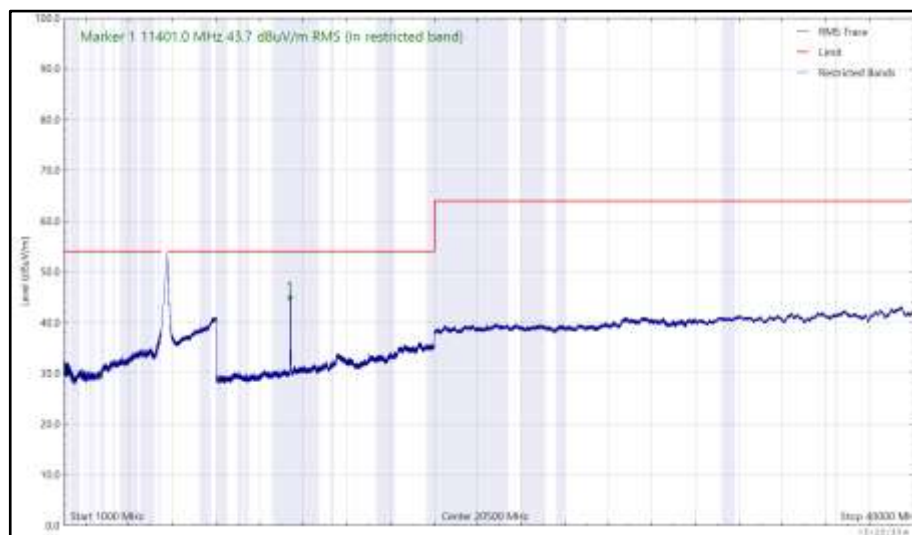
Figure 1102 - U-NII-2C - 5700 MHz (CH140), HT20, CDD, Core 0 + Core 1, 1 GHz to 40 GHz, Horizontal (RMS)
