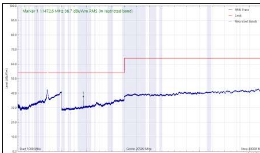
Figure 1134 - 5745 MHz (CH149), HE20, RU26-0, Core 0 + Core 1, 1 GHz to 40 GHz, Horizontal (RMS)
