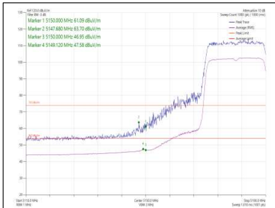
Figure 1004 - 802.11ax HE20, Core 1, SU - 5180 MHz, Band Edge Frequency 5150 MHz
