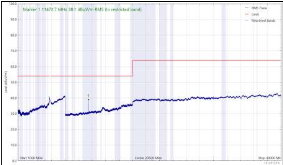
Figure 1136 - 5745 MHz (CH149), HE20, RU26-0, Core 0 + Core 1, 1 GHz to 40 GHz, Vertical (RMS)
