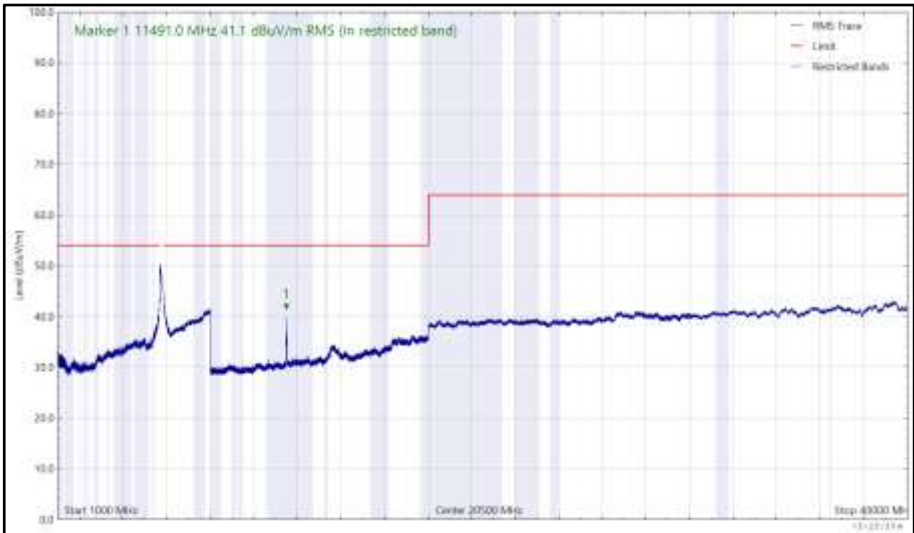
Figure 1108 - U-NII-3 - 5745 MHz (CH149), HT20, CDD, Core 0 + Core 1, 1 GHz to 40 GHz, Vertical (RMS)
