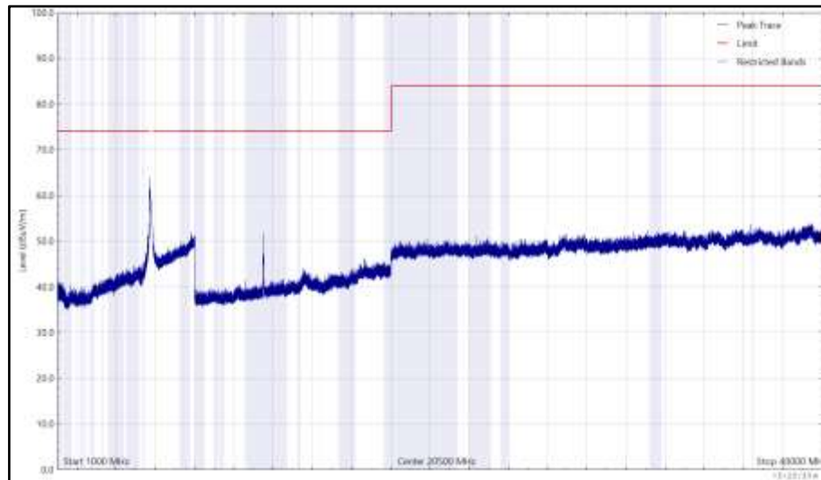
Figure 1105 - U-NII-3 - 5745 MHz (CH149), HT20, CDD, Core 0 + Core 1, 1 GHz to 40 GHz, Horizontal (Peak)
