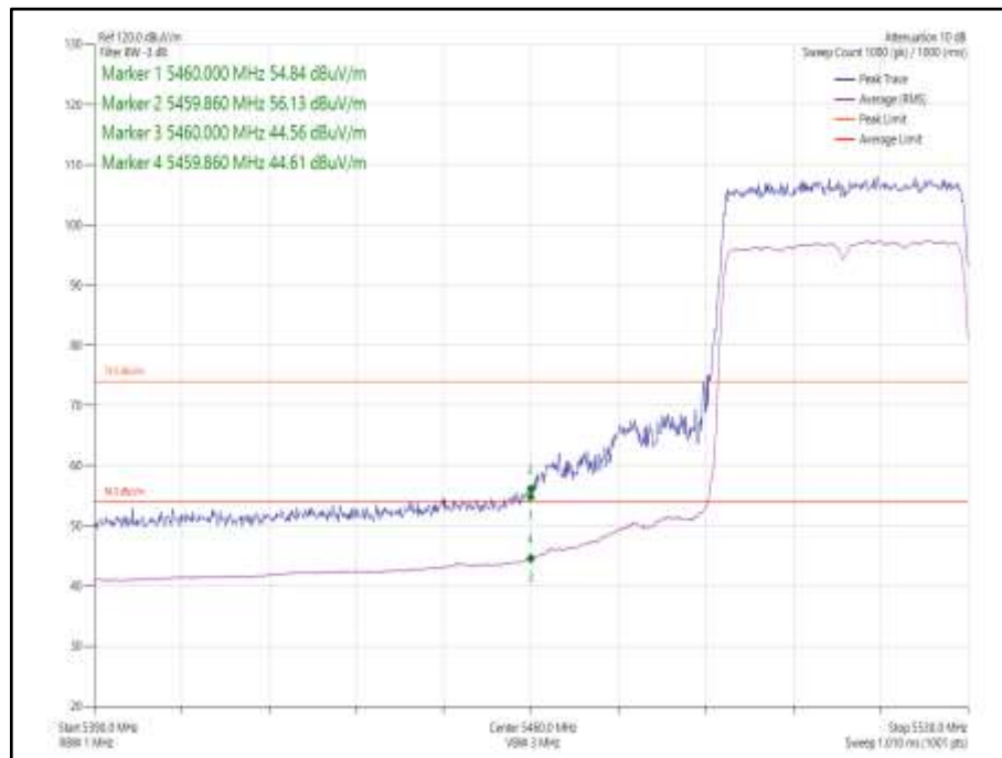
Figure 1055 - 802.11ax HE40 CDD, Cores 0-1, SU - 5510 MHz Band Edge Frequency 5460 MHz
