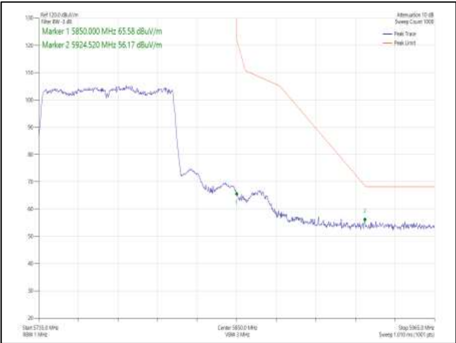
Figure 997 - 802.11ac VHT80 SDM, Cores 0-1 - 5775 MHz Band Edge Frequency 5850 MHz
