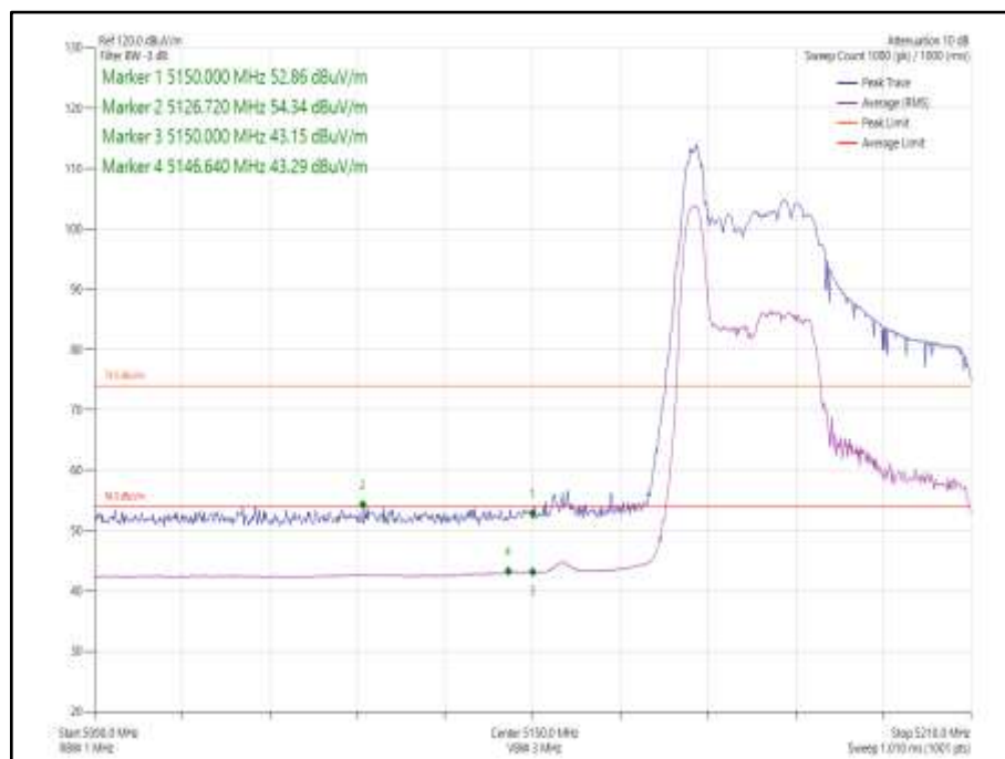
Figure 1034 - 802.11ax HE40, Core 1, 26-0 - 5190 MHz Band Edge Frequency 5150 MHz
