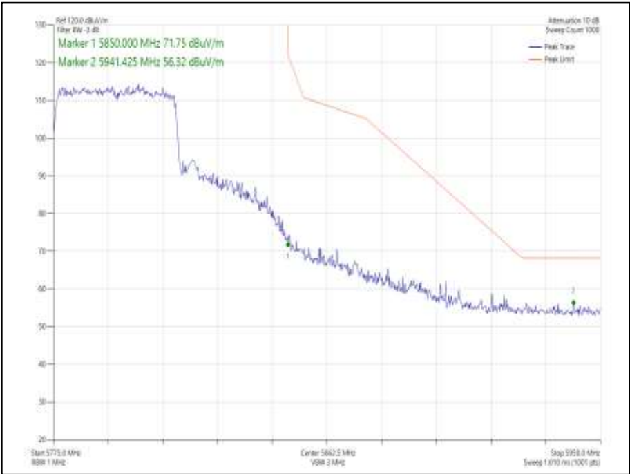
Figure 940 - 802.11ax HE40, Core 0, SU - 5795 MHz Band Edge Frequency 5850 MHz
