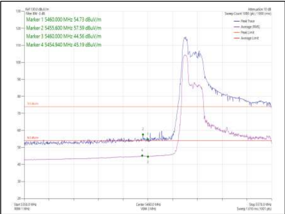
Figure 1085 - 802.11ax HE80 SDM, Cores 0-1, 52-37 - 5530 MHz Band Edge Frequency 5460 MHz
