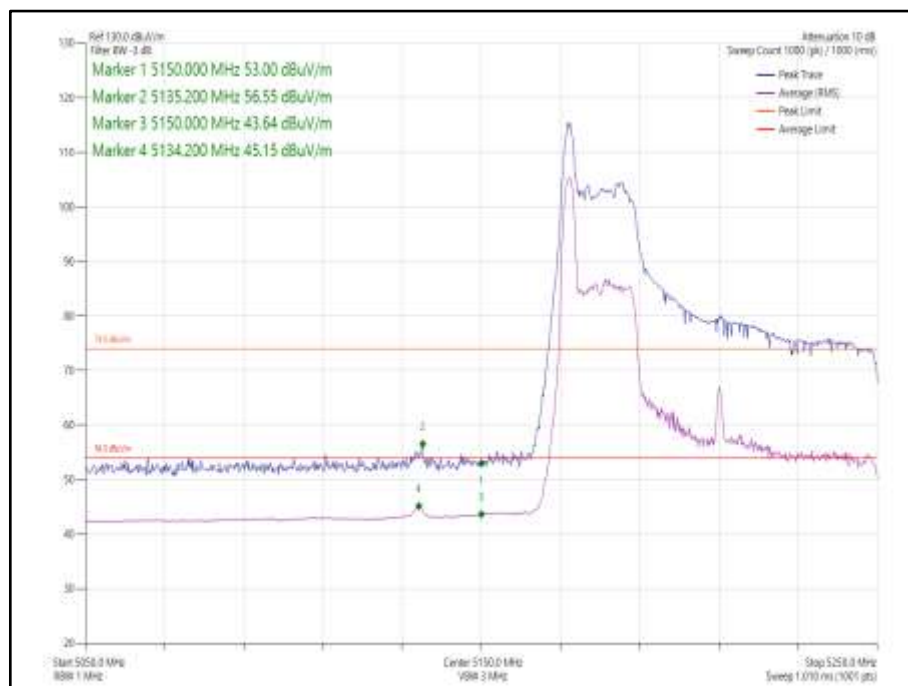
Figure 1063 - 802.11ax HE80, Core 1, 26-0 - 5210 MHz Band Edge Frequency 5150 MHz
