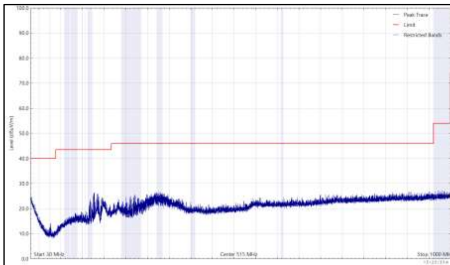
Figure 1109 - U-NII-3 - 5825 MHz (CH165), HT20, CDD, Core 0 + Core 1, 30 MHz to 1 GHz, Horizontal (Peak)
