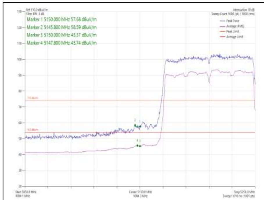
Figure 1068 - 802.11ac VHT80 CDD, Cores 0-1- 5210 MHz Band Edge Frequency 5150 MHz
