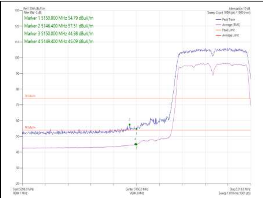
Figure 1042 - 802.11n HT40 SDM Cores 0-1 - 5190 MHz Band Edge Frequency 5150 MHz
