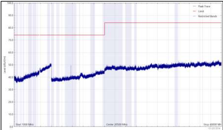
Figure 1141 - 5825 MHz (CH165), HE20, RU26-8, Core 0 + Core 1, 1 GHz to 40 GHz, Vertical (Peak)
