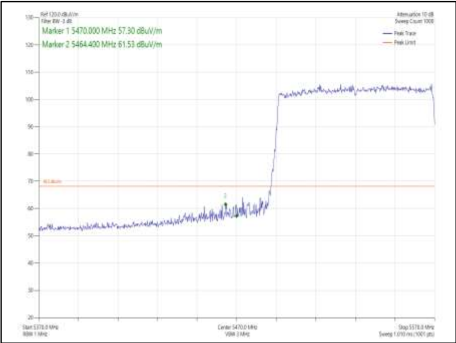
Figure 980 - 802.11ax HE80 CDD, Cores 0-1, SU - 5530 MHz Band Edge Frequency 5470 MHz
