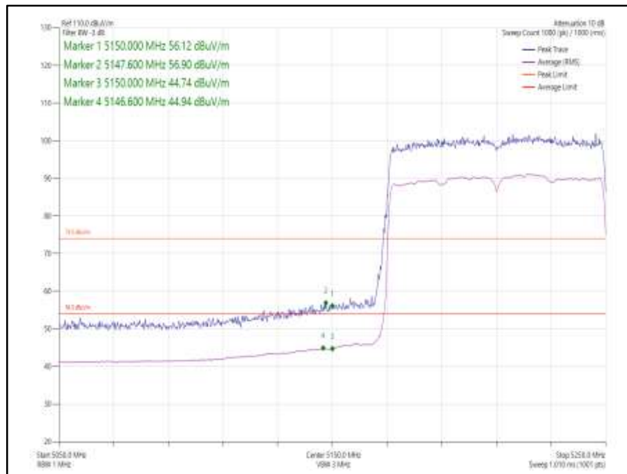
Figure 1072 - 802.11ax HE80 SDM, Cores 0-1, SU - 5210 MHz Band Edge Frequency 5150 MHz
