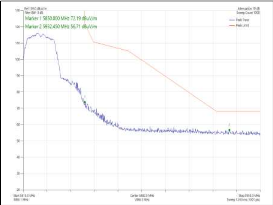
Figure 902 - 802.11a, Core 0, - 5825 MHz Band Edge Frequency 5850 MHz
