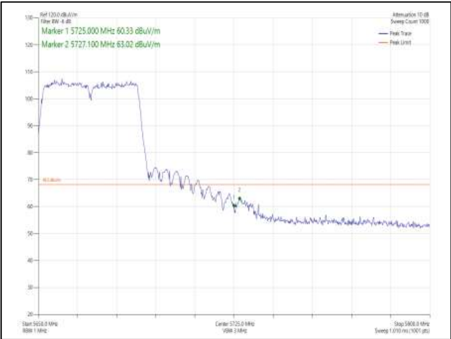
Figure 949 - 802.11n HT40 SDM, Cores 0-1 - 5670 MHz Band Edge Frequency 5725 MHz
