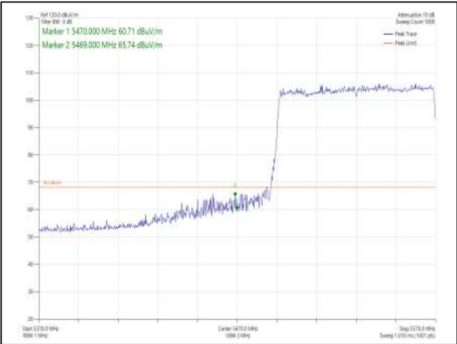
Figure 970 - 802.11ax HE80 Core 0 SU - 5530 MHz Band Edge Frequency 5470 MHz
