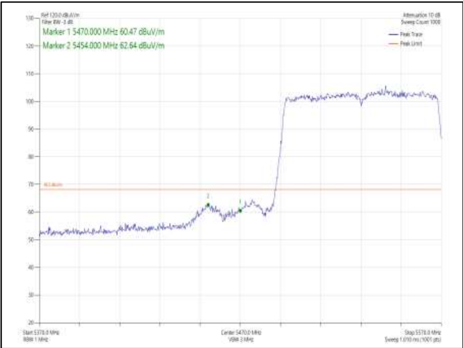
Figure 979 - 802.11ac VHT80 SDM, Cores 0-1 - 5530 MHz Band Edge Frequency 5470 MHz
