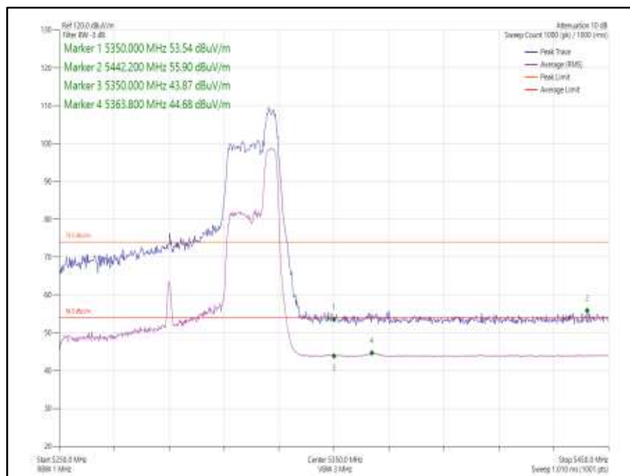
Figure 1077 - 802.11ax HE80 CDD, Cores 0-1, 52-52- 5290 MHz Band Edge Frequency 5350 MHz
