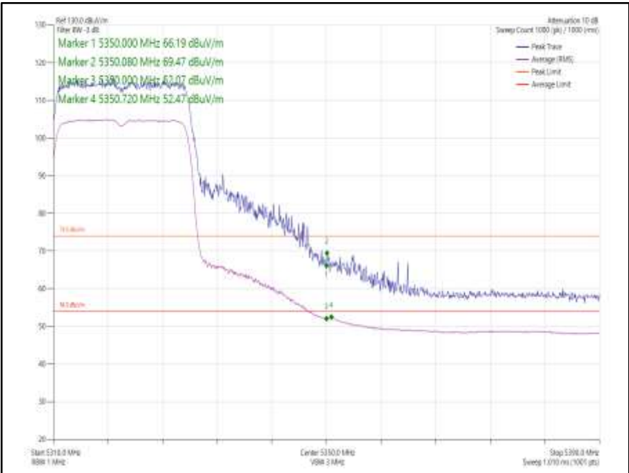
Figure 1008 - 802.11ax HE20, Core 0, SU - 5320 MHz, Band Edge Frequency 5350 MHz
