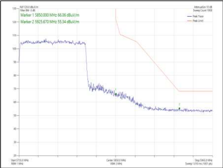
Figure 1000 - 802.11ax HE80 SDM, Cores 0-1, SU -- 5775 MHz Band Edge Frequency 5850 MHz
