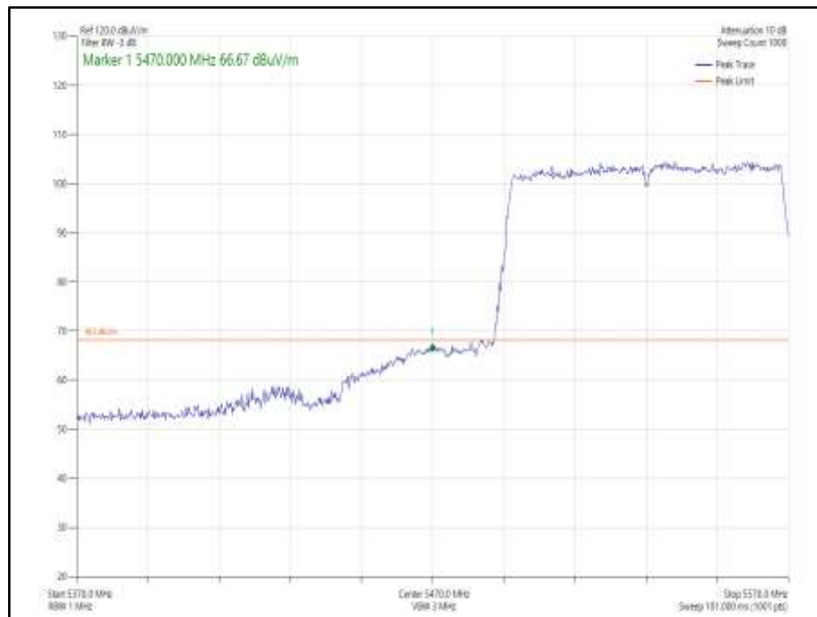
Figure 966 - 802.11ac VHT80 Core 0 - 5530 MHz Band Edge Frequency 5470 MHz
