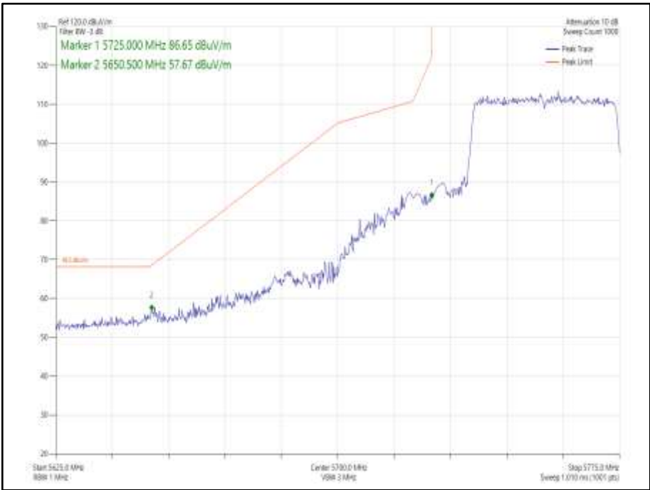
Figure 956 - 802.11ax HE40 CDD, Cores 0-1, SU - 5755 MHz Band Edge Frequency 5725 MHz
