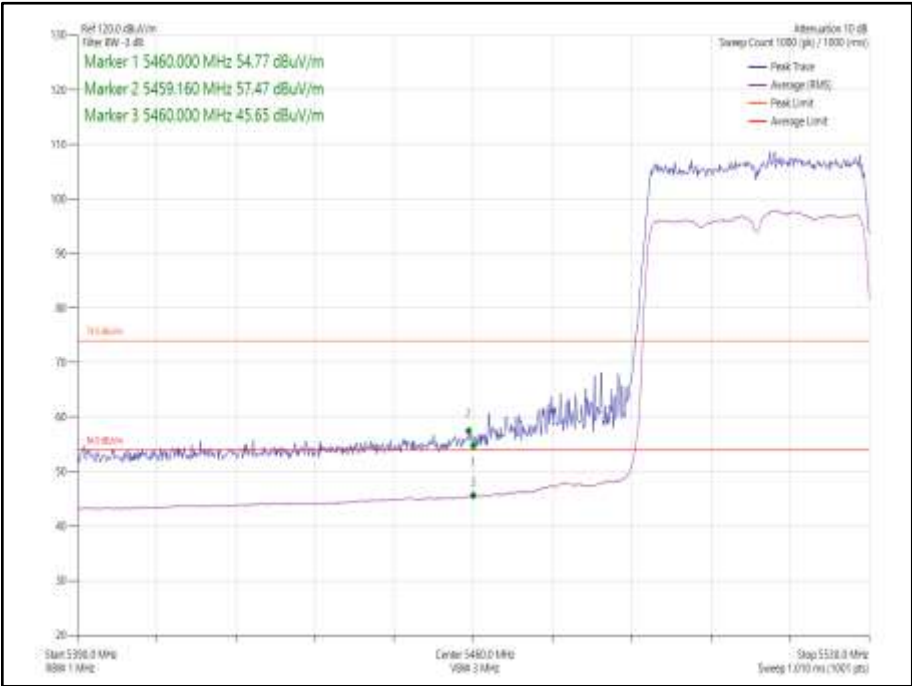
Figure 1057 - 802.11ax HE40 SDM, Cores 0-1, SU - 5510 MHz Band Edge Frequency 5460 MHz
