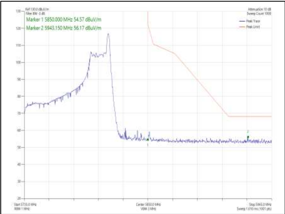
Figure 999 - 802.11ax HE80 CDD, Cores 0-1, 26-36 - 5775 MHz Band Edge Frequency 5850 MHz
