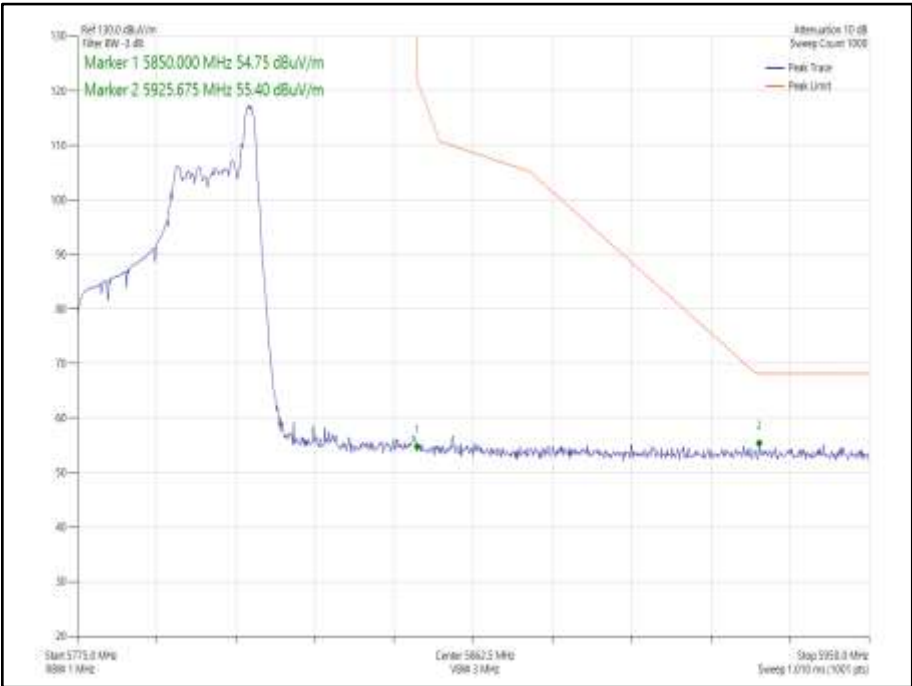
Figure 963 - 802.11ax HE40 CDD, Cores 0-1, 26-17 - 5795 MHz Band Edge Frequency 5850 MHz
