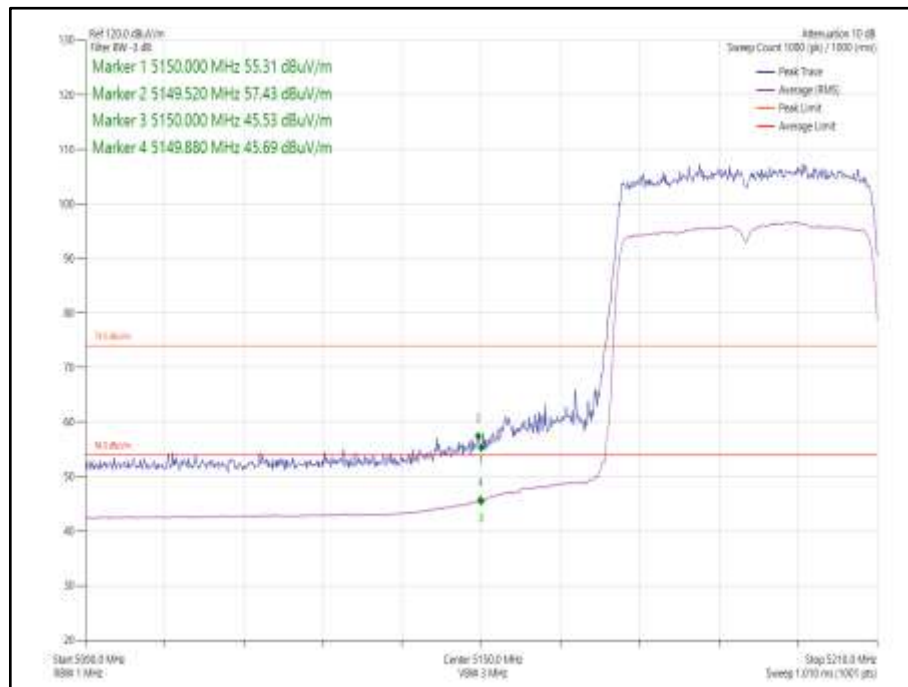
Figure 1033 - 802.11ax HE40, Core 1, SU - 5190 MHz Band Edge Frequency 5150 MHz
