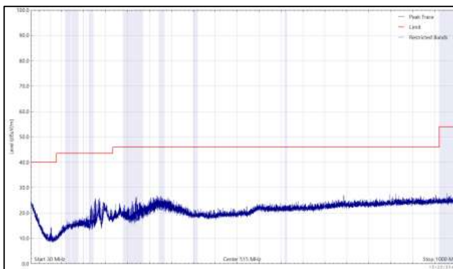
Figure 1115 - 5180 MHz (CH36), HE20, RU26-0, Core 0 + Core 1, 30 MHz to 1 GHz, Horizontal (Peak)
