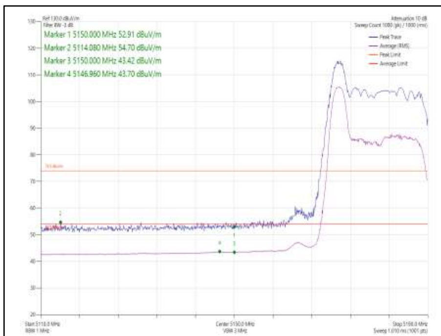
Figure 1005 - 802.11ax HE20, Core 1, 26-0 - 5180 MHz, Band Edge Frequency 5150 MHz
