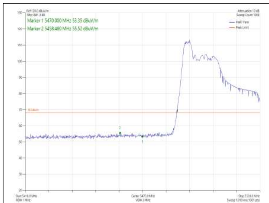
Figure 945 - 802.11ax HE40 CDD, Cores 0-1, 52-37 - 5510 MHz Band Edge Frequency 5470 MHz
