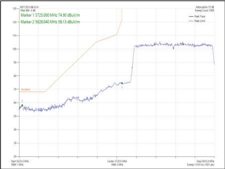
Figure 990 - 802.11ac VHT80 CDD, Cores 0-1 - 5775 MHz Band Edge Frequency 5725 MHz
