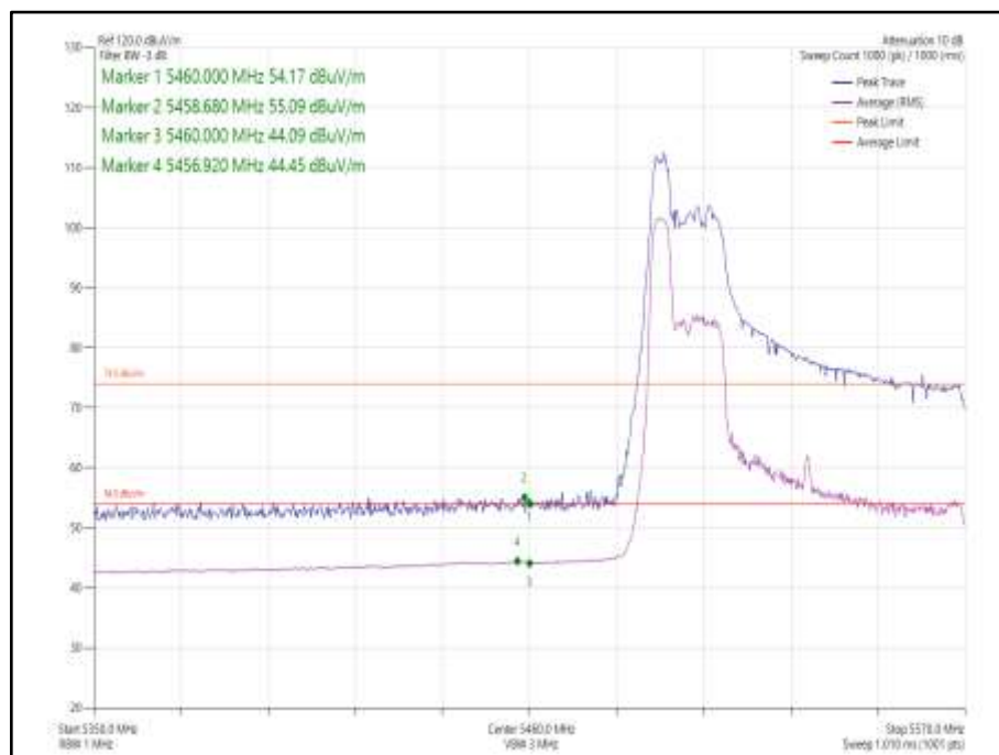
Figure 1083 - 802.11ax HE80 CDD, Cores 0-1, 52-37 - 5530 MHz Band Edge Frequency 5460 MHz
