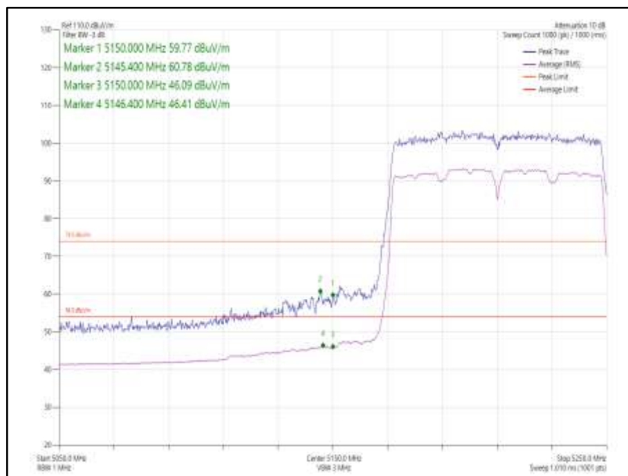
Figure 1059 - 802.11ac VHT80, Core 1 - 5210 MHz Band Edge Frequency 5150 MHz
