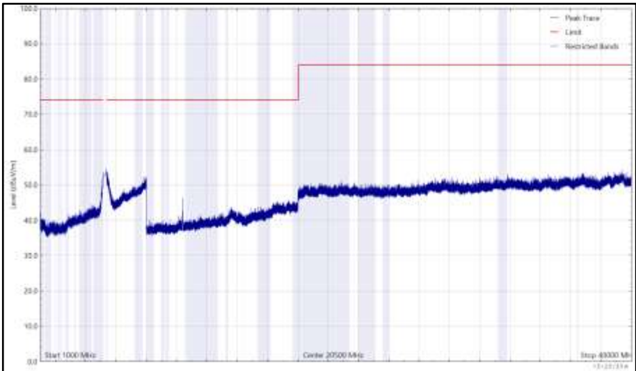
Figure 1088 - U-NII-1 - 5180 MHz (CH36), HT20, CDD, Core 0 + Core 1, 1 GHz to 40 GHz, Horizontal (Peak)
