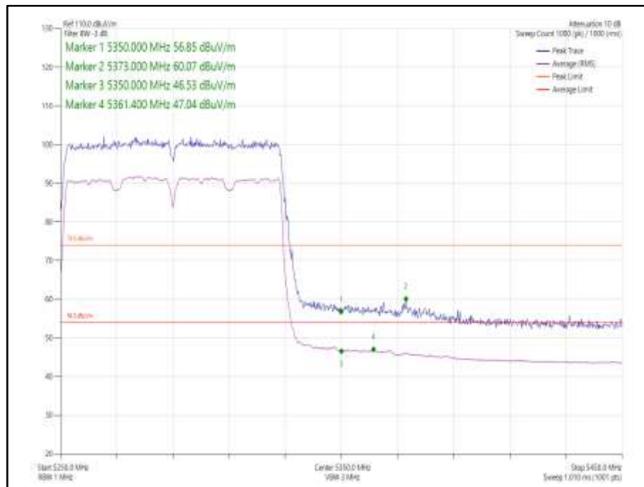
Figure 1074 - 802.11ac VHT80 CDD, Cores 0-1- 5290 MHz Band Edge Frequency 5350 MHz
