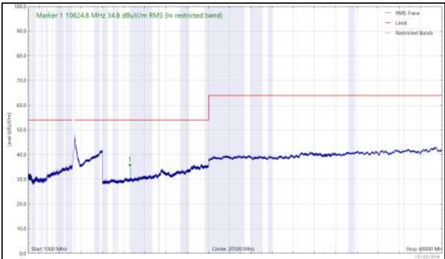
Figure 1122 - 5320 MHz (CH64), HE20, RU52-37, Core 0 + Core 1, 1 GHz to 40 GHz, Horizontal (RMS)
