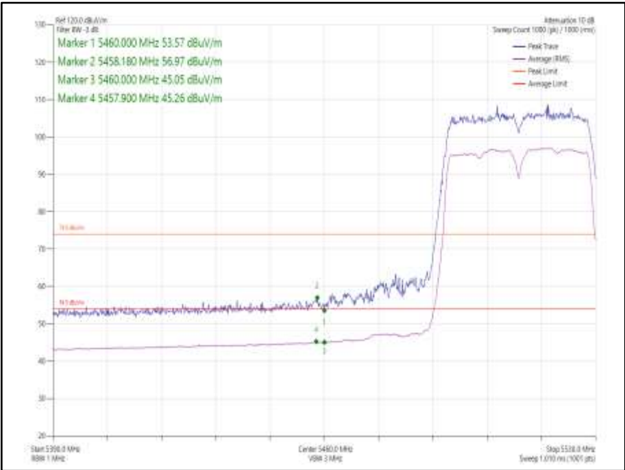
Figure 1054 - 802.11n HT40 SDM, Cores 0-1 - 5510 MHz Band Edge Frequency 5460 MHz
