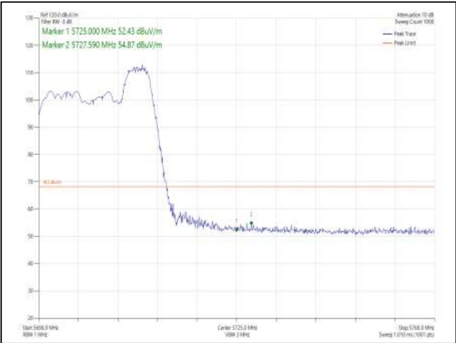
Figure 915 - 802.11ax HE20 CDD, Cores 0-1, 52-40 - 5700 MHz Band Edge Frequency 5725 MHz
