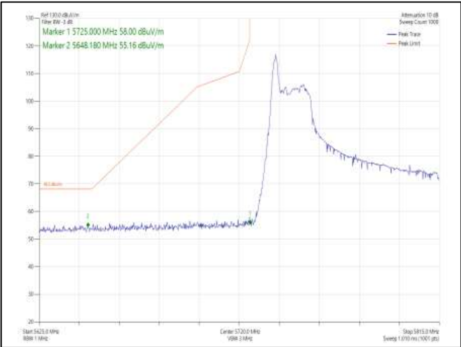
Figure 995 - 802.11ax HE80 SDM, Cores 0-1, 26-0 - 5775 MHz Band Edge Frequency 5725 MHz
