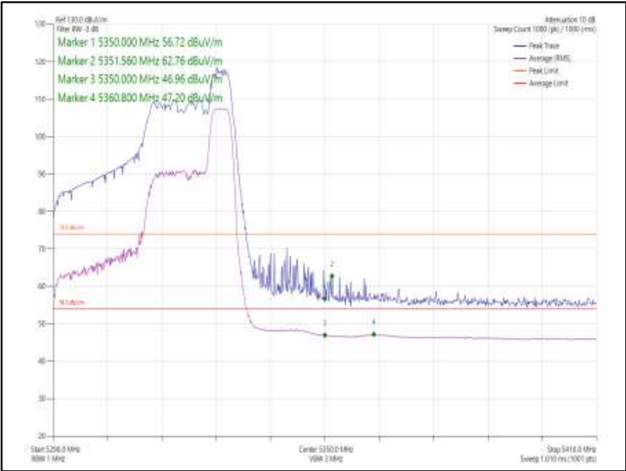
Figure 1037 - 802.11ax HE40, Core 0, 52-40 - 5310 MHz Band Edge Frequency 5350 MHz
