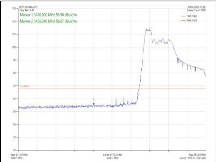
Figure 947 - 802.11ax HE40 SDM, Cores 0-1, 52-37 - 5510 MHz Band Edge Frequency 5470 MHz
