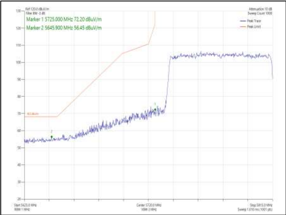
Figure 992 - 802.11ax HE80 CDD, Cores 0-1, SU - 5775 MHz Band Edge Frequency 5725 MHz
