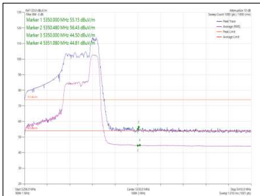
Figure 1050 - 802.11ax HE40 CDD, Cores 0-1, 52-44- 5310 MHz Band Edge Frequency 5350 MHz
