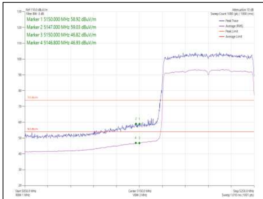
Figure 1062 - 802.11ax HE80, Core 1, SU - 5210 MHz Band Edge Frequency 5150 MHz
