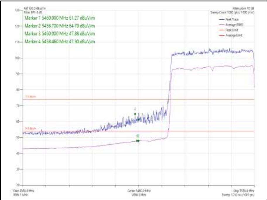
Figure 1066 - 802.11ax HE80, Core 0, SU - 5530 MHz Band Edge Frequency 5460 MHz
