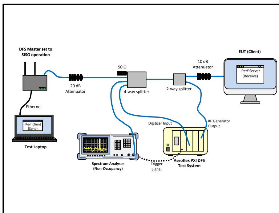
Figure 1143 - Test Equipment Setup Diagram for Client without Radar Detection with Injection at the Master – Master-to-Client Mode
