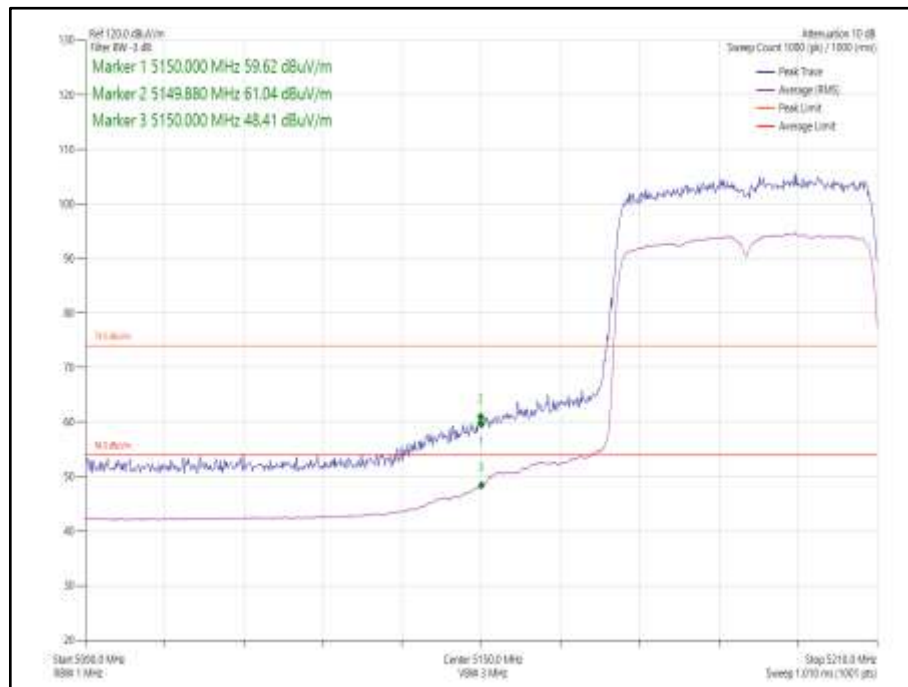
Figure 1045 802.11ax HE40 SDM, Cores 0-1, SU - 5190 MHz Band Edge Frequency 5150 MHz
