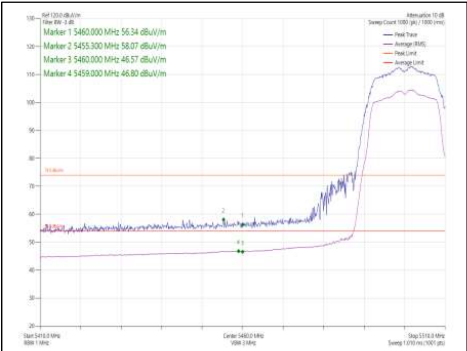
Figure 1010 - 802.11a, Core 0 - 5500 MHz, Band Edge Frequency 5460 MHz
