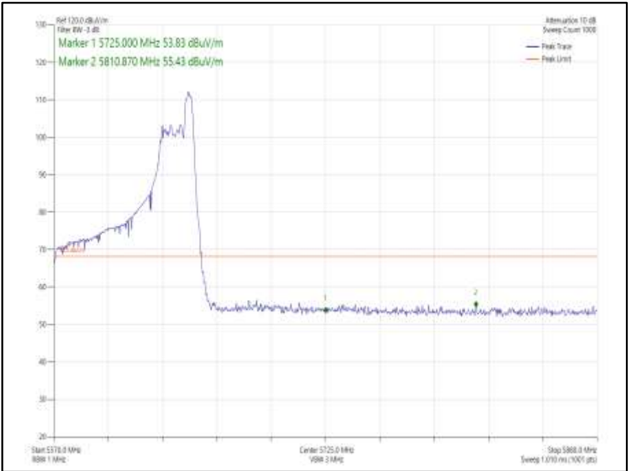
Figure 987 - 802.11ax HE80 CDD, Cores 0-1, 52-52- 5610 MHz Band Edge Frequency 5725 MHz
