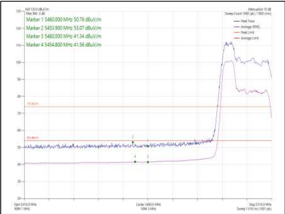
Figure 1029 - 802.11ax HE20 CDD, Cores 0-1, 52-37 - 5500 MHz Band Edge Frequency 5460 MHz
