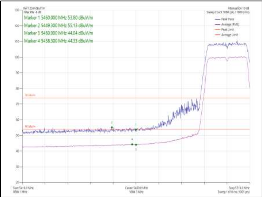
Figure 1026 - 802.11n HT20 CDD, Cores 0-1 - 5500 MHz Band Edge Frequency 5460 MHz
