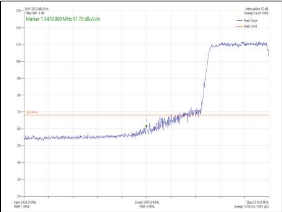
Figure 910 - 802.11ax HE20 SDM, Cores 0-1 SU - 5500 MHz Band Edge Frequency 5470 MHz
