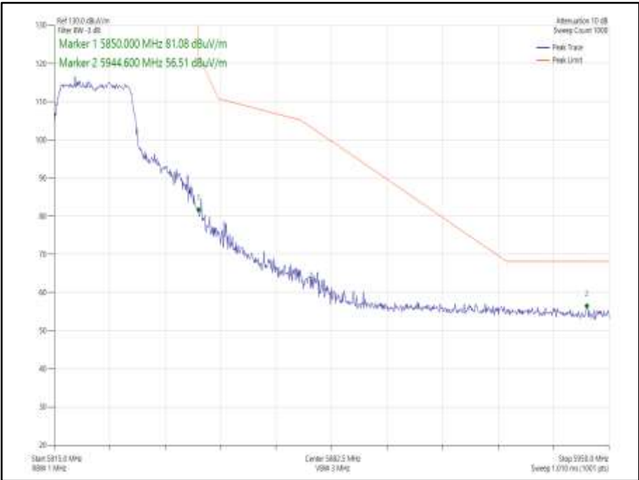
Figure 925 - 802.11n HT20 SDM, Cores 0-1 - 5825 MHz Band Edge Frequency 5850 MHz
