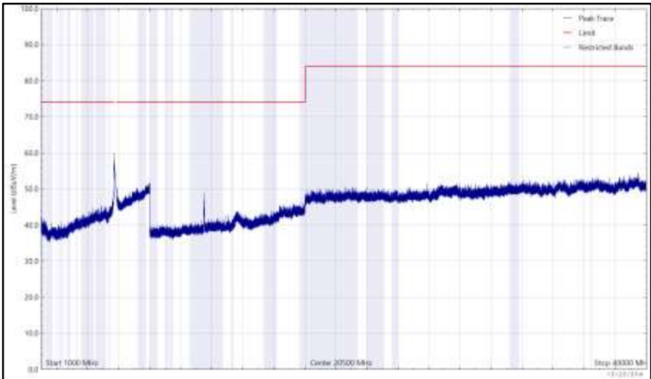
Figure 1107 - U-NII-3 - 5745 MHz (CH149), HT20, CDD, Core 0 + Core 1, 1 GHz to 40 GHz, Vertical (Peak)
