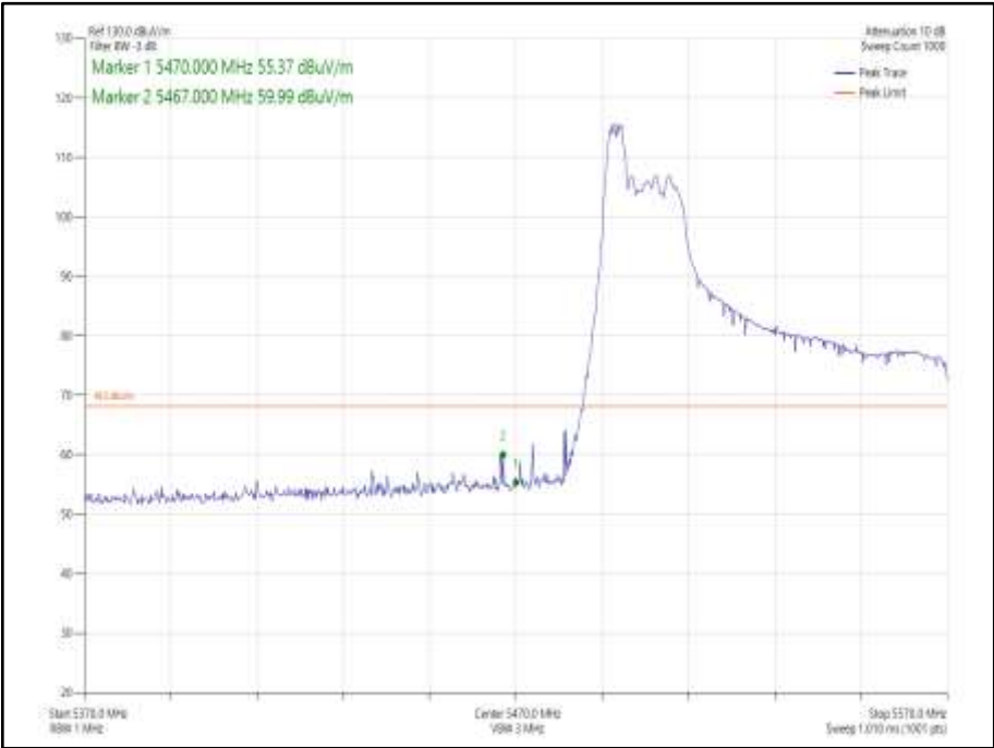
Figure 971 - 802.11ax HE80 Core 0 26-0- 5530 MHz Band Edge Frequency 5470 MHz
