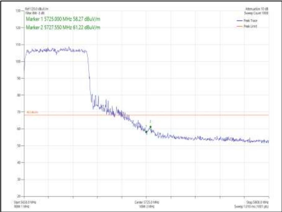
Figure 950 - 802.11ax HE40 CDD, Cores 0-1, SU - 5670 MHz Band Edge Frequency 5725 MHz
