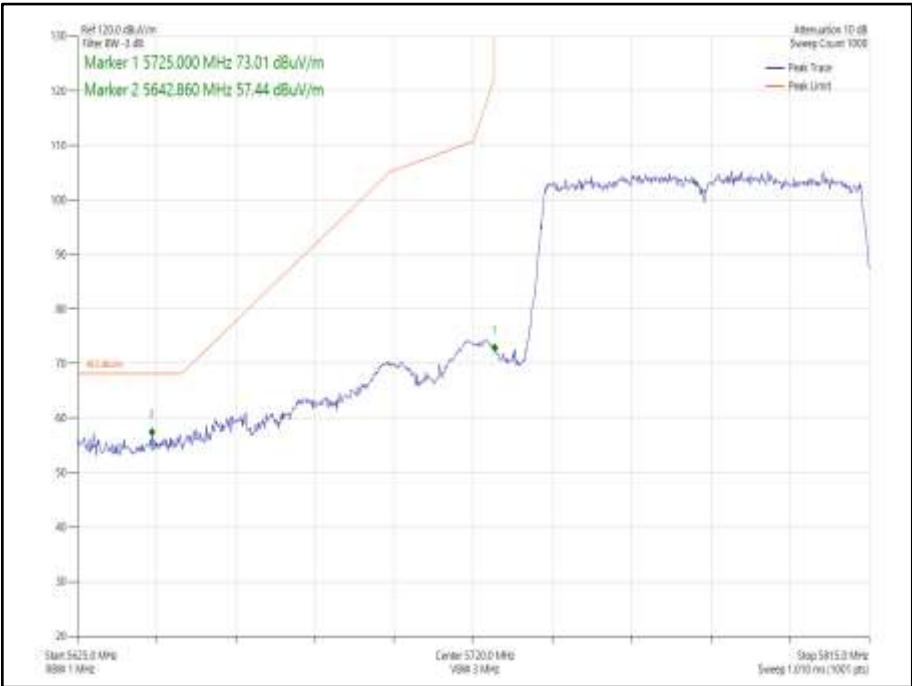
Figure 991 - 802.11ac VHT80 SDM, Cores 0-1 - 5775 MHz Band Edge Frequency 5725 MHz
