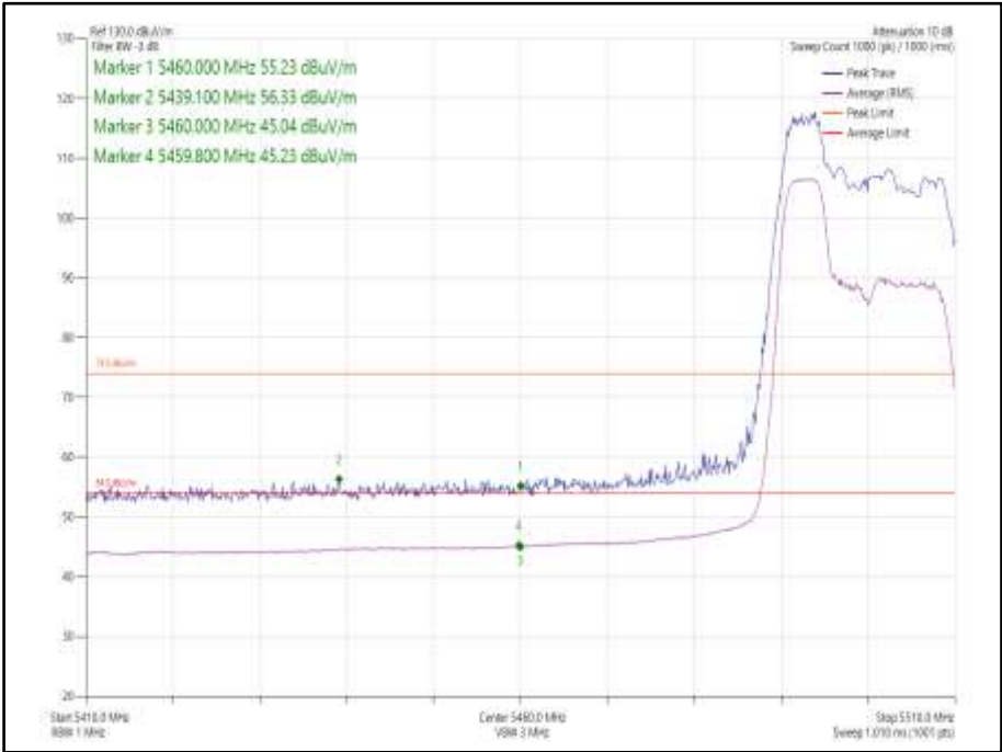
Figure 1013 - 802.11ax HE20, Core 0, 52-37 - 5500 MHz, Band Edge Frequency 5460 MHz
