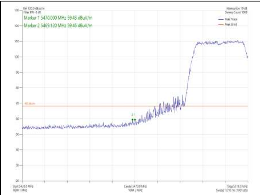
Figure 907 - 802.11n HT20 SDM, Cores 0-1 - 5500 MHz Band Edge Frequency 5470 MHz
