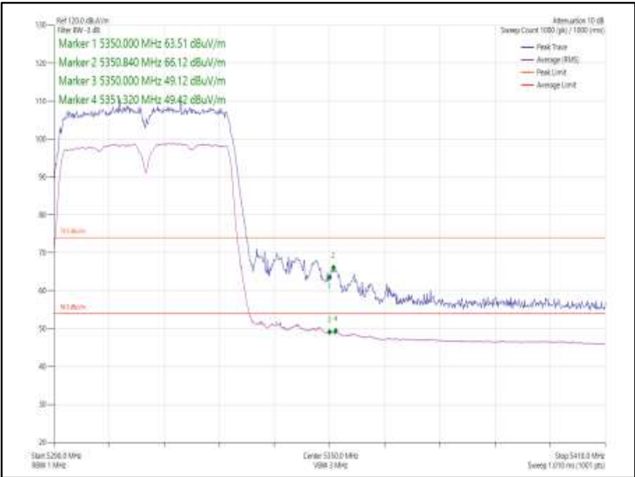
Figure 1048 - 802.11n HT40 SDM, Cores 0-1 - 5310 MHz Band Edge Frequency 5350 MHz
