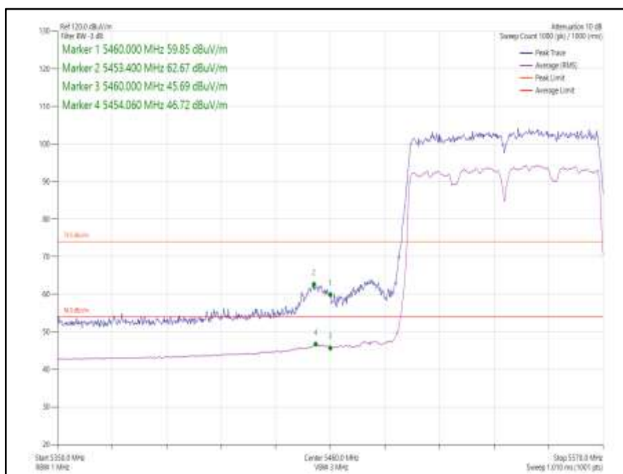
Figure 1081 - 802.11ac VHT80 SDM, Cores 0-1- 5530 MHz Band Edge Frequency 5460 MHz
