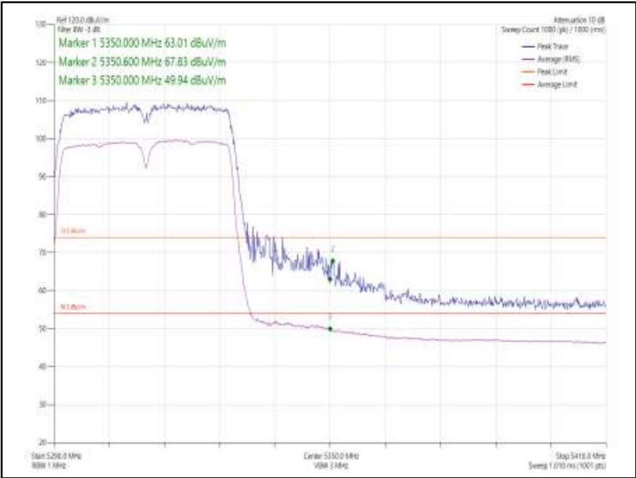
Figure 1035 - 802.11n HT40, Core 0 - 5310 MHz Band Edge Frequency 5350 MHz
