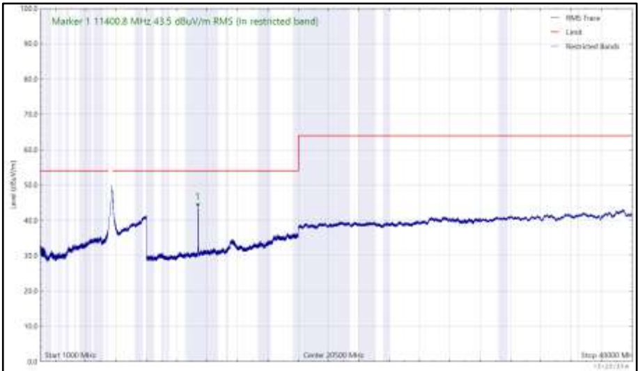
Figure 1104 - U-NII-2C - 5700 MHz (CH140), HT20, CDD, Core 0 + Core 1, 1 GHz to 40 GHz, Vertical (RMS)
