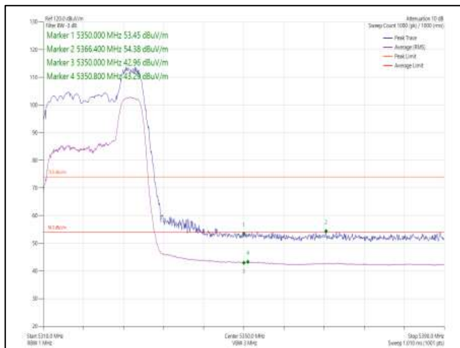
Figure 1023 - 802.11ax HE20 CDD, Cores 0-1, 52-40 - 5320 MHz Band Edge Frequency 5350 MHz
