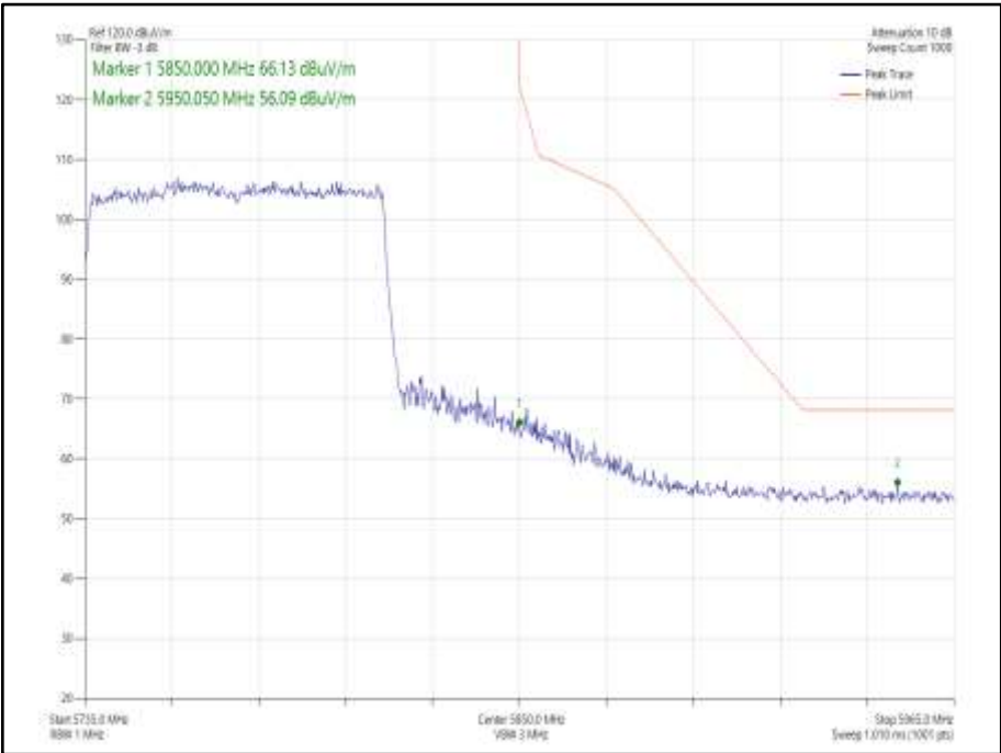
Figure 976 - 802.11ax HE80 Core 0 SU - 5775 MHz Band Edge Frequency 5850 MHz
