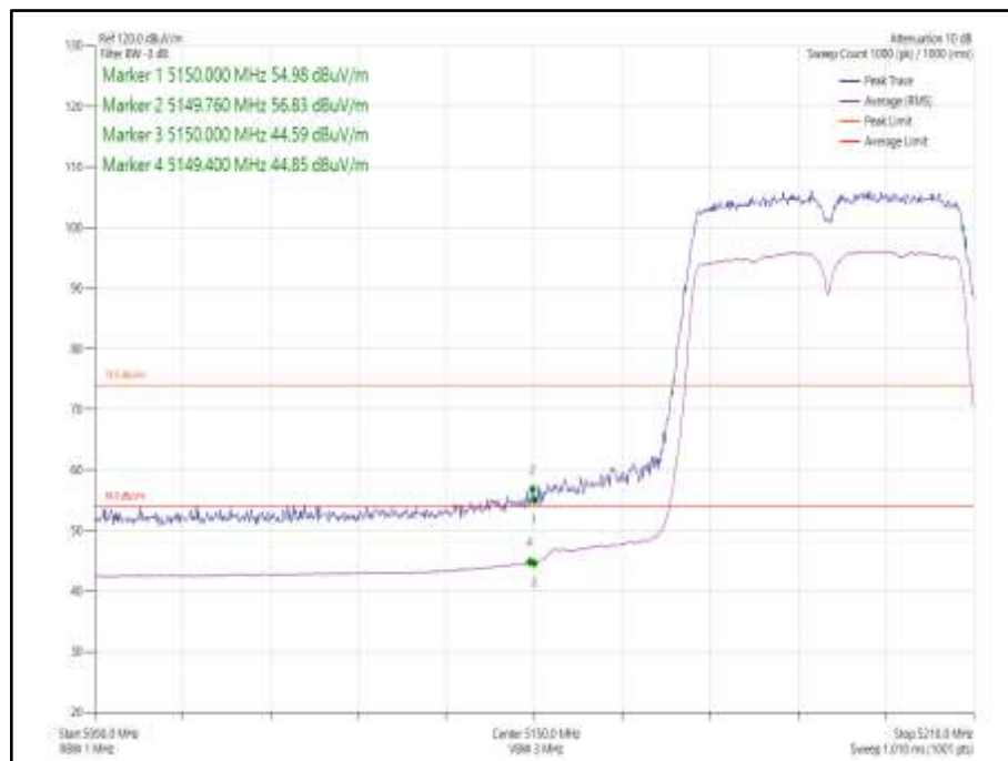
Figure 1032 - 802.11n HT40, Core 1 - 5190 MHz Band Edge Frequency 5150 MHz
