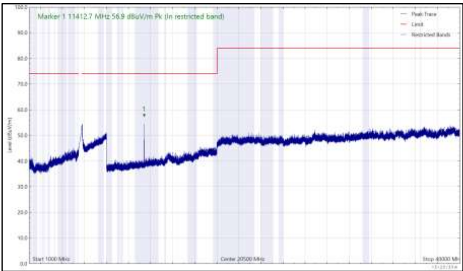
Figure 1129 - 5700 MHz (CH140), HE20, RU52-40, Core 0 + Core 1, 1 GHz to 40 GHz, Horizontal (Peak)
