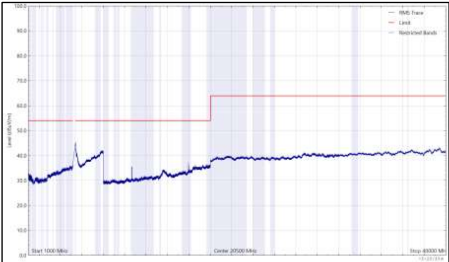
Figure 1096 - U-NII-2A - 5320 MHz (CH64), HT20, CDD, Core 0 + Core 1, 1 GHz to 40 GHz, Vertical (RMS)
