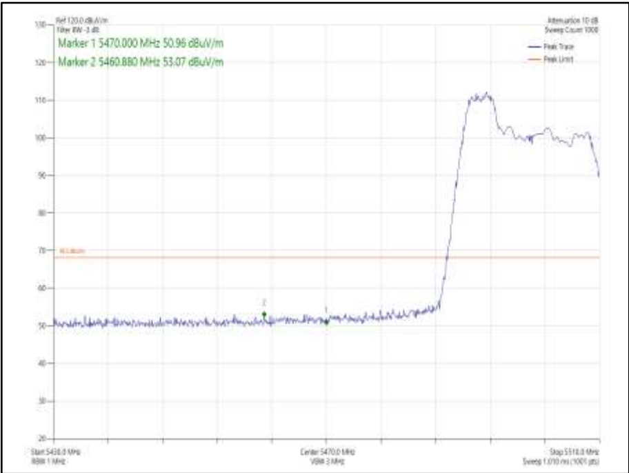
Figure 909 - 802.11ax HE20 CDD, Cores 0-1 52-37 - 5500 MHz Band Edge Frequency 5470 MHz
