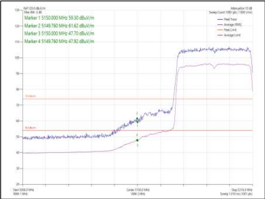
Figure 1043 - 802.11ax HE40 CDD, Cores 0-1, SU - 5190 MHz Band Edge Frequency 5150 MHz
