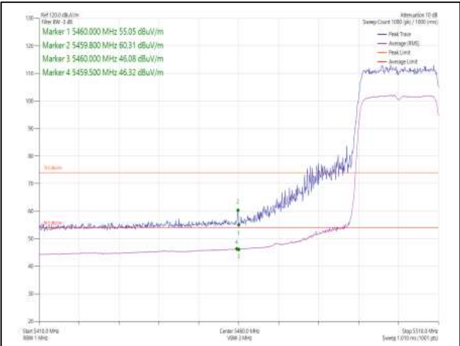
Figure 1012 - 802.11ax HE20, Core 0, SU - 5500 MHz, Band Edge Frequency 5460 MHz
