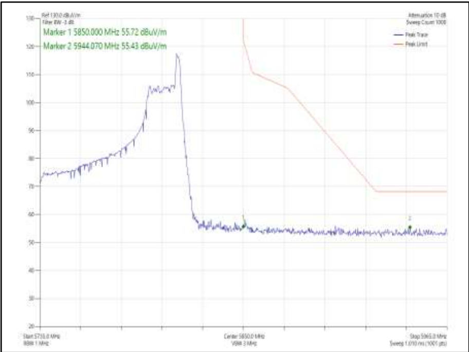
Figure 1001 - 802.11ax HE80 SDM, Cores 0-1, 26-36 - 5775 MHz Band Edge Frequency 5850 MHz
