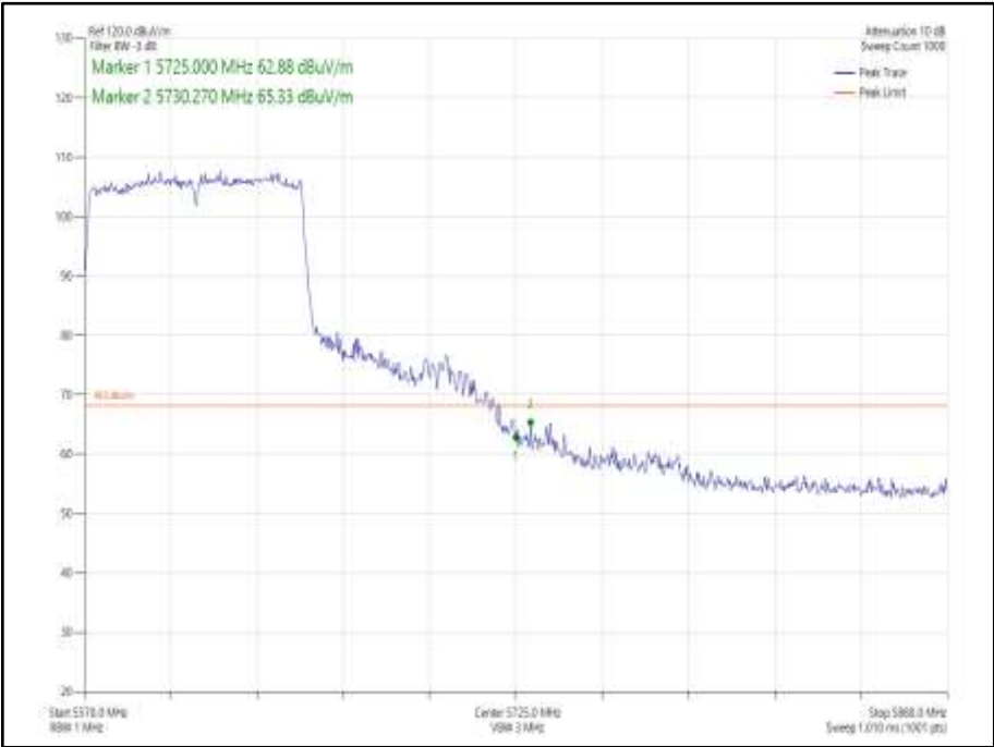
Figure 967 - 802.11ac VHT80 Core 0 - 5610 MHz Band Edge Frequency 5725 MHz
