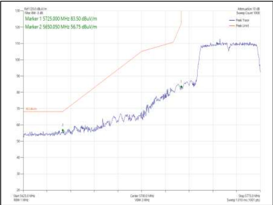
Figure 955 - 802.11n HT40 SDM, Cores 0-1 - 5755 MHz Band Edge Frequency 5725 MHz
