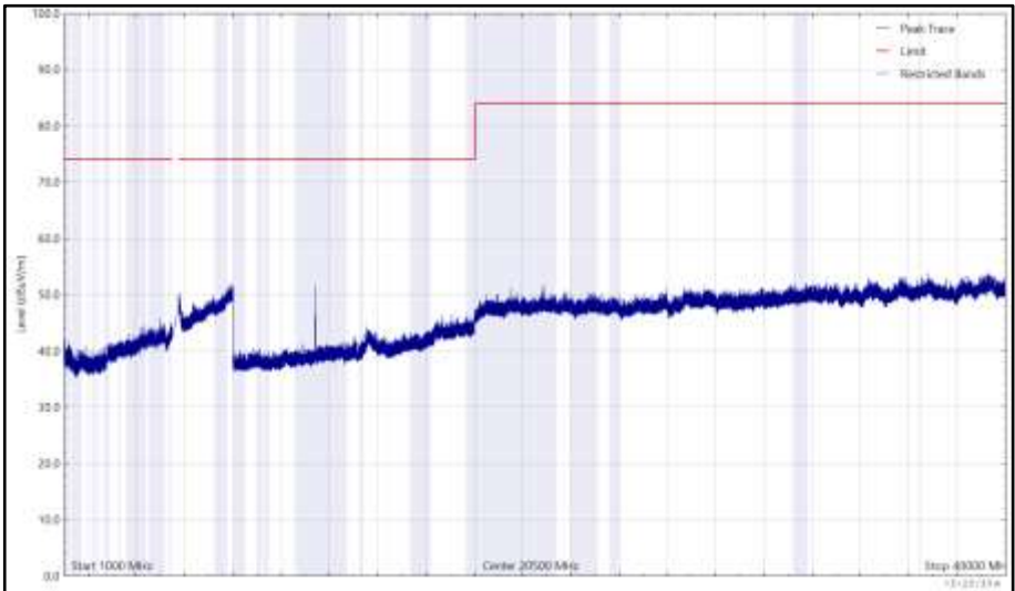
Figure 1131 - 5700 MHz (CH140), HE20, RU52-40, Core 0 + Core 1, 1 GHz to 40 GHz, Vertical (Peak)
