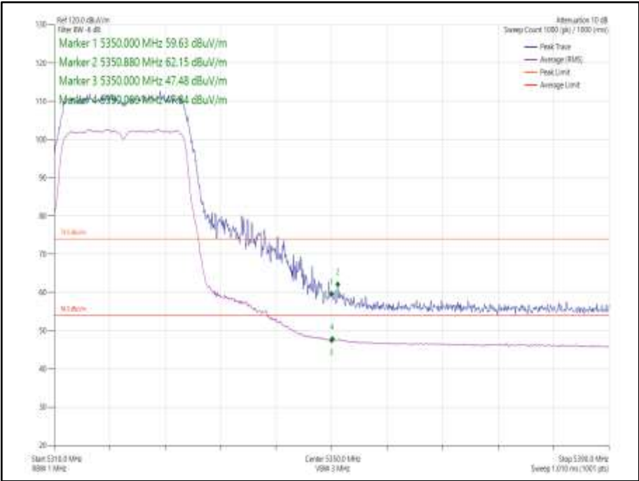
Figure 1020 - 802.11n HT20 CDD, Cores 0-1 - 5320 MHz Band Edge Frequency 5350 MHz
