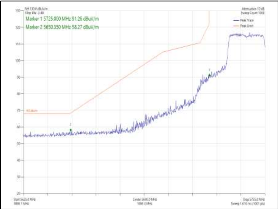
Figure 922 - 802.11ax HE20 SDM, Cores 0-1, SU - 5745 MHz Band Edge Frequency 5725 MHz
