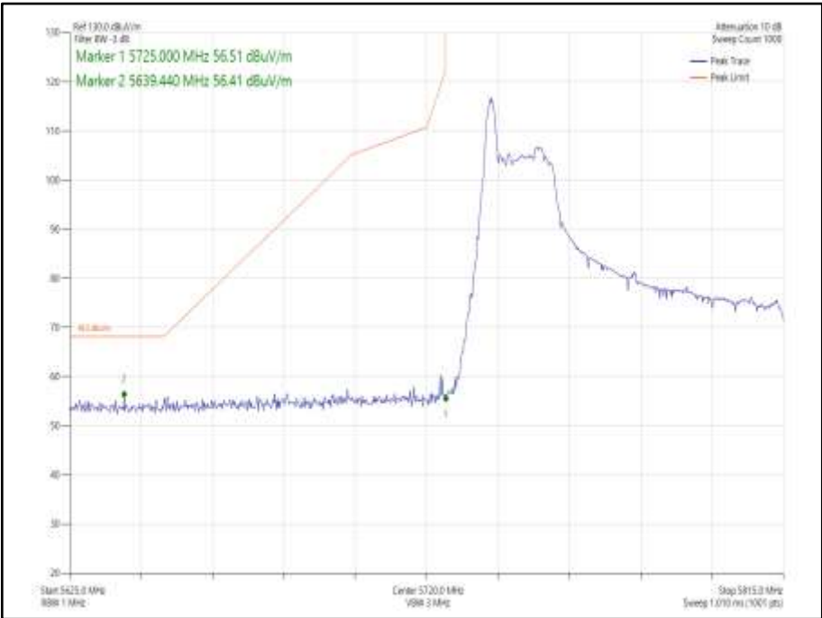
Figure 993 - 802.11ax HE80 CDD, Cores 0-1, 26-0 - 5775 MHz Band Edge Frequency 5725 MHz
