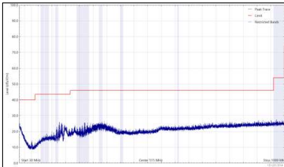
Figure 1137 - 5825 MHz (CH165), HE20, RU26-8, Core 0 + Core 1, 30 MHz to 1 GHz, Horizontal (Peak)
