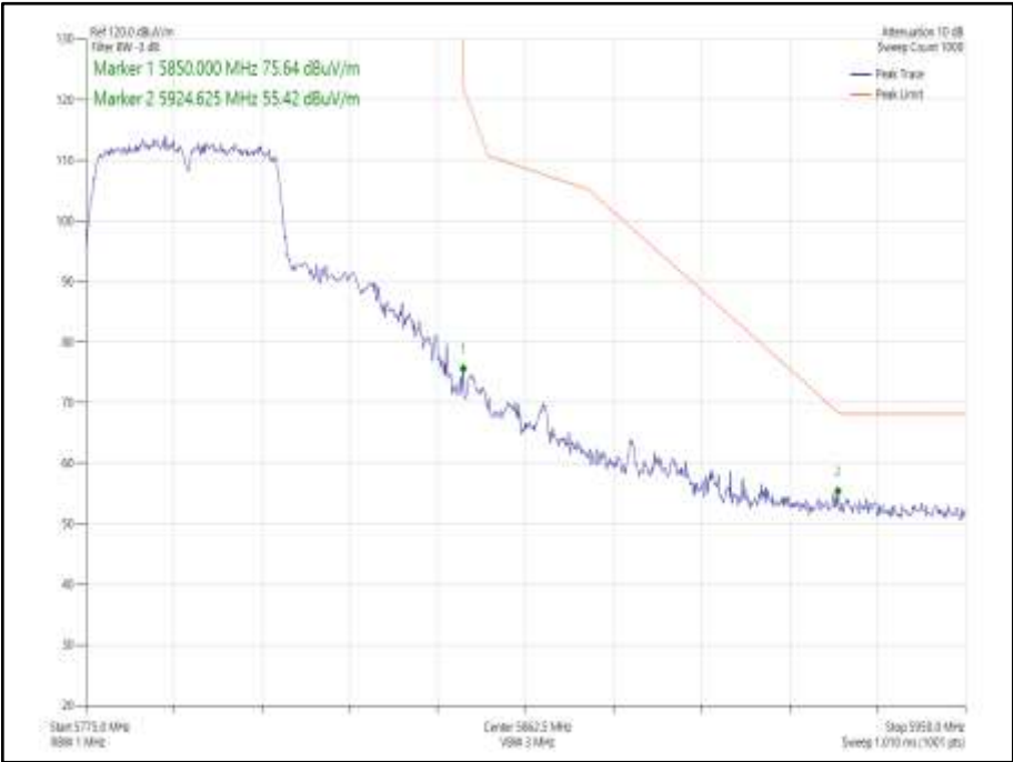
Figure 960 - 802.11n HT40 CDD, Cores 0-1 - 5795 MHz Band Edge Frequency 5850 MHz
