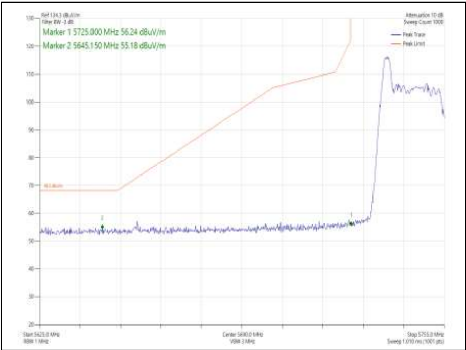
Figure 923 - 802.11ax HE20 SDM, Cores 0-1, 26-0 - 5745 MHz Band Edge Frequency 5725 MHz
