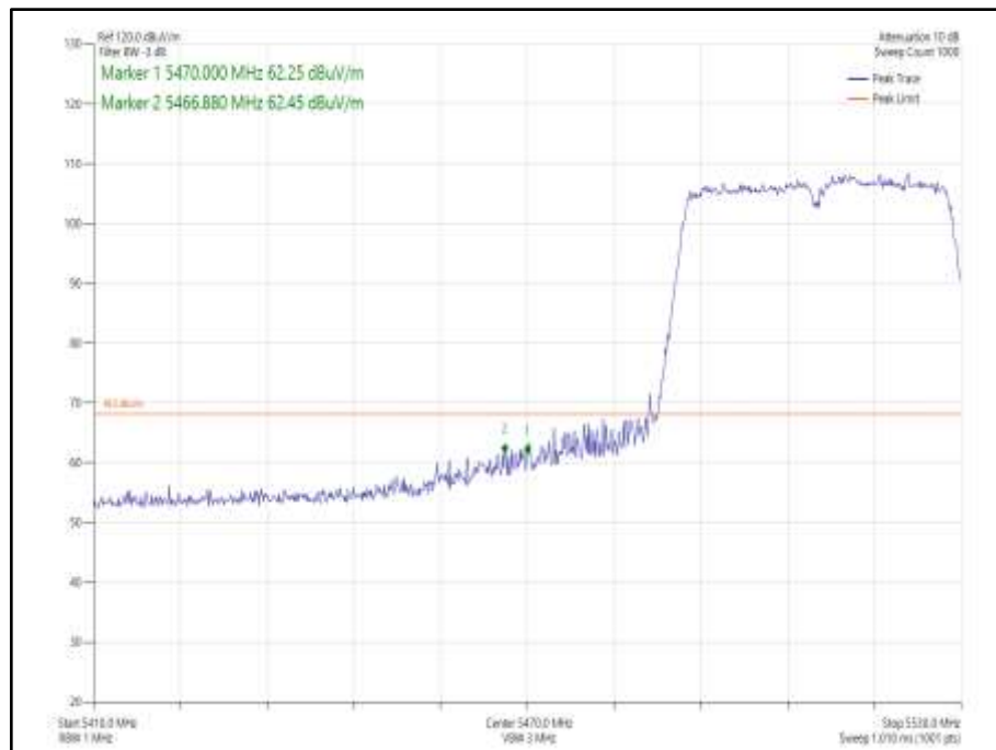
Figure 930 - 802.11n HT40, Core 0 - 5510 MHz Band Edge Frequency 5470 MHz
