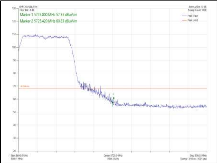
Figure 912 - 802.11n HT20 CDD, Cores 0-1 - 5700 MHz Band Edge Frequency 5725 MHz
