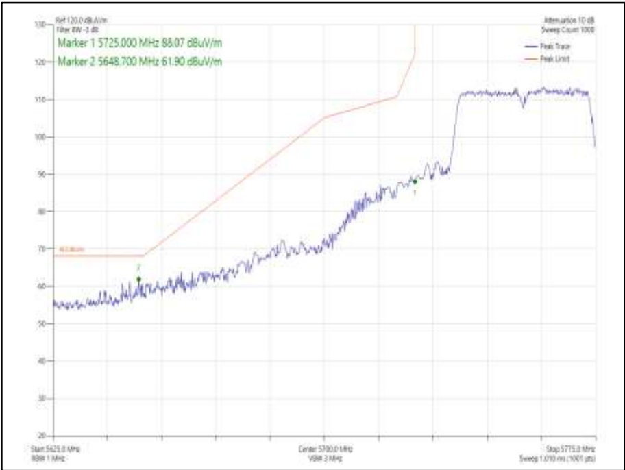
Figure 932 - 802.11n HT40, Core 0 - 5755 MHz Band Edge Frequency 5725 MHz
