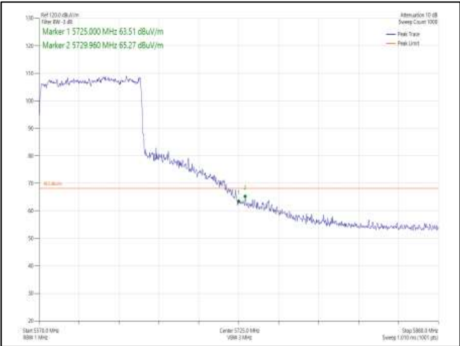
Figure 972 - 802.11ax HE80 Core 0 SU - 5610 MHz Band Edge Frequency 5725 MHz
