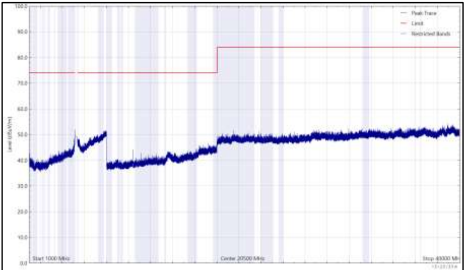
Figure 1091 - U-NII-1 - 5180 MHz (CH36), HT20, CDD, Core 0 + Core 1, 1 GHz to 40 GHz, Vertical (Peak)
