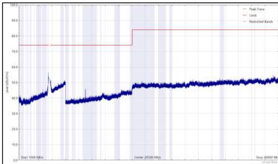
Figure 1097 - U-NII-2C - 5500 MHz (CH100), HT20, CDD, Core 0 + Core 1, 1 GHz to 40 GHz, Horizontal (Peak)
