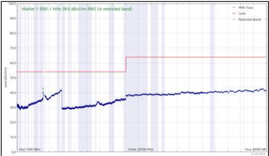
Figure 1120 - 5180 MHz (CH36), HE20, RU26-0, Core 0 + Core 1, 1 GHz to 40 GHz, Vertical (RMS)
