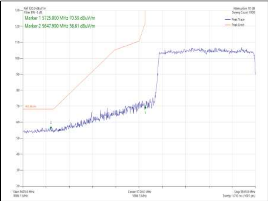
Figure 994 - 802.11ax HE80 SDM, Cores 0-1, SU - 5775 MHz Band Edge Frequency 5725 MHz
