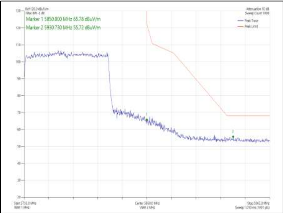
Figure 998 - 802.11ax HE80 CDD, Cores 0-1, SU - 5775 MHz Band Edge Frequency 5850 MHz
