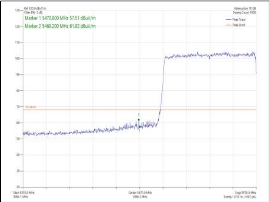
Figure 982 - 802.11ax HE80 SDM, Cores 0-1, SU - 5530 MHz Band Edge Frequency 5470 MHz
