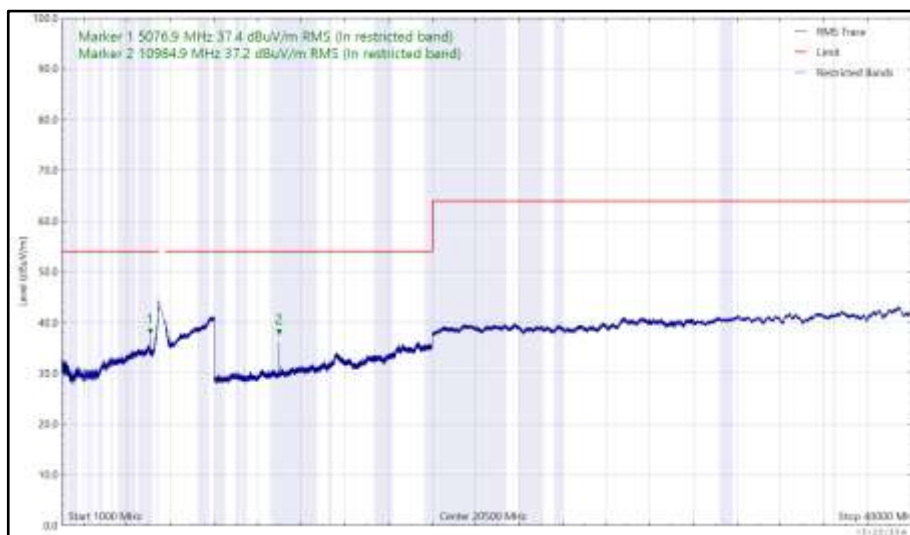
Figure 1126 - 5500 MHz (CH100), HE20, RU52-37, Core 0 + Core 1, 1 GHz to 40 GHz, Horizontal (RMS)
