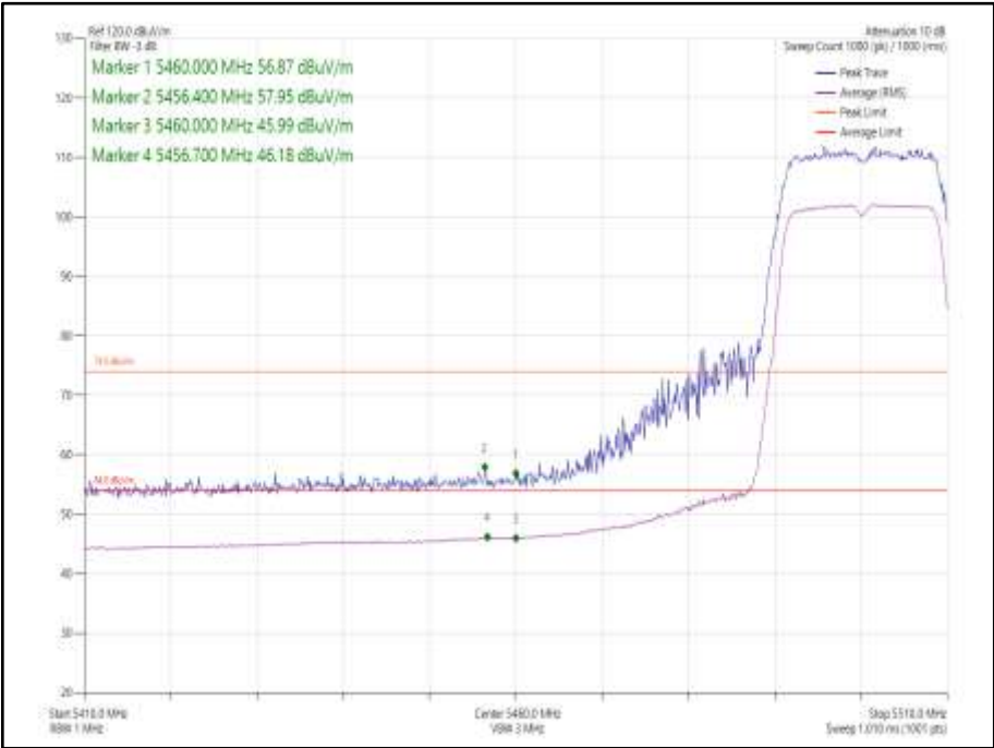
Figure 1011 - 802.11n HT20, Core 0 - 5500 MHz, Band Edge Frequency 5460 MHz
