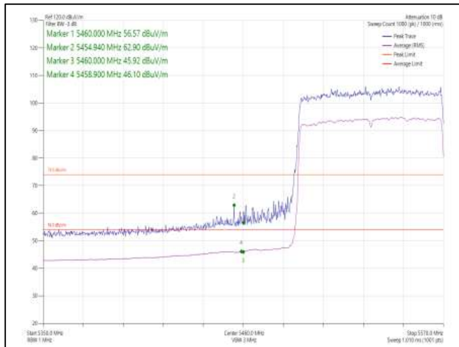
Figure 1082 - 802.11ax HE80 CDD, Cores 0-1, SU - 5530 MHz Band Edge Frequency 5460 MHz
