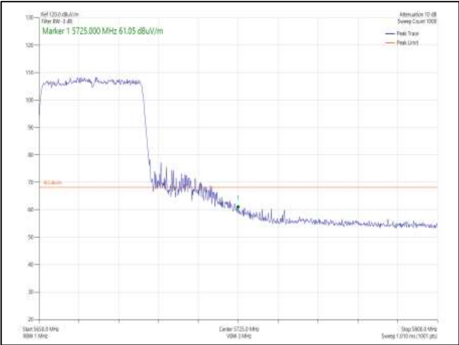
Figure 952 - 802.11ax HE40 SDM, Cores 0-1, SU - 5670 MHz Band Edge Frequency 5725 MHz
