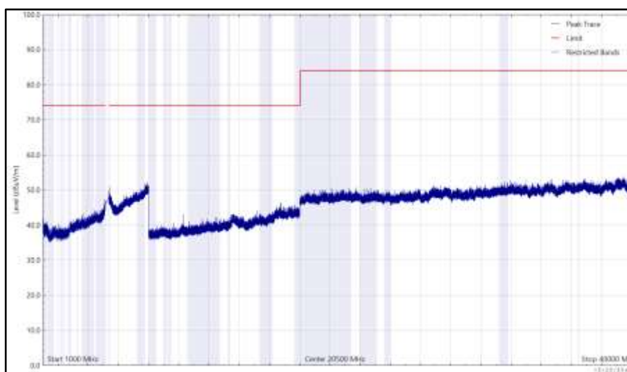
Figure 1116 - 5180 MHz (CH36), HE20, RU26-0, Core 0 + Core 1, 1 GHz to 40 GHz, Horizontal (Peak)
