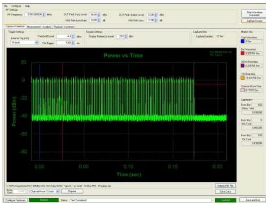
Figure 1146 - First 200 ms of Channel Shutdown Period
