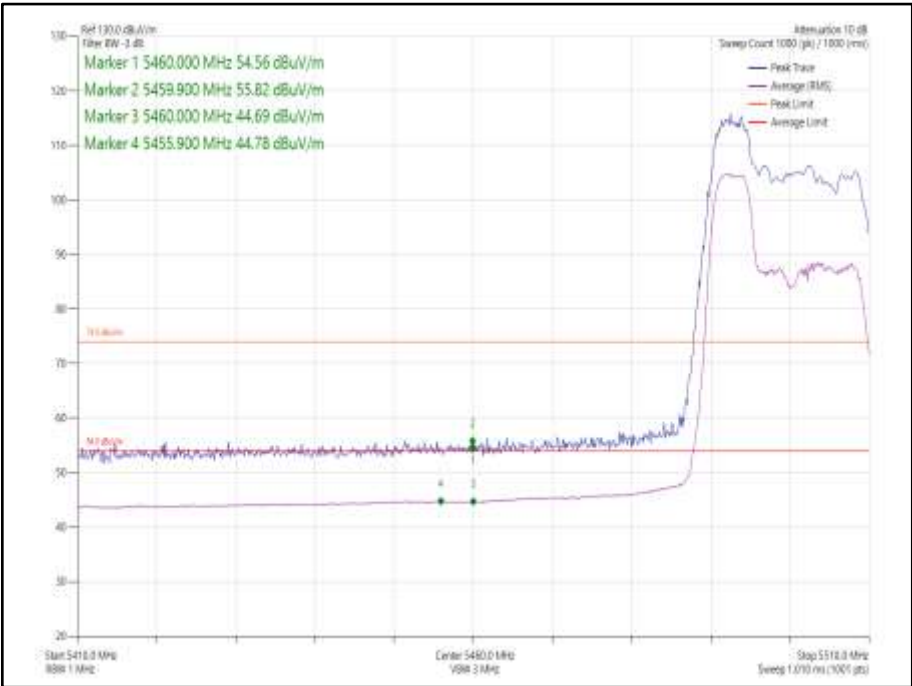
Figure 1031 - 802.11ax HE20 SDM, Cores 0-1, 52-37 - 5500 MHz Band Edge Frequency 5460 MHz
