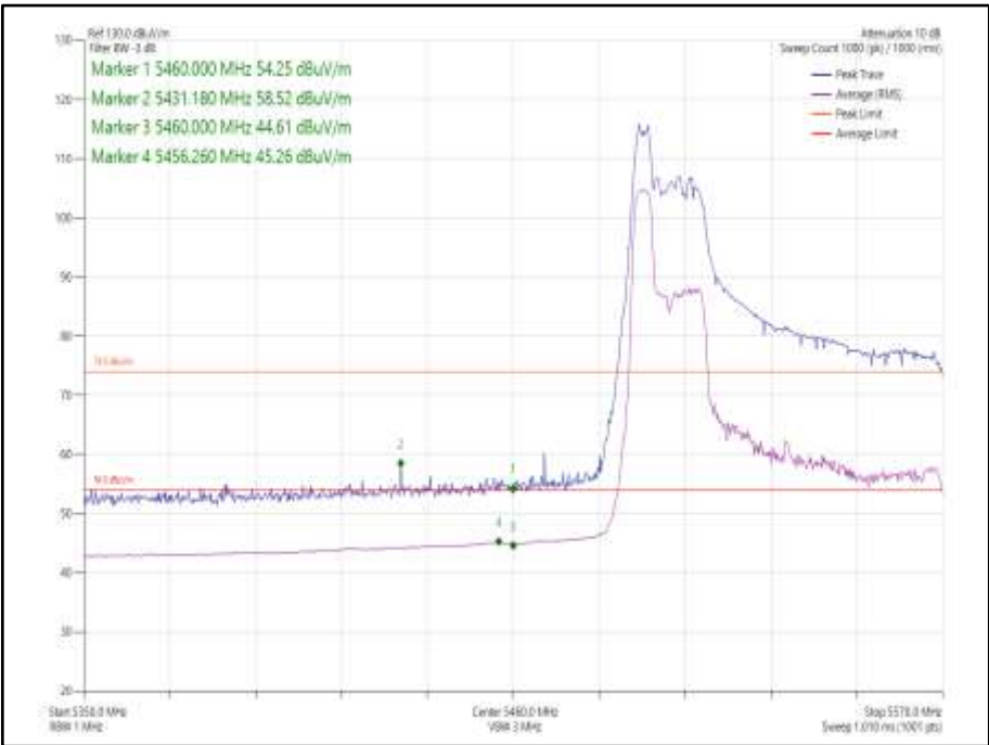
Figure 1067 - 802.11ax HE80, Core 0, 52-37 - 5530 MHz Band Edge Frequency 5460 MHz
