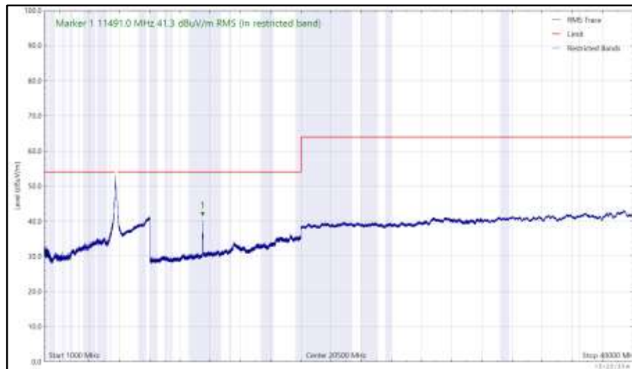
Figure 1106 - U-NII-3 - 5745 MHz (CH149), HT20, CDD, Core 0 + Core 1, 1 GHz to 40 GHz, Horizontal (RMS)
