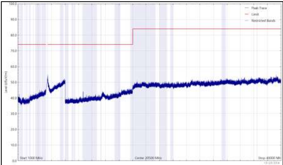
Figure 1095 - U-NII-2A - 5320 MHz (CH64), HT20, CDD, Core 0 + Core 1, 1 GHz to 40 GHz, Vertical (Peak)
