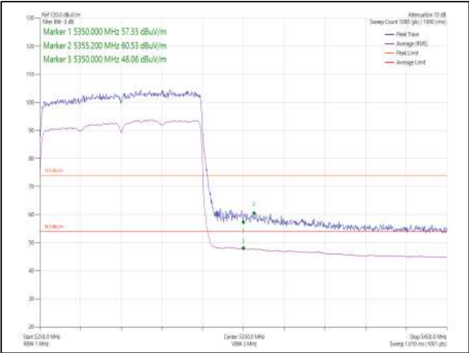
Figure 1078 - 802.11ax HE80 SDM, Cores 0-1, SU - 5290 MHz Band Edge Frequency 5350 MHz
