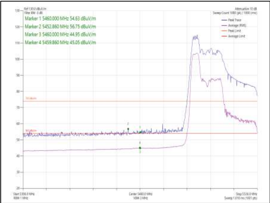
Figure 1058 - 802.11ax HE40 SDM, Cores 0-1, 26-0 - 5510 MHz Band Edge Frequency 5460 MHz
