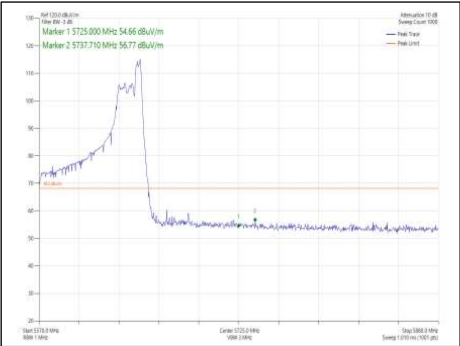
Figure 989 - 802.11ax HE80 SDM, Cores 0-1, 52-52 - 5610 MHz Band Edge Frequency 5725 MHz
