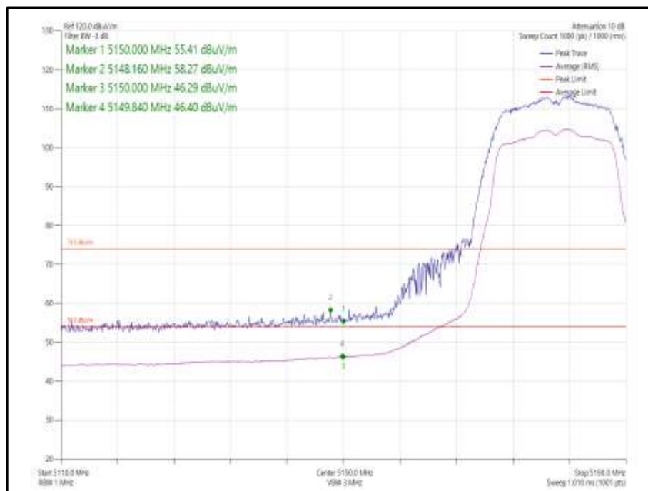
Figure 1002 - 802.11a, Core 1 - 5180 MHz, Band Edge Frequency 5150 MHz
