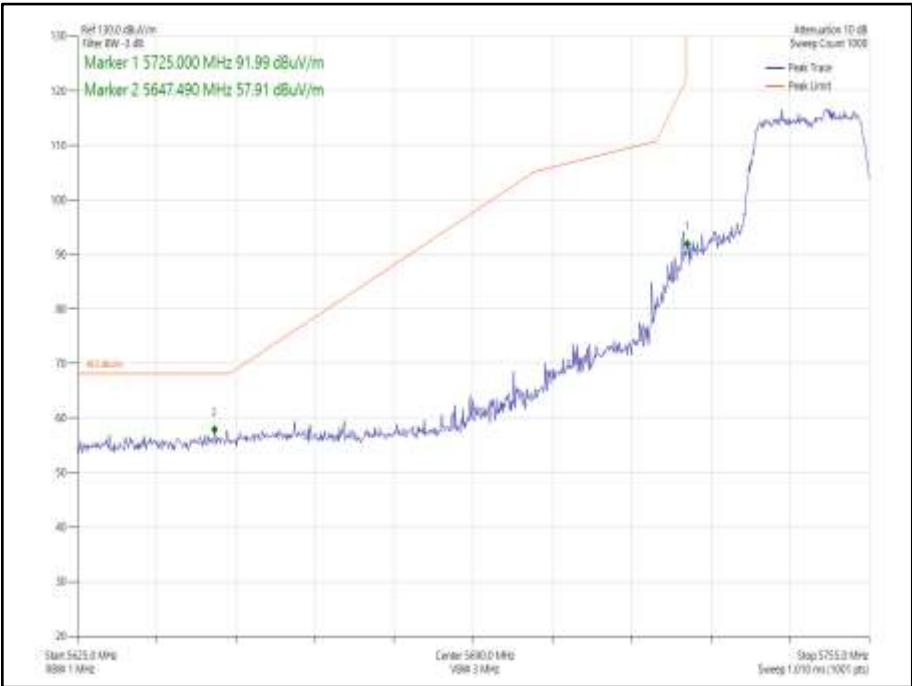
Figure 919 - 802.11n HT20 SDM, Cores 0-1 - 5745 MHz Band Edge Frequency 5725 MHz
