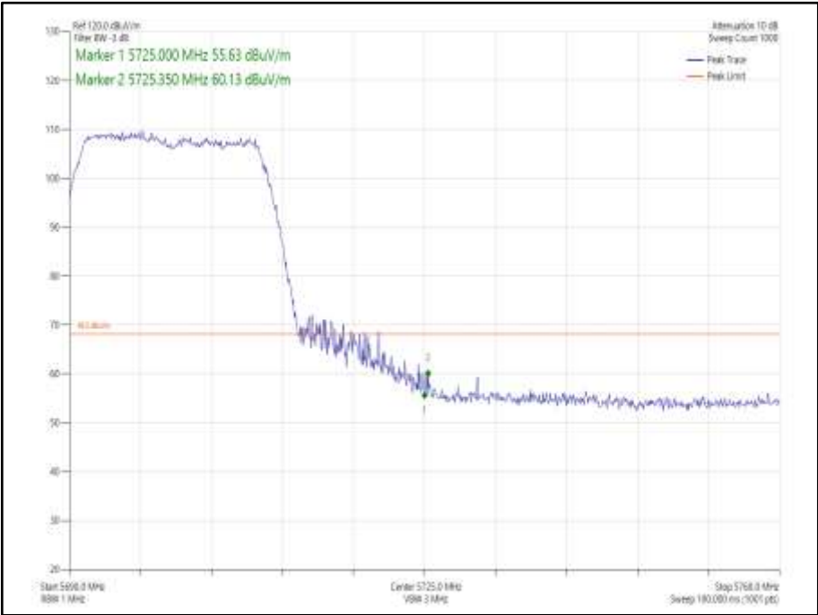
Figure 914 - 802.11ax HE20 CDD, Cores 0-1, SU - 5700 MHz Band Edge Frequency 5725 MHz
