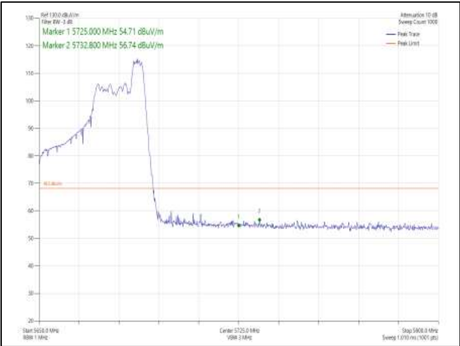
Figure 953 - 802.11ax HE40 SDM, Cores 0-1, 52-44 - 5670 MHz Band Edge Frequency 5725 MHz
