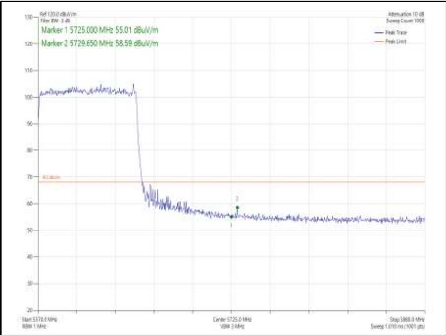
Figure 988 - 802.11ax HE80 SDM, Cores 0-1, SU - 5610 MHz Band Edge Frequency 5725 MHz
