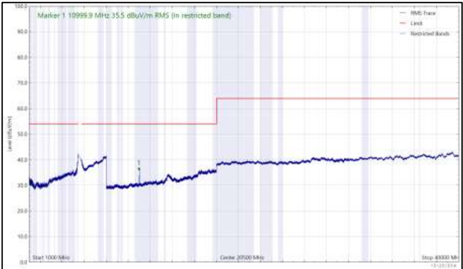
Figure 1100 - U-NII-2C - 5500 MHz (CH100), HT20, CDD, Core 0 + Core 1, 1 GHz to 40 GHz, Vertical (RMS)
