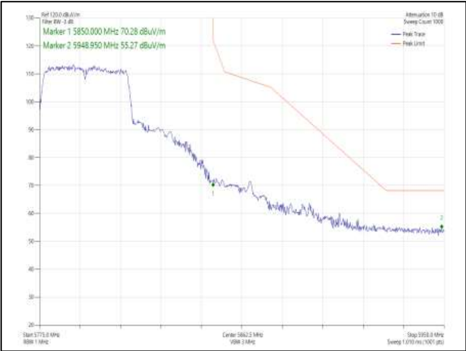
Figure 933 - 802.11n HT40, Core 0 - 5795 MHz Band Edge Frequency 5850 MHz
