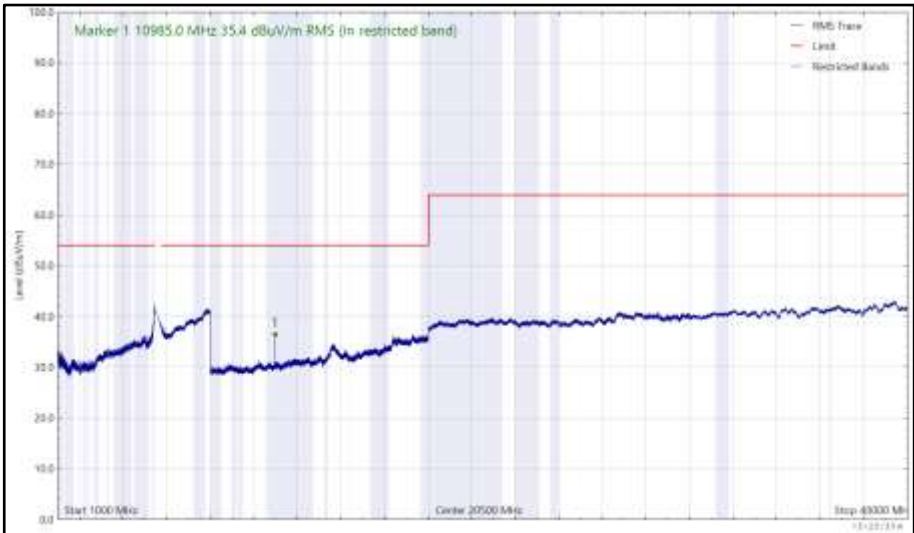
Figure 1128 - 5500 MHz (CH100), HE20, RU52-37, Core 0 + Core 1, 1 GHz to 40 GHz, Vertical (RMS)
