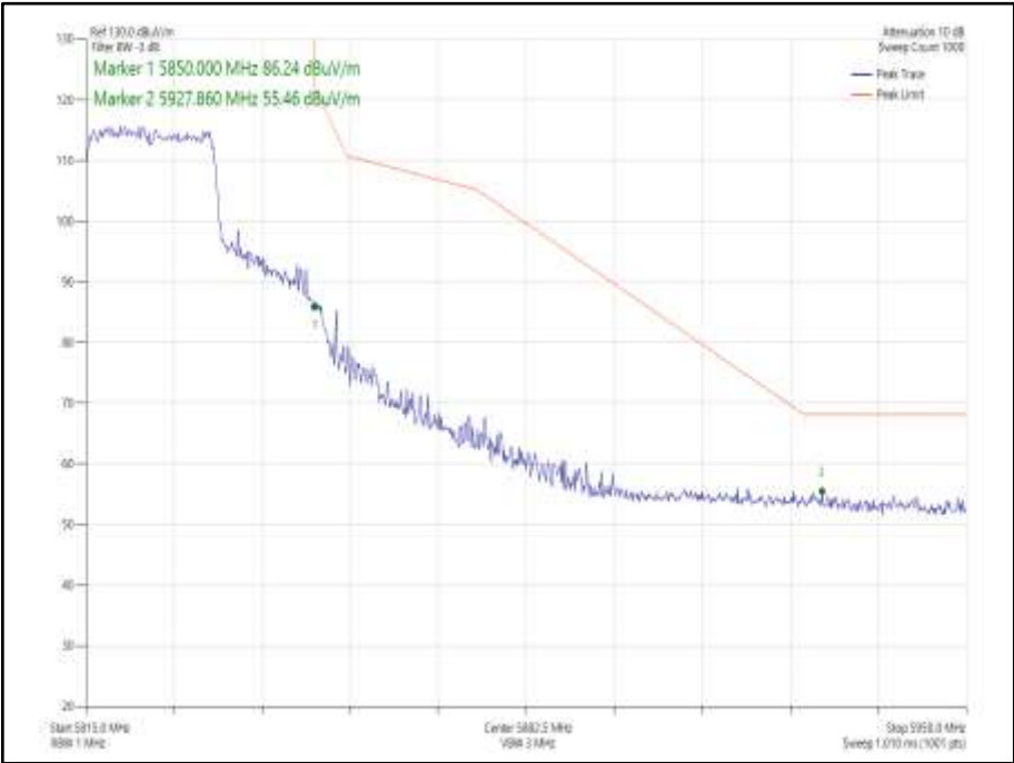
Figure 926 - 802.11ax HE20 CDD, Cores 0-1, SU - 5825 MHz Band Edge Frequency 5850 MHz
