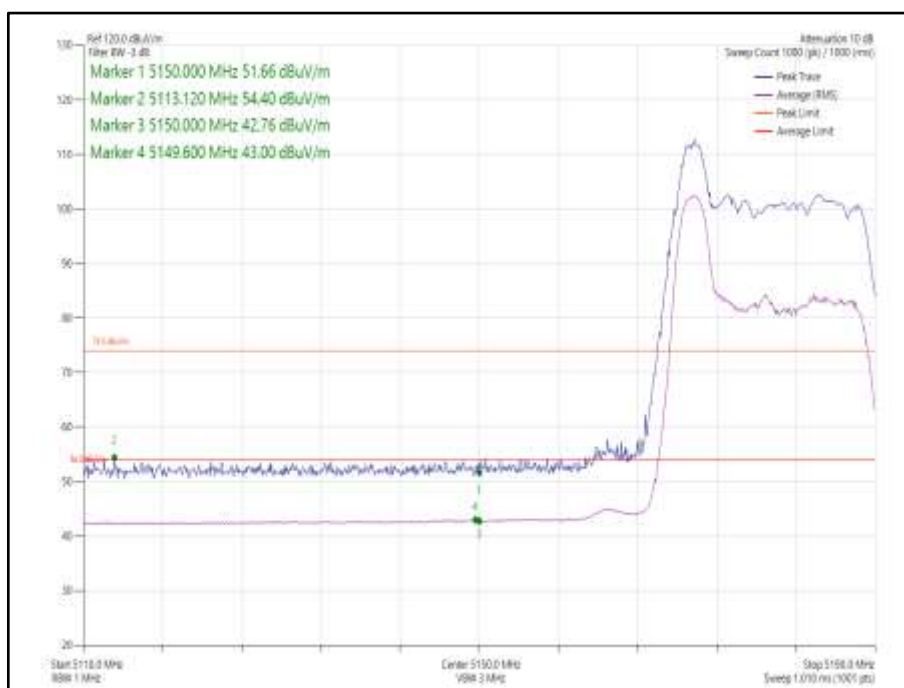
Figure 1019 - 802.11ax HE20 SDM, Cores 0-1, 26-0 - 5180 MHz Band Edge Frequency 5150 MHz
