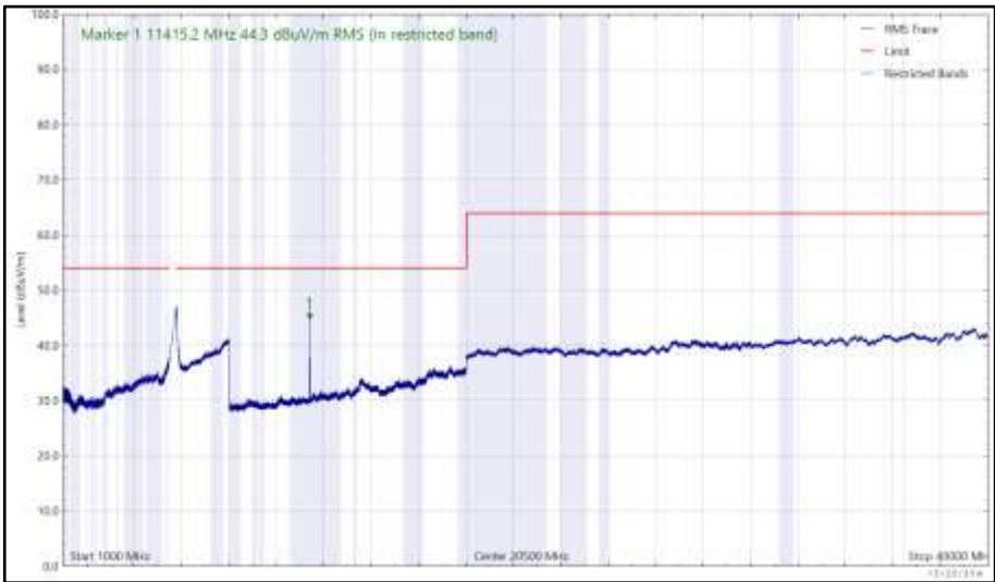
Figure 1130 - 5700 MHz (CH140), HE20, RU52-40, Core 0 + Core 1, 1 GHz to 40 GHz, Horizontal (RMS)
