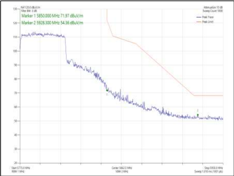
Figure 962 - 802.11ax HE40 CDD, Cores 0-1, SU - 5795 MHz Band Edge Frequency 5850 MHz
