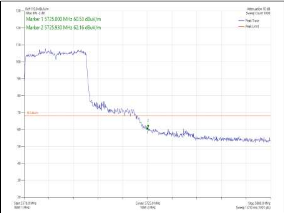
Figure 984 - 802.11ac VHT80 CDD, Cores 0-1 - 5610 MHz Band Edge Frequency 5725 MHz
