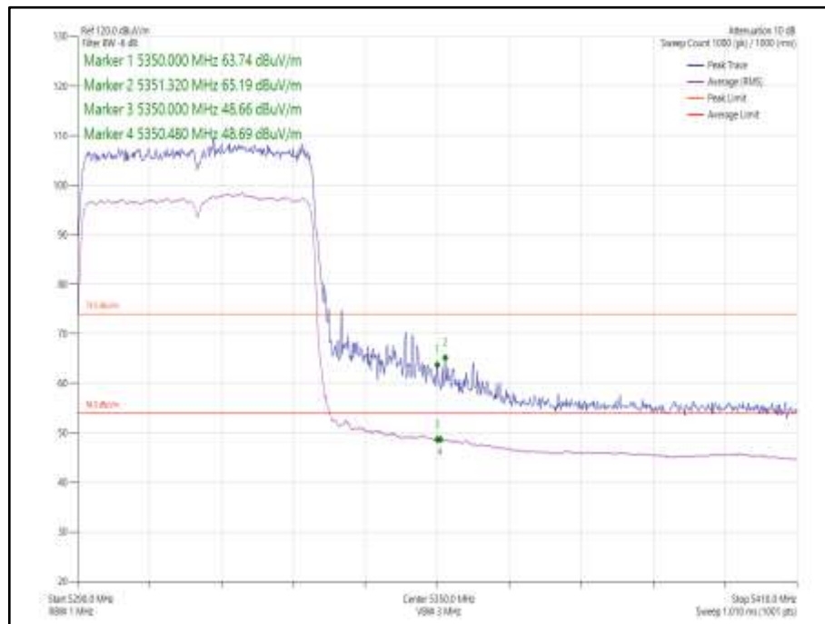
Figure 1049 - 802.11ax HE40 CDD, Cores 0-1, SU - 5310 MHz Band Edge Frequency 5350 MHz
