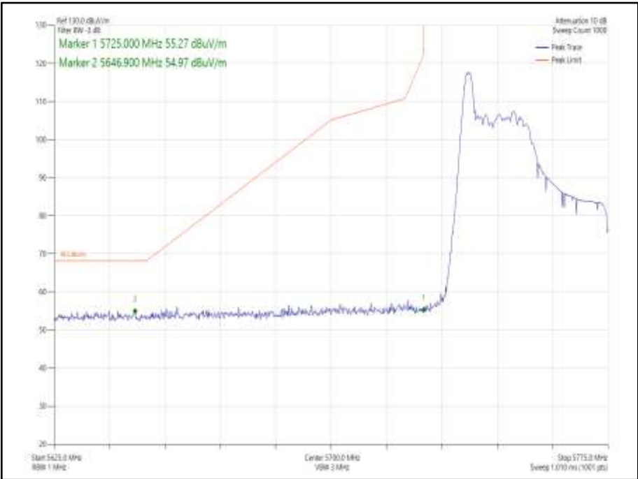
Figure 959 - 802.11ax HE40 SDM, Cores 0-1, 26-0 - 5755 MHz Band Edge Frequency 5725 MHz
