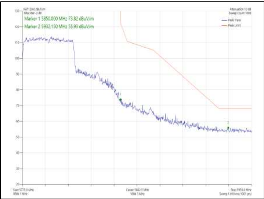
Figure 964 - 802.11ax HE40 SDM, Cores 0-1, SU - 5795 MHz Band Edge Frequency 5850 MHz
