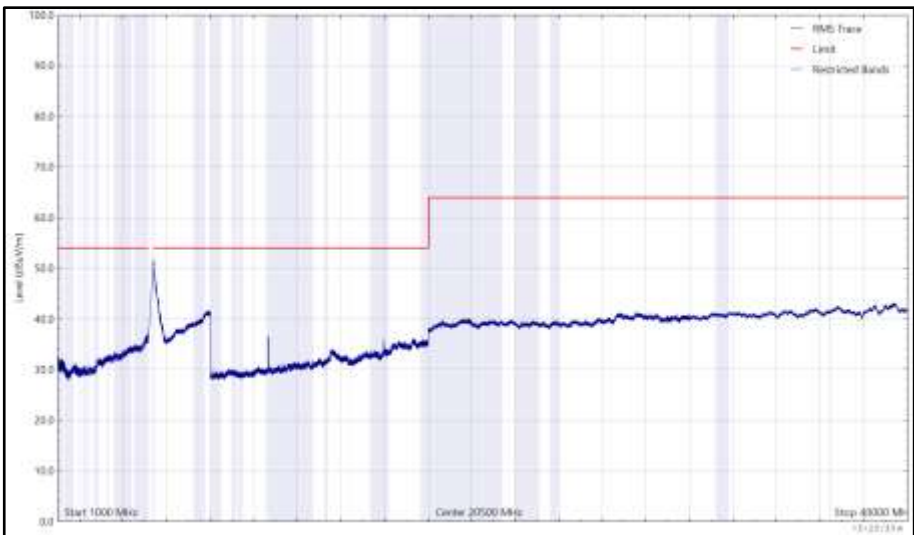
Figure 1094 - U-NII-2A - 5320 MHz (CH64), HT20, CDD, Core 0 + Core 1, 1 GHz to 40 GHz, Horizontal (RMS)
