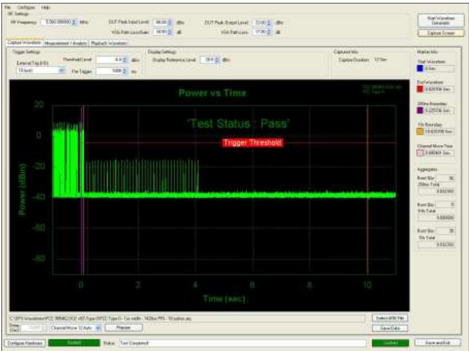
Figure 1153 - First 12 s of Channel Shutdown Period
