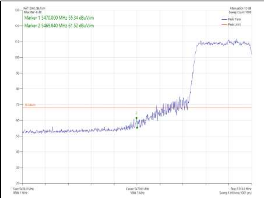
Figure 908 - 802.11ax HE20 CDD, Cores 0-1, SU - 5500 MHz Band Edge Frequency 5470 MHz
