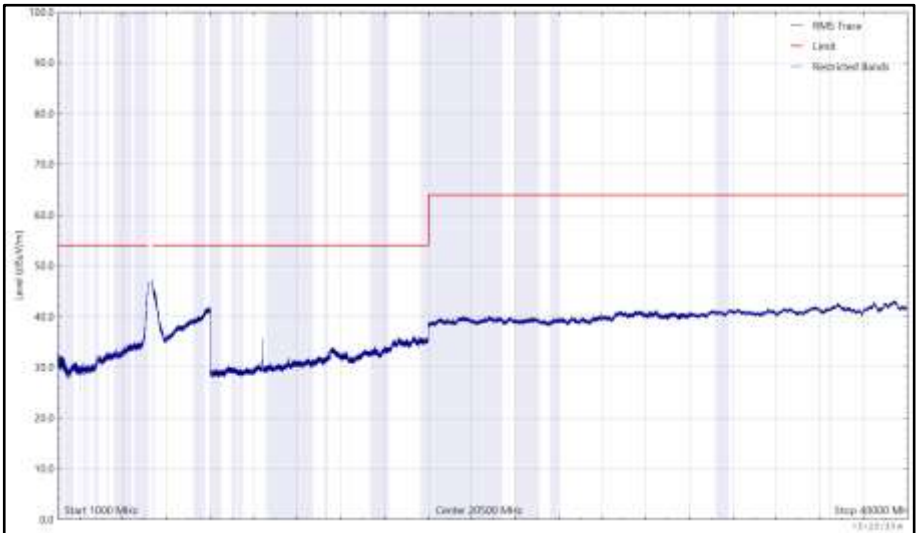
Figure 1089 - U-NII-1 - 5180 MHz (CH36), HT20, CDD, Core 0 + Core 1, 1 GHz to 40 GHz, Horizontal (RMS)
