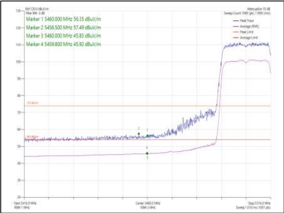
Figure 1030 - 802.11ax HE20 SDM, Cores 0-1, SU- 5500 MHz Band Edge Frequency 5460 MHz
