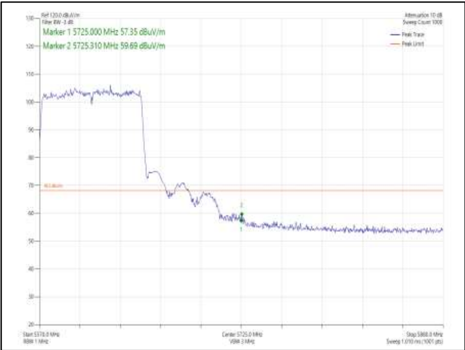
Figure 985 - 802.11ac VHT80 SDM, Cores 0-1 - 5610 MHz Band Edge Frequency 5725 MHz
