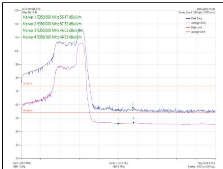
Figure 1052 - 802.11ax HE40 SDM, Cores 0-1, 52-44 - 5310 MHz Band Edge Frequency 5350 MHz
