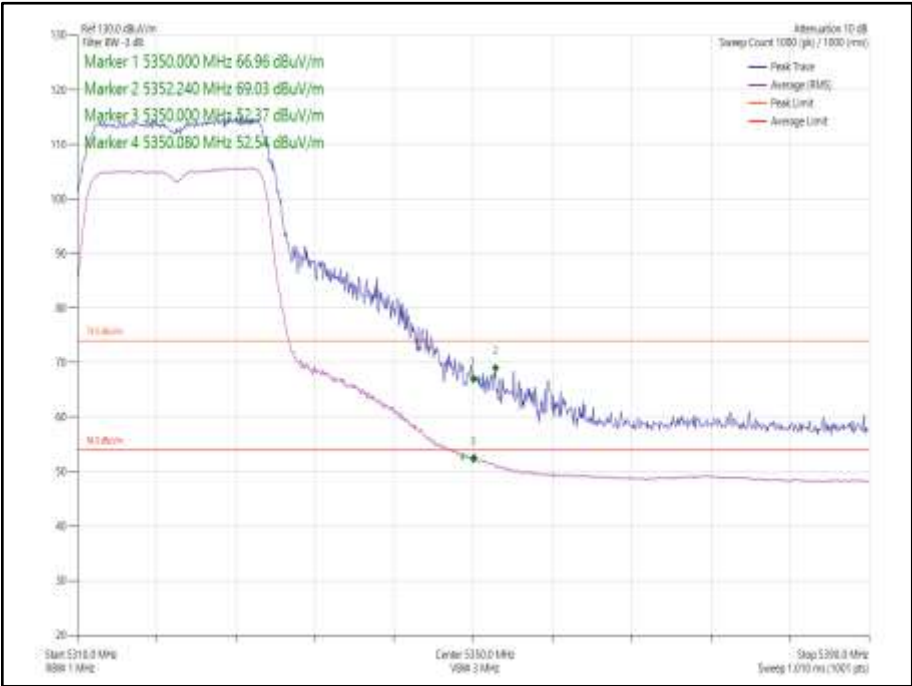
Figure 1007 - 802.11n HT20, Core 0 - 5320 MHz, Band Edge Frequency 5350 MHz
