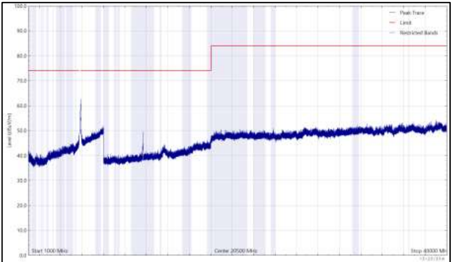
Figure 1113 - U-NII-3 - 5825 MHz (CH165), HT20, CDD, Core 0 + Core 1, 1 GHz to 40 GHz, Vertical (Peak)
