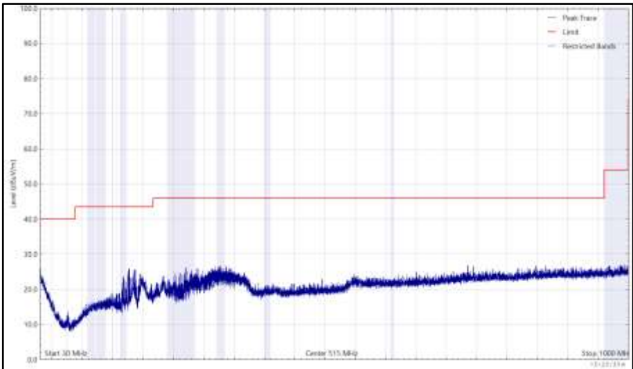
Figure 1087 - U-NII-1 - 5180 MHz (CH36), HT20, CDD, Core 0 + Core 1, 30 MHz to 1 GHz, Horizontal (Peak)
