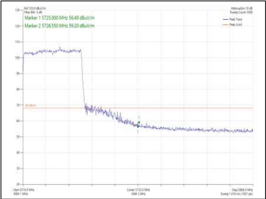
Figure 986 - 802.11ax HE80 CDD, Cores 0-1, SU - 5610 MHz Band Edge Frequency 5725 MHz
