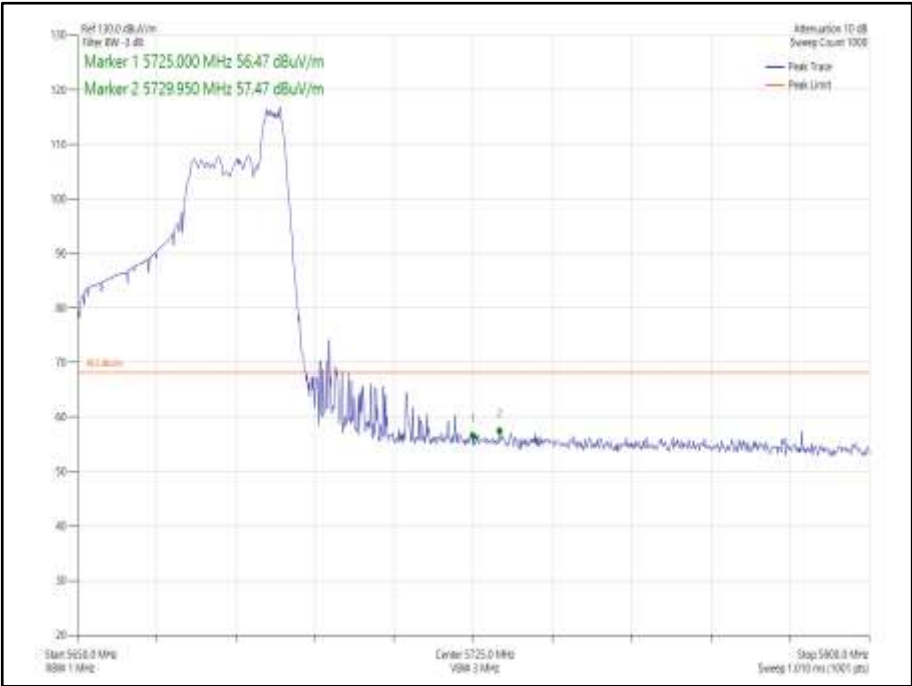
Figure 937 - 802.11ax HE40, Core 0, 52-44 - 5670 MHz Band Edge Frequency 5725 MHz
