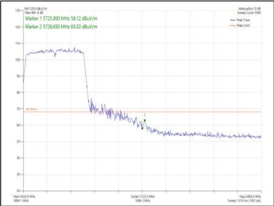
Figure 948 - 802.11n HT40 CDD, Cores 0-1 - 5670 MHz Band Edge Frequency 5725 MHz
