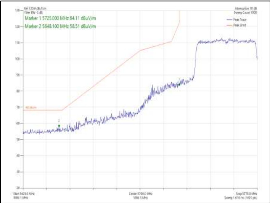
Figure 958 - 802.11ax HE40 SDM, Cores 0-1, SU - 5755 MHz Band Edge Frequency 5725 MHz
