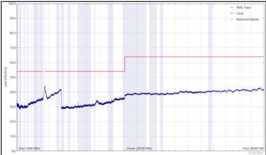
Figure 1124 - 5320 MHz (CH64), HE20, RU52-37, Core 0 + Core 1, 1 GHz to 40 GHz, Vertical (RMS)
