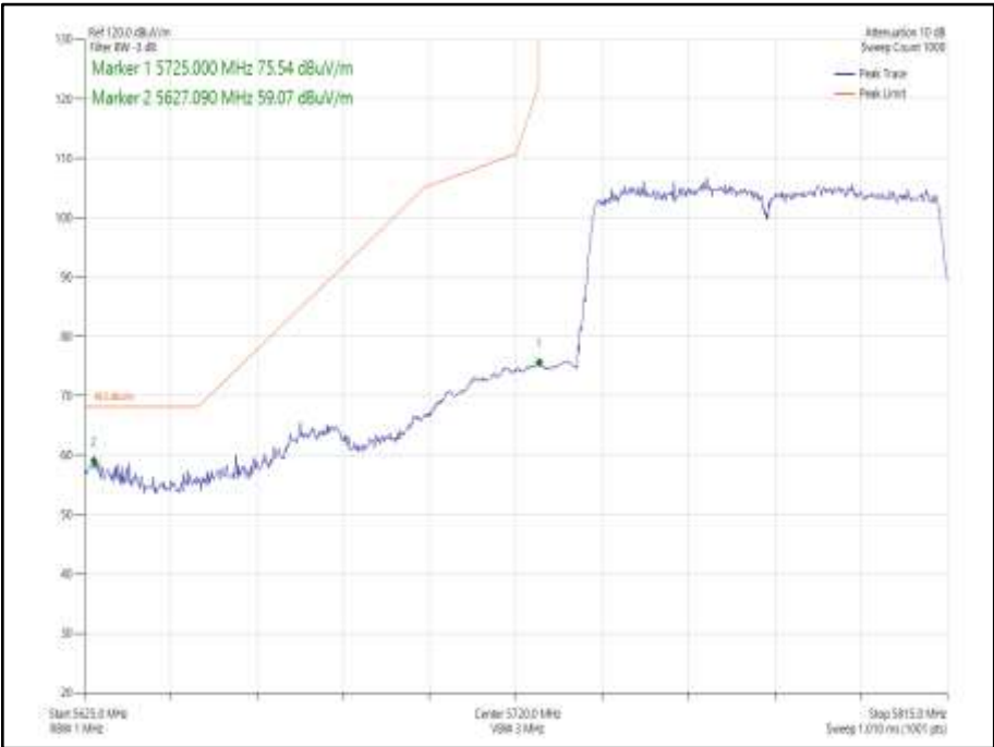
Figure 968 - 802.11ac VHT80 Core 0 - 5775 MHz Band Edge Frequency 5725 MHz
