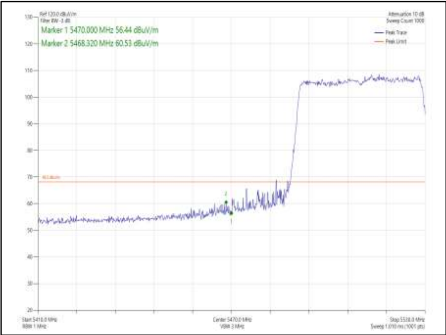
Figure 946 - 802.11ax HE40 SDM, Cores 0-1, SU - 5510 MHz Band Edge Frequency 5470 MHz
