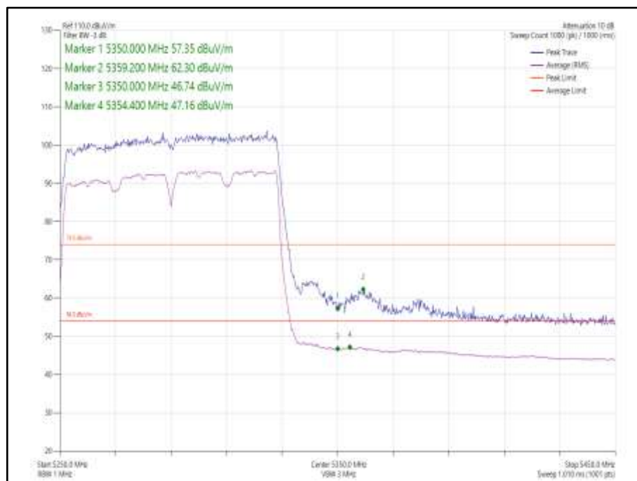
Figure 1075 - 802.11ac VHT80 SDM ,Cores 0-1- 5290 MHz Band Edge Frequency 5350 MHz
