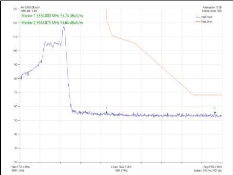
Figure 941 - 802.11ax HE40, Core 0, 26-17 - 5795 MHz Band Edge Frequency 5850 MHz
