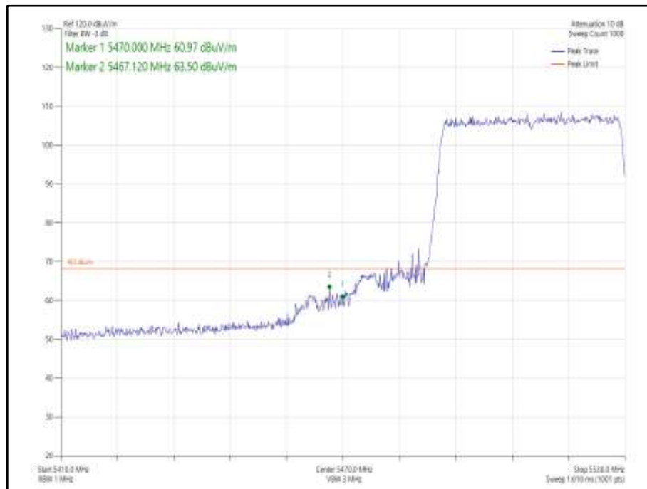
Figure 944 - 802.11ax HE40 CDD, Cores 0-1, SU - 5510 MHz Band Edge Frequency 5470 MHz
