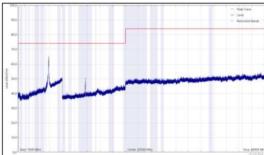
Figure 1110 - U-NII-3 - 5825 MHz (CH165), HT20, CDD, Core 0 + Core 1, 1 GHz to 40 GHz, Horizontal (Peak)
