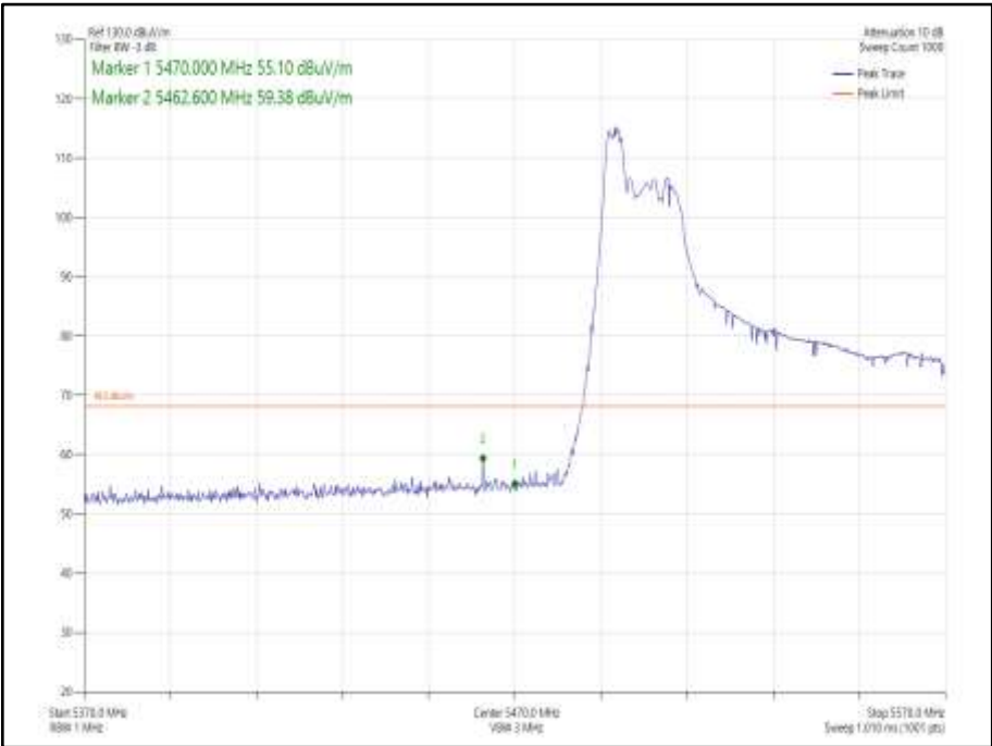
Figure 983 - 802.11ax HE80 SDM, Cores 0-1, 52-44 - 5530 MHz Band Edge Frequency 5470 MHz
