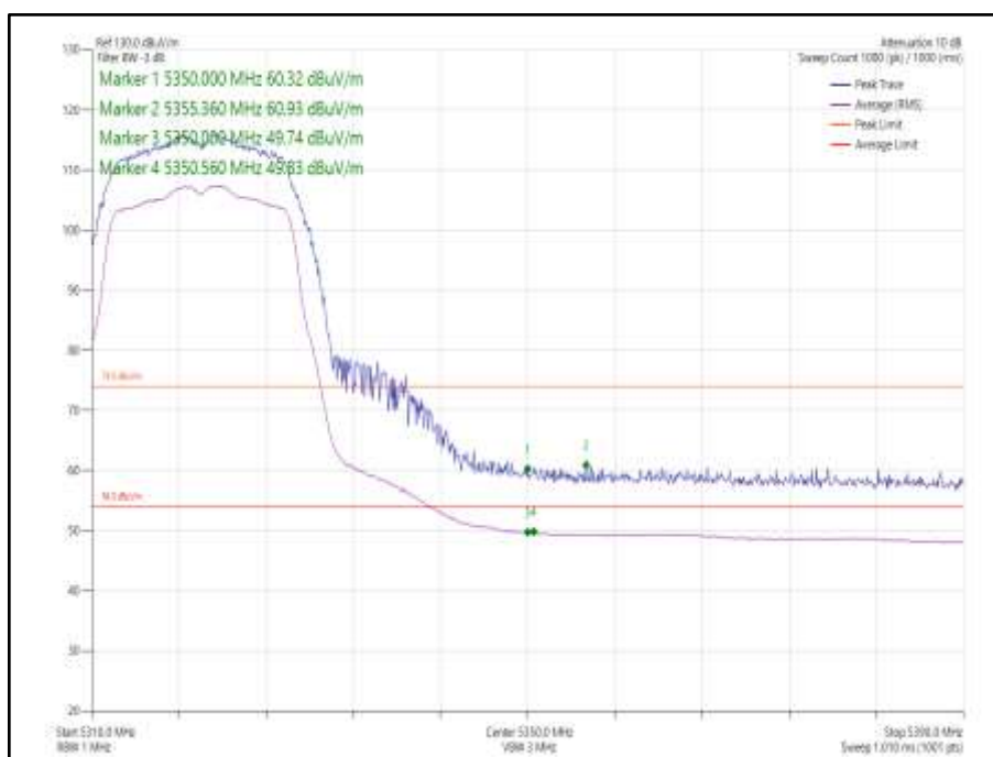
Figure 1006 - 802.11a, Core 0 - 5320 MHz, Band Edge Frequency 5350 MHz
