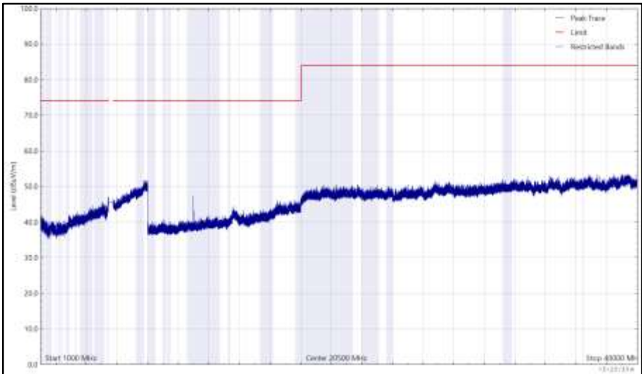
Figure 1127 - 5500 MHz (CH100), HE20, RU52-37, Core 0 + Core 1, 1 GHz to 40 GHz, Vertical (Peak)
