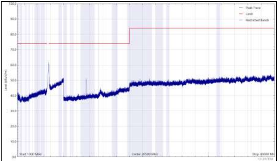
Figure 1103 - U-NII-2C - 5700 MHz (CH140), HT20, CDD, Core 0 + Core 1, 1 GHz to 40 GHz, Vertical (Peak)
