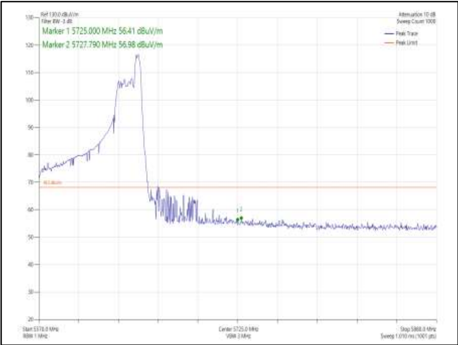
Figure 973 - 802.11ax HE80 Core 0 26-36 - 5610 MHz Band Edge Frequency 5725 MHz
