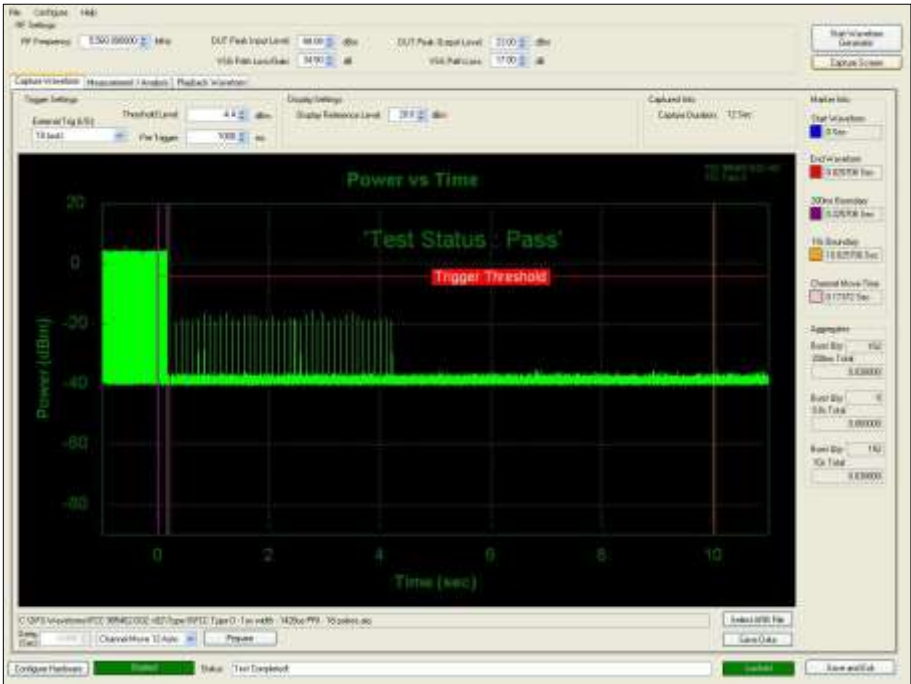
Figure 1147 - First 12 s of Channel Shutdown Period
