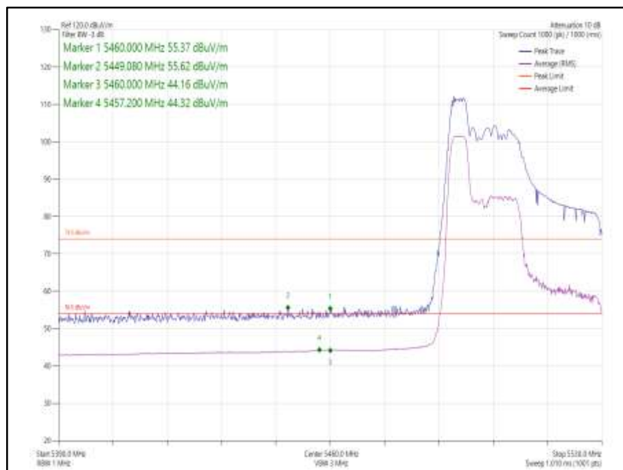
Figure 1056 - 802.11ax HE40 CDD, Cores 0-1, 52-37 - 5510 MHz Band Edge Frequency 5460 MHz
