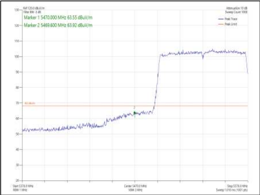
Figure 978 - 802.11ac VHT80 CDD, Cores 0-1 - 5530 MHz Band Edge Frequency 5470 MHz
