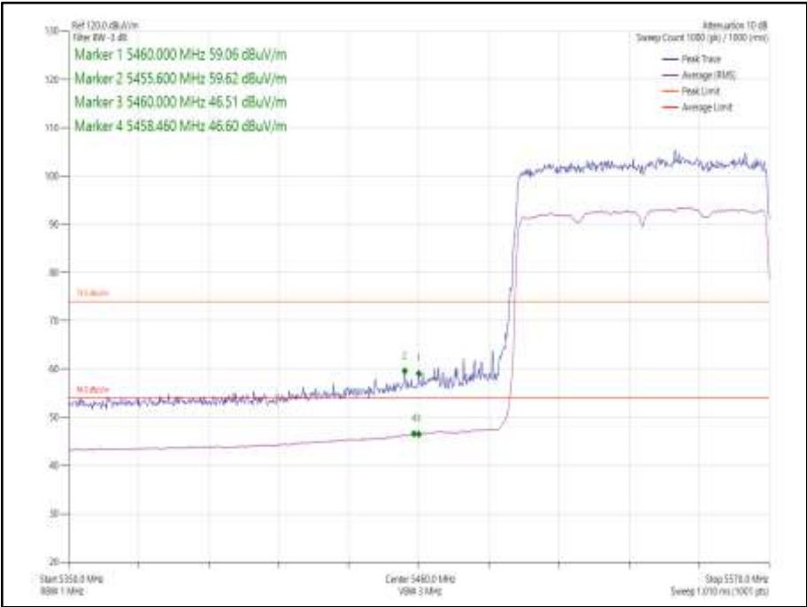
Figure 1084 - 802.11ax HE80 SDM, Cores 0-1, SU - 5530 MHz Band Edge Frequency 5460 MHz
