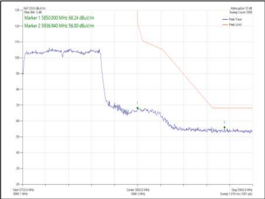
Figure 969 - 802.11ac VHT80 Core 0 - 5775 MHz Band Edge Frequency 5850 MHz
