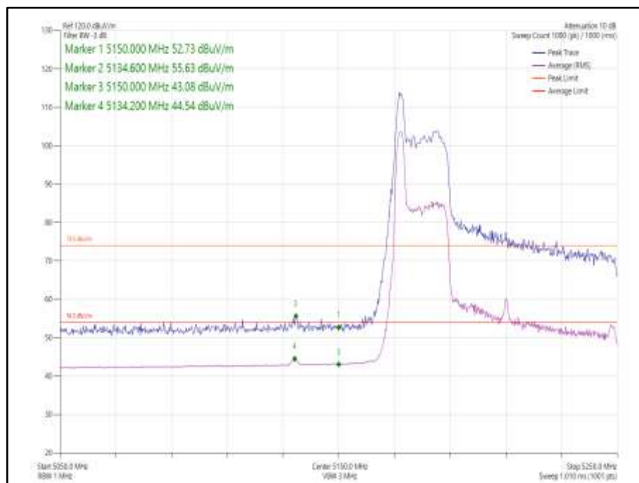
Figure 1073 - 802.11ax HE80 SDM, Cores 0-1, 26-0 - 5210 MHz Band Edge Frequency 5150 MHz
