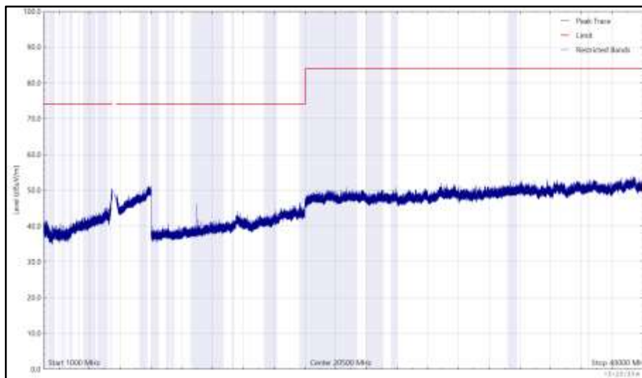
Figure 1125 - 5500 MHz (CH100), HE20, RU52-37, Core 0 + Core 1, 1 GHz to 40 GHz, Horizontal (Peak)
