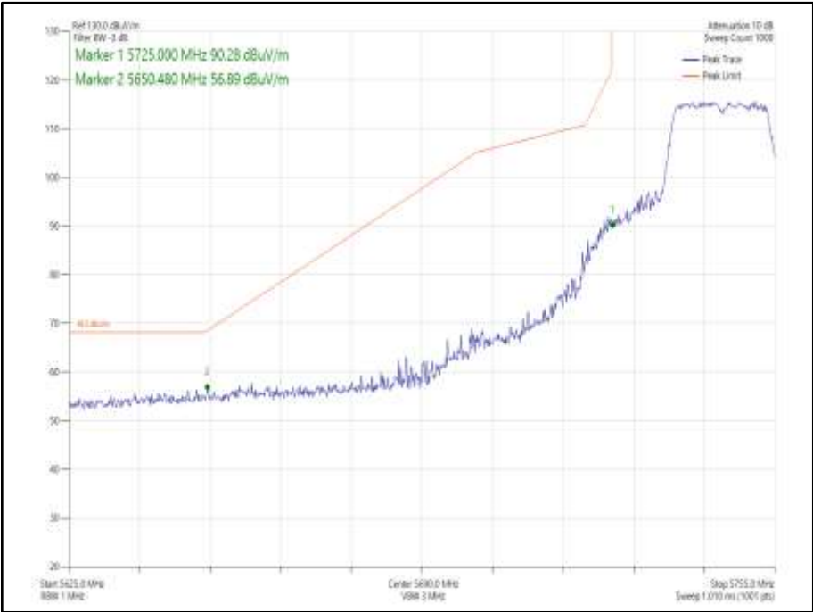
Figure 920 - 802.11ax HE20 CDD, Cores 0-1, SU - 5745 MHz Band Edge Frequency 5725 MHz
