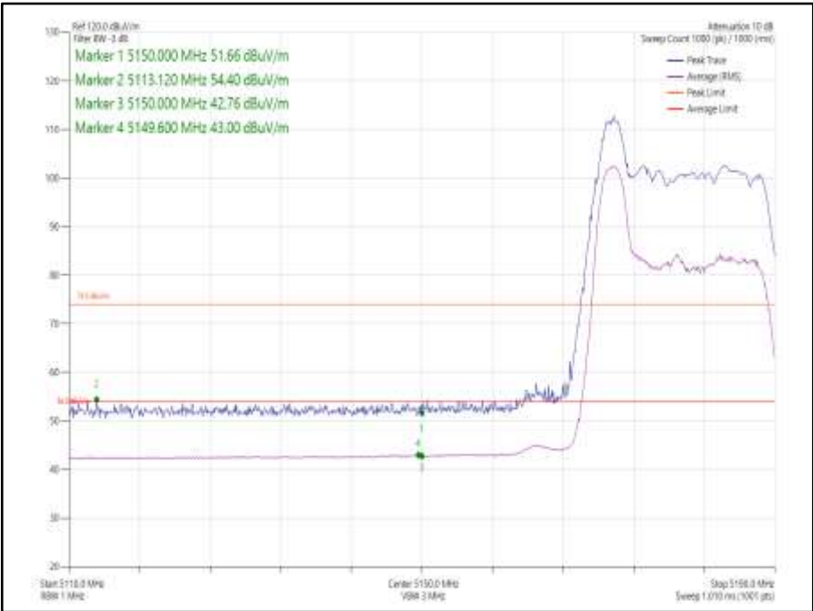
Figure 1017 - 802.11ax HE20 CDD, Cores 0-1, 26-0 - 5180 MHz Band Edge Frequency 5150 MHz
