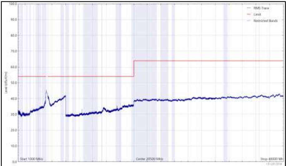
Figure 1092 - U-NII-1 - 5180 MHz (CH36), HT20, CDD, Core 0 + Core 1, 1 GHz to 40 GHz, Vertical (RMS)
