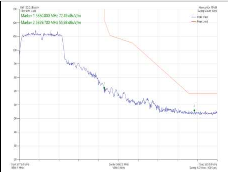
Figure 961 - 802.11n HT40 SDM, Cores 0-1 - 5795 MHz Band Edge Frequency 5850 MHz
