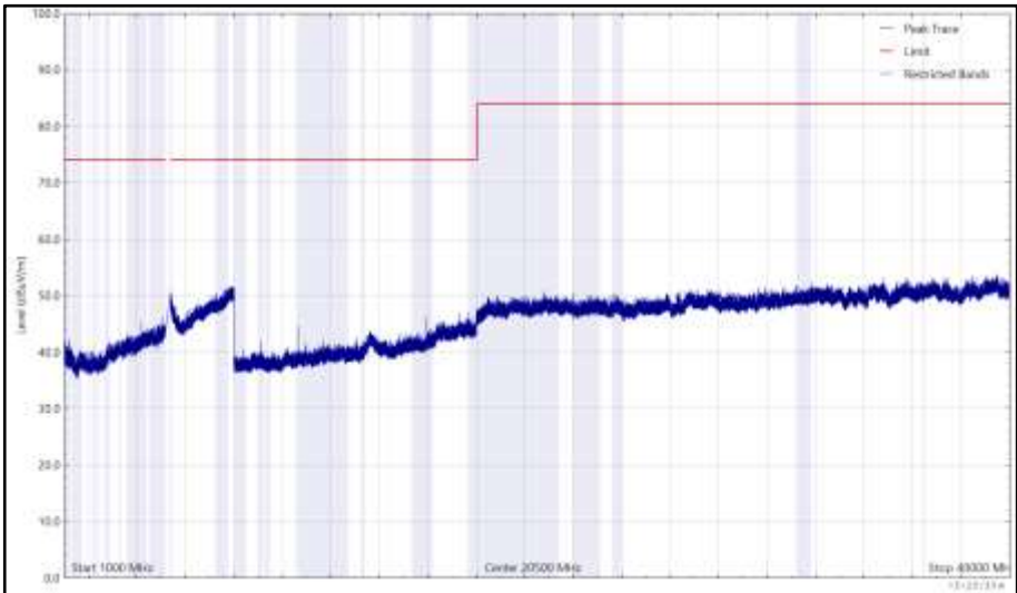
Figure 1123 - 5320 MHz (CH64), HE20, RU52-37, Core 0 + Core 1, 1 GHz to 40 GHz, Vertical (Peak)
