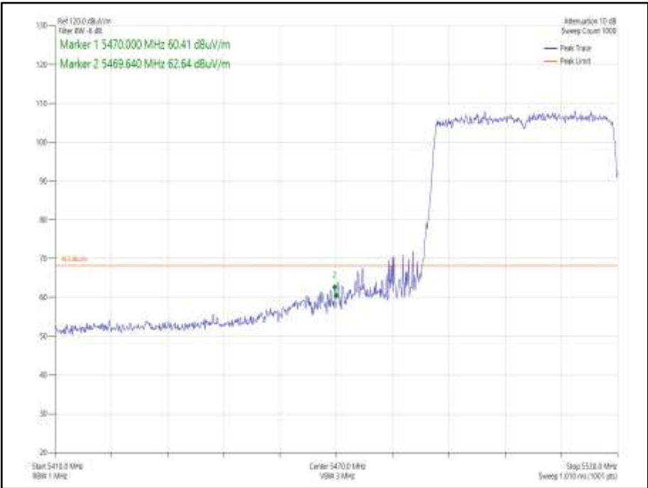
Figure 934 - 802.11ax HE40, Core 0, SU - 5510 MHz Band Edge Frequency 5470 MHz
