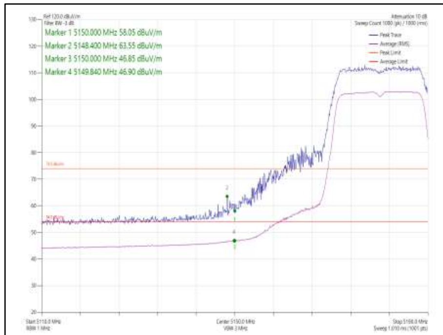
Figure 1003 - 802.11n HT20, Core 1 - 5180 MHz, Band Edge Frequency 5150 MHz
