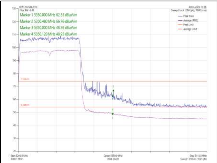
Figure 1036 - 802.11ax HE40, Core 0, SU - 5310 MHz Band Edge Frequency 5350 MHz
