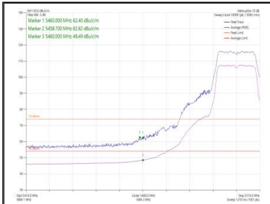
Figure 9 - 802.11a, Core 0 - 5500 MHz, Band Edge Frequency 5460 MHz
