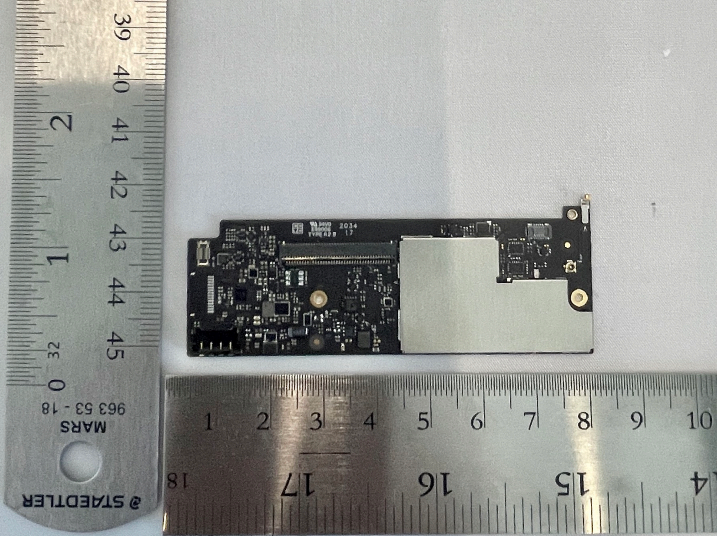
A2449 MLB Front - with shields
