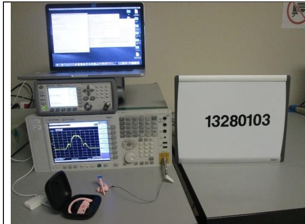
RF CONDUCTED
