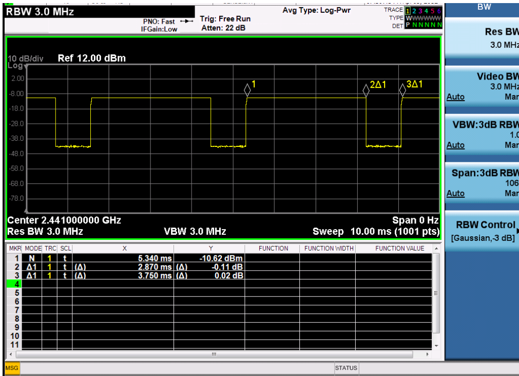
Figure 8-3 Bluetooth Transmission Plot – Ant 4a – Variant 1
