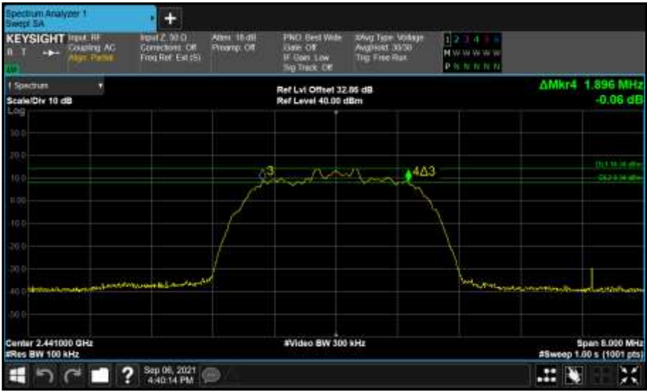
Figure 58 - Core 0 (A) 2441 MHz (CH39) 6 dB Bandwidth
