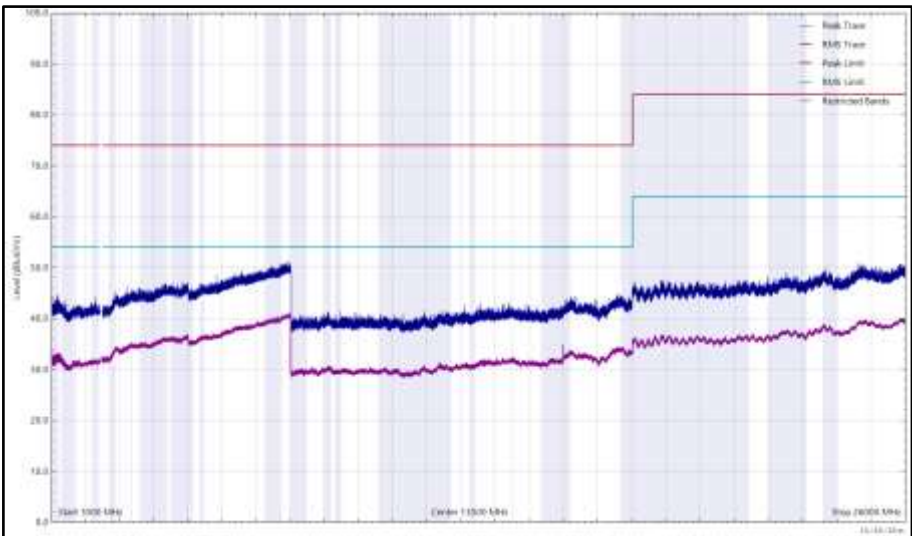
Figure 213 - 2440 MHz (CH17), LE1M, ePA, Core 0 + Core 1, 1 GHz to 26 GHz, Horizontal
