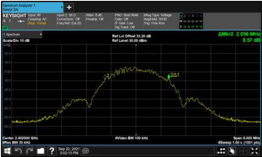
Figure 103 - Core 1 (B) 2402 MHz (CH37) 99% Bandwidth
