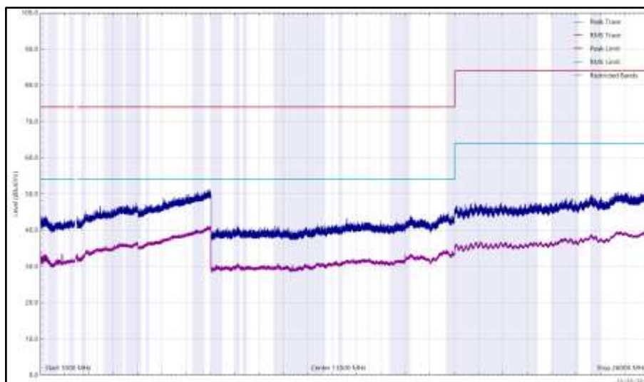
Figure 224 - 2480 MHz (CH39), LE1M, iPA, Core 0 + Core 1, 1 GHz to 26 GHz, Horizontal
