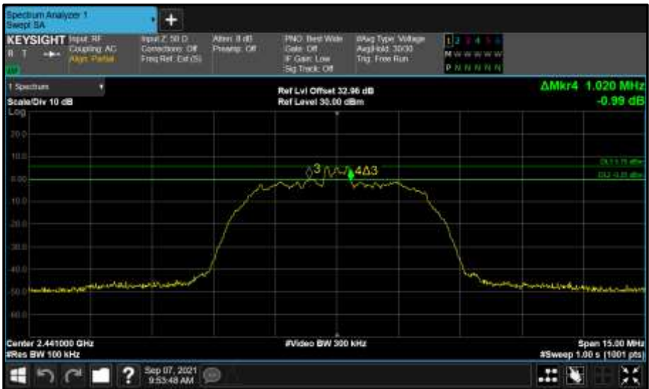
Figure 134 - Core 2 (C) 2441 MHz (CH39) 6 dB Bandwidth
