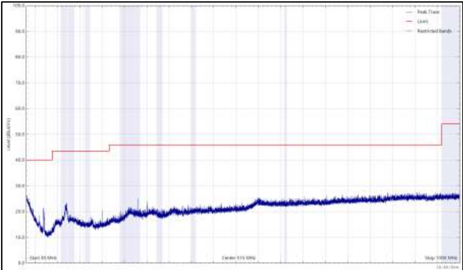
Figure 212 - 2440 MHz (CH17), LE1M, ePA, Core 0 + Core 1, 30 MHz to 1 GHz, Horizontal (Peak)
