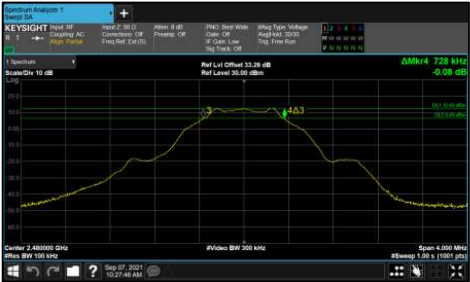
Figure 166 - Core 1 (B) 2480 MHz (CH39) 6 dB Bandwidth
