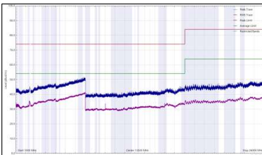
Figure 75 - 2402 MHz (CH0), DH5, iPA, Core 0 + Core 1, 1 GHz to 26 GHz, Vertical
