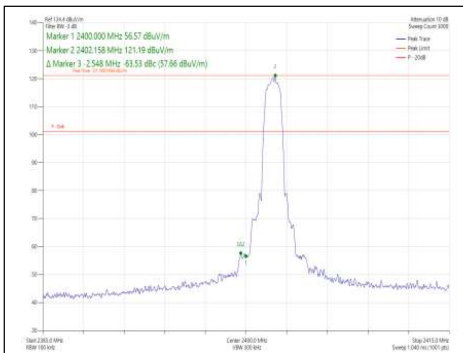
Figure 123 - Static - \pi/4 DQPSK/2DH5 - 2402 MHz - Band Edge Frequency 2400.0 MHz
