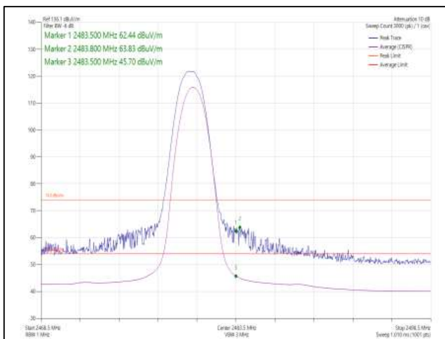
Figure 29 - Static - \pi/4 DQPSK/2DH5 - 2480 MHz - Band Edge Frequency 2483.5 MHz
