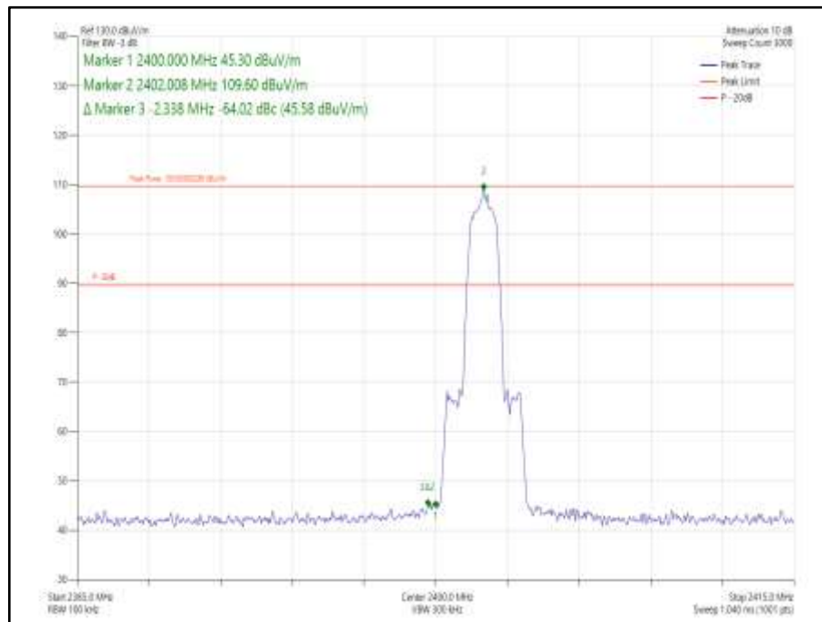
Figure 111 - Static - \pi/4 DQPSK/2DH5 - 2402 MHz - Band Edge Frequency 2400.0 MHz
