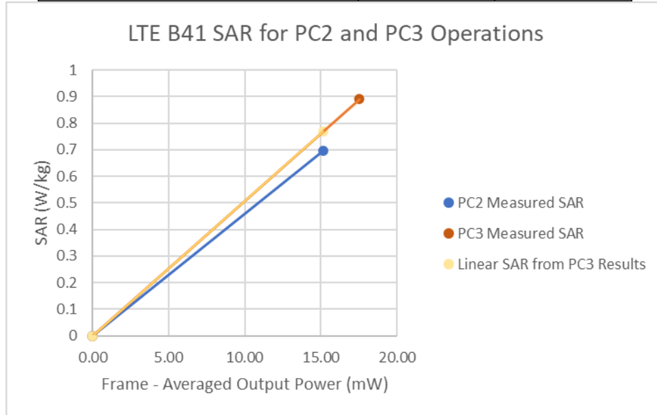
Figure 13-6 LTE Band 41 ULCA Body Linearity – Antenna 3a
