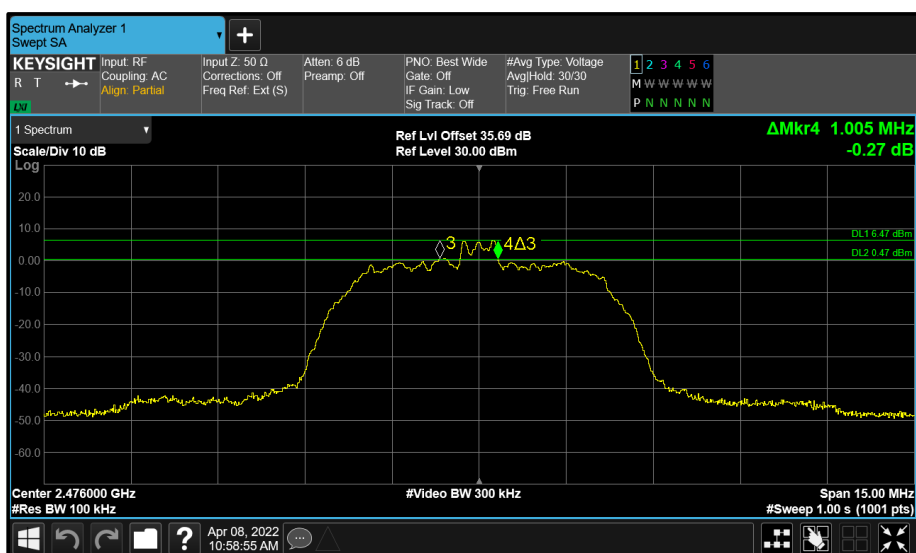
Figure 116 - Core 0 (A) 2476 MHz (CH74) 6 dB Bandwidth
