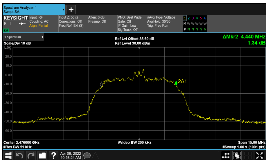
Figure 115 - Core 0 (A) 2476 MHz (CH74) 99% Bandwidth
