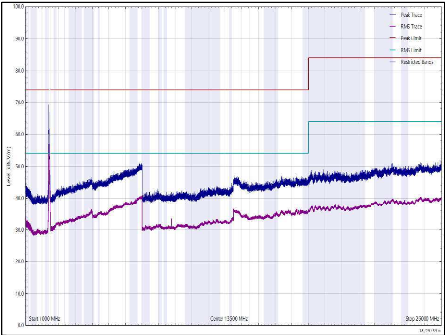
Figure 67 - 2412 MHz (CH1), 802.11g, Core 1, 1 GHz to 26 GHz, Vertical
