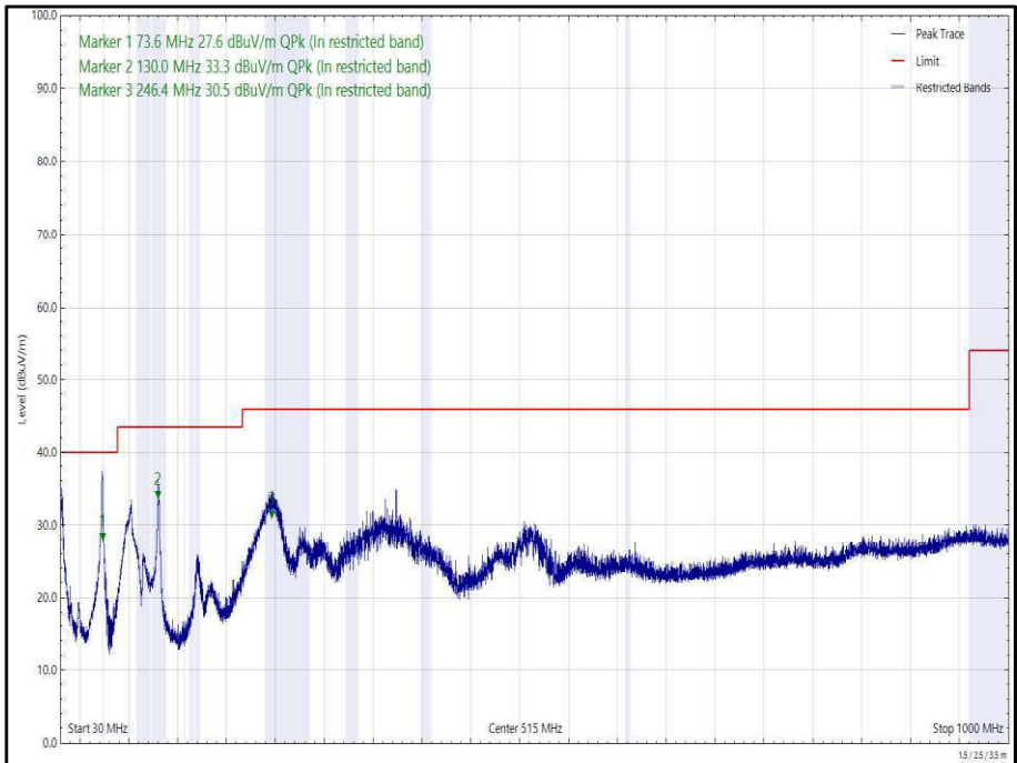
Figure 68 - 2437 MHz (CH6), 802.11g, Core 1, 30 MHz to 1 GHz, Horizontal (Peak)
