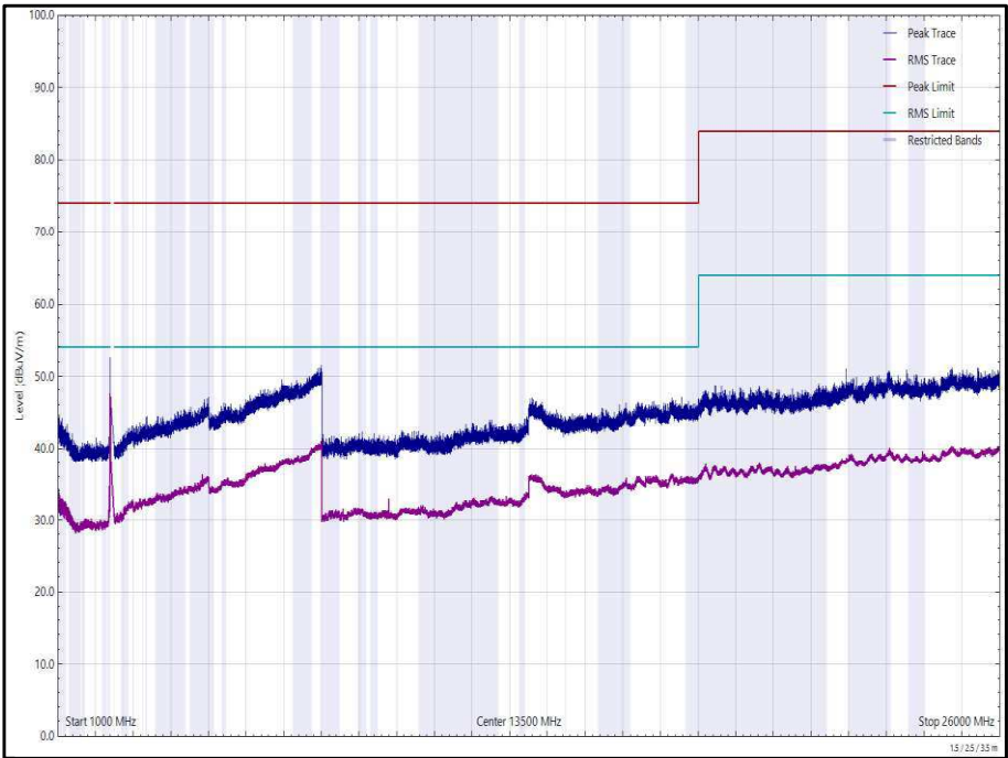
Figure 83 - 2412 MHz (CH1), 802.11b, Core 1, 1 GHz to 26 GHz, Vertical
