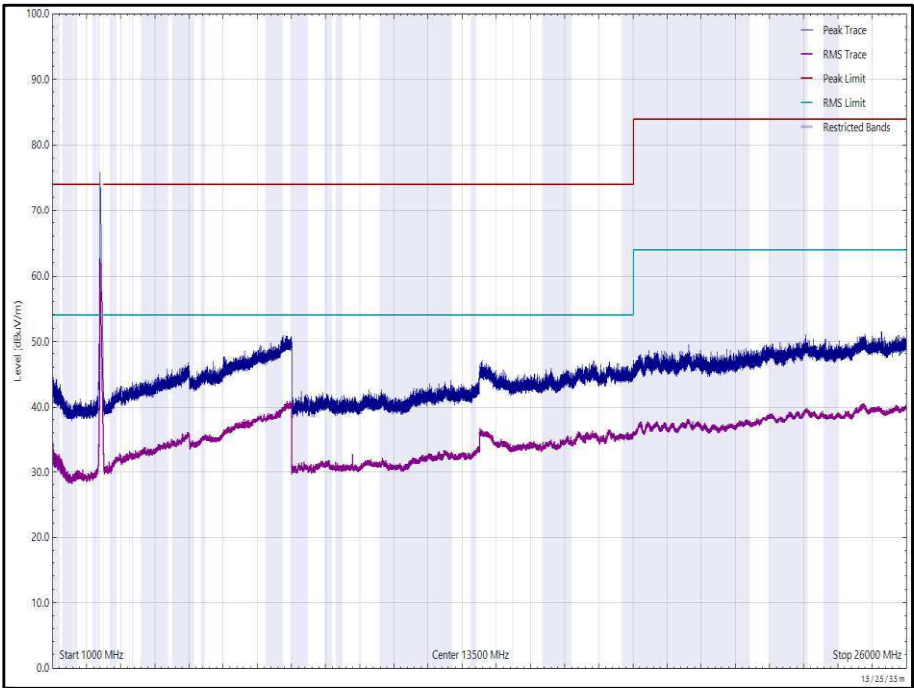
Figure 51 - 2412 MHz (CH1), HT20, CDD, Core 0 + Core 1, 1 GHz to 26 GHz, Vertical
