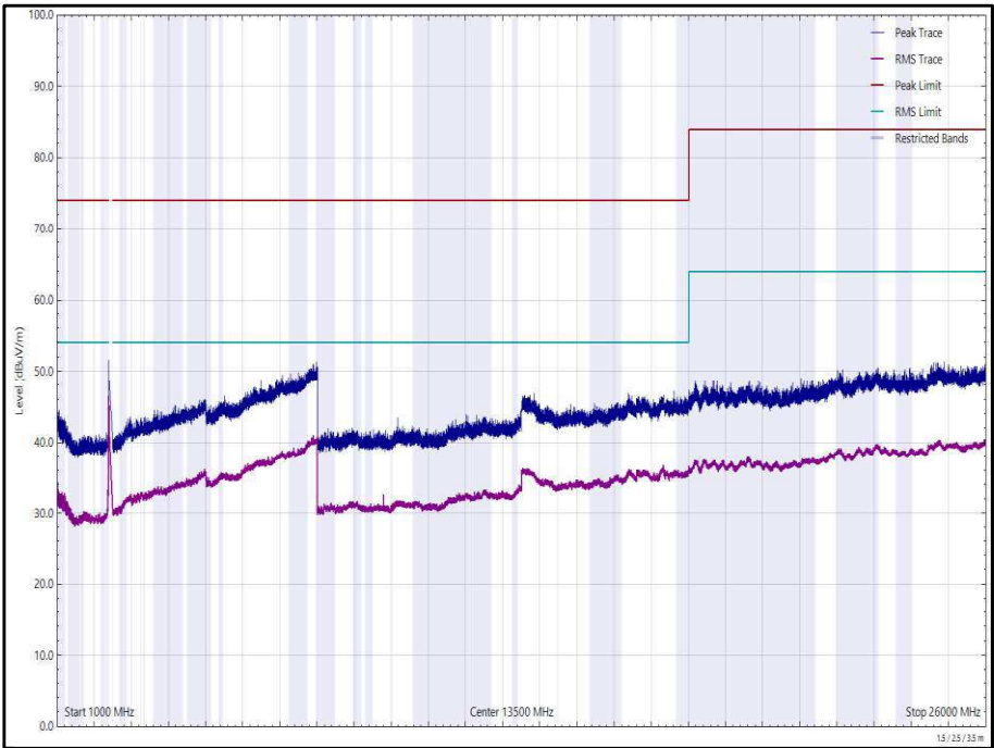
Figure 75 - 2412 MHz (CH1), 802.11b, Core 0, 1 GHz to 26 GHz, Vertical
