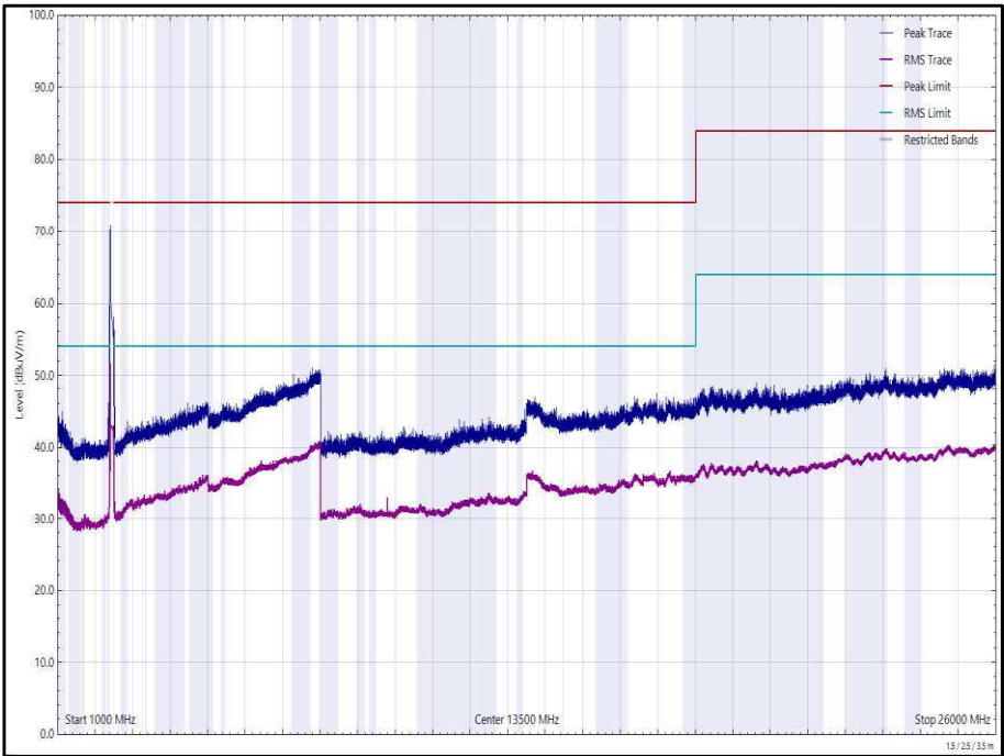
Figure 91 - 2437 MHz (CH6), HE20, RU26-0, Core 0 + Core 1, 1 GHz to 26 GHz, Vertical
