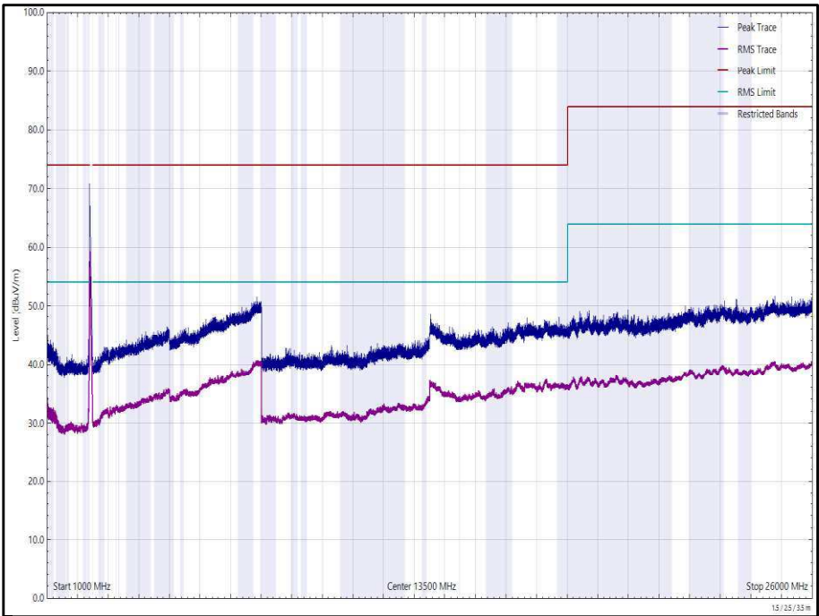
Figure 50 - 2412 MHz (CH1), HT20, CDD, Core 0 + Core 1, 1 GHz to 26 GHz, Horizontal
