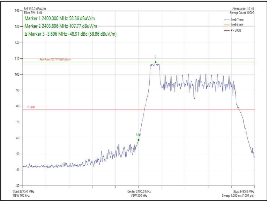
Figure 98- 802.11ax HE20, Core 0, 26-0 - 2412 MHz Band Edge Frequency 2400 MHz
