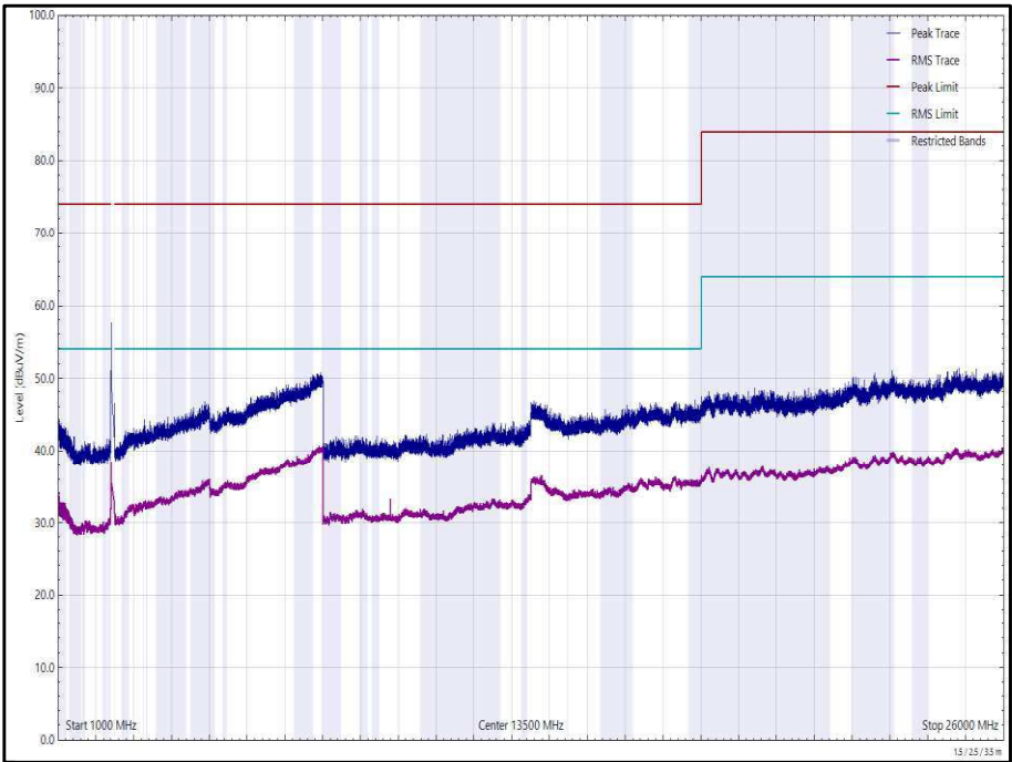
Figure 79 - 2437 MHz (CH6), 802.11b, Core 0, 1 GHz to 26 GHz, Vertical
