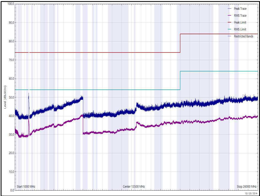
Figure 61 - 2437 MHz (CH6), 802.11g, Core 0, 1 GHz to 26 GHz, Horizontal
