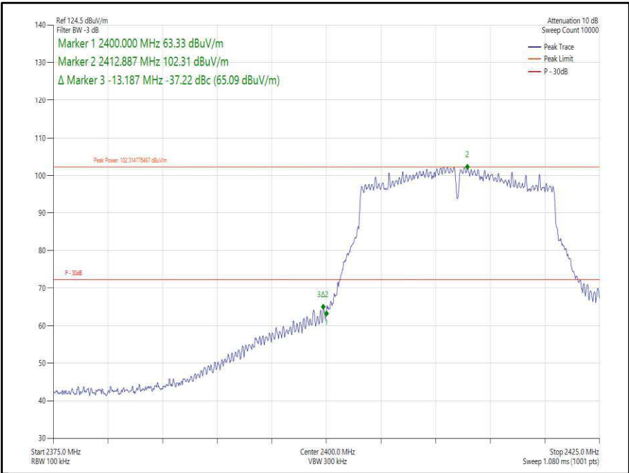
Figure 96- 802.11n HT20, Core 0 - 2412 MHz Band Edge Frequency 2400 MHz
