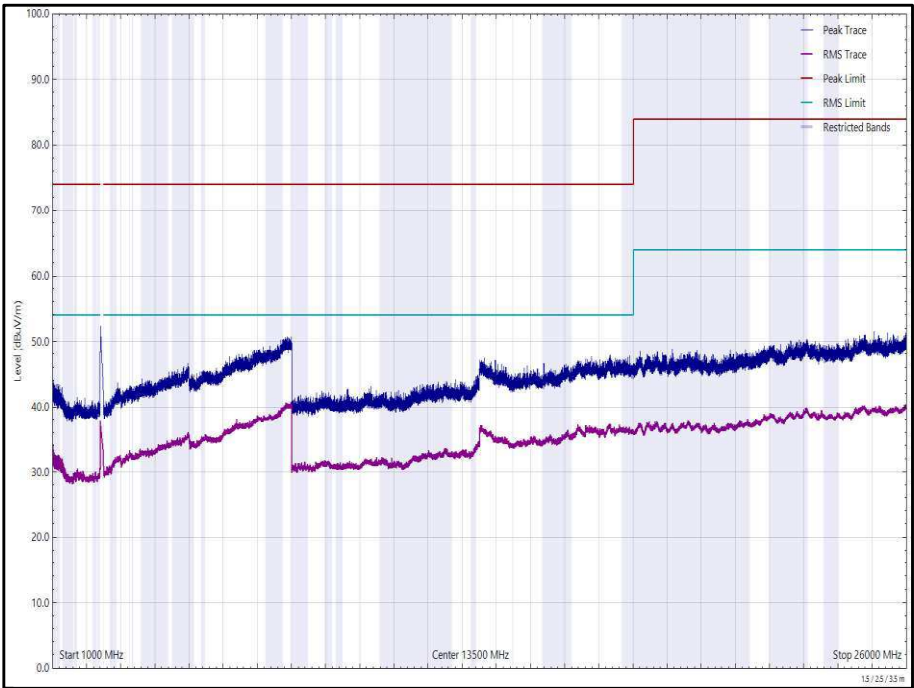
Figure 69 - 2437 MHz (CH6), 802.11g, Core 1, 1 GHz to 26 GHz, Horizontal
