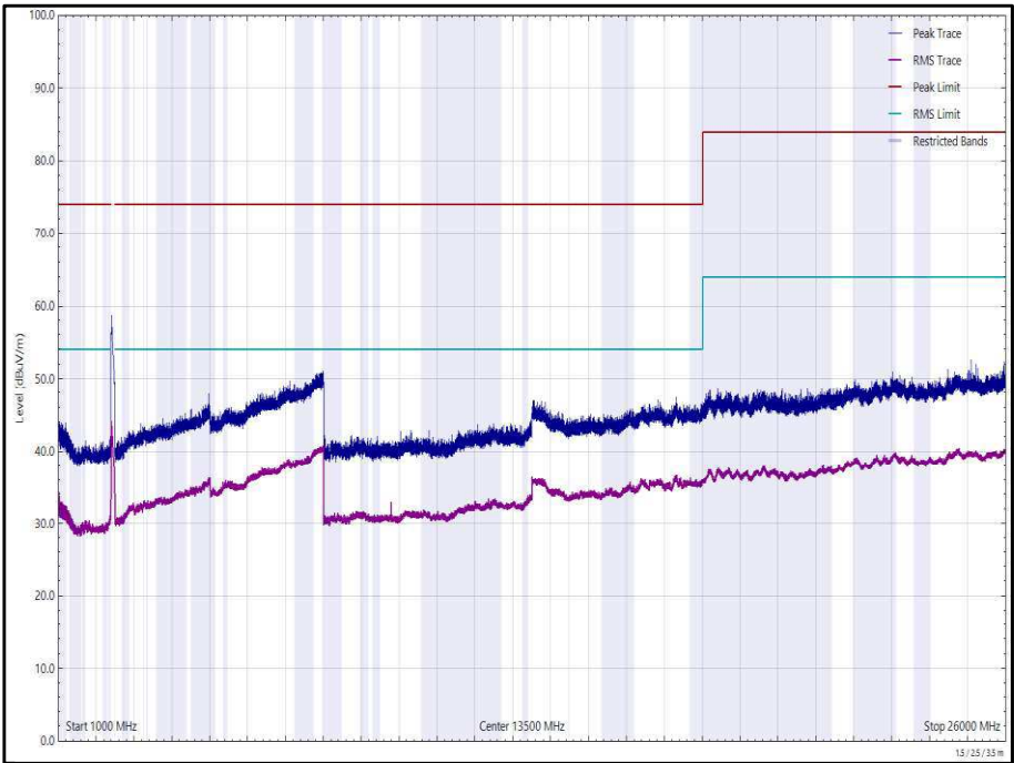
Figure 63 - 2437 MHz (CH6), 802.11g, Core 0, 1 GHz to 26 GHz, Vertical
