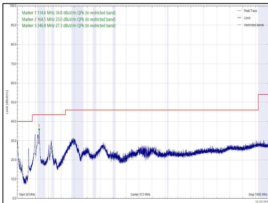
Figure 76 - 2437 MHz (CH6), 802.11b, Core 0, 30 MHz to 1 GHz, Horizontal (Peak)
