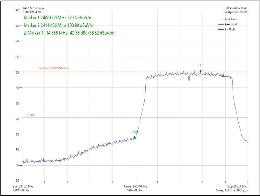
Figure 97- 802.11ax HE20, Core 0, SU - 2412 MHz Band Edge Frequency 2400 MHz
