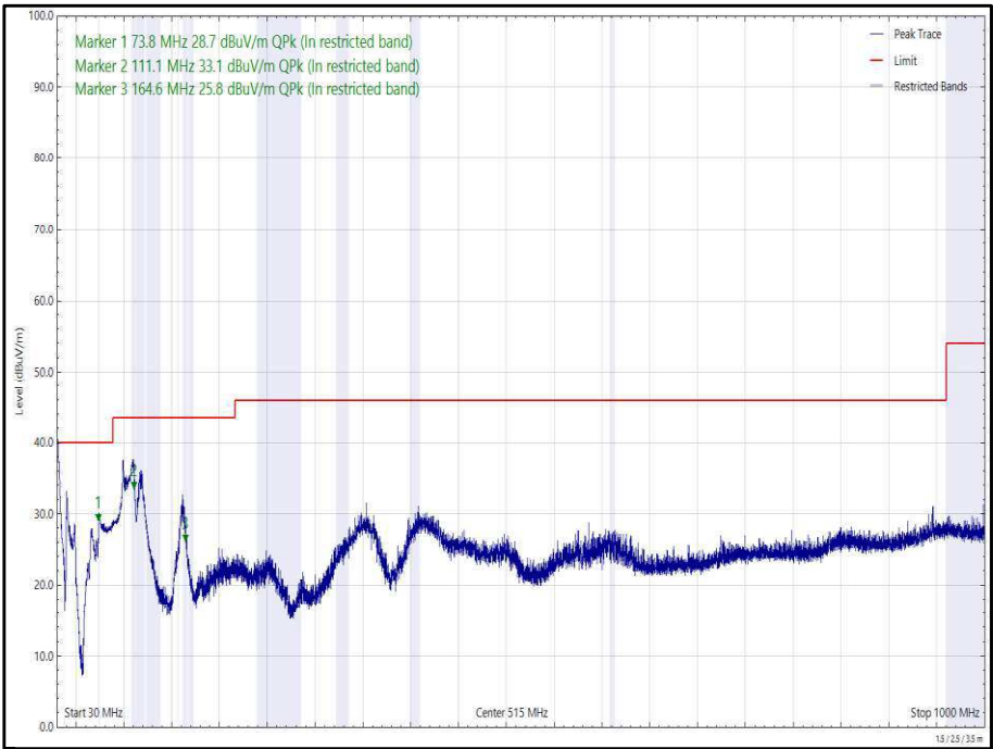
Figure 78 - 2437 MHz (CH6), 802.11b, Core 0, 30 MHz to 1 GHz, Vertical (Peak)
