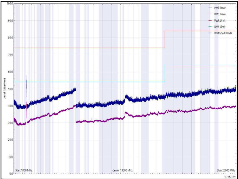
Figure 71 - 2437 MHz (CH6), 802.11g, Core 1, 1 GHz to 26 GHz, Vertical
