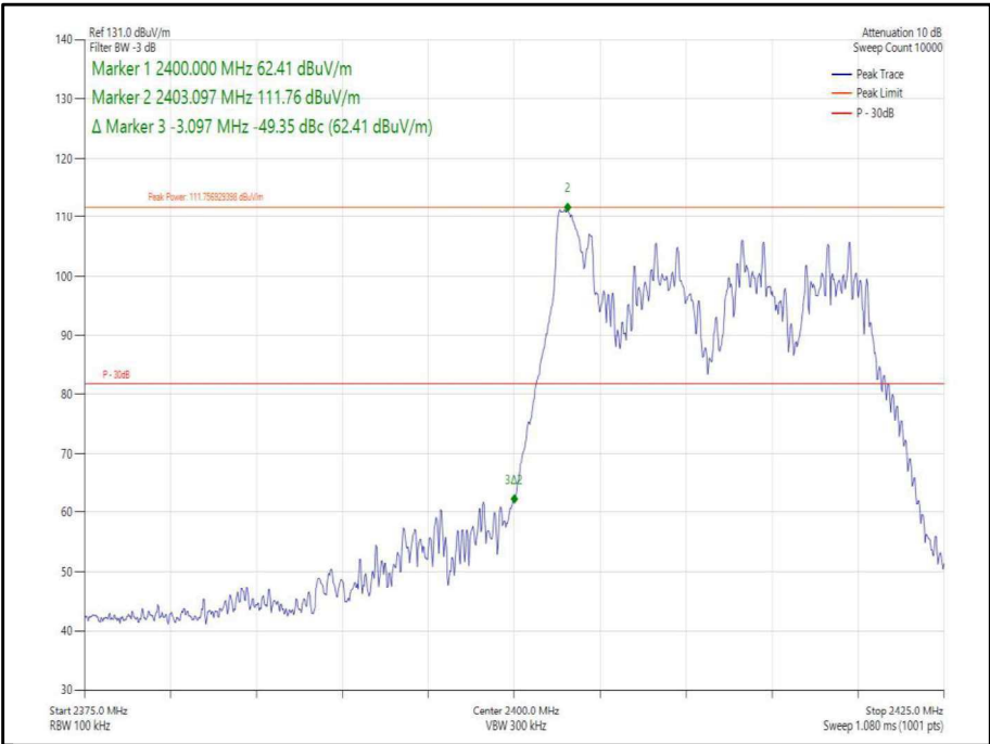
Figure 101- 802.11ax HE20, Cores 0-1, 26-0 - 2412 MHz Band Edge Frequency 2400 MHz
