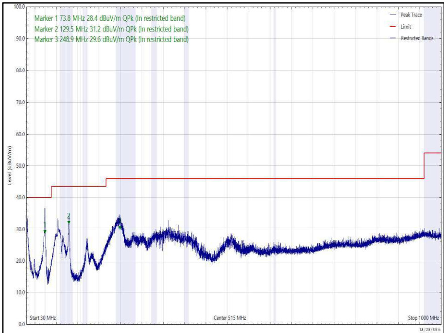
Figure 60 - 2437 MHz (CH6), 802.11g, Core 0, 30 MHz to 1 GHz, Horizontal (Peak)
