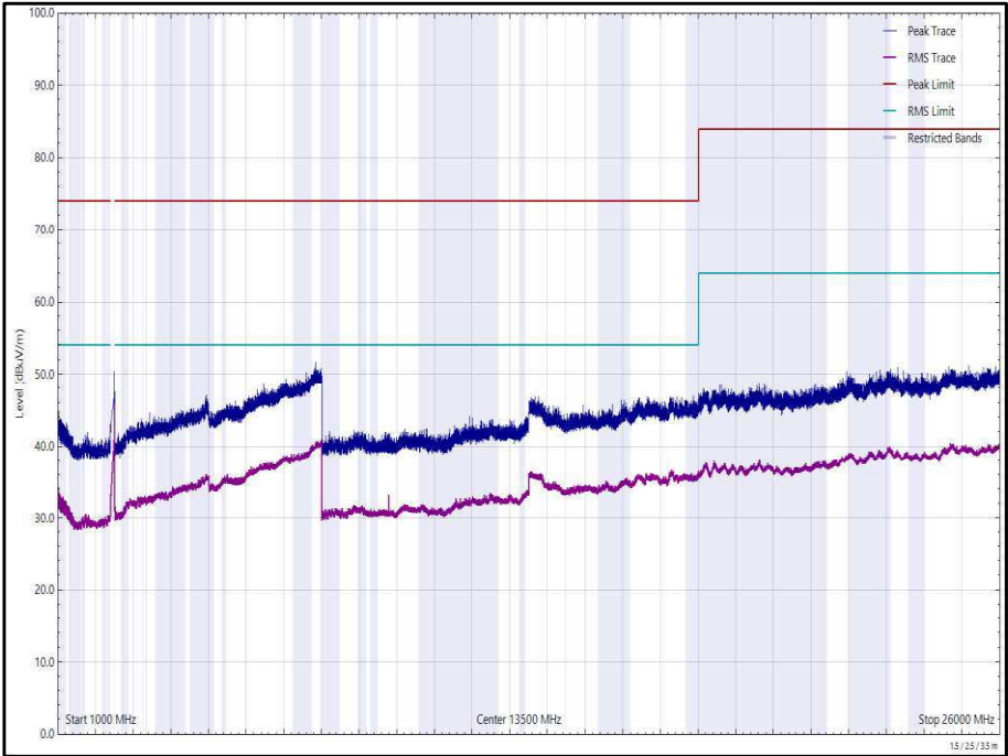
Figure 87 - 2472 MHz (CH13), 802.11b, Core 1, 1 GHz to 26 GHz, Vertical
