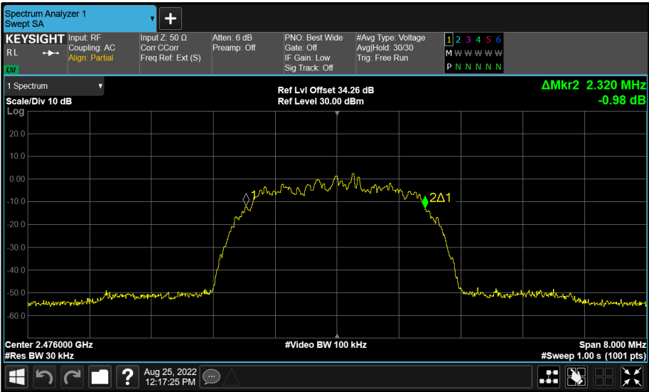
Figure 61 - Core 1 (B) 2476 MHz (CH74) 99% Bandwidth
