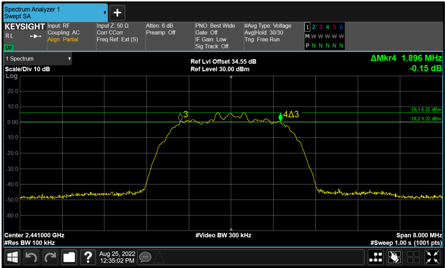
Figure 48 - BT Core 2 (C) 2441 MHz (CH39) 6 dB Bandwidth
