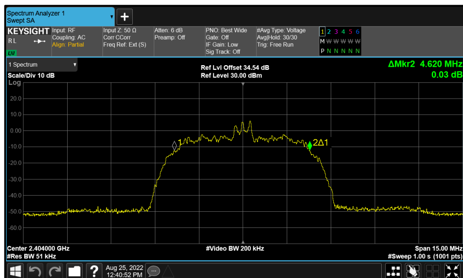
Figure 51 - BT Core 2 (C) 2404 MHz (CH2) 99% Bandwidth
