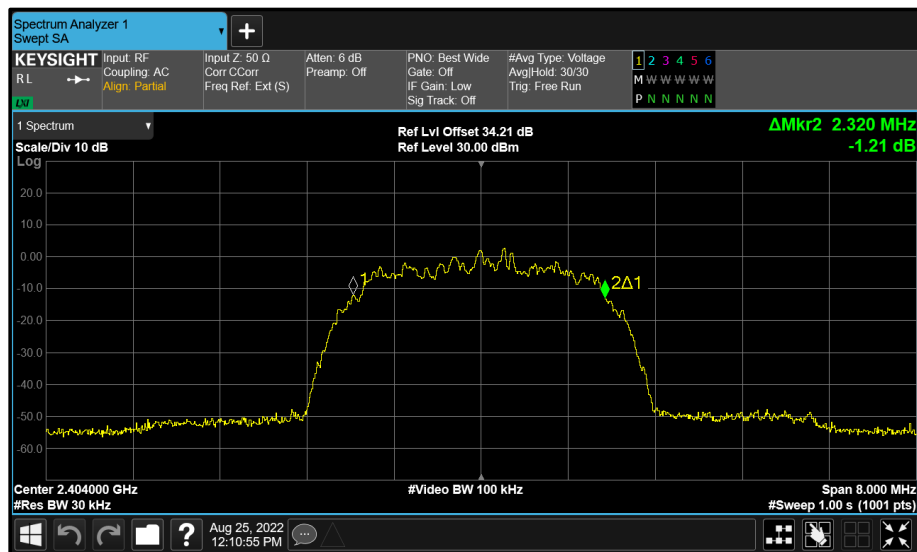
Figure 57 - Core 1 (B) 2404 MHz (CH2) 99% Bandwidth
