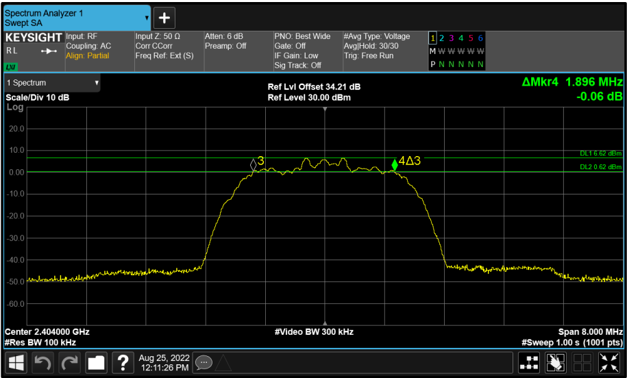
Figure 58 - Core 1 (B) 2404 MHz (CH2) 6 dB Bandwidth
