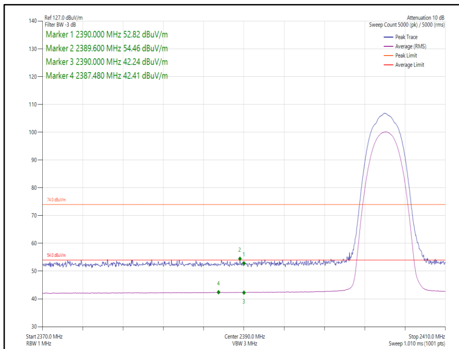
Figure 25 Core 0-1- Static - GFSK/4-DH5 - 2404 MHz - Band Edge Frequency 2390.0 MHz
