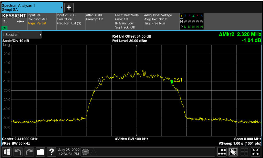
Figure 47 - BT Core 2 (C) 2441 MHz (CH39) 99% Bandwidth
