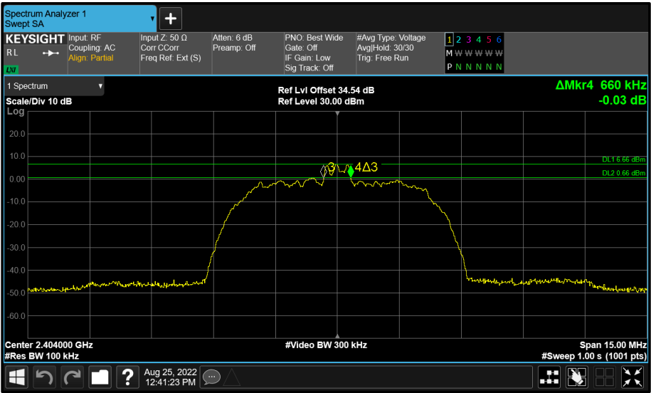
Figure 52 - BT Core 2 (C) 2404 MHz (CH2) 6 dB Bandwidth
