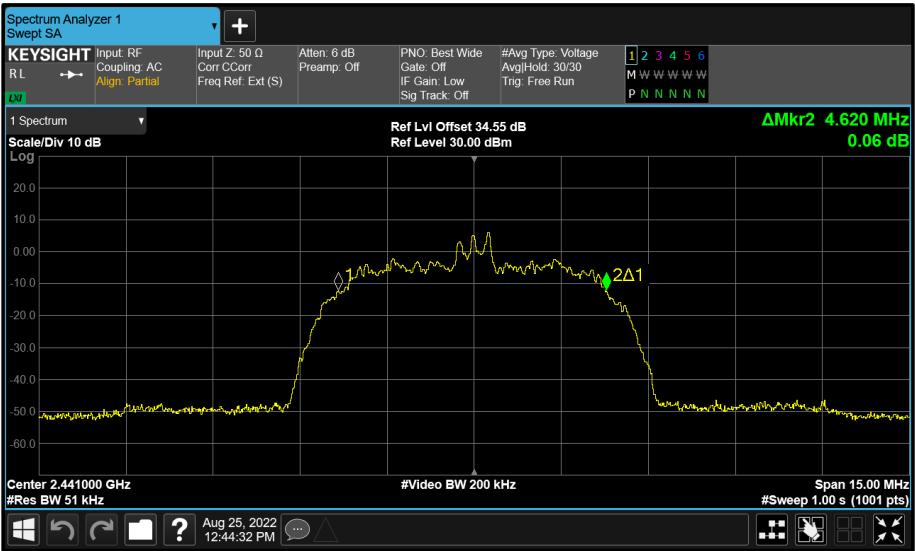
Figure 53 - BT Core 2 (C) 2441 MHz (CH39) 99% Bandwidth
