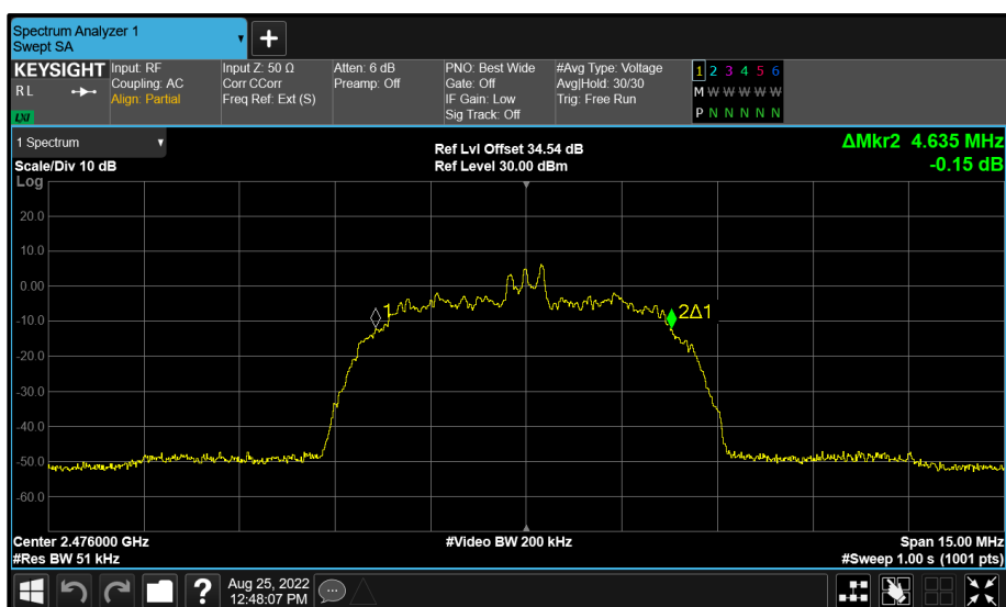
Figure 55 - BT Core 2 (C) 2476 MHz (CH74) 99% Bandwidth
