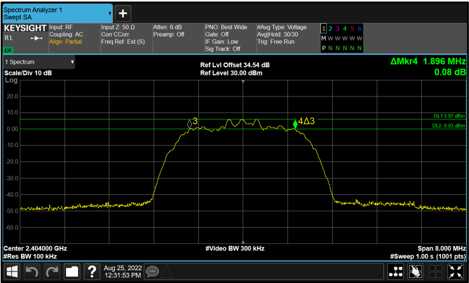
Figure 46 - BT Core 2 (C) 2404 MHz (CH2) 6 dB Bandwidth
