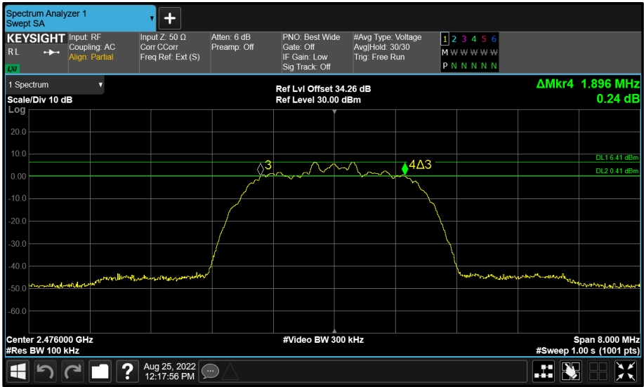
Figure 62 - Core 1 (B) 2476 MHz (CH74) 6 dB Bandwidth
