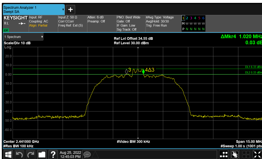
Figure 54 - BT Core 2 (C) 2441 MHz (CH39) 6 dB Bandwidth
