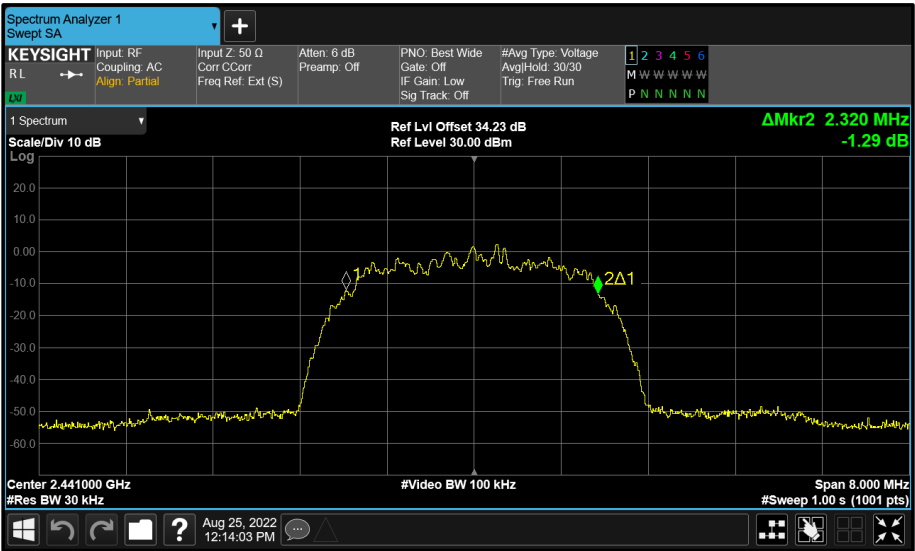
Figure 59 - Core 1 (B) 2441 MHz (CH39) 99% Bandwidth
