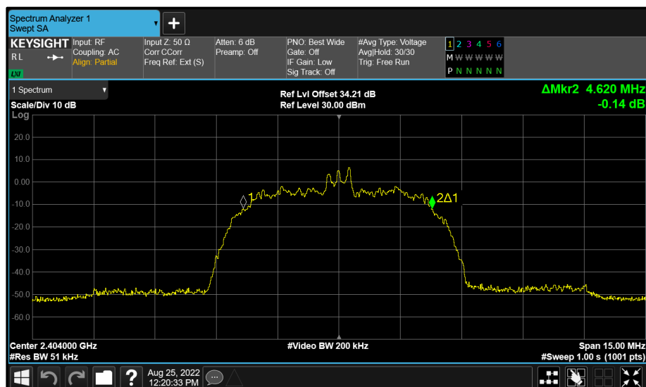
Figure 63 - Core 1 (B) 2404 MHz (CH2) 99% Bandwidth
