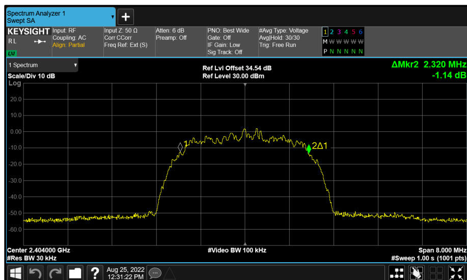
Figure 45 - BT Core 2 (C) 2404 MHz (CH2) 99% Bandwidth
