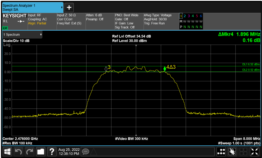
Figure 50 - BT Core 2 (C) 2476 MHz (CH74) 6 dB Bandwidth
