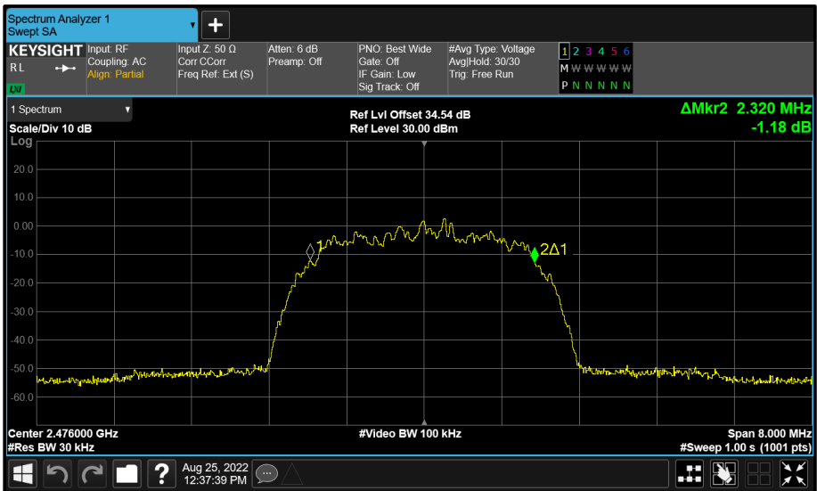
Figure 49 - BT Core 2 (C) 2476 MHz (CH74) 99% Bandwidth
