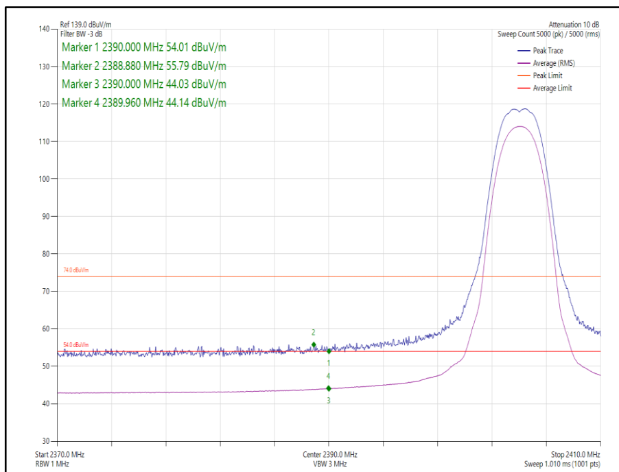
Figure 15 Core 1- Static - GFSK/4-DH5 - 2404 MHz - Band Edge Frequency 2390.0 MHz
