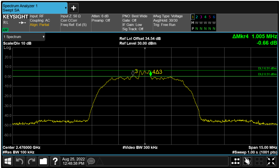
Figure 56 - BT Core 2 (C) 2476 MHz (CH74) 6 dB Bandwidth
