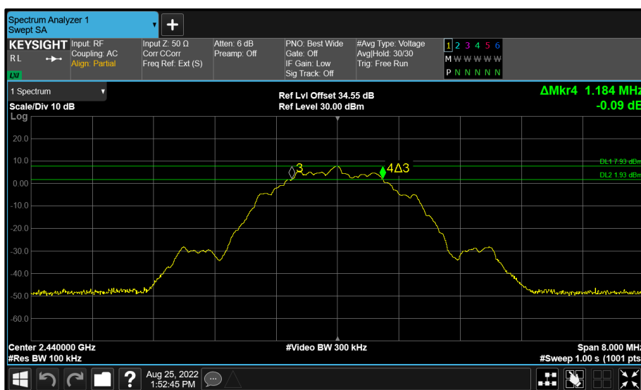
Figure 90 - BT Core 2 (C) 2440 MHz (CH17) 6 dB Bandwidth
