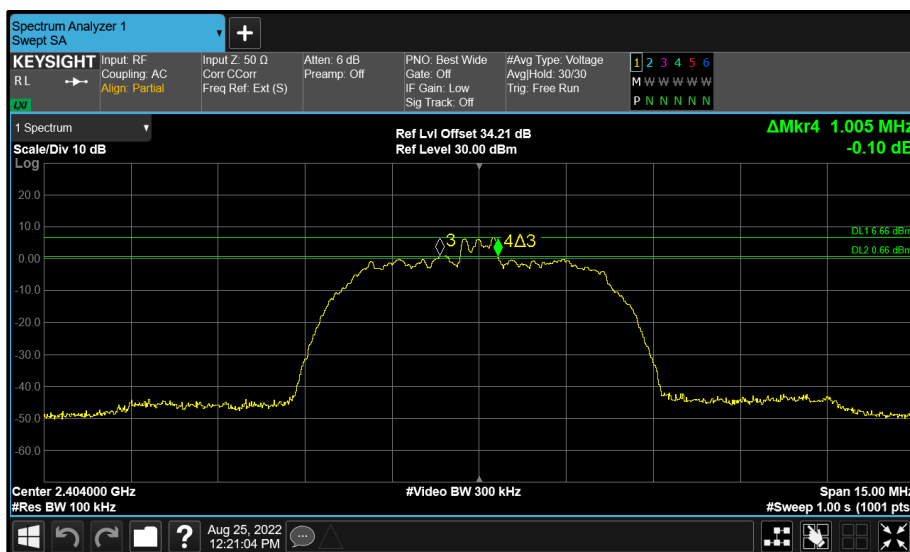
Figure 64 - Core 1 (B) 2404 MHz (CH2) 6 dB Bandwidth
