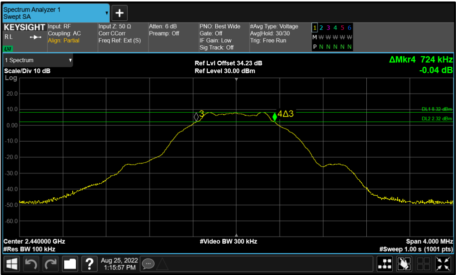
Figure 72 - Core 1 (B) 2440 MHz (CH17) 6 dB Bandwidth
