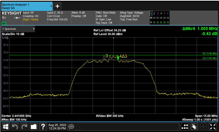
Figure 66 - Core 1 (B) 2441 MHz (CH39) 6 dB Bandwidth
