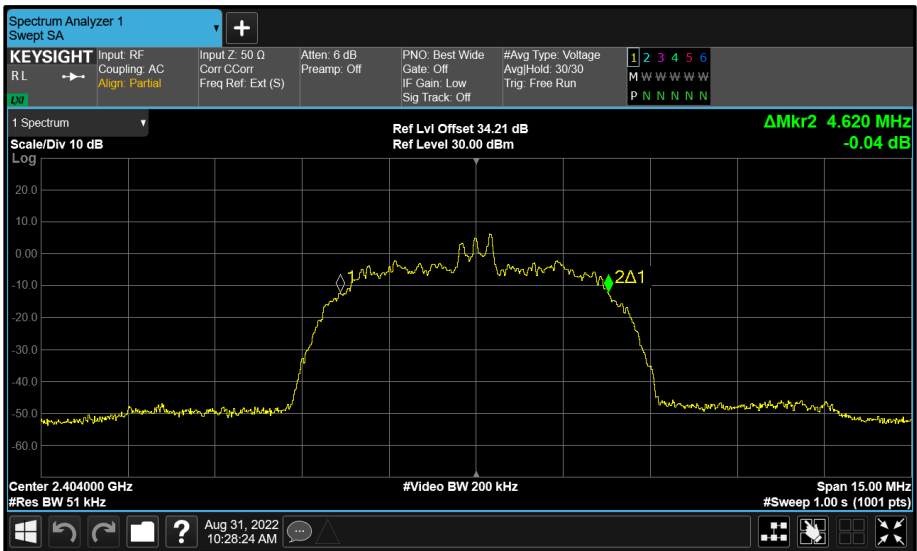
Figure 131 - Core 1 (B) 2404 MHz (CH2) 99% Bandwidth
