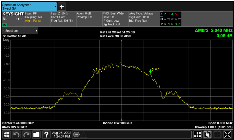
Figure 77 - Core 1 (B) 2440 MHz (CH17) 99% Bandwidth
