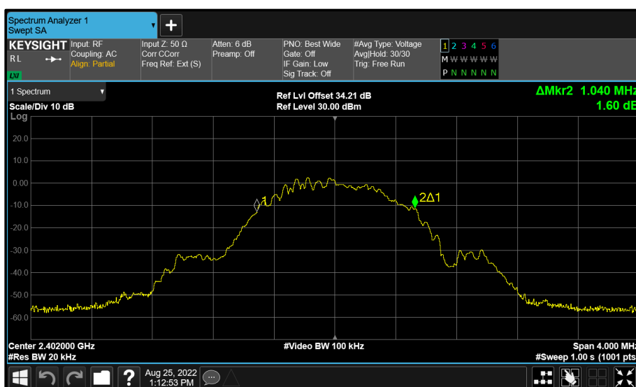
Figure 69 - Core 1 (B) 2402 MHz (CH37) 99% Bandwidth
