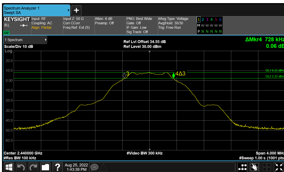
Figure 84 - BT Core 2 (C) 2440 MHz (CH17) 6 dB Bandwidth
