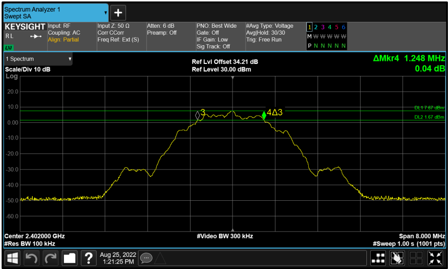
Figure 76 - Core 1 (B) 2402 MHz (CH37) 6 dB Bandwidth
