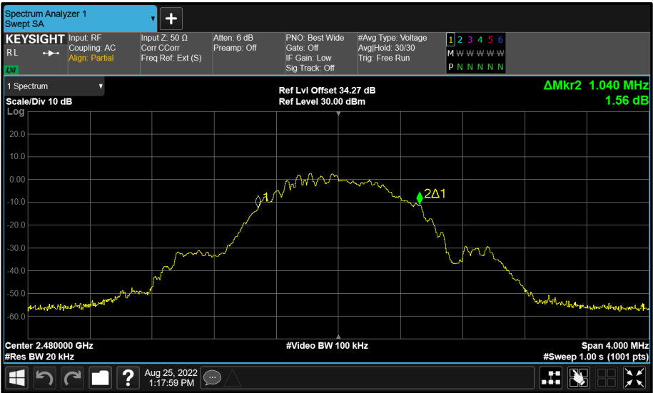
Figure 73 - Core 1 (B) 2480 MHz (CH39) 99% Bandwidth
