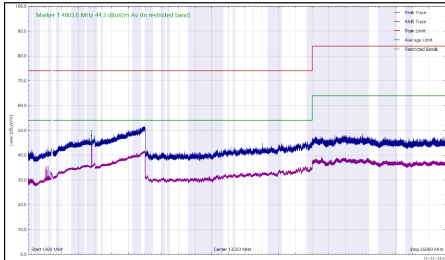
Figure 129 - 2402 MHz (CH0), DH5, iPA, Core 2, 1 GHz to 26 GHz, Horizontal
