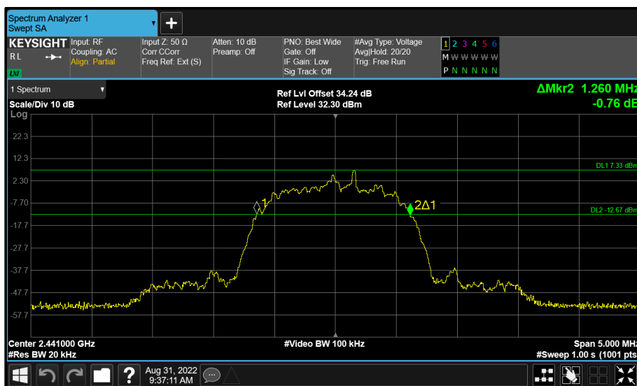
Figure 116 - Core 0 (A) 2441 MHz (CH39) 20 dB Bandwidth
