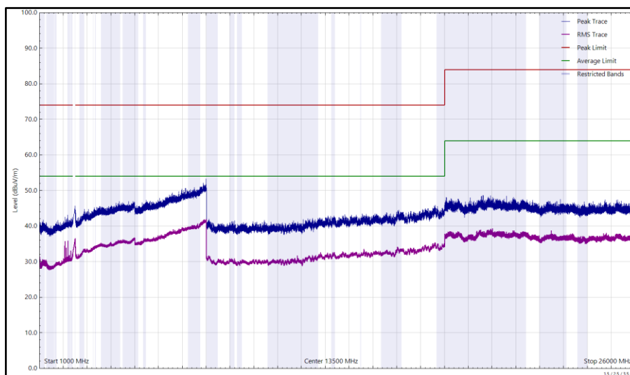
Figure 143 - 2480 MHz (CH78), 2DH5, ePA, Core 0 + Core 1, 1 GHz to 26 GHz, Horizontal
