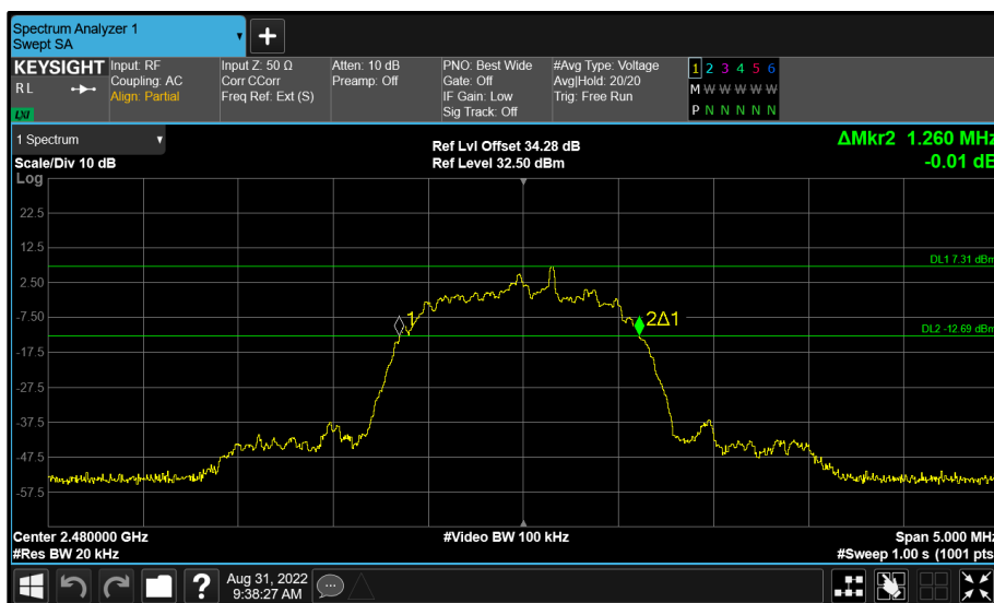
Figure 118 - Core 0 (A) 2480 MHz (CH78) 20 dB Bandwidth
