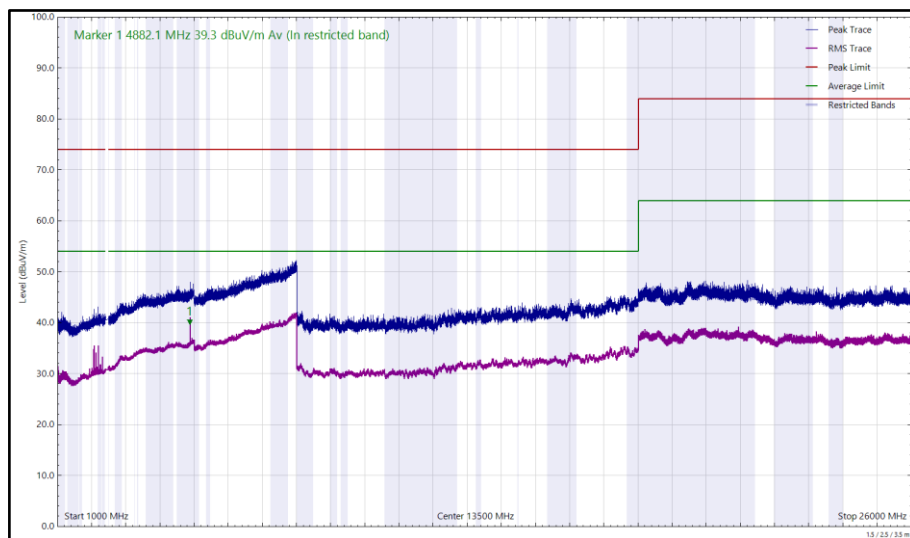
Figure 132 - 2441 MHz (CH39), DH5, iPA, Core 2, 1 GHz to 26 GHz, Horizontal
