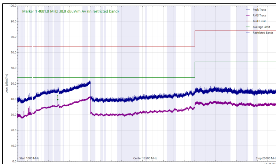
Figure 124 - 2441 MHz (CH39), DH5, iPA, Core 0 + Core 1, 1 GHz to 26 GHz, Horizontal
