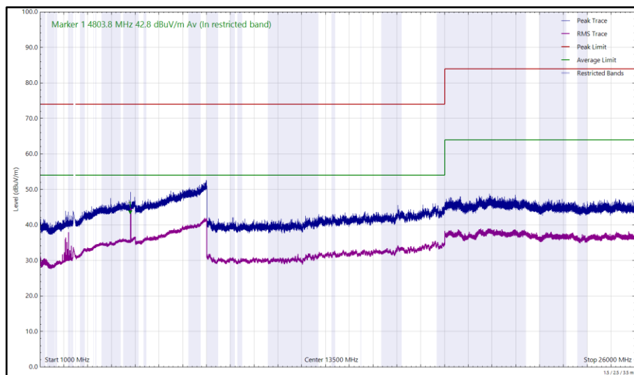
Figure 130 - 2402 MHz (CH0), DH5, iPA, Core 2, 1 GHz to 26 GHz, Vertical
