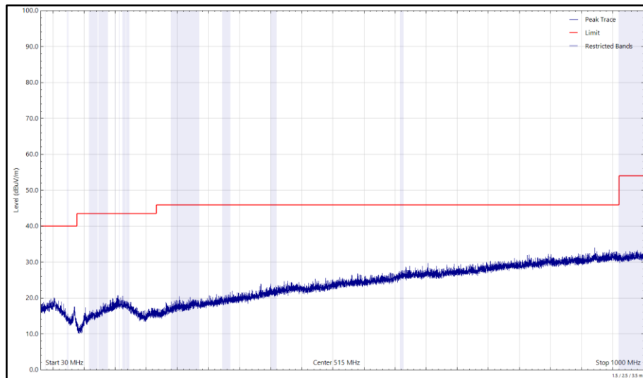
Figure 131 - 2441 MHz (CH39), DH5, iPA, Core 2, 30 MHz to 1 GHz, Horizontal (Peak)
