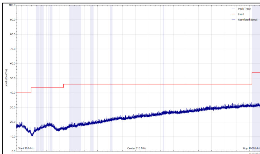
Figure 123 - 2441 MHz (CH39), DH5, iPA, Core 0 + Core 1, 30 MHz to 1 GHz, Horizontal (Peak)
