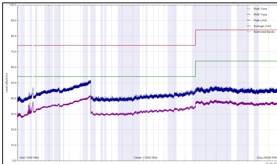
Figure 144 - 2480 MHz (CH78), 2DH5, ePA, Core 0 + Core 1, 1 GHz to 26 GHz, Vertical
