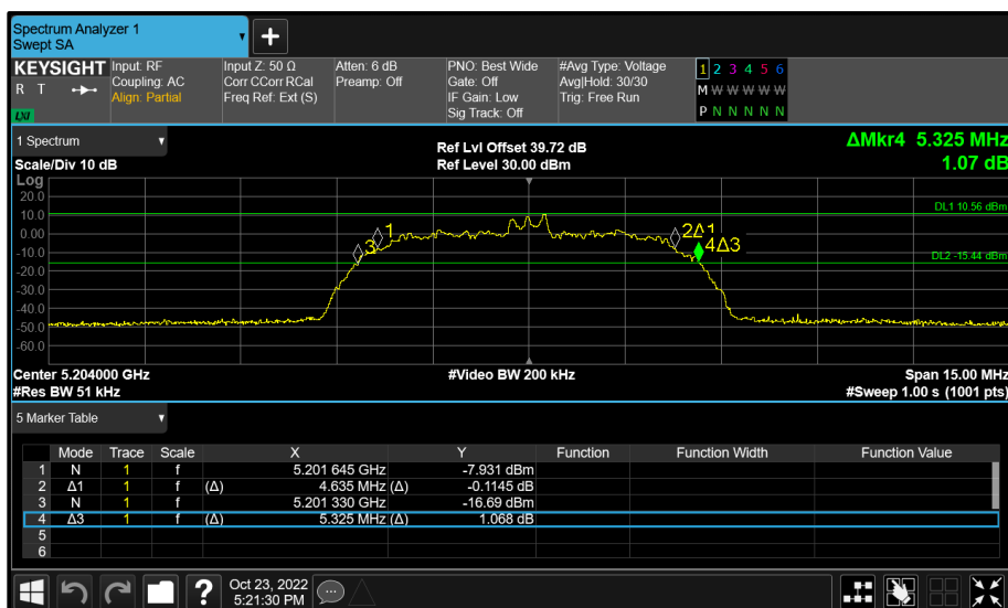
Figure 25 - Core 1 (B) 5204 MHz (CH54) 26 dB and 99% Bandwidth
