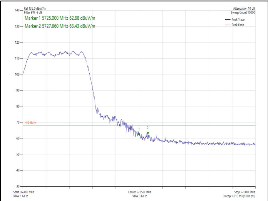
Figure 234 - 802.11n HT20 CDD, Cores 0-1 - 5700 MHz Band Edge Frequency 5725 MHz
