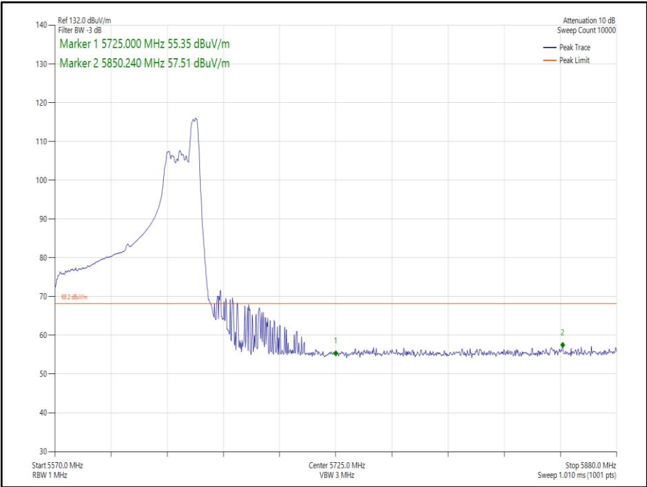
Figure 293 - 802.11ax HE80 Core 1 52-52 - 5610 MHz Band Edge Frequency 5725 MHz
