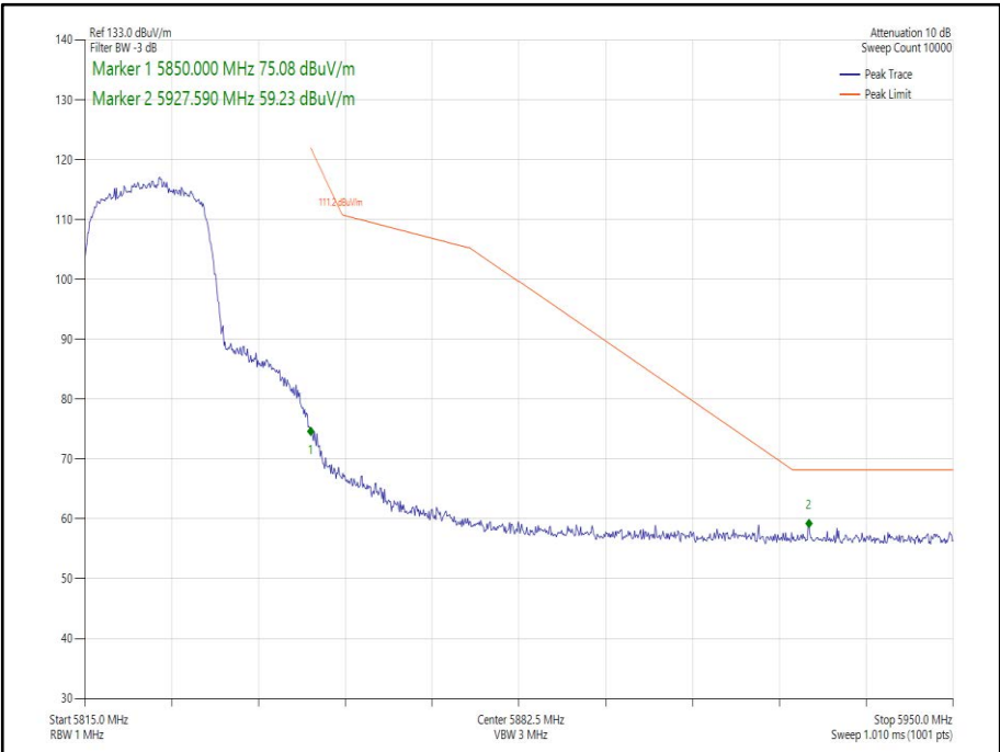
Figure 225 - 802.11n HT20, Core 1 - 5825 MHz Band Edge Frequency 5850 MHz
