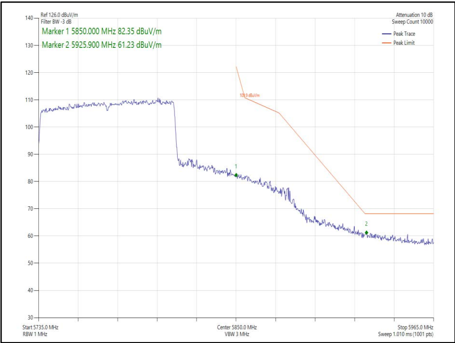
Figure 298 - 802.11ax HE80 Core 1 SU - 5775 MHz Band Edge Frequency 5850 MHz
