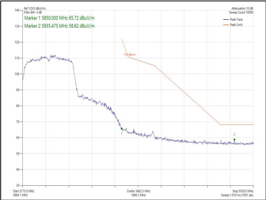
Figure 261 - 802.11n HT40, Core 1 - 5795 MHz Band Edge Frequency 5850 MHz
