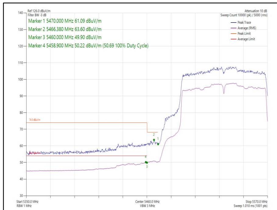
Figure 288 - 802.11ac VHT80 Core 1 - 5530 MHz Band Edge Frequency 5470 MHz
