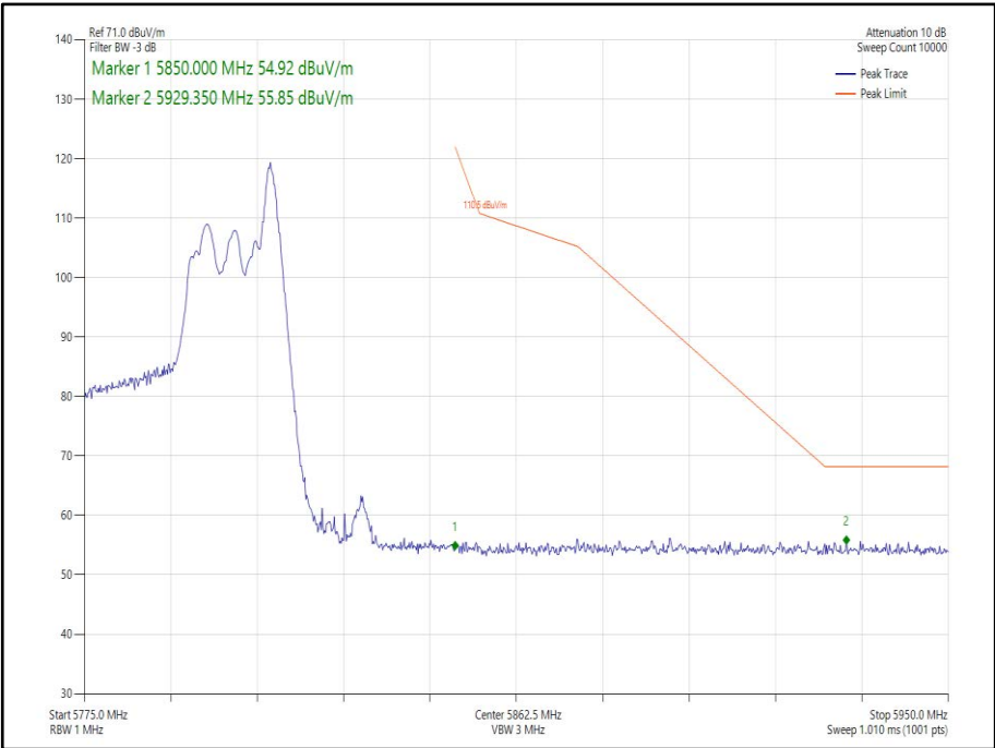
Figure 287 - 802.11ax HE40 SDM, Cores 0-1, 26-17 - 5795 MHz Band Edge Frequency 5850 MHz
