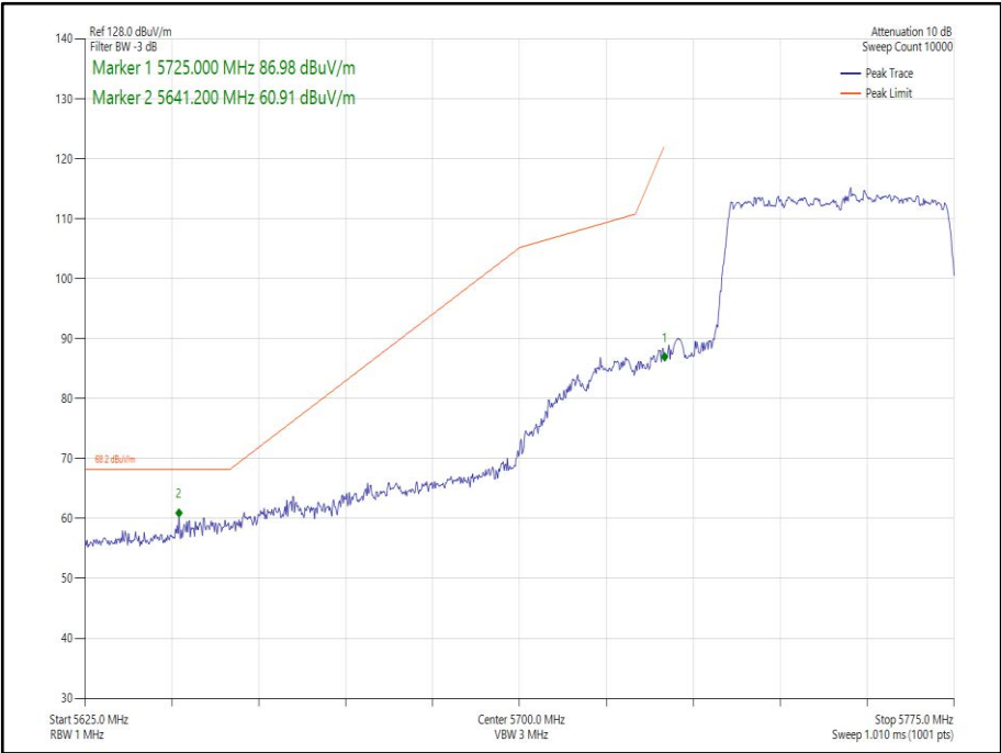
Figure 280 - 802.11ax HE40 SDM, Cores 0-1, SU - 5755 MHz Band Edge Frequency 5725 MHz
