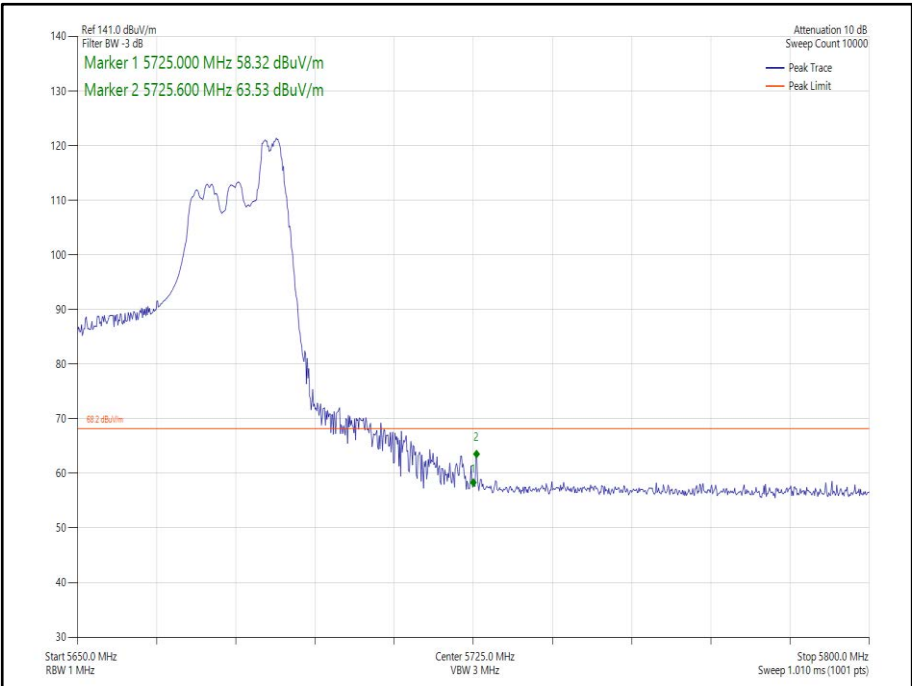
Figure 273 - 802.11ax HE40 CDD, Cores 0-1, 52-44 - 5670 MHz Band Edge Frequency 5725 MHz
