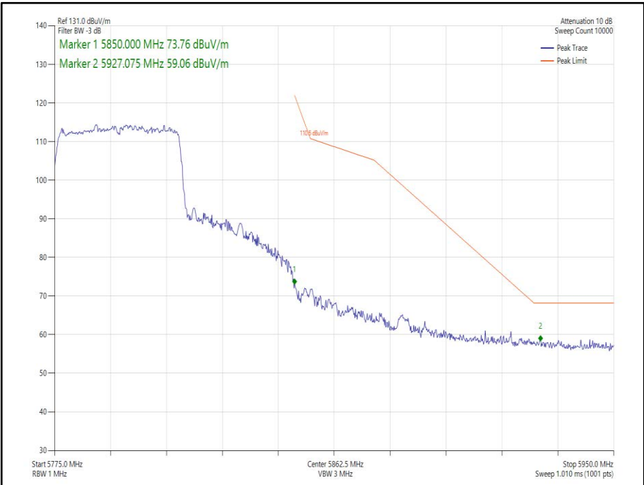
Figure 262 - 802.11ax HE40, Core 1, SU - 5795 MHz Band Edge Frequency 5850 MHz
