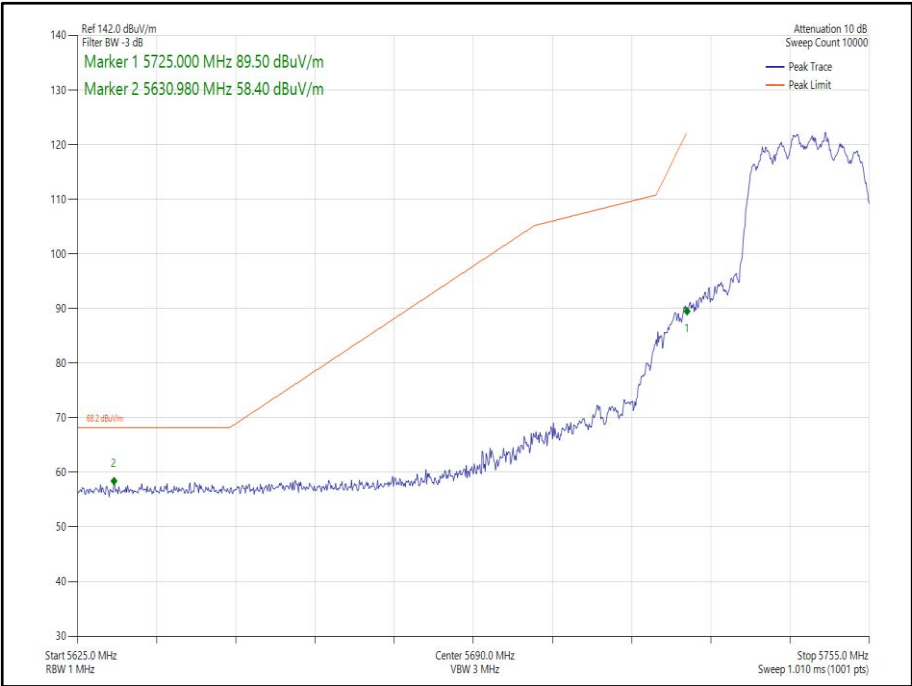
Figure 242 - 802.11ax HE20 CDD, Cores 0-1, SU - 5745 MHz Band Edge Frequency 5725 MHz
