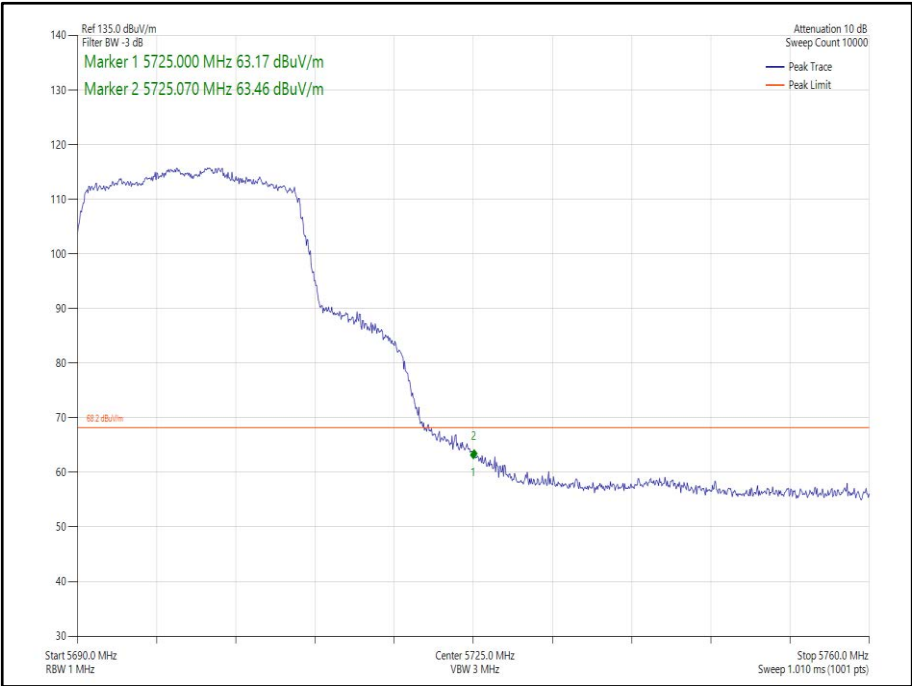
Figure 238 - 802.11ax HE20 SDM, Cores 0-1, SU - 5700 MHz Band Edge Frequency 5725 MHz
