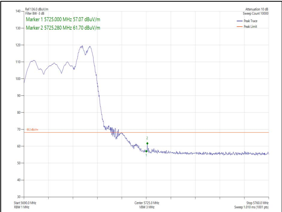
Figure 239 - 802.11ax HE20 SDM, Cores 0-1, 52-40 - 5700 MHz Band Edge Frequency 5725 MHz
