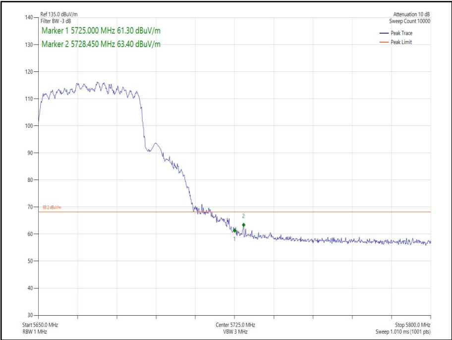
Figure 272 - 802.11ax HE40 CDD, Cores 0-1, SU - 5670 MHz Band Edge Frequency 5725 MHz
