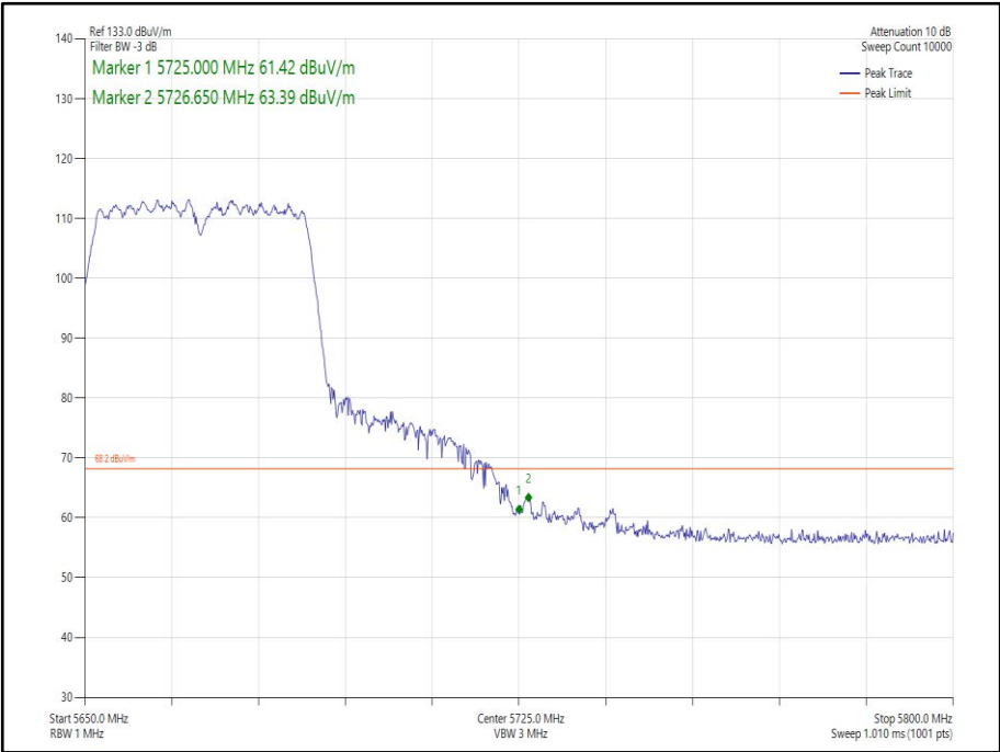
Figure 270 - 802.11n HT40 CDD, Cores 0-1 - 5670 MHz Band Edge Frequency 5725 MHz
