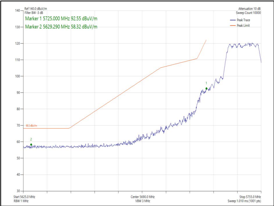
Figure 240 - 802.11n HT20 CDD, Cores 0-1 - 5745 MHz Band Edge Frequency 5725 MHz
