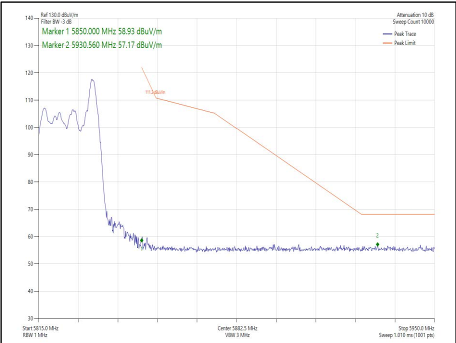
Figure 251 - 802.11ax HE20 SDM, Cores 0-1, 26-8 - 5825 MHz Band Edge Frequency 5850 MHz
