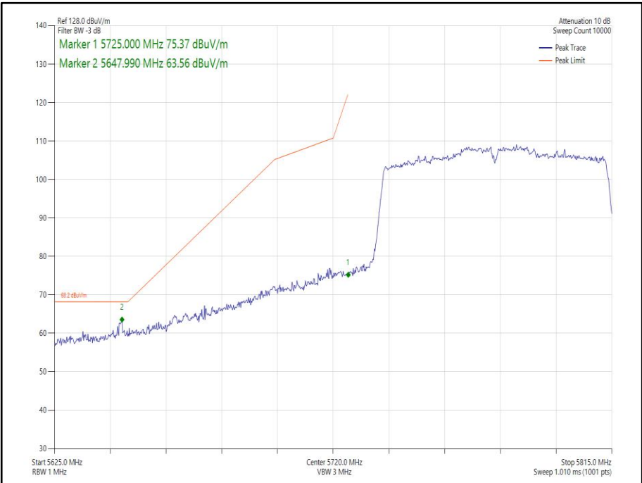
Figure 294 - 802.11ac VHT80 Core 1 - 5775 MHz Band Edge Frequency 5725 MHz
