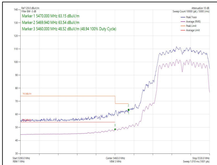
Figure 264 - 802.11n HT40 CDD, Cores 0-1 - 5510 MHz Band Edge Frequency 5470 MHz
