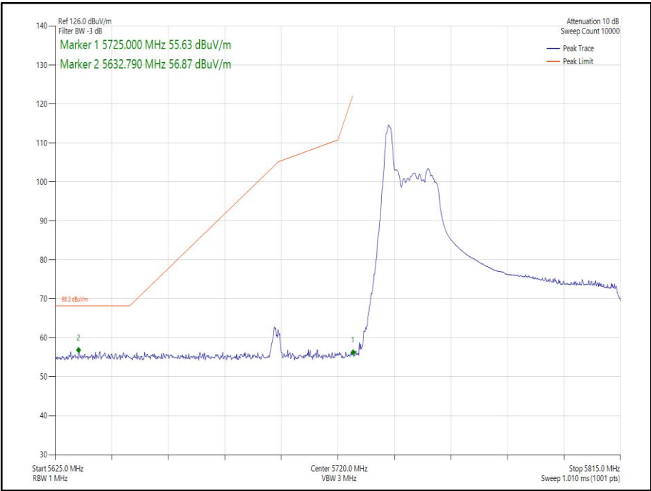
Figure 296 - 802.11ax HE80 Core 1 26-0 - 5775 MHz Band Edge Frequency 5725 MHz
