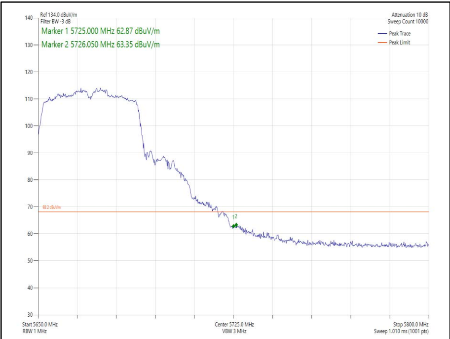
Figure 271 - 802.11n HT40 SDM, Cores 0-1 - 5670 MHz Band Edge Frequency 5725 MHz
