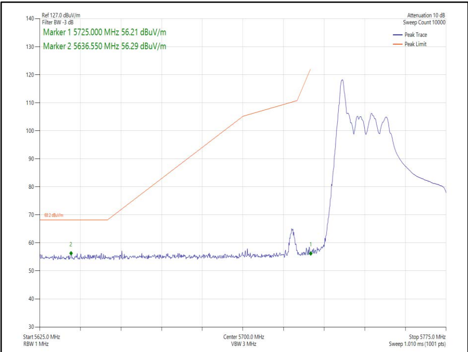
Figure 281 - 802.11ax HE40 SDM, Cores 0-1, 26-0 - 5755 MHz Band Edge Frequency 5725 MHz
