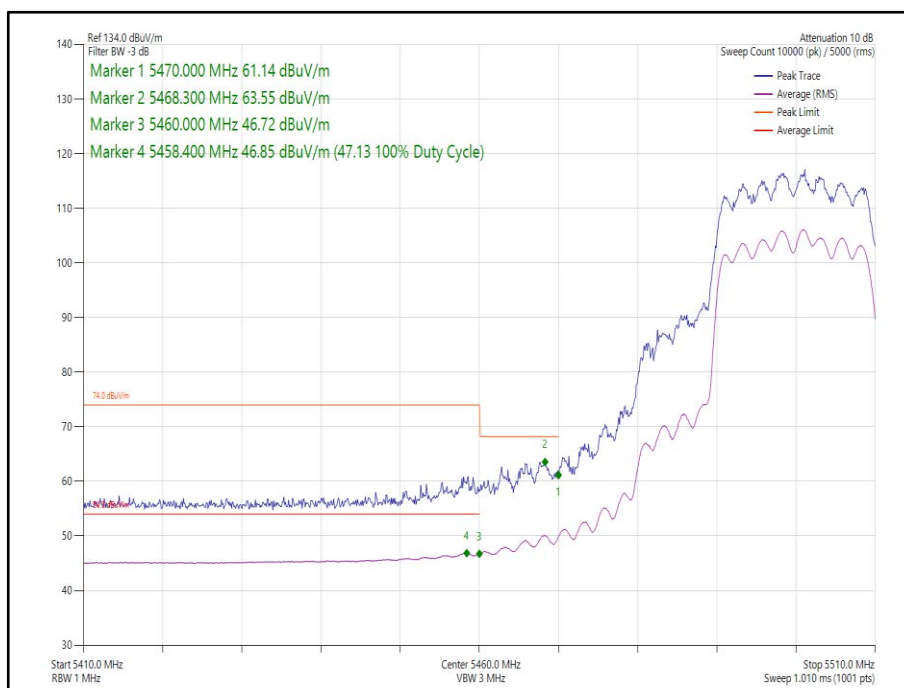
Figure 230 - 802.11ax HE20 CDD, Cores 0-1, SU - 5500 MHz Band Edge Frequency 5470 MHz
