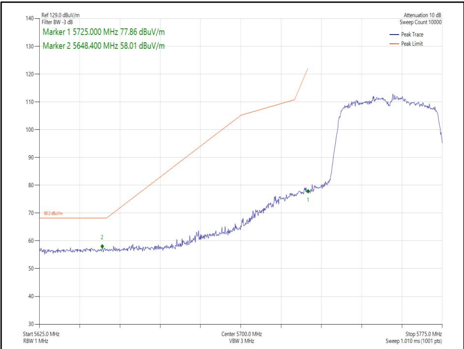
Figure 258 - 802.11n HT40, Core 1 - 5755 MHz Band Edge Frequency 5725 MHz
