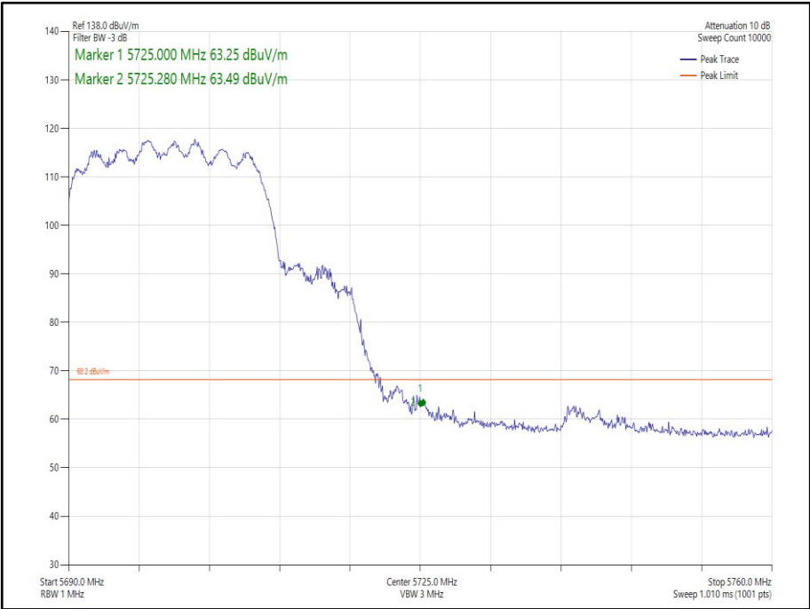
Figure 236 - 802.11ax HE20 CDD, Cores 0-1, SU - 5700 MHz Band Edge Frequency 5725 MHz
