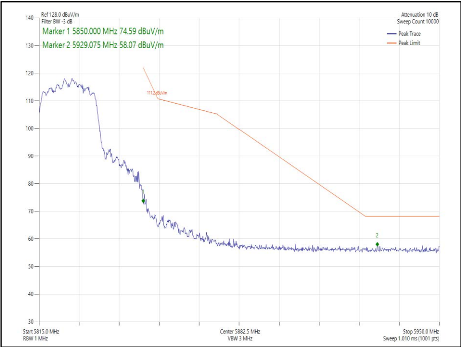
Figure 246 - 802.11n HT20 CDD, Cores 0-1 - 5825 MHz Band Edge Frequency 5850 MHz
