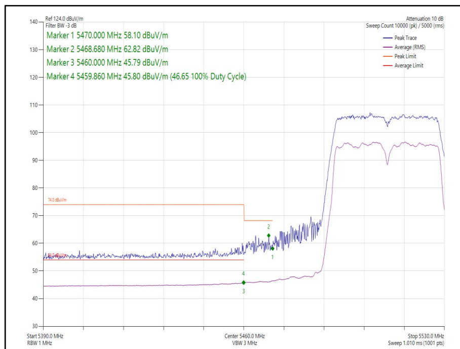
Figure 265 - 802.11n HT40 SDM, Cores 0-1 - 5510 MHz Band Edge Frequency 5470 MHz
