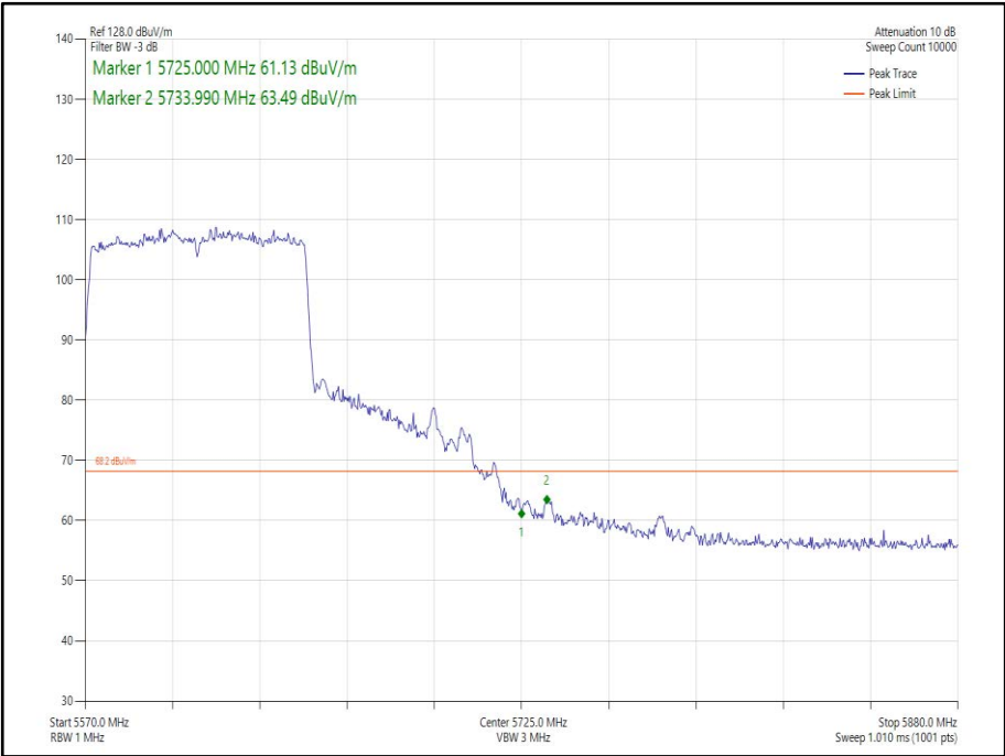
Figure 291 - 802.11ac VHT80 Core 1 - 5610 MHz Band Edge Frequency 5725 MHz
