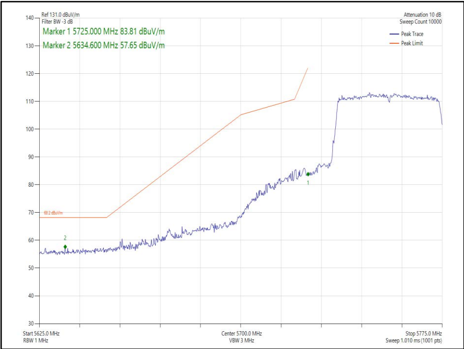
Figure 259 - 802.11ax HE40, Core 1, SU - 5755 MHz Band Edge Frequency 5725 MHz
