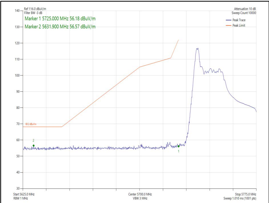
Figure 260 - 802.11ax HE40, Core 1, 26-0 - 5755 MHz Band Edge Frequency 5725 MHz
