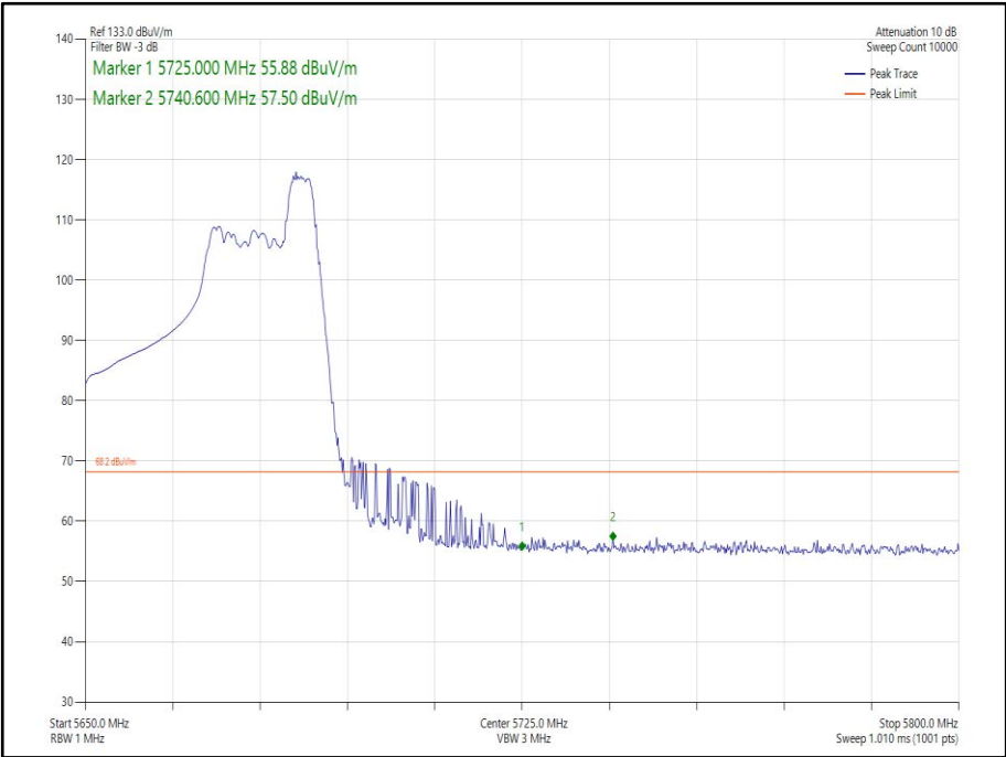
Figure 257 - 802.11ax HE40, Core 1, 52-44 - 5670 MHz Band Edge Frequency 5725 MHz
