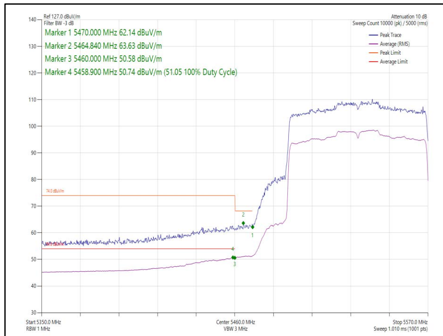
Figure 289 - 802.11ax HE80 Core 1 SU - 5530 MHz Band Edge Frequency 5470 MHz
