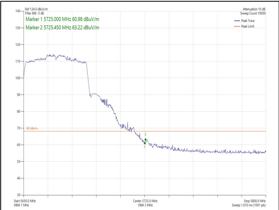
Figure 256 - 802.11ax HE40, Core 1, SU - 5670 MHz Band Edge Frequency 5725 MHz
