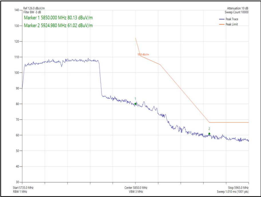
Figure 297 - 802.11ac VHT80 Core 1 - 5775 MHz Band Edge Frequency 5850 MHz
