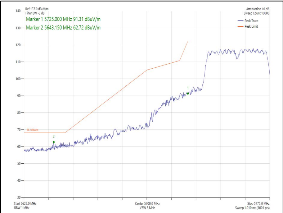
Figure 276 - 802.11n HT40 CDD, Cores 0-1 - 5755 MHz Band Edge Frequency 5725 MHz
