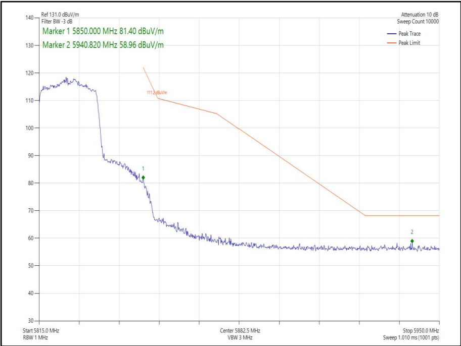
Figure 250 - 802.11ax HE20 SDM, Cores 0-1, SU - 5825 MHz Band Edge Frequency 5850 MHz
