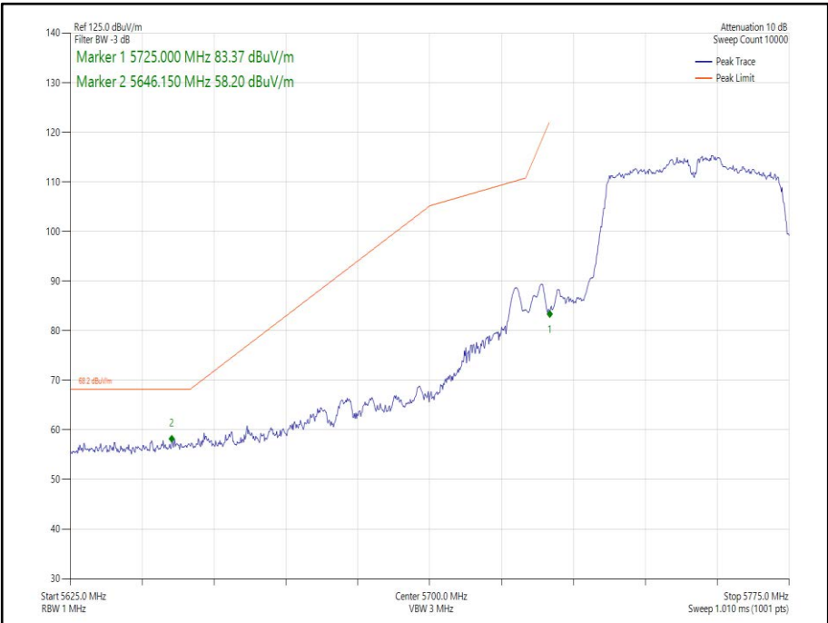
Figure 277 - 802.11n HT40 SDM, Cores 0-1 - 5755 MHz Band Edge Frequency 5725 MHz
