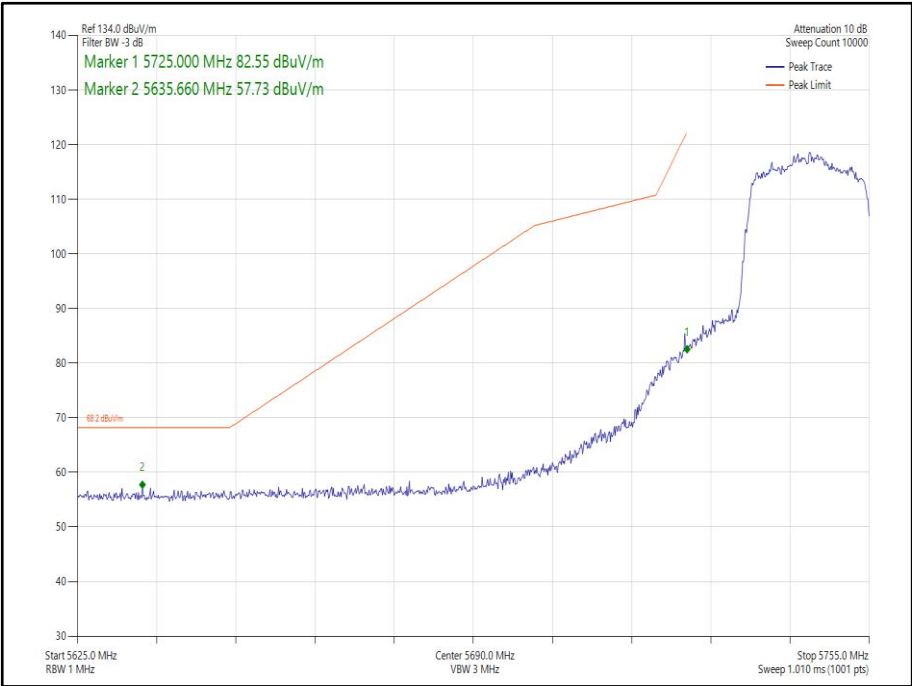
Figure 244 - 802.11ax HE20 SDM, Cores 0-1, SU - 5745 MHz Band Edge Frequency 5725 MHz
