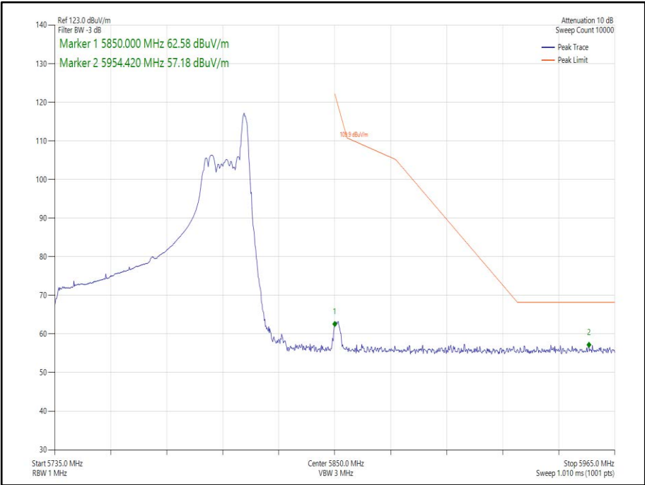
Figure 299 - 802.11ax HE80 Core 1 26-36 - 5775 MHz Band Edge Frequency 5850 MHz
