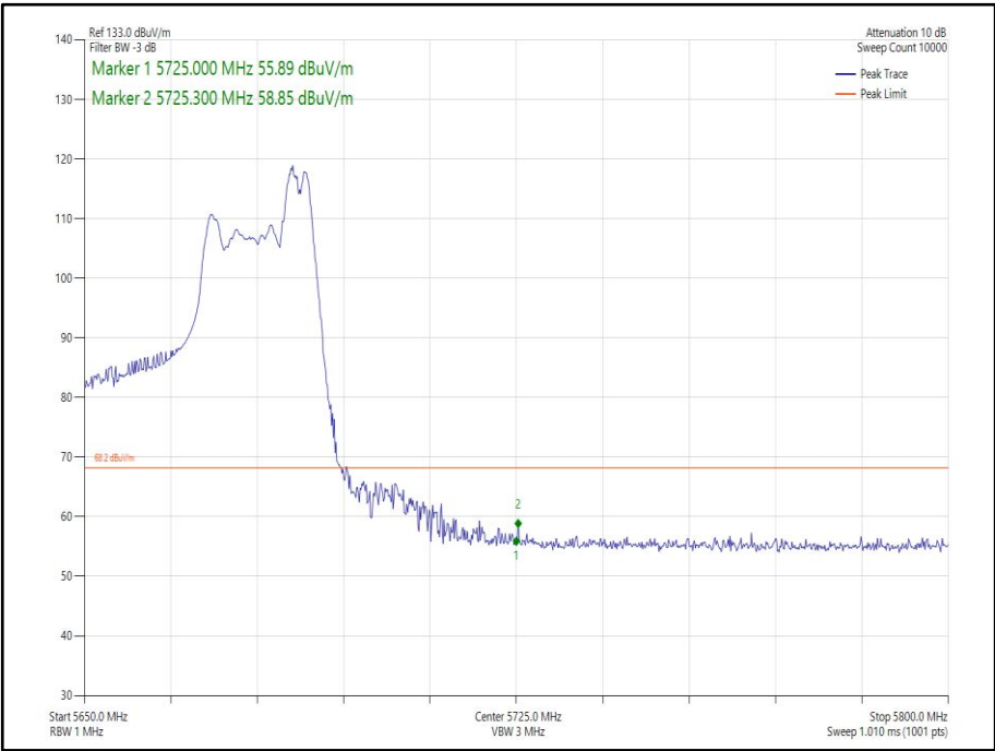
Figure 275 - 802.11ax HE40 SDM, Cores 0-1, 52-44 - 5670 MHz Band Edge Frequency 5725 MHz
