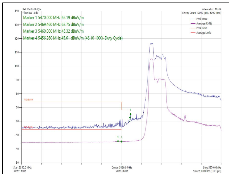
Figure 290 - 802.11ax HE80 Core 1 52-37- 5530 MHz Band Edge Frequency 5470 MHz
