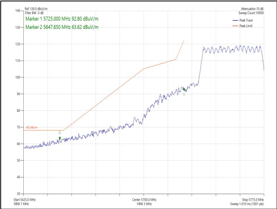
Figure 278 - 802.11ax HE40 CDD, Cores 0-1, SU - 5755 MHz Band Edge Frequency 5725 MHz
