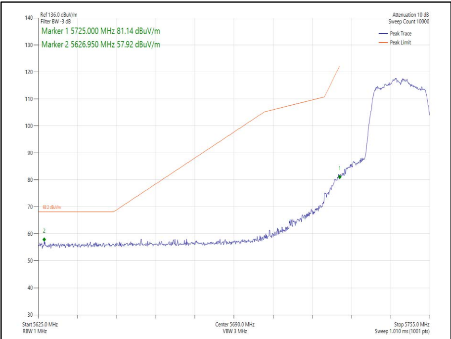
Figure 241 - 802.11n HT20 SDM, Cores 0-1 - 5745 MHz Band Edge Frequency 5725 MHz
