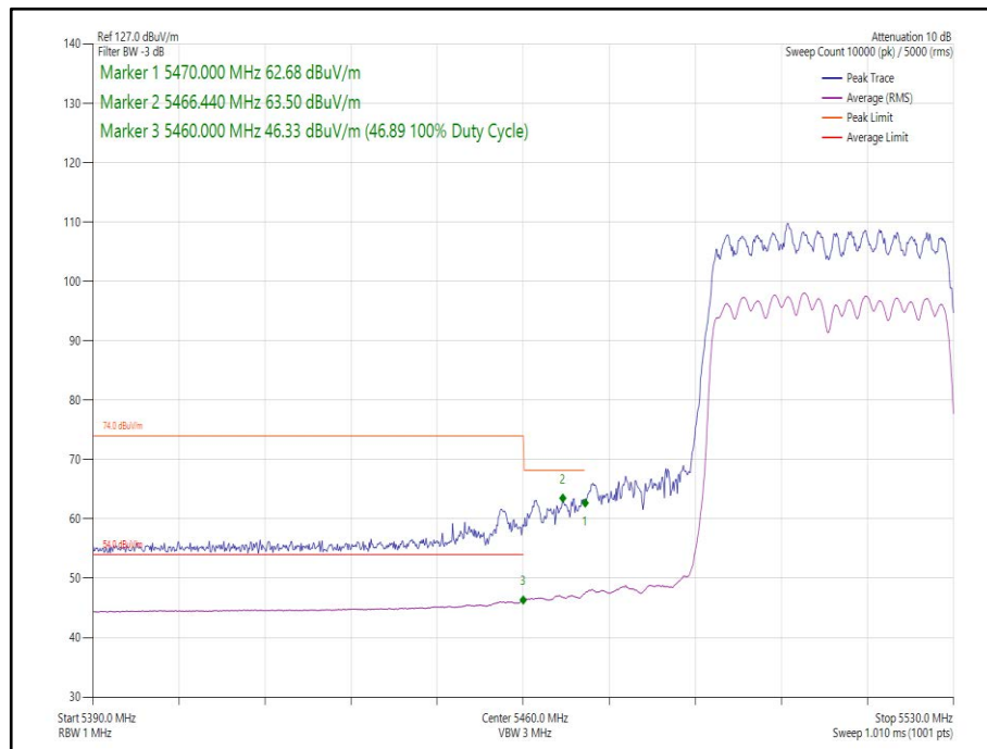
Figure 266 - 802.11ax HE40 CDD, Cores 0-1, SU - 5510 MHz Band Edge Frequency 5470 MHz
