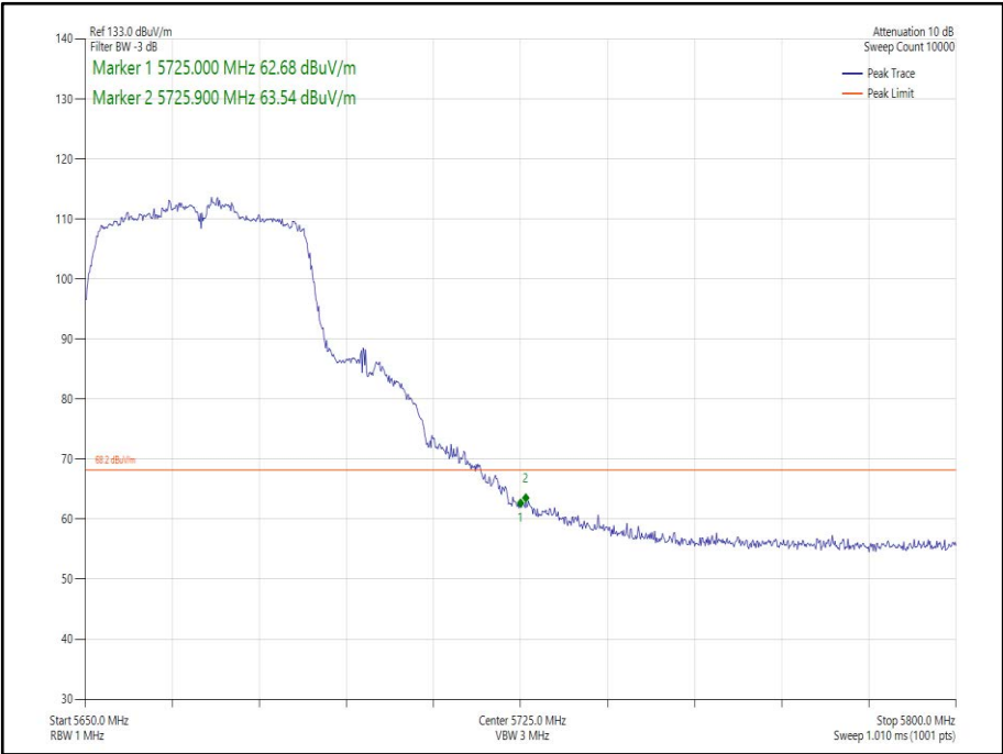
Figure 255 - 802.11n HT40, Core 1 - 5670 MHz Band Edge Frequency 5725 MHz
