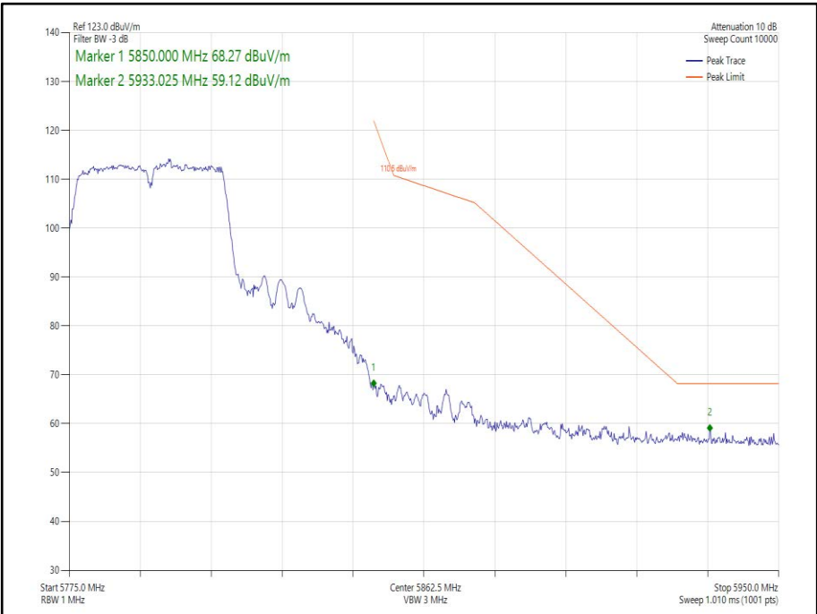
Figure 283 - 802.11n HT40 SDM, Cores 0-1 - 5795 MHz Band Edge Frequency 5850 MHz
