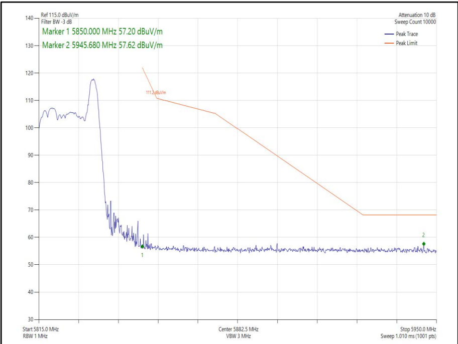
Figure 227 - 802.11ax HE20, Core 1, 26-8 - 5825 MHz Band Edge Frequency 5850 MHz
