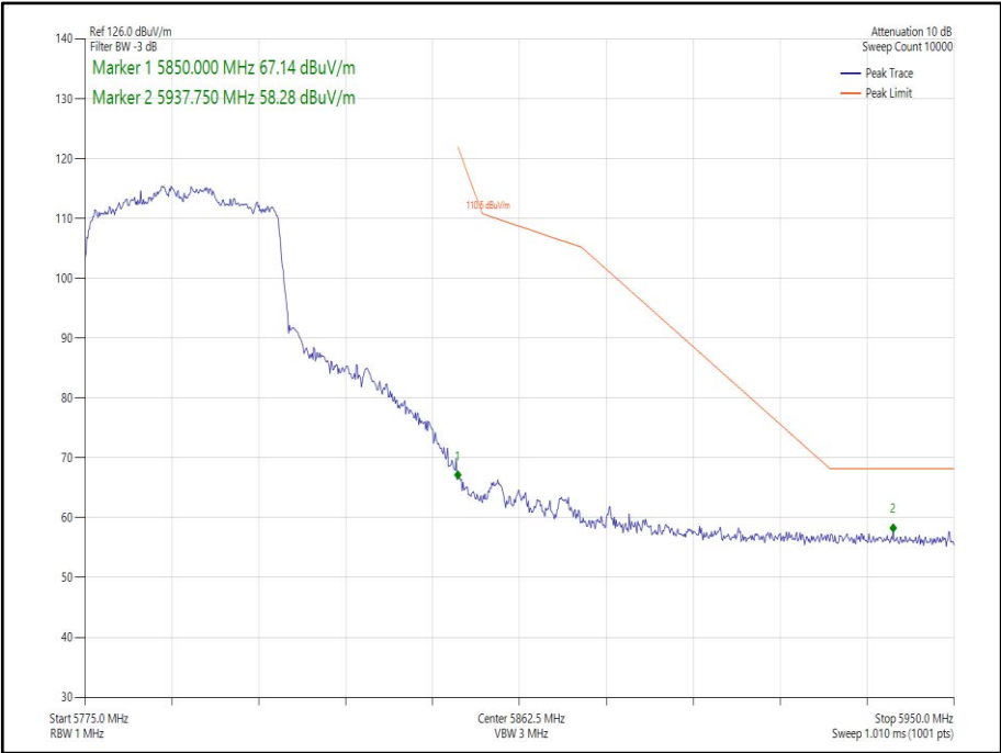
Figure 286 - 802.11ax HE40 SDM, Cores 0-1, SU - 5795 MHz Band Edge Frequency 5850 MHz
