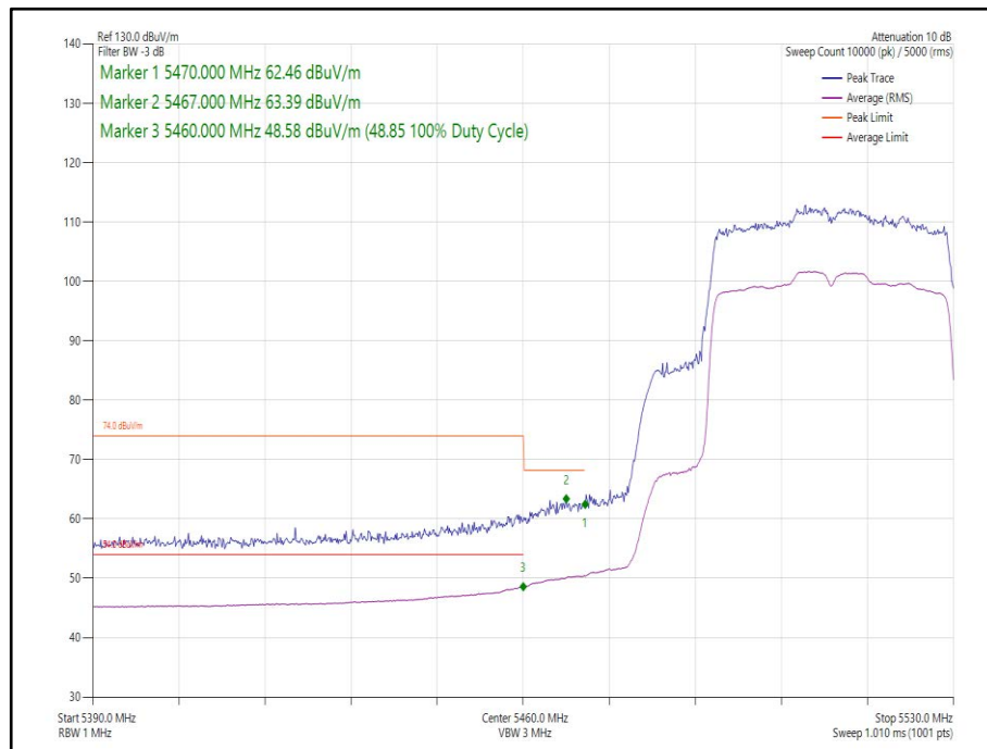
Figure 253 - 802.11ax HE40, Core 1, SU - 5510 MHz Band Edge Frequency 5470 MHz
