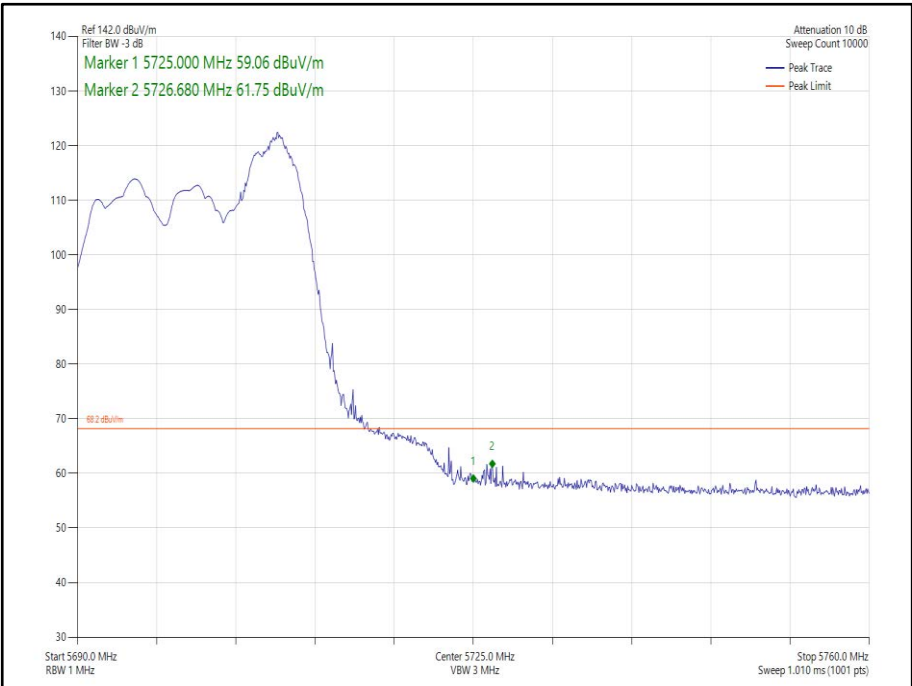
Figure 237 - 802.11ax HE20 CDD, Cores 0-1, 52-40 - 5700 MHz Band Edge Frequency 5725 MHz
