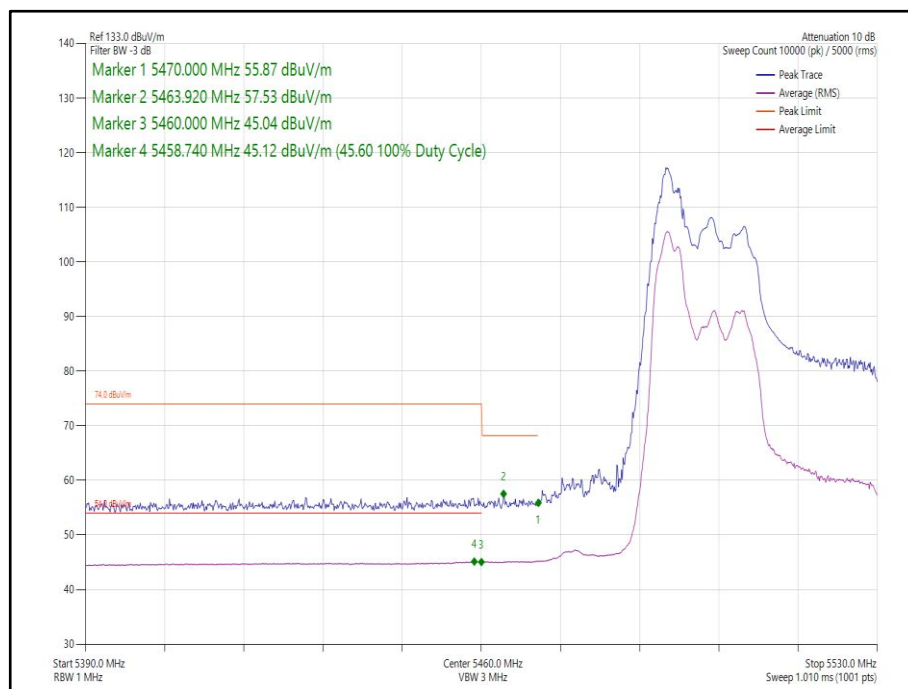
Figure 269 - 802.11ax HE40 SDM, Cores 0-1, 52-37 - 5510 MHz Band Edge Frequency 5470 MHz
