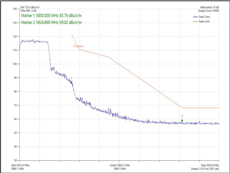
Figure 226 - 802.11ax HE20, Core 1, SU - 5825 MHz Band Edge Frequency 5850 MHz
