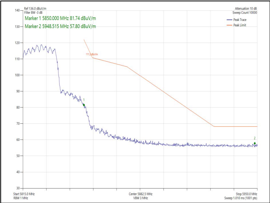
Figure 248 - 802.11ax HE20 CDD, Cores 0-1, SU - 5825 MHz Band Edge Frequency 5850 MHz
