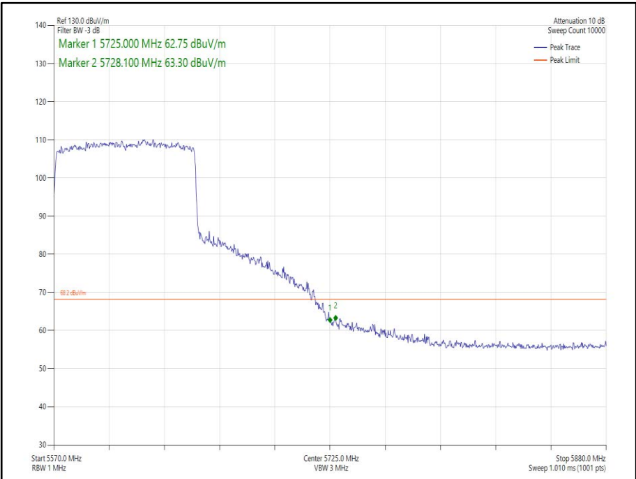
Figure 292 - 802.11ax HE80 Core 1 SU - 5610 MHz Band Edge Frequency 5725 MHz
