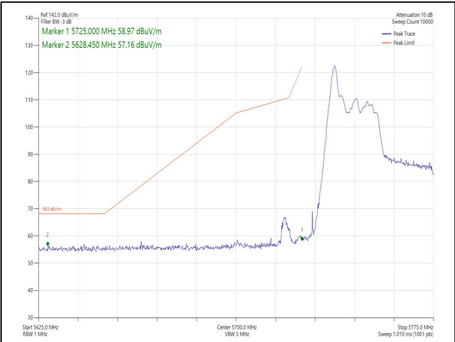
Figure 279 - 802.11ax HE40 CDD, Cores 0-1, 26-0 - 5755 MHz Band Edge Frequency 5725 MHz
