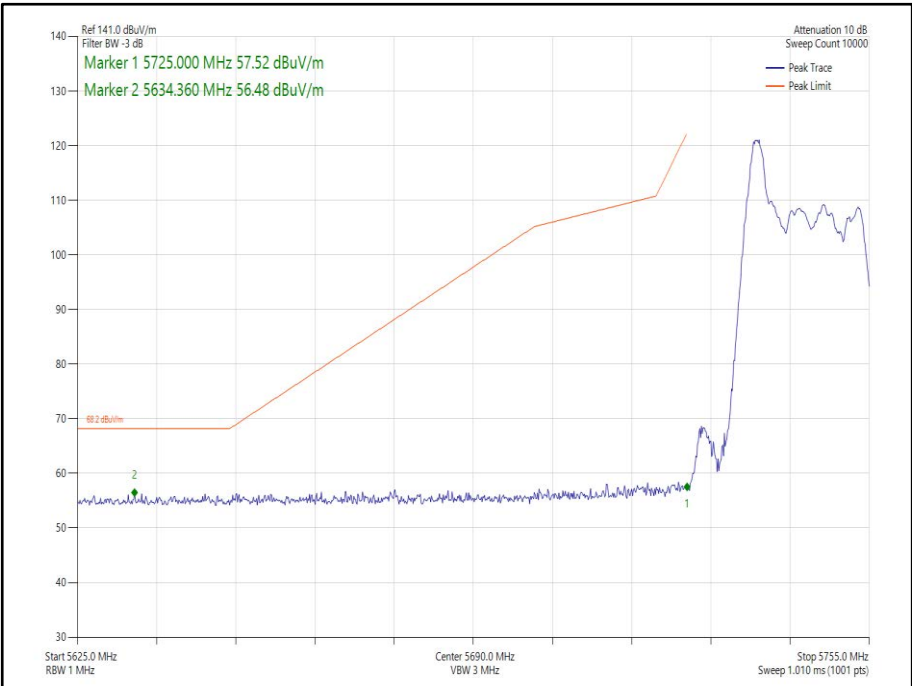
Figure 243 - 802.11ax HE20 CDD, Cores 0-1, 26-0 - 5745 MHz Band Edge Frequency 5725 MHz
