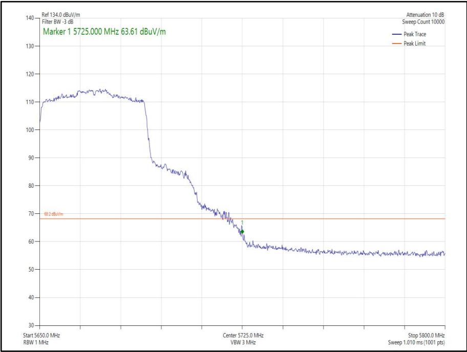
Figure 274 - 802.11ax HE40 SDM, Cores 0-1, SU - 5670 MHz Band Edge Frequency 5725 MHz
