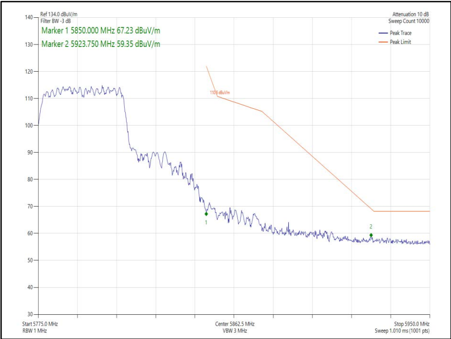
Figure 282 - 802.11n HT40 CDD, Cores 0-1 - 5795 MHz Band Edge Frequency 5850 MHz
