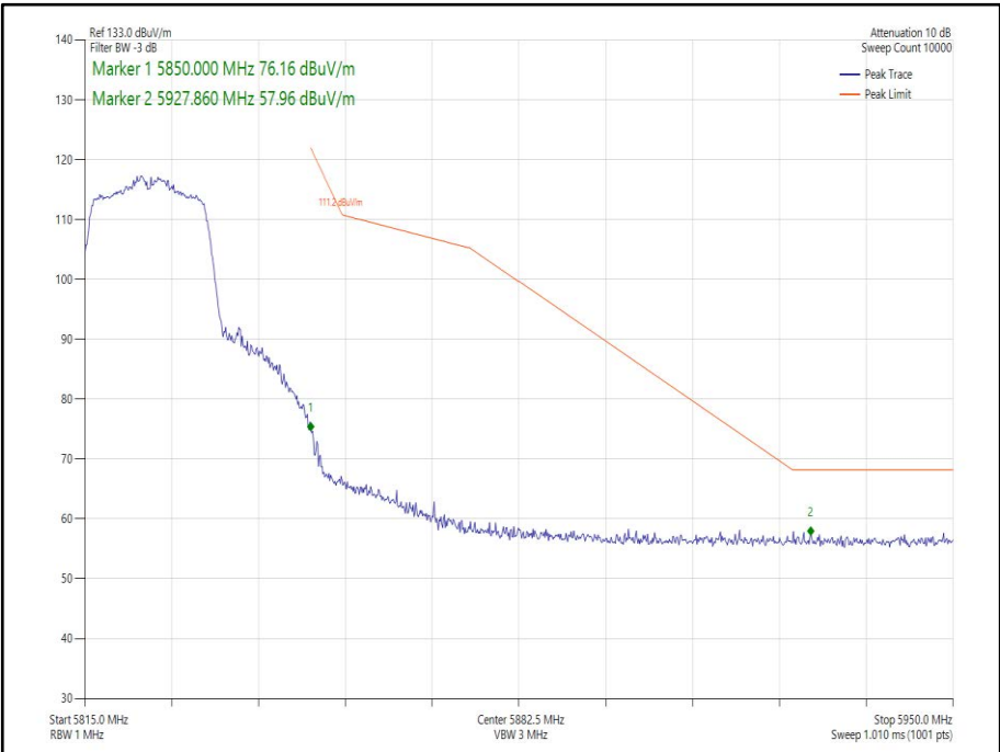
Figure 247 - 802.11n HT20 SDM, Cores 0-1 - 5825 MHz Band Edge Frequency 5850 MHz
