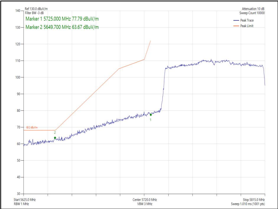
Figure 295 - 802.11ax HE80 Core 1 SU - 5775 MHz Band Edge Frequency 5725 MHz
