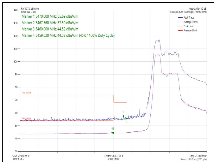
Figure 254 - 802.11ax HE40, Core 1, 52-37 - 5510 MHz Band Edge Frequency 5470 MHz
