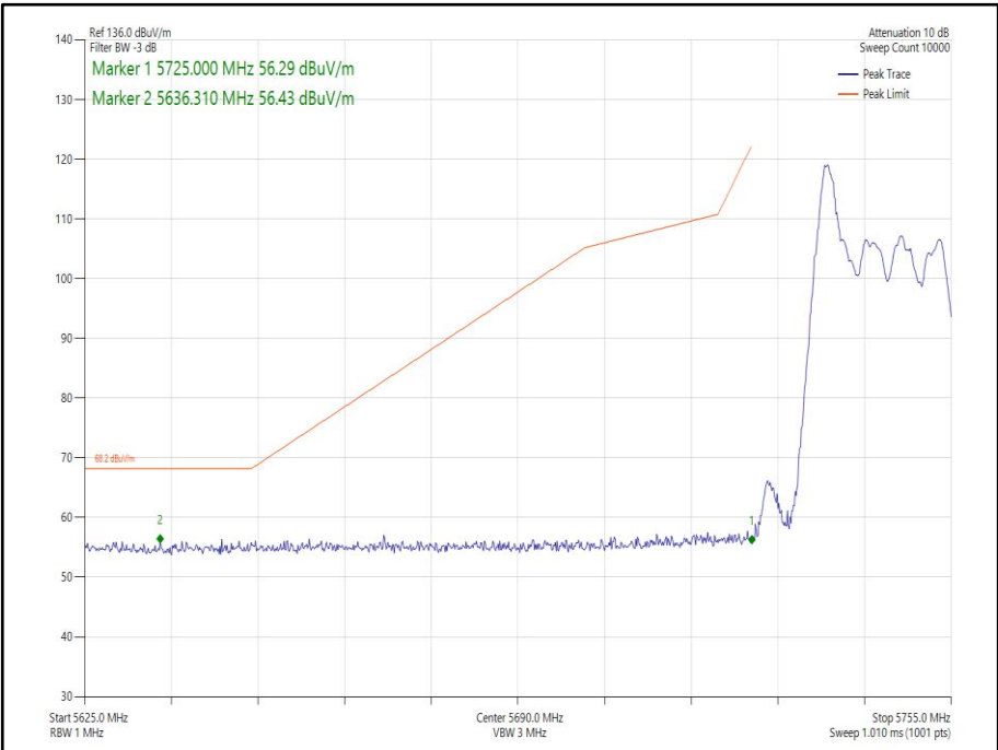
Figure 245 - 802.11ax HE20 SDM, Cores 0-1, 26-0 - 5745 MHz Band Edge Frequency 5725 MHz
