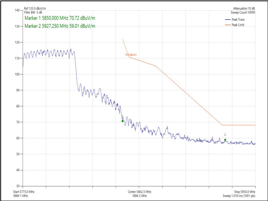
Figure 284 - 802.11ax HE40 CDD, Cores 0-1, SU - 5795 MHz Band Edge Frequency 5850 MHz
