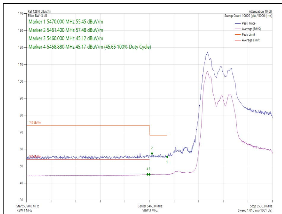
Figure 267 - 802.11ax HE40 CDD, Cores 0-1, 52-37 - 5510 MHz Band Edge Frequency 5470 MHz
