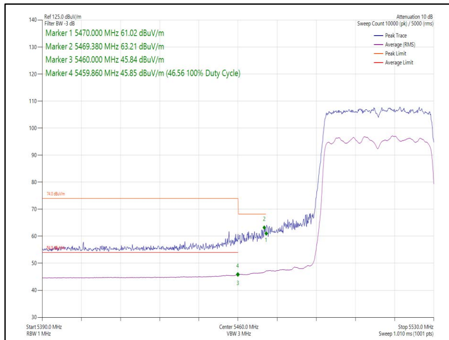
Figure 268 - 802.11ax HE40 SDM, Cores 0-1, SU - 5510 MHz Band Edge Frequency 5470 MHz
