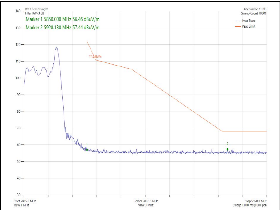
Figure 249 - 802.11ax HE20 CDD, Cores 0-1, 26-8 - 5825 MHz Band Edge Frequency 5850 MHz
