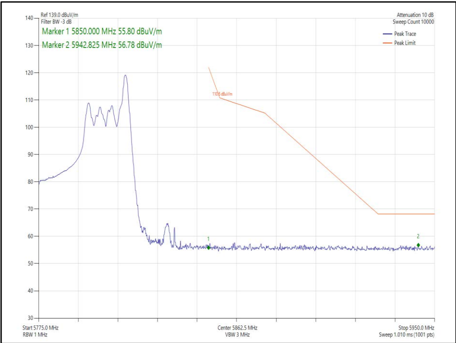
Figure 285 - 802.11ax HE40 CDD, Cores 0-1, 26-17 - 5795 MHz Band Edge Frequency 5850 MHz
