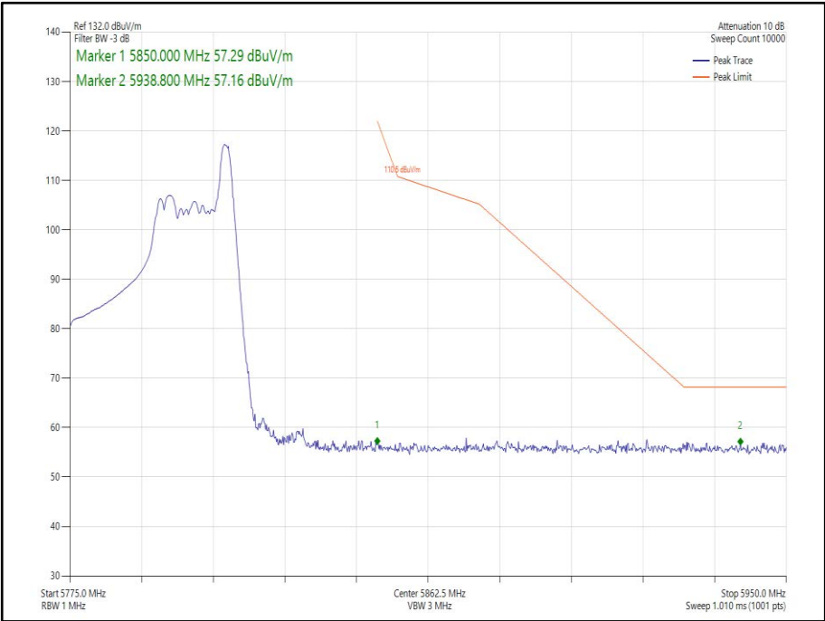
Figure 263 - 802.11ax HE40, Core 1, 26-17 - 5795 MHz Band Edge Frequency 5850 MHz
