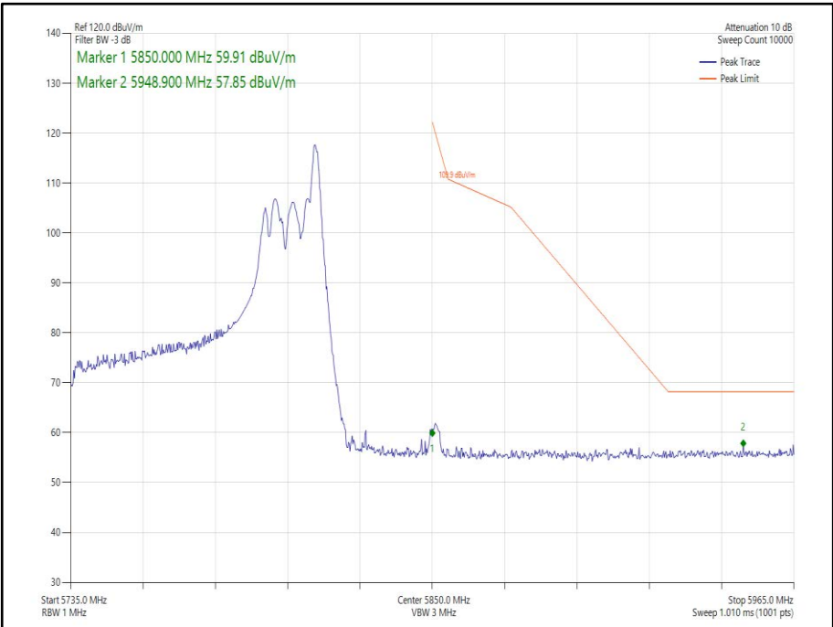
Figure 321 - 802.11ax HE80 CDD, Cores 0-1, 2d 6-36 - 5775 MHz Band Edge Frequency 5850 MHz
