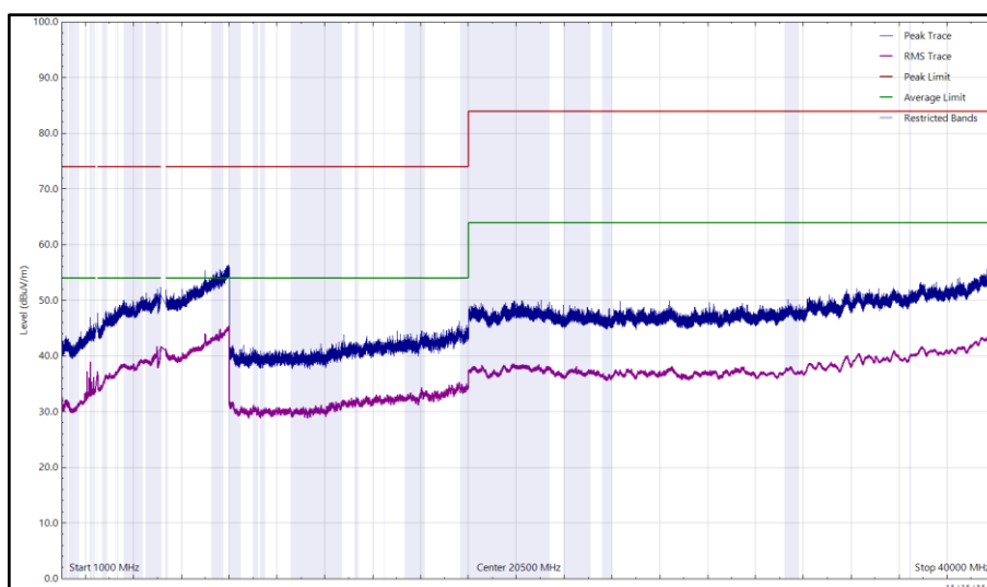
Figure 35 - U-NII-1 - 5200 MHz (CH40), VHT20, CDD, Core 0 + Core 1 and 2480 MHz (CH78), 2-DH5, ePA, Core 0 + Core 1, 1 GHz to 40 GHz, Horizontal
