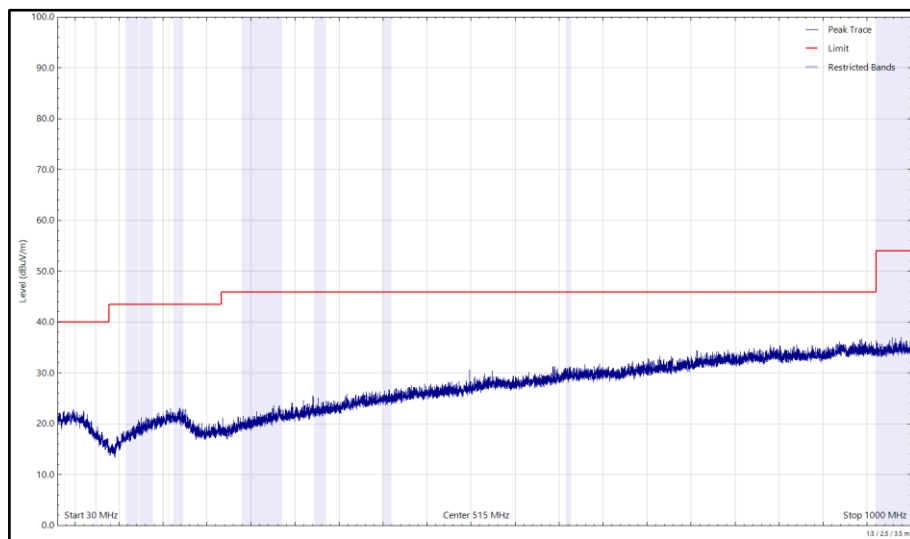
Figure 42 - U-NII-5 – 5955 MHz (CH1), HE20, SU, CDD, Core 0 + Core 1 and 2402 MHz (CH0), 2-DH5, ePA, Core 0 + Core 1, 30 MHz to 1 GHz, Horizontal (Peak)
