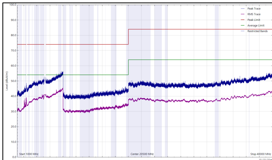
Figure 27 - U-NII-1 - 5200 MHz (CH40), VHT20, CDD, Core 0 + Core 1 and 2402 MHz (CH0), 2-DH5, ePA, Core 0 + Core 1, 1 GHz to 40 GHz, Horizontal
