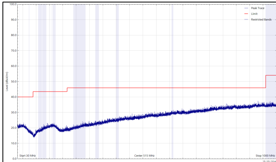
Figure 38 - U-NII-2C - 5680 MHz (CH136), VHT20, CDD, Core 0 + Core 1 and 2402 MHz (CH0), 2-DH5, ePA, Core 0 + Core 1, 30 MHz to 1 GHz, Horizontal (Peak)
