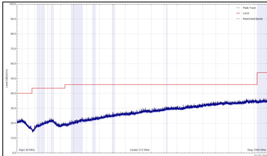
Figure 26 - U-NII-1 - 5200 MHz (CH40), VHT20, CDD, Core 0 + Core 1 and 2402 MHz (CH0), 2-DH5, ePA, Core 0 + Core 1, 30 MHz to 1 GHz, Horizontal (Peak)
