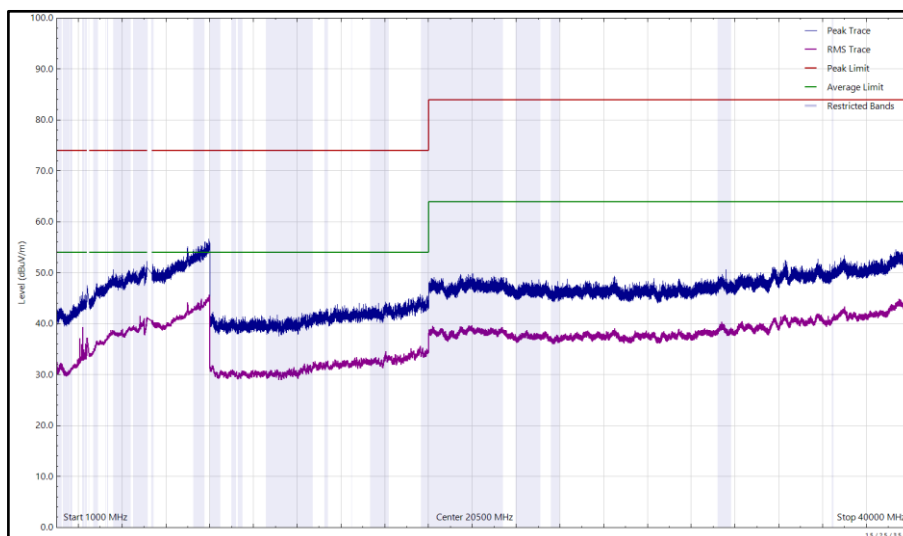
Figure 3 - U-NII-1 - 5200 MHz (CH40), VHT20, CDD, Core 0 + Core 1 and 2402 MHz (CH0), 2-DH5, ePA, Core 0, 1 GHz to 40 GHz, Horizontal
