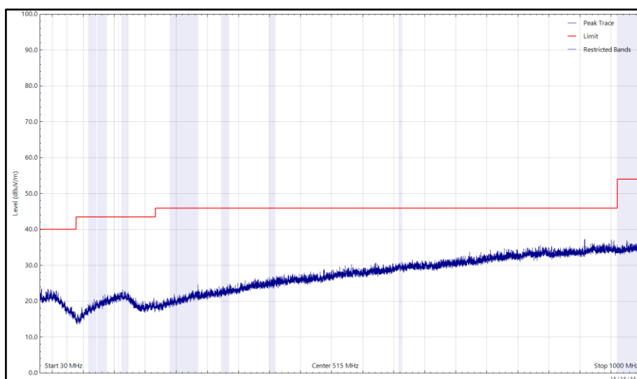
Figure 2 - U-NII-1 - 5200 MHz (CH40), VHT20, CDD, Core 0 + Core 1 and 2402 MHz (CH0), 2-DH5, ePA, Core 0, 30 MHz to 1 GHz, Horizontal (Peak)
