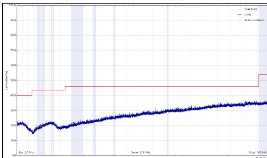
Figure 34 - U-NII-1 - 5200 MHz (CH40), VHT20, CDD, Core 0 + Core 1 and 2480 MHz (CH78), 2-DH5, ePA, Core 0 + Core 1, 30 MHz to 1 GHz, Horizontal (Peak)
