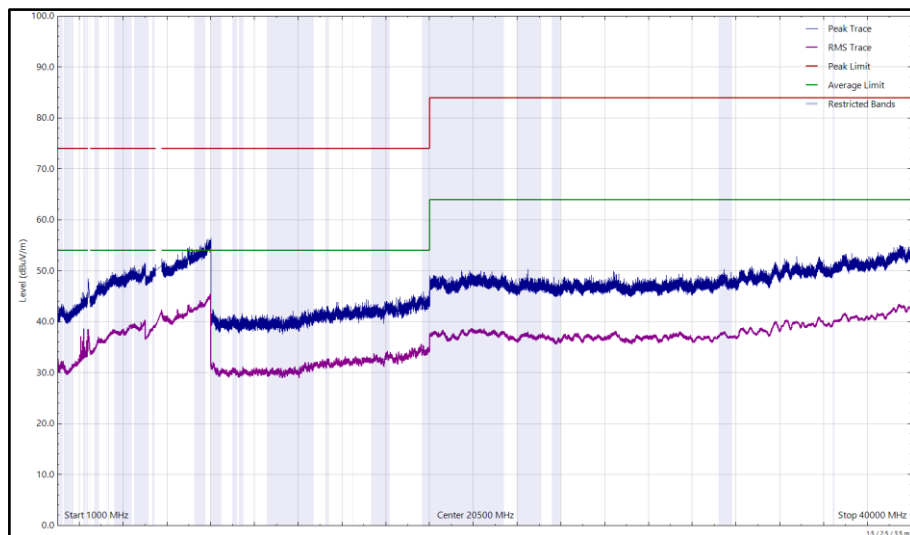
Figure 39 - U-NII-2C - 5680 MHz (CH136), VHT20, CDD, Core 0 + Core 1 and 2402 MHz (CH0), 2-DH5, ePA, Core 0 + Core 1, 1 GHz to 40 GHz, Horizontal
