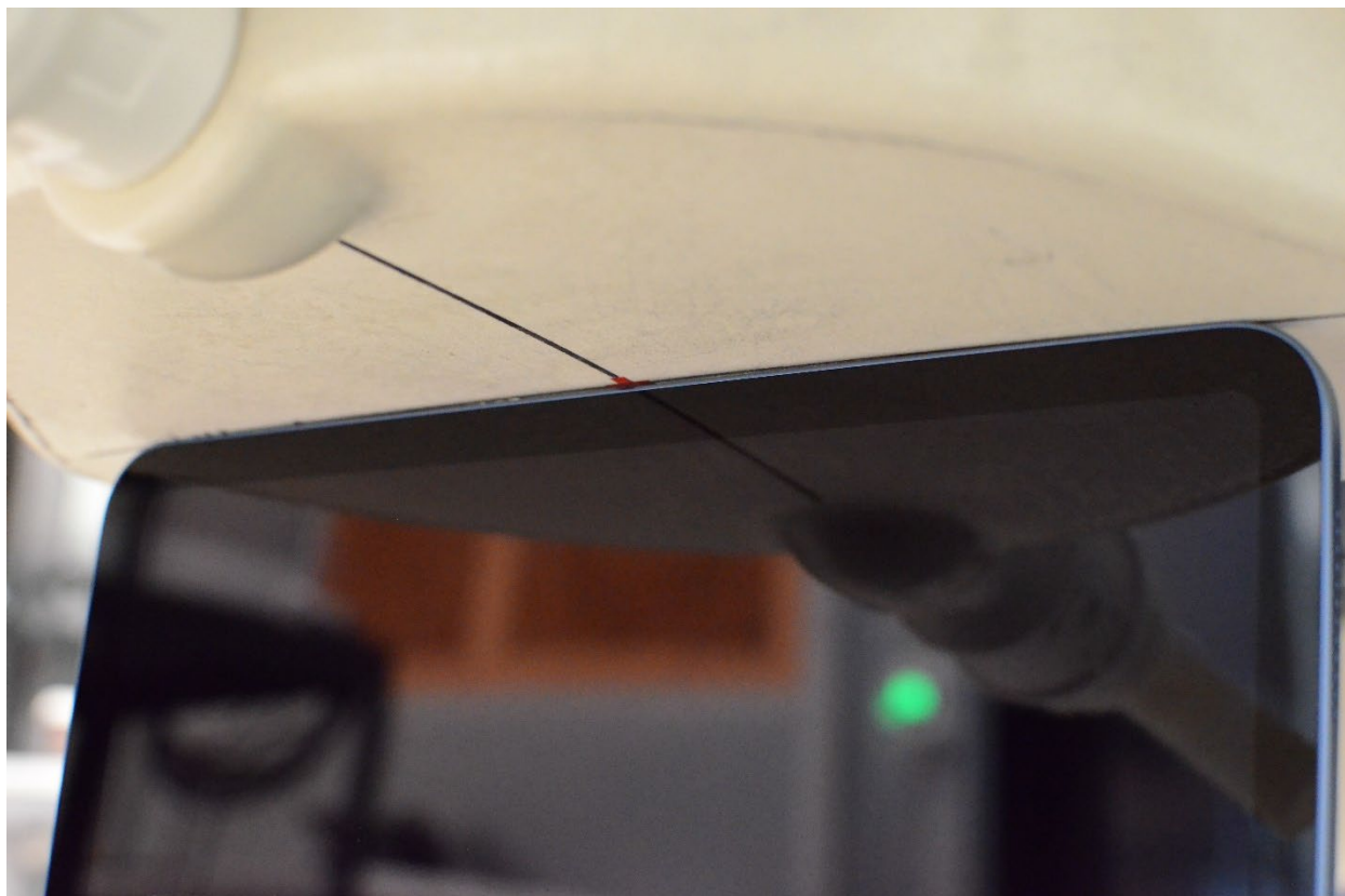
SAR Test Setup Photo 5: Body, Left Edge at 0.0 cm
