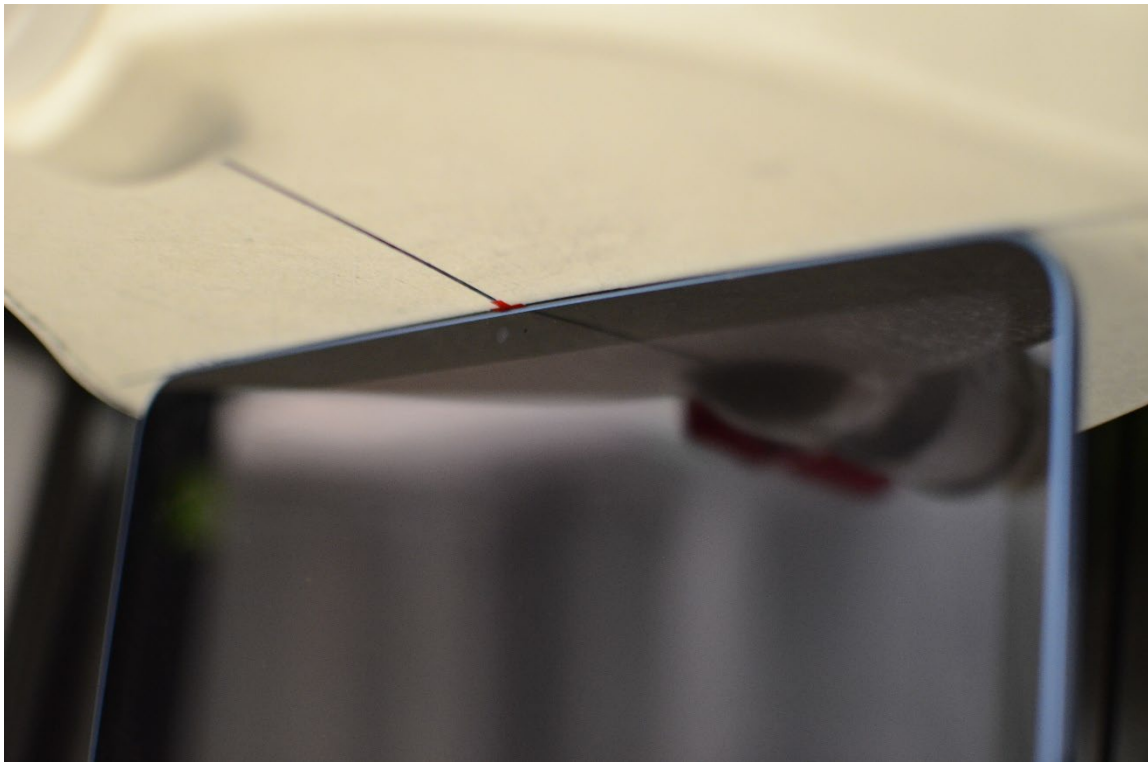
SAR Test Setup Photo 4: Body, Right Edge at 0.0 cm
