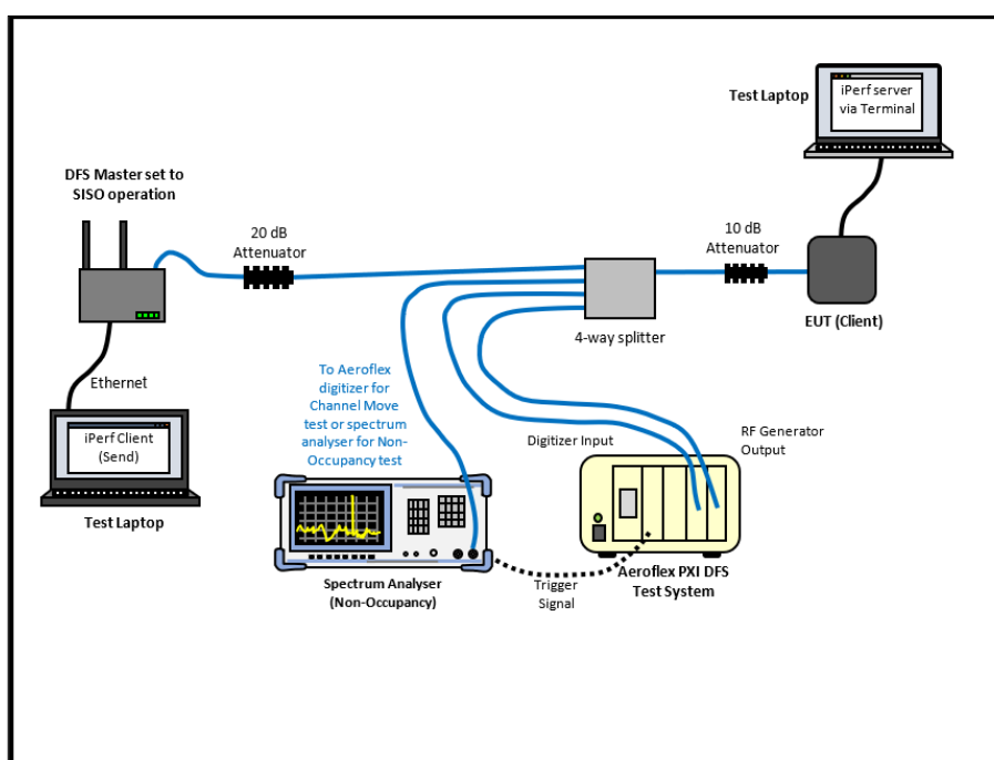
Figure 338 - Test Equipment Setup Diagram for Client without Radar Detection with Injection at the Master
