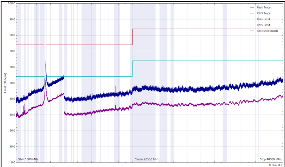
Figure 323 - U-NII-1 - 5180 MHz (CH36), HE20, RU26-0, CDD, Core 0 + Core 1, 1 GHz to 40 GHz, Horizontal
