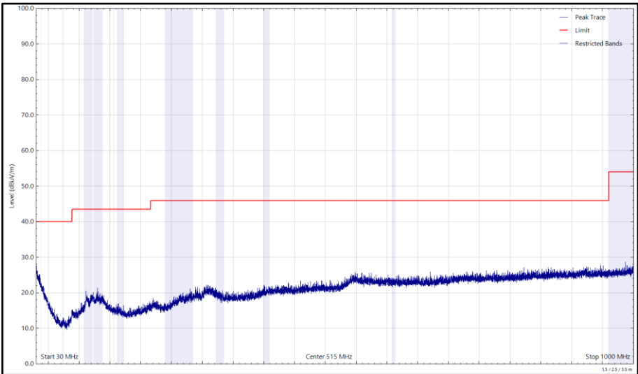
Figure 318 - U-NII-3 - 5825 MHz (CH165), VHT20, CDD, Core 0 + Core 1, 30 MHz to 1 GHz, Horizontal (Peak)
