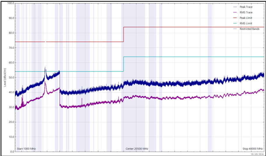
Figure 333 - U-NII-3 - 5745 MHz (CH149), HE20, RU26-0, CDD, Core 0 + Core 1, 1 GHz to 40 GHz, Vertical
