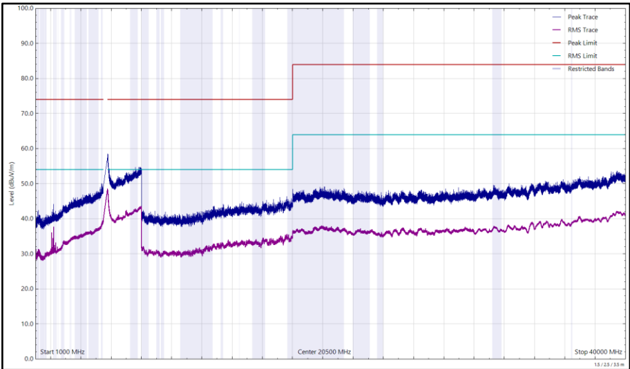
Figure 282 - U-NII-2C - 5700 MHz (CH140), 802.11a, Core 0, 1 GHz to 40 GHz, Horizontal
