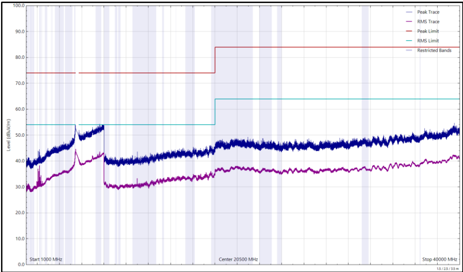
Figure 329 - U-NII-2C - 5500 MHz (CH100), HE20, RU52-37, CDD, Core 0 + Core 1, 1 GHz to 40 GHz, Vertical
