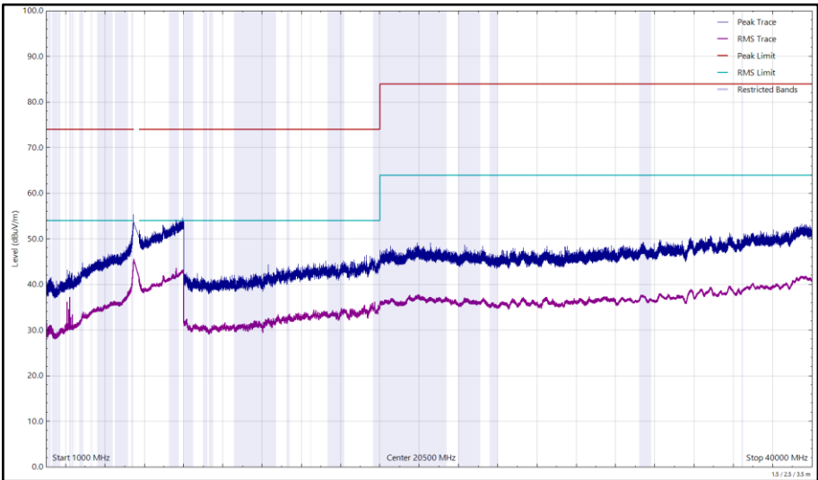
Figure 296 - U-NII-2C - 5500 MHz (CH100), 802.11a, Core 1, 1 GHz to 40 GHz, Horizontal
