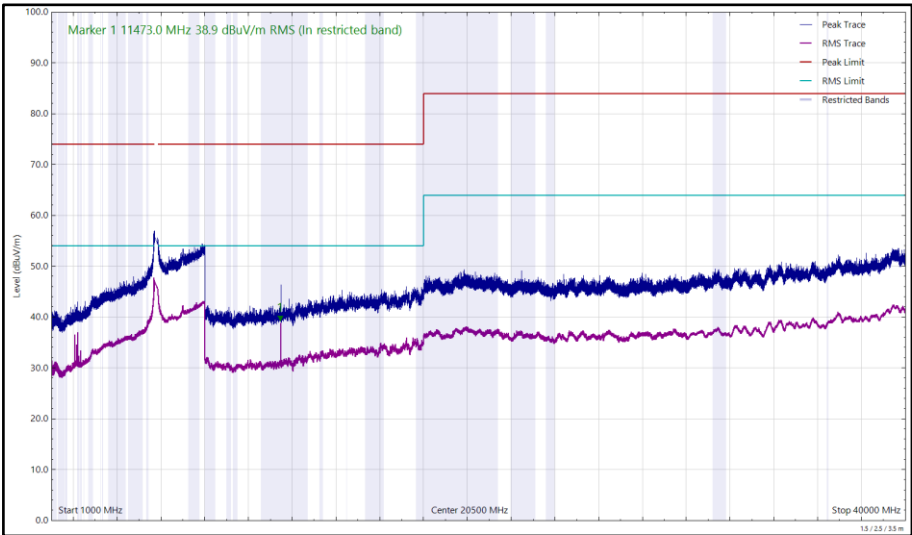
Figure 332 - U-NII-3 - 5745 MHz (CH149), HE20, RU26-0, CDD, Core 0 + Core 1, 1 GHz to 40 GHz, Horizontal
