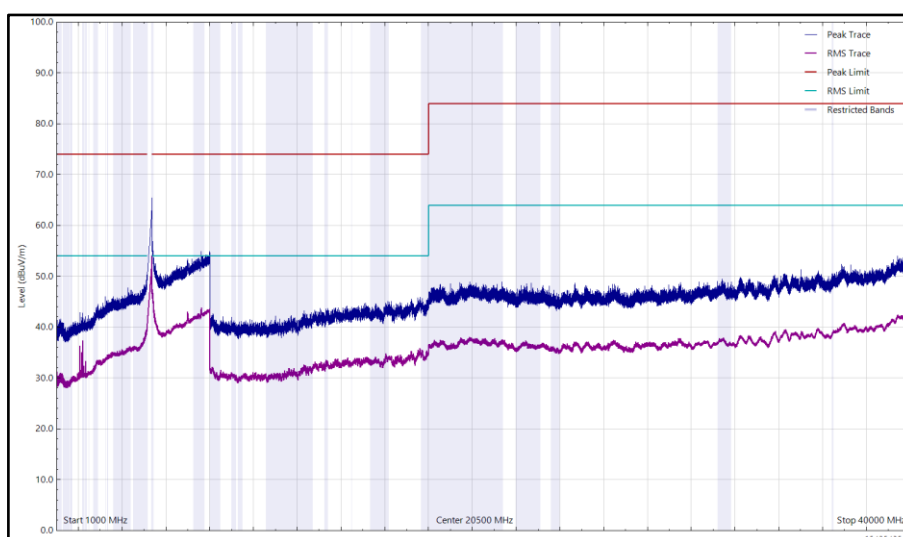
Figure 275 - U-NII-1 - 5180 MHz (CH36), 802.11a, Core 0, 1 GHz to 40 GHz, Horizontal
