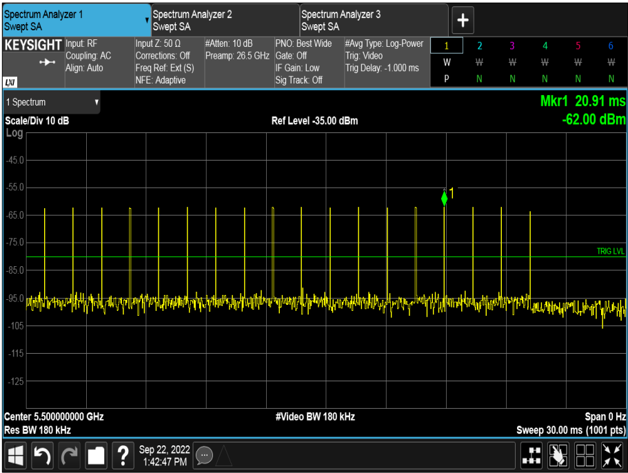
Figure 339 - Verification of Radar Type 0
