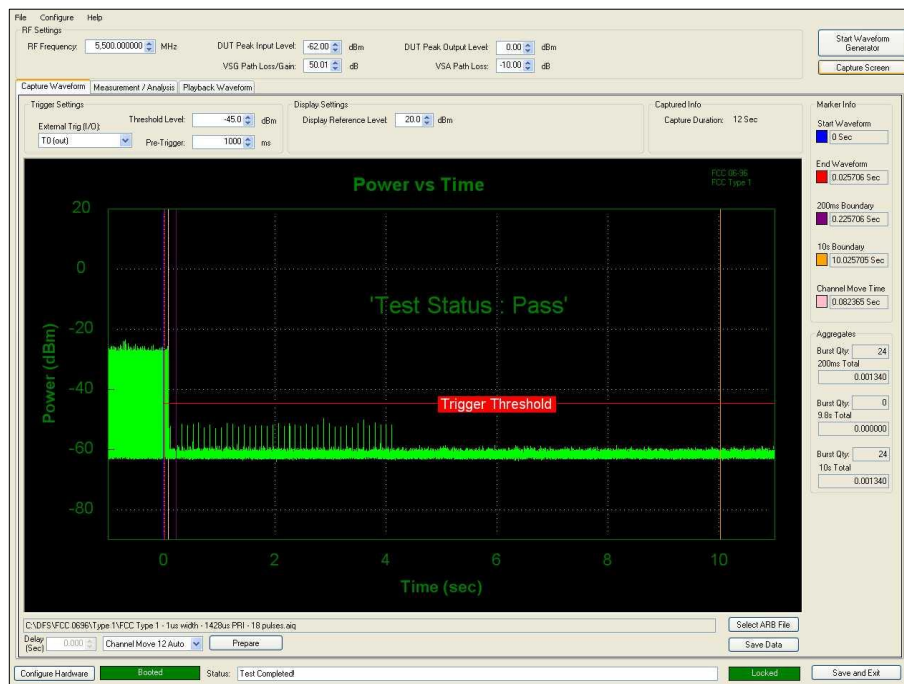
Figure 342 - First 12 s of Channel Shutdown Period
