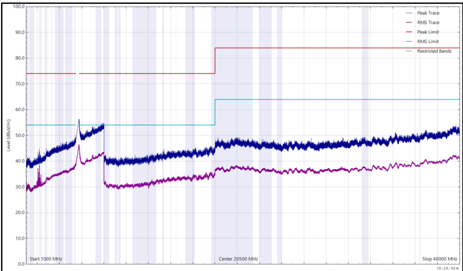
Figure 299 - U-NII-2C - 5700 MHz (CH140), 802.11a, Core 1, 1 GHz to 40 GHz, Vertical
