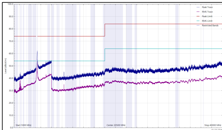
Figure 325 - U-NII-1 - 5180 MHz (CH36), HE20, RU26-0, CDD, Core 0 + Core 1, 1 GHz to 40 GHz, Vertical
