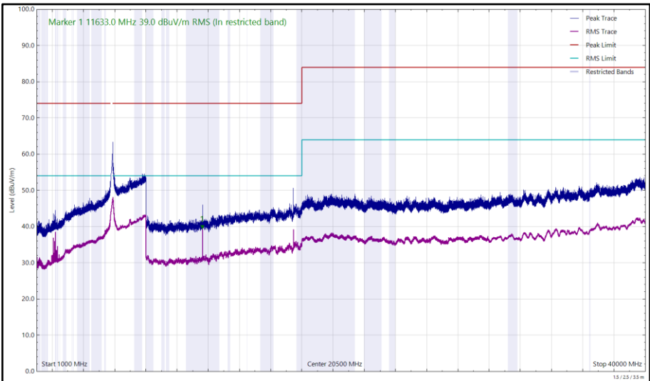
Figure 337 - U-NII-3 - 5825 MHz (CH165), HE20, RU26-0, CDD, Core 0 + Core 1, 1 GHz to 40 GHz, Vertical
