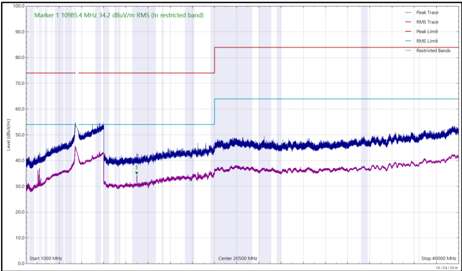
Figure 328 - U-NII-2C - 5500 MHz (CH100), HE20, RU52-37, CDD, Core 0 + Core 1, 1 GHz to 40 GHz, Horizontal
