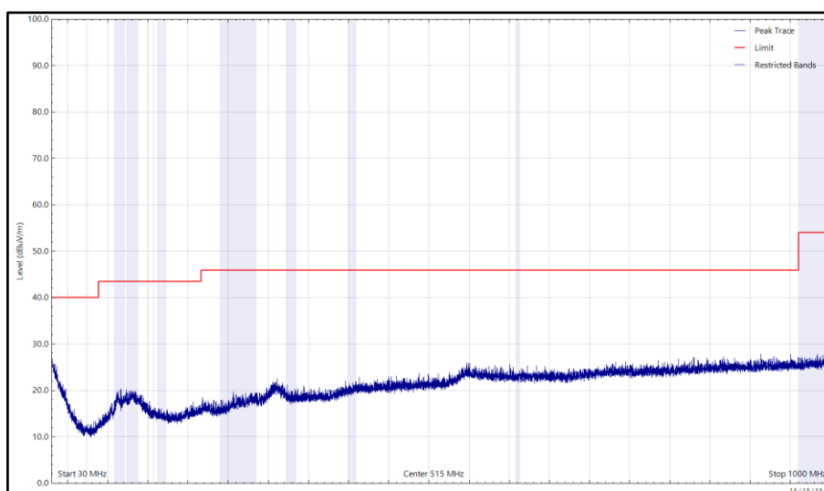
Figure 274 - U-NII-1 - 5180 MHz (CH36), 802.11a, Core 0, 30 MHz to 1 GHz, Horizontal (Peak)
