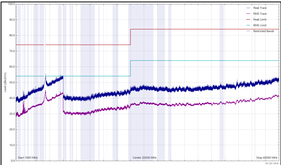
Figure 295 - U-NII-2A - 5320 MHz (CH64), 802.11a, Core 1, 1 GHz to 40 GHz, Vertical
