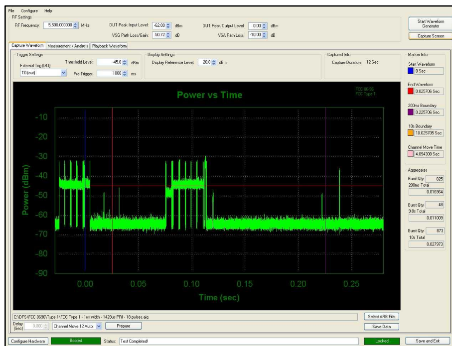
Figure 347 - First 200 ms of Channel Shutdown Period
