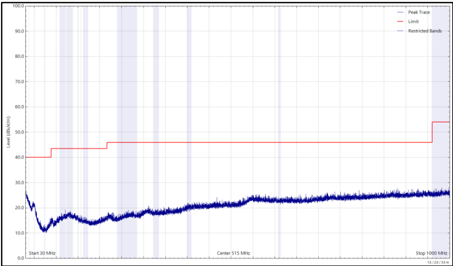
Figure 304 - U-NII-3 - 5825 MHz (CH165), 802.11a, Core 1, 30 MHz to 1 GHz, Vertical (Peak)
