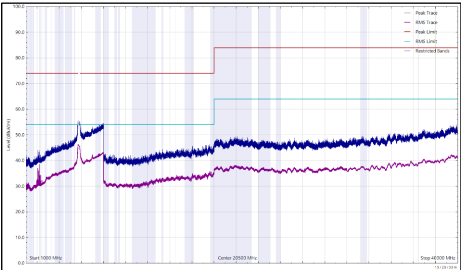
Figure 285 - U-NII-3 - 5745 MHz (CH149), 802.11a, Core 0, 1 GHz to 40 GHz, Vertical
