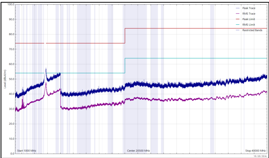
Figure 315 - U-NII-2C - 5700 MHz (CH140), VHT20, CDD, Core 0 + Core 1, 1 GHz to 40 GHz, Vertical
