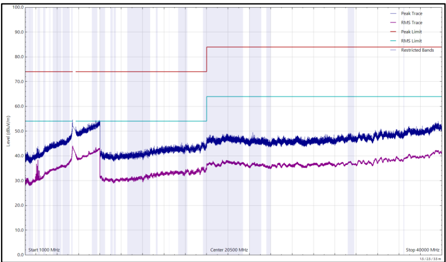
Figure 313 - U-NII-2C - 5500 MHz (CH100), VHT20, CDD, Core 0 + Core 1, 1 GHz to 40 GHz, Vertical
