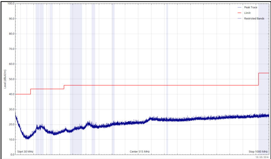
Figure 286 - U-NII-3 - 5825 MHz (CH165), 802.11a, Core 0, 30 MHz to 1 GHz, Horizontal (Peak)
