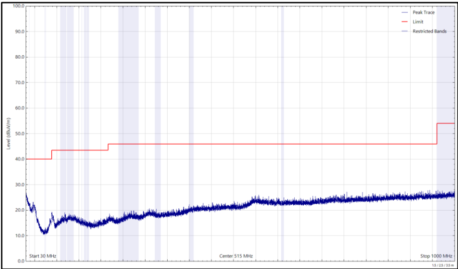
Figure 320 - U-NII-3 - 5825 MHz (CH165), VHT20, CDD, Core 0 + Core 1, 30 MHz to 1 GHz, Vertical (Peak)
