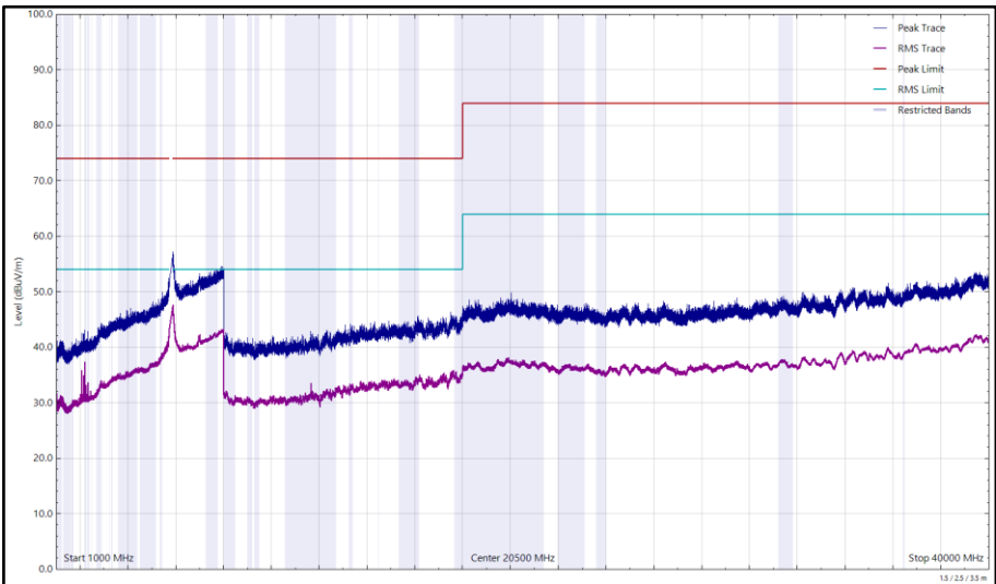
Figure 303 - U-NII-3 - 5825 MHz (CH165), 802.11a, Core 1, 1 GHz to 40 GHz, Horizontal
