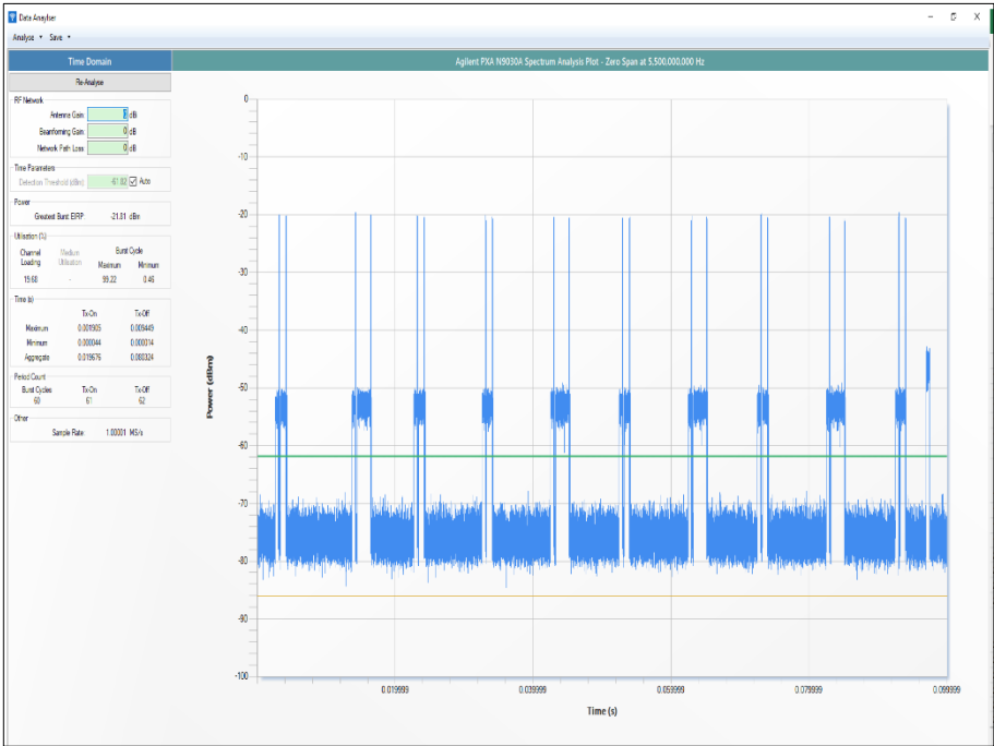
Figure 340 - Channel Loading
