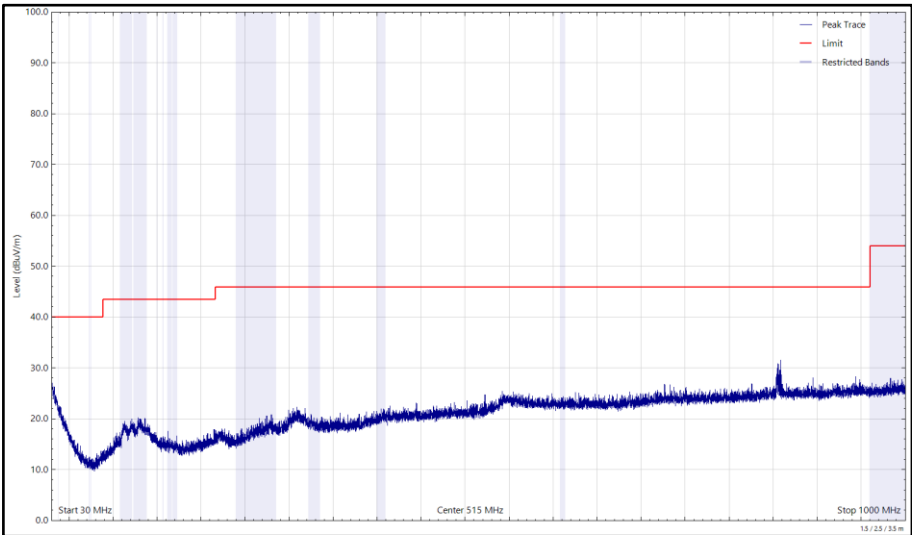
Figure 302 - U-NII-3 - 5825 MHz (CH165), 802.11a, Core 1, 30 MHz to 1 GHz, Horizontal (Peak)
