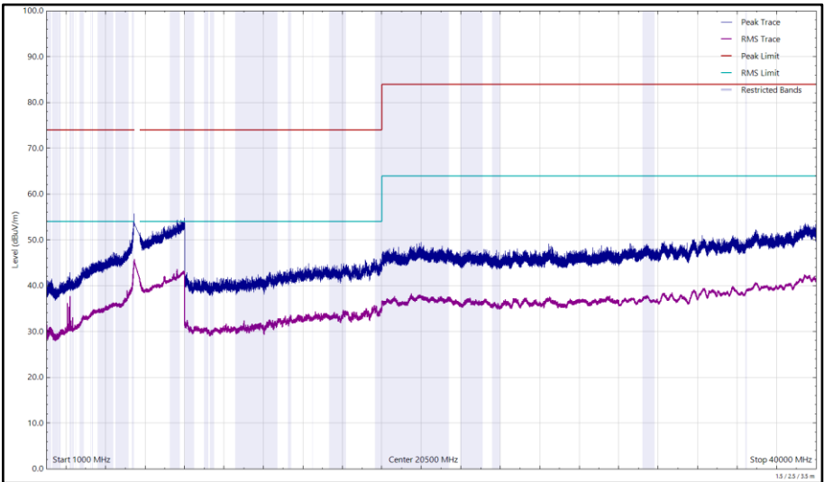
Figure 312 - U-NII-2C - 5500 MHz (CH100), VHT20, CDD, Core 0 + Core 1, 1 GHz to 40 GHz, Horizontal
