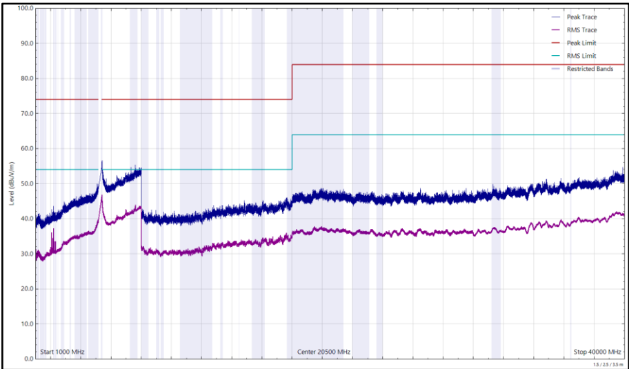
Figure 278 - U-NII-2A - 5320 MHz (CH64), 802.11a, Core 0, 1 GHz to 40 GHz, Horizontal
