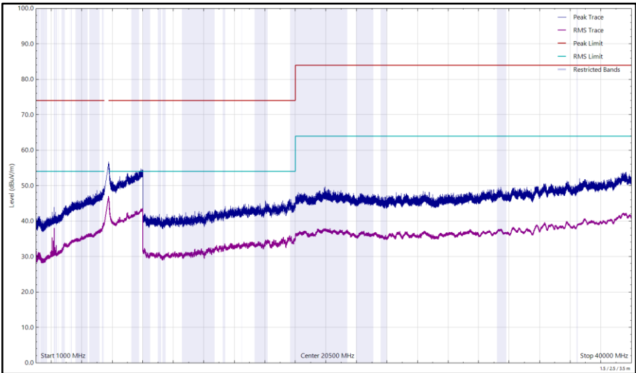
Figure 298 - U-NII-2C - 5700 MHz (CH140), 802.11a, Core 1, 1 GHz to 40 GHz, Horizontal
