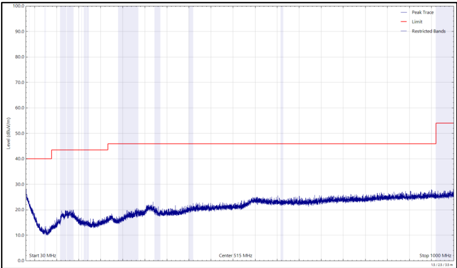
Figure 306 - U-NII-1 - 5180 MHz (CH36), VHT20, CDD, Core 0 + Core 1, 30 MHz to 1 GHz, Horizontal (Peak)
