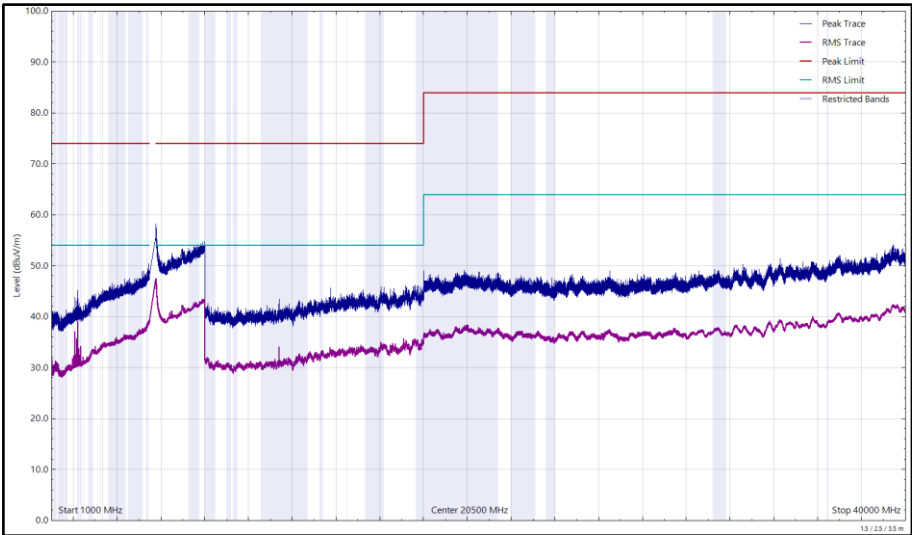
Figure 331 - U-NII-2C - 5700 MHz (CH140), HE20, RU52-37, CDD, Core 0 + Core 1, 1 GHz to 40 GHz, Vertical
