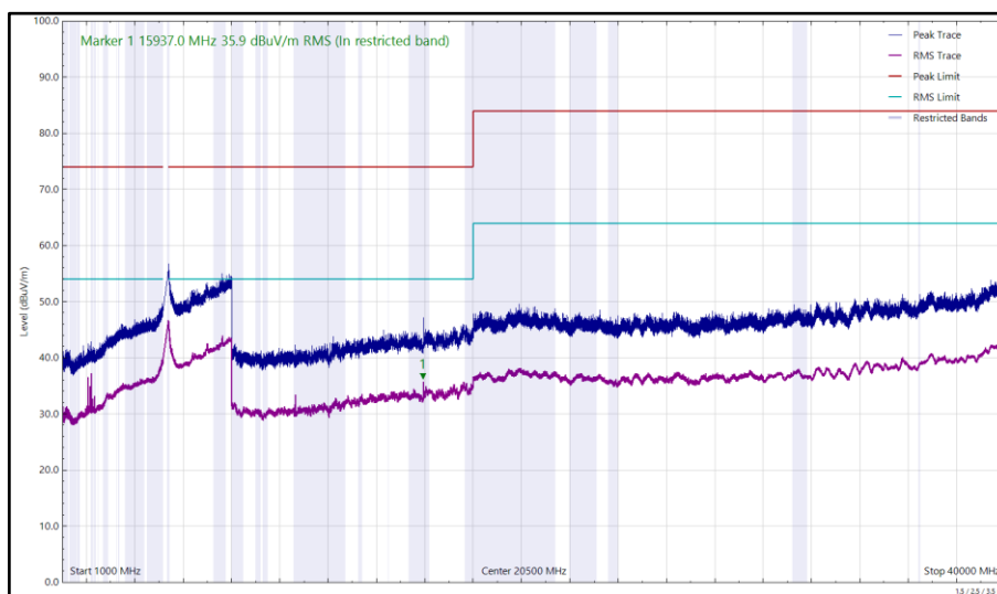
Figure 326 - U-NII-2A - 5320 MHz (CH64), HE20, RU52-37, CDD, Core 0 + Core 1, 1 GHz to 40 GHz, Horizontal
