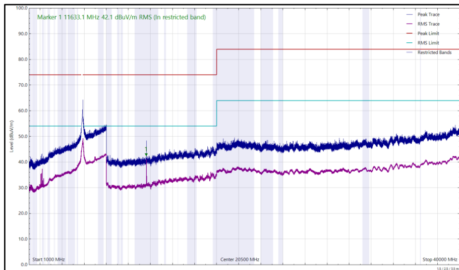
Figure 335 - U-NII-3 - 5825 MHz (CH165), HE20, RU26-0, CDD, Core 0 + Core 1, 1 GHz to 40 GHz, Horizontal
