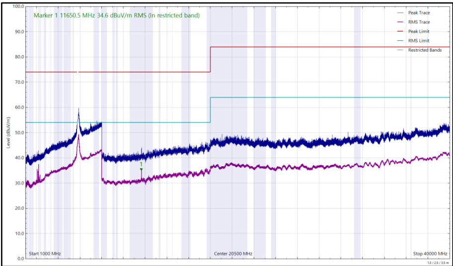
Figure 319 - U-NII-3 - 5825 MHz (CH165), VHT20, CDD, Core 0 + Core 1, 1 GHz to 40 GHz, Horizontal
