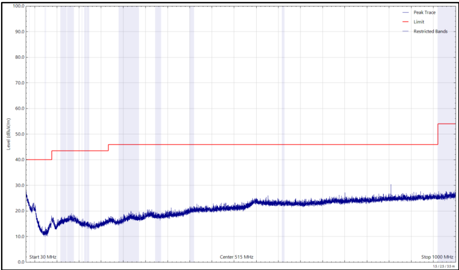
Figure 308 - U-NII-1 - 5180 MHz (CH36), VHT20, CDD, Core 0 + Core 1, 30 MHz to 1 GHz, Vertical (Peak)
