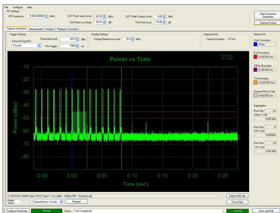
Figure 341 - First 200 ms of Channel Shutdown Period
