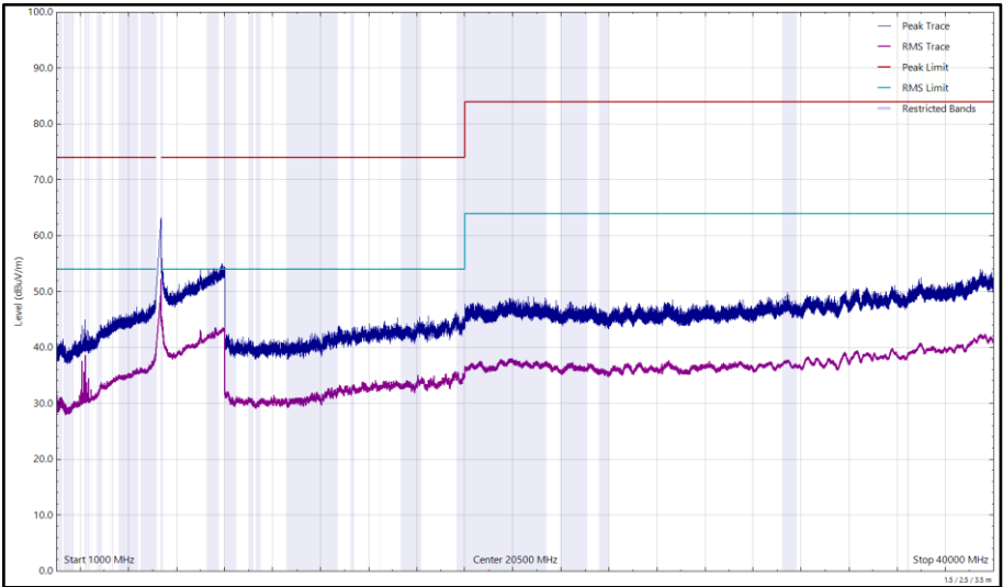
Figure 277 - U-NII-1 - 5180 MHz (CH36), 802.11a, Core 0, 1 GHz to 40 GHz, Vertical
