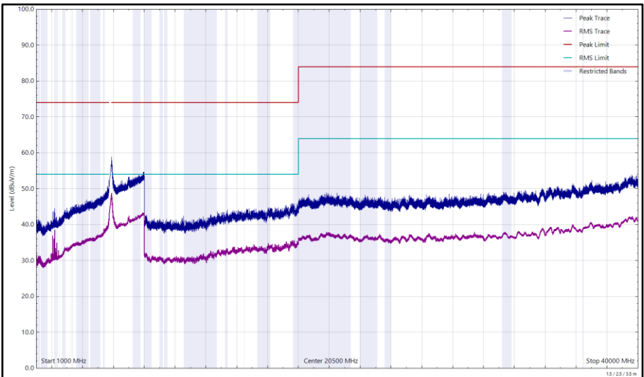
Figure 289 - U-NII-3 - 5825 MHz (CH165), 802.11a, Core 0, 1 GHz to 40 GHz, Vertical
