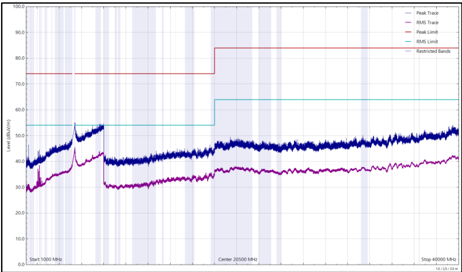
Figure 311 - U-NII-2A - 5320 MHz (CH64), VHT20, CDD, Core 0 + Core 1, 1 GHz to 40 GHz, Vertical
