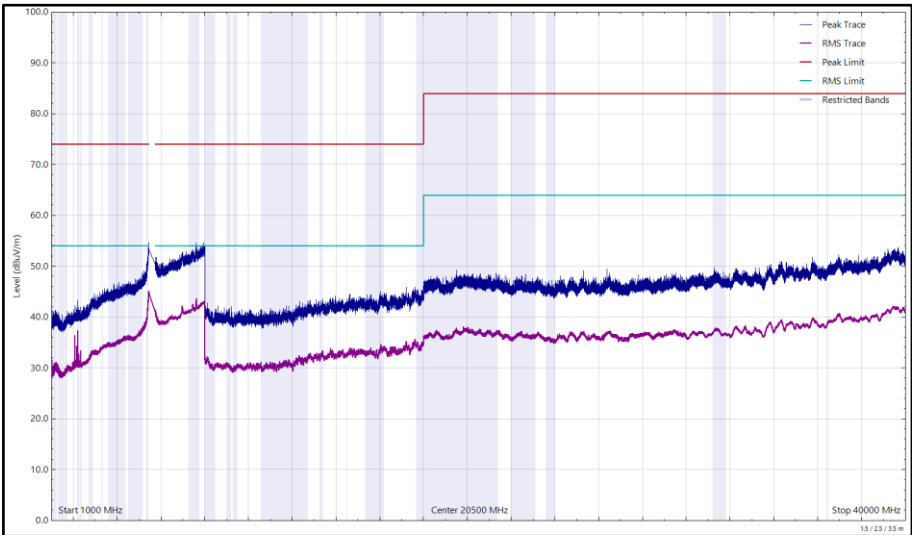
Figure 280 - U-NII-2C - 5500 MHz (CH100), 802.11a, Core 0, 1 GHz to 40 GHz, Horizontal
