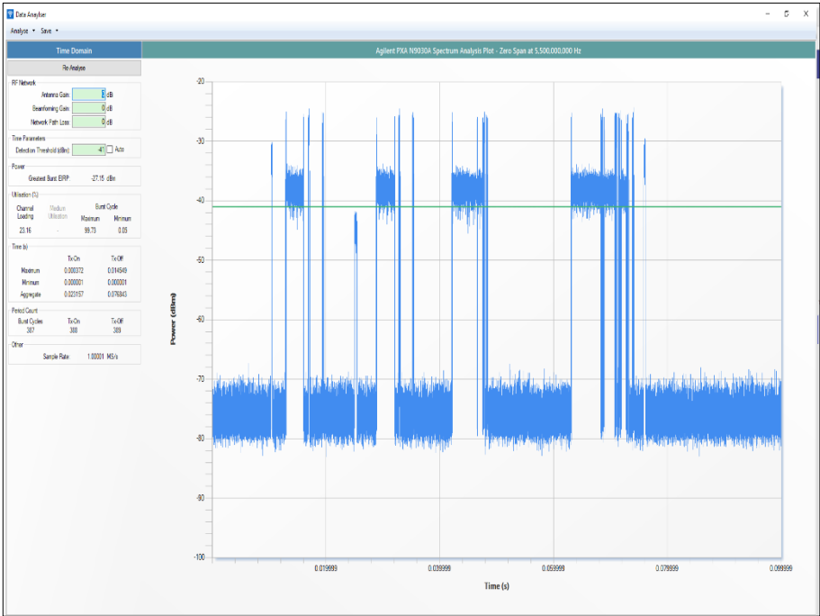
Figure 346 - Channel Loading
