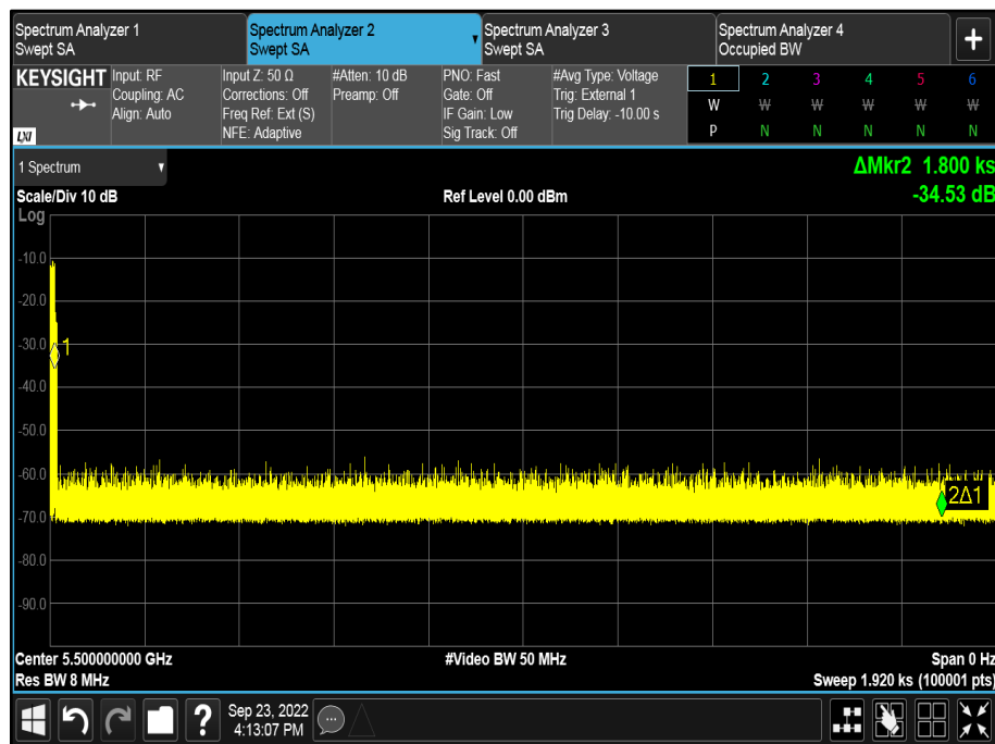
Figure 349 - 30-minute Non-Occupancy Period
