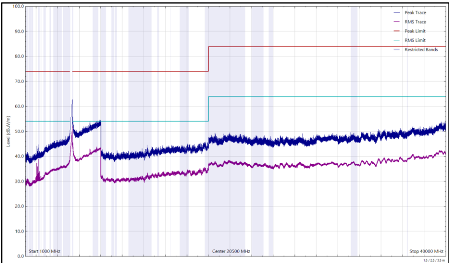
Figure 309 - U-NII-1 - 5180 MHz (CH36), VHT20, CDD, Core 0 + Core 1, 1 GHz to 40 GHz, Vertical
