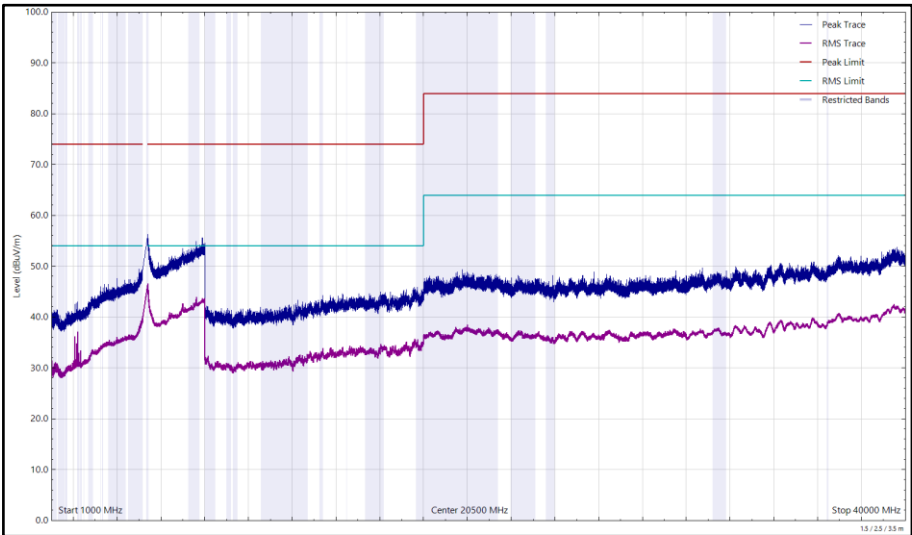
Figure 310 - U-NII-2A - 5320 MHz (CH64), VHT20, CDD, Core 0 + Core 1, 1 GHz to 40 GHz, Horizontal
