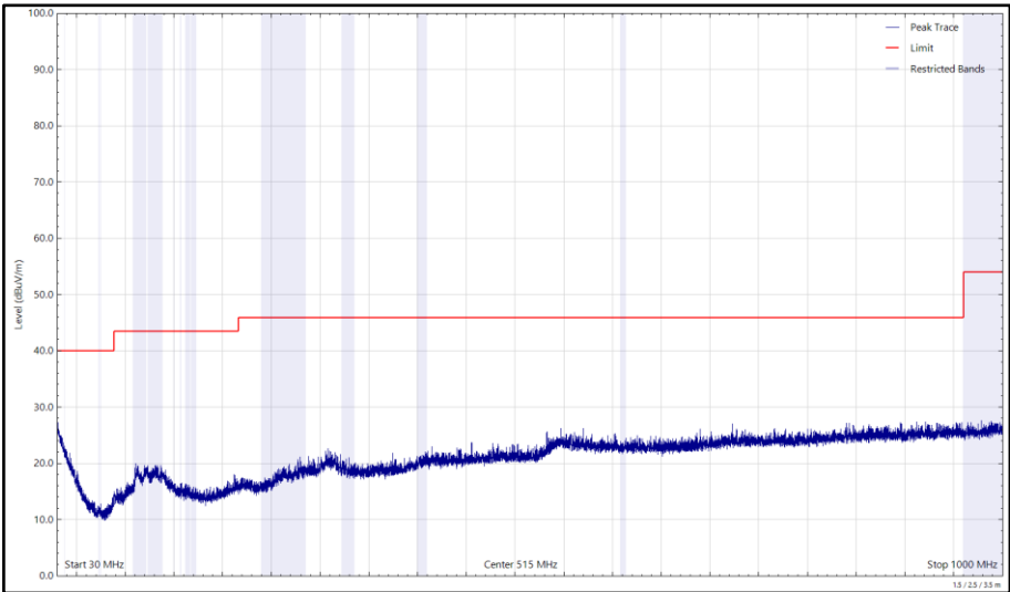
Figure 322 - U-NII-1 - 5180 MHz (CH36), HE20, RU26-0, CDD, Core 0 + Core 1, 30 MHz to 1 GHz, Horizontal (Peak)
