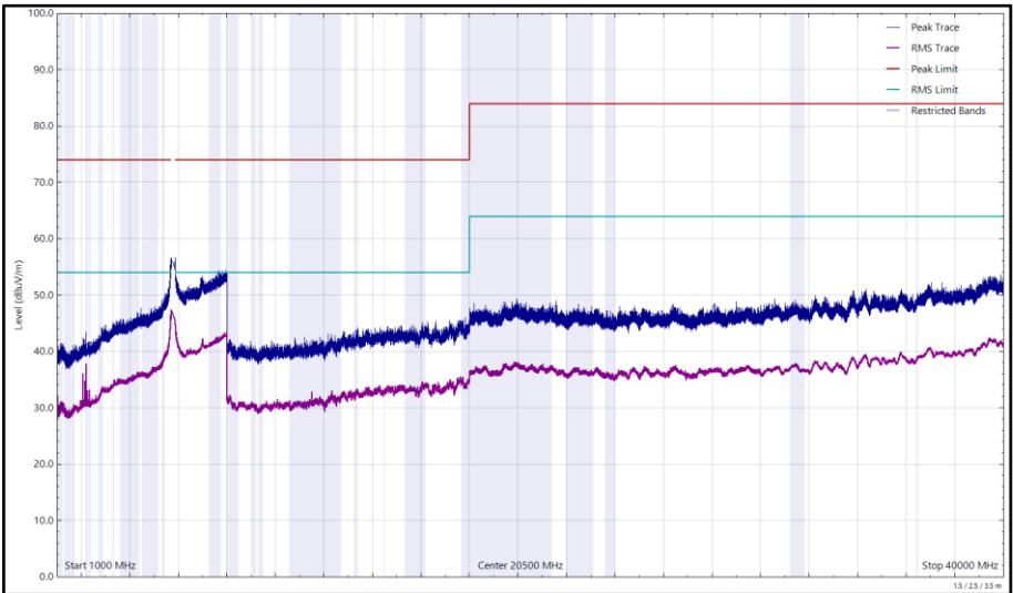
Figure 316 - U-NII-3 - 5745 MHz (CH149), VHT20, CDD, Core 0 + Core 1, 1 GHz to 40 GHz, Horizontal
