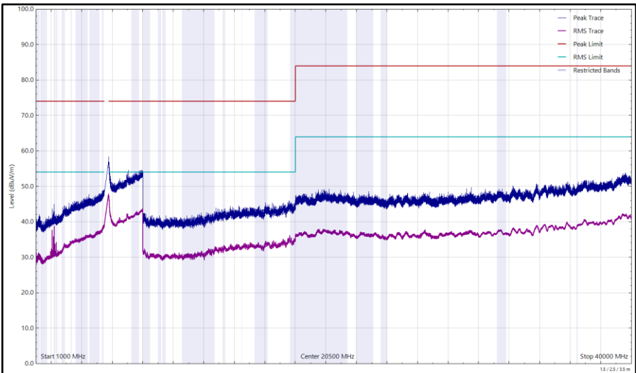
Figure 283 - U-NII-2C - 5700 MHz (CH140), 802.11a, Core 0, 1 GHz to 40 GHz, Vertical
