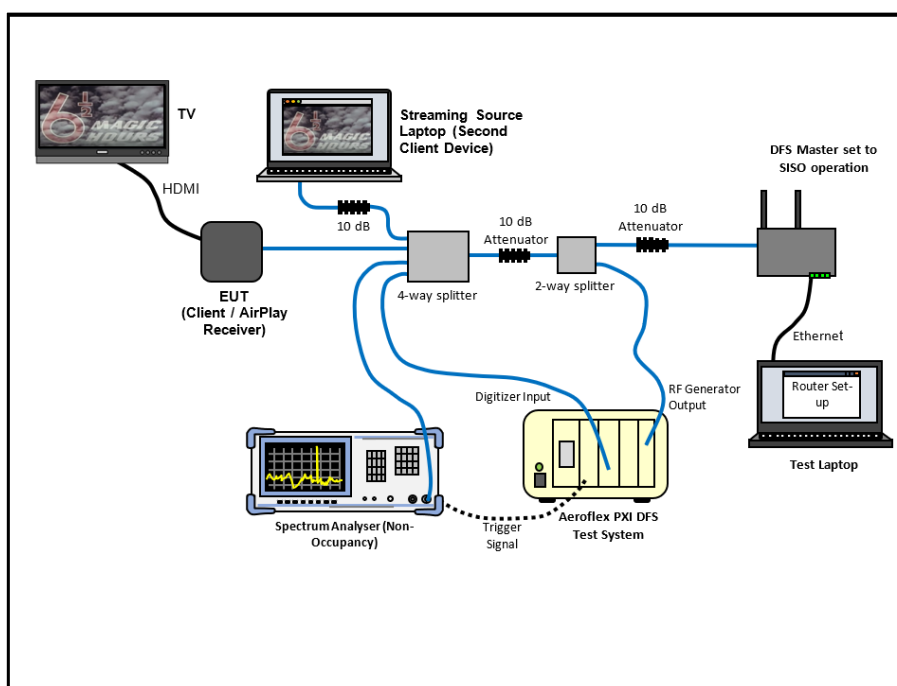
Figure 344 - Test Equipment Setup Diagram for Client without Radar Detection with Injection at the Master
