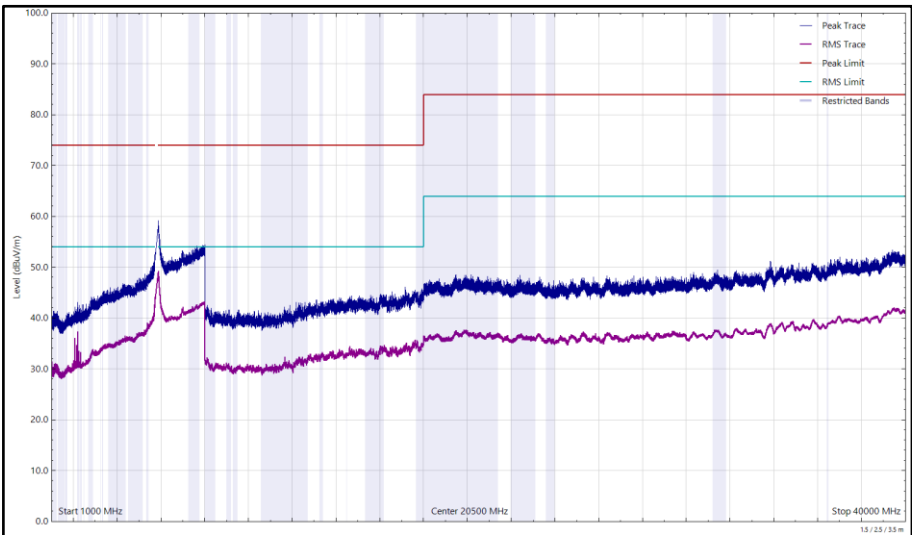
Figure 287 - U-NII-3 - 5825 MHz (CH165), 802.11a, Core 0, 1 GHz to 40 GHz, Horizontal
