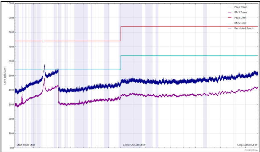
Figure 314 - U-NII-2C - 5700 MHz (CH140), VHT20, CDD, Core 0 + Core 1, 1 GHz to 40 GHz, Horizontal
