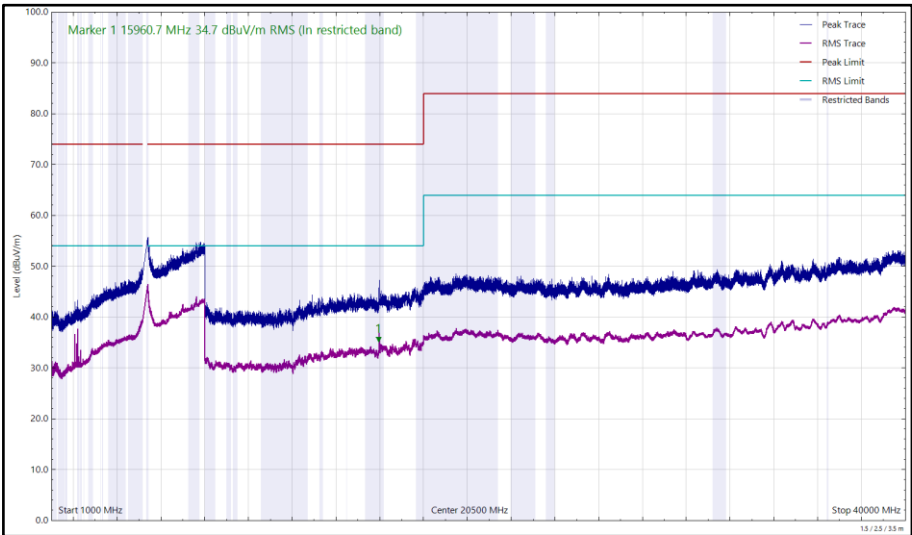
Figure 294 - U-NII-2A - 5320 MHz (CH64), 802.11a, Core 1, 1 GHz to 40 GHz, Horizontal
