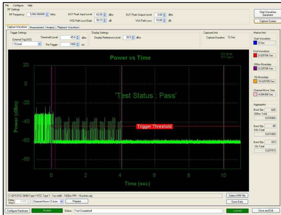
Figure 348 - First 12 s of Channel Shutdown Period
