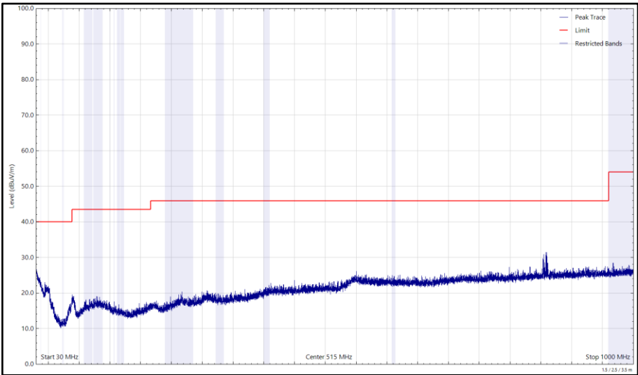
Figure 336 - U-NII-3 - 5825 MHz (CH165), HE20, RU26-0, CDD, Core 0 + Core 1, 30 MHz to 1 GHz, Vertical (Peak)
