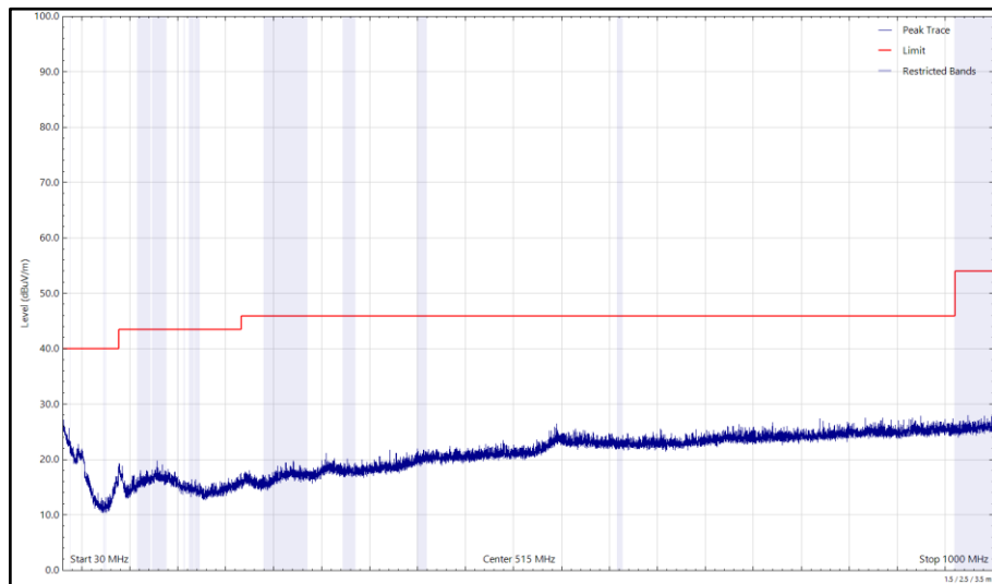
Figure 324 - U-NII-1 - 5180 MHz (CH36), HE20, RU26-0, CDD, Core 0 + Core 1, 30 MHz to 1 GHz, Vertical (Peak)
