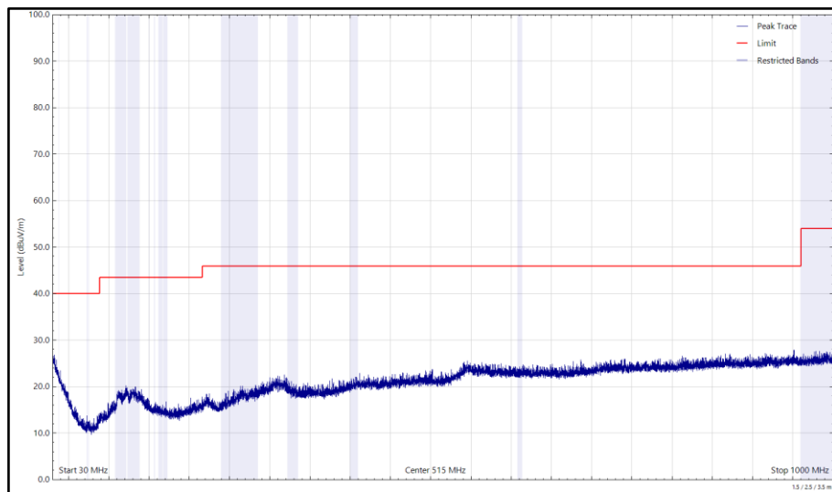
Figure 334 - U-NII-3 - 5825 MHz (CH165), HE20, RU26-0, CDD, Core 0 + Core 1, 30 MHz to 1 GHz, Horizontal (Peak)
