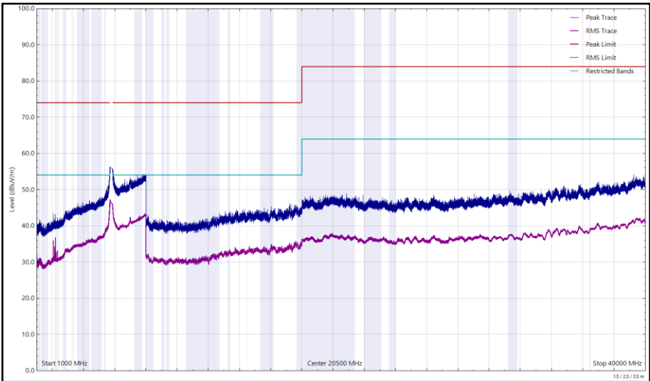
Figure 284 - U-NII-3 - 5745 MHz (CH149), 802.11a, Core 0, 1 GHz to 40 GHz, Horizontal
