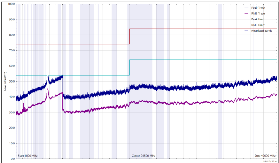
Figure 301 - U-NII-3 - 5745 MHz (CH149), 802.11a, Core 1, 1 GHz to 40 GHz, Vertical
