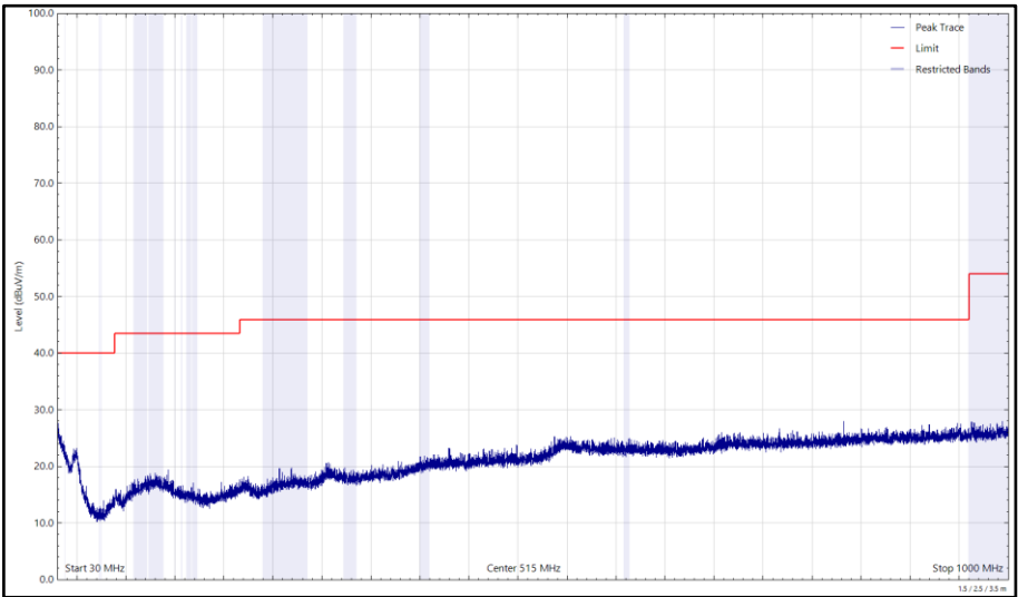
Figure 276 - U-NII-1 - 5180 MHz (CH36), 802.11a, Core 0, 30 MHz to 1 GHz, Vertical (Peak)
