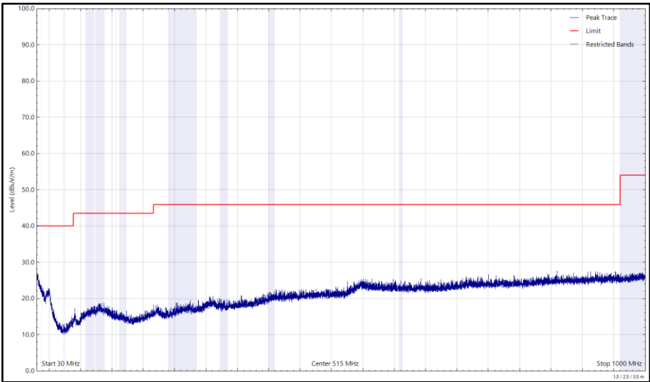
Figure 292 - U-NII-1 - 5180 MHz (CH36), 802.11a, Core 1, 30 MHz to 1 GHz, Vertical (Peak)
