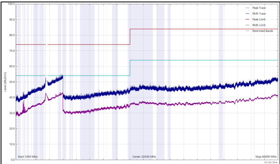
Figure 297 - U-NII-2C - 5500 MHz (CH100), 802.11a, Core 1, 1 GHz to 40 GHz, Vertical
