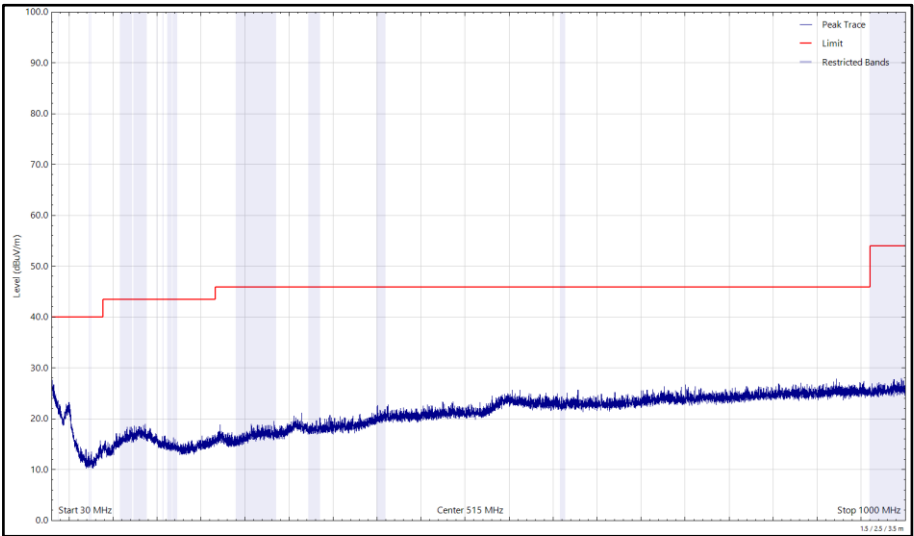
Figure 288 - U-NII-3 - 5825 MHz (CH165), 802.11a, Core 0, 30 MHz to 1 GHz, Vertical (Peak)
