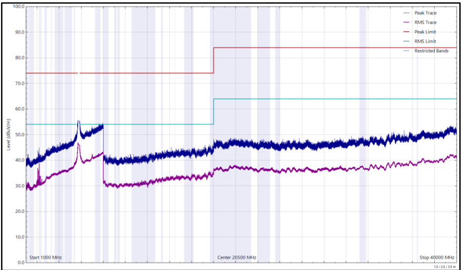
Figure 317 - U-NII-3 - 5745 MHz (CH149), VHT20, CDD, Core 0 + Core 1, 1 GHz to 40 GHz, Vertical
