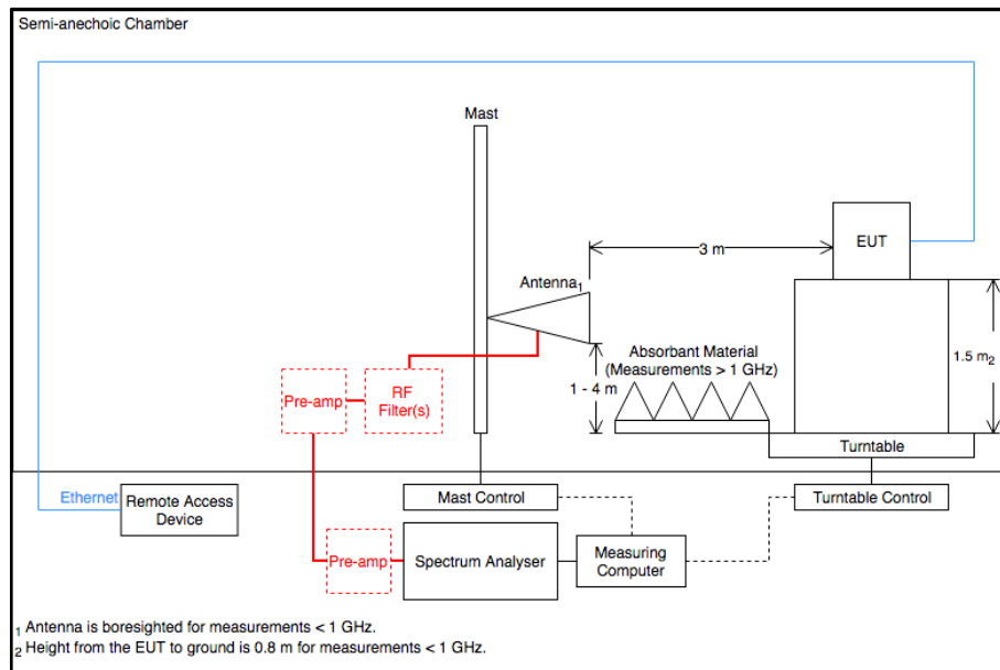
Figure 273 - Radiated Emissions Test Setup Diagram
