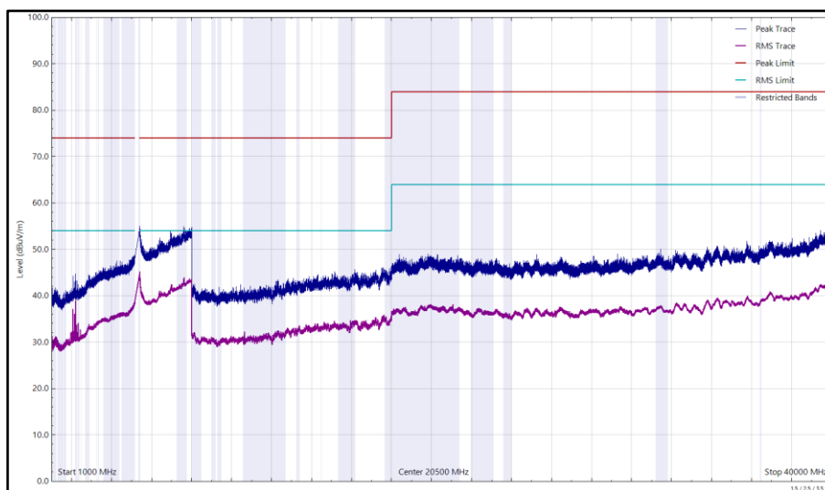
Figure 327 - U-NII-2A - 5320 MHz (CH64), HE20, RU52-37, CDD, Core 0 + Core 1, 1 GHz to 40 GHz, Vertical
