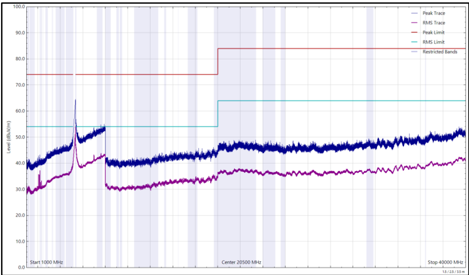
Figure 307 - U-NII-1 - 5180 MHz (CH36), VHT20, CDD, Core 0 + Core 1, 1 GHz to 40 GHz, Horizontal
