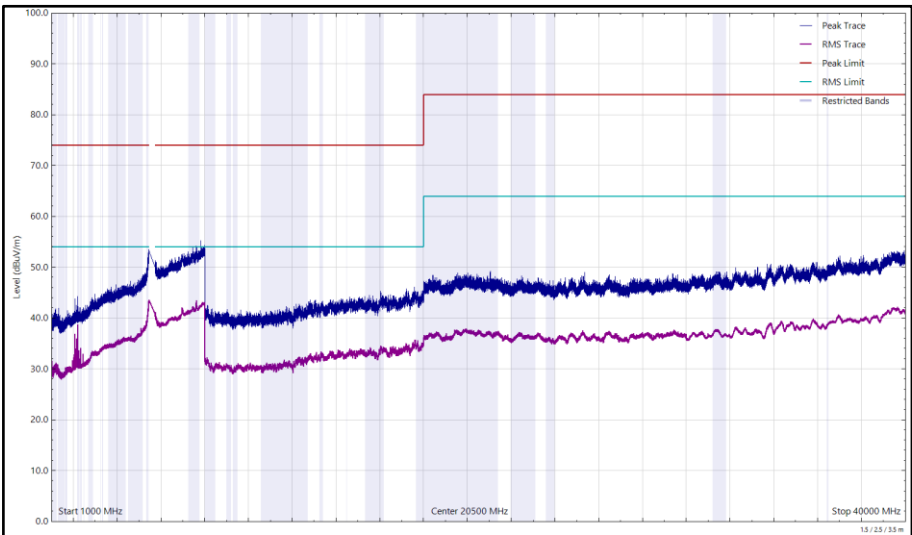
Figure 281 - U-NII-2C - 5500 MHz (CH100), 802.11a, Core 0, 1 GHz to 40 GHz, Vertical
