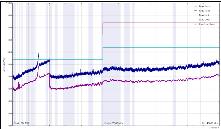
Figure 321 - U-NII-3 - 5825 MHz (CH165), VHT20, CDD, Core 0 + Core 1, 1 GHz to 40 GHz, Vertical
