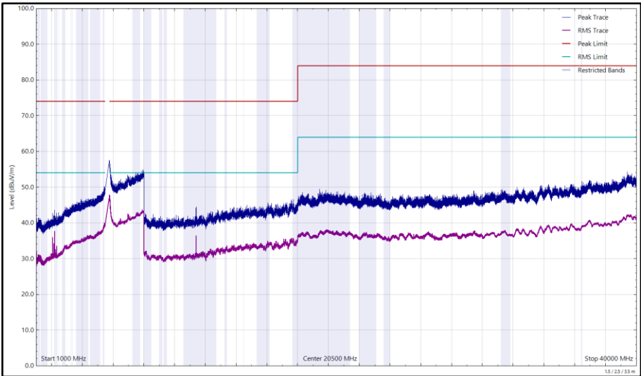
Figure 330 - U-NII-2C - 5700 MHz (CH140), HE20, RU52-37, CDD, Core 0 + Core 1, 1 GHz to 40 GHz, Horizontal
