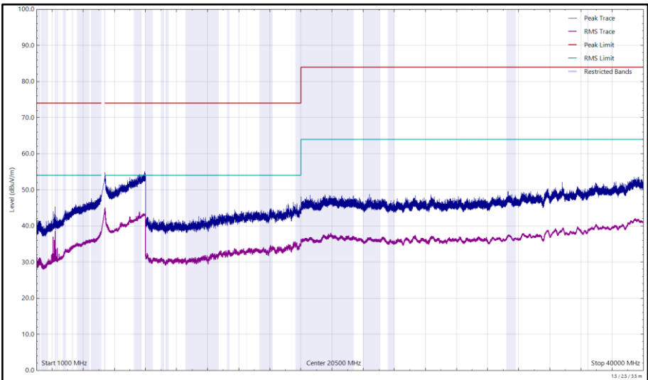
Figure 279 - U-NII-2A - 5320 MHz (CH64), 802.11a, Core 0, 1 GHz to 40 GHz, Vertical
