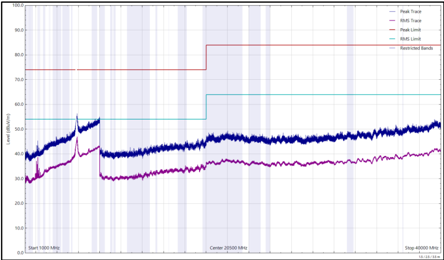
Figure 305 - U-NII-3 - 5825 MHz (CH165), 802.11a, Core 1, 1 GHz to 40 GHz, Vertical
