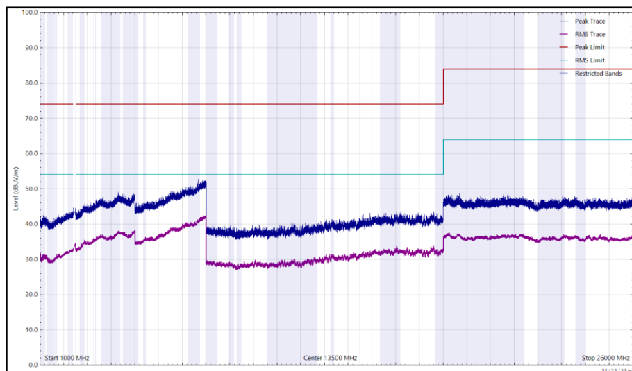
Figure 65 - 2472 MHz (CH13), 802.11g, Core 0, 1 GHz to 26 GHz, Vertical
