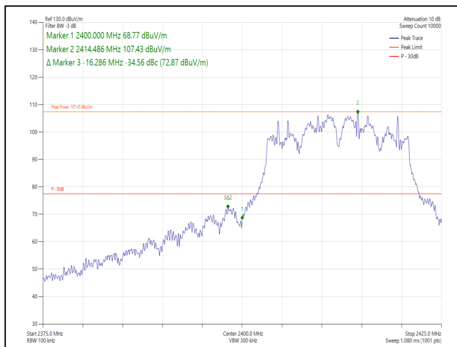
Figure 103 - 802.11n HT20, Cores 0-1 - 2412 MHz Band Edge Frequency 2400 MHz
