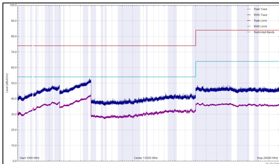
Figure 64 - 2472 MHz (CH13), 802.11g, Core 0, 1 GHz to 26 GHz, Horizontal
