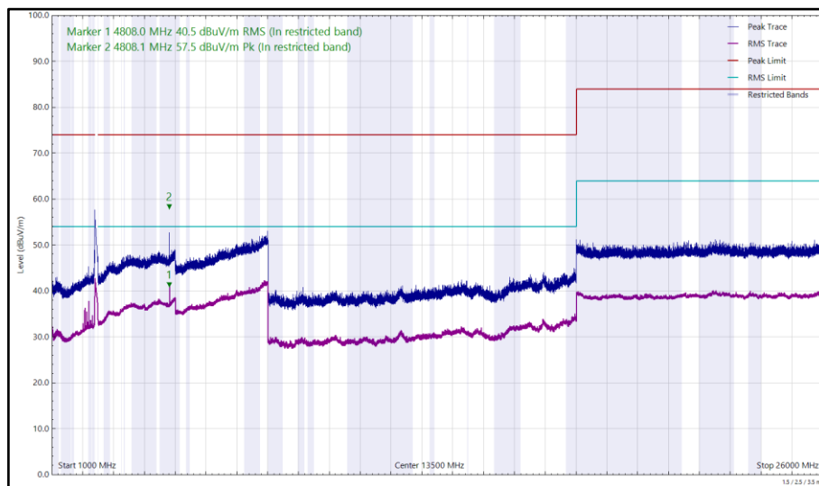
Figure 90 - 2412 MHz (CH1), HE20, RU26-0, Core 0 + Core 1, 1 GHz to 26 GHz, Horizontal
