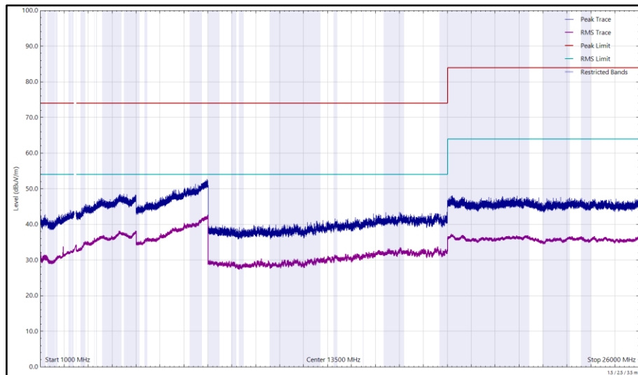
Figure 89 - 2472 MHz (CH13), 802.11g, Core 1, 1 GHz to 26 GHz, Vertical
