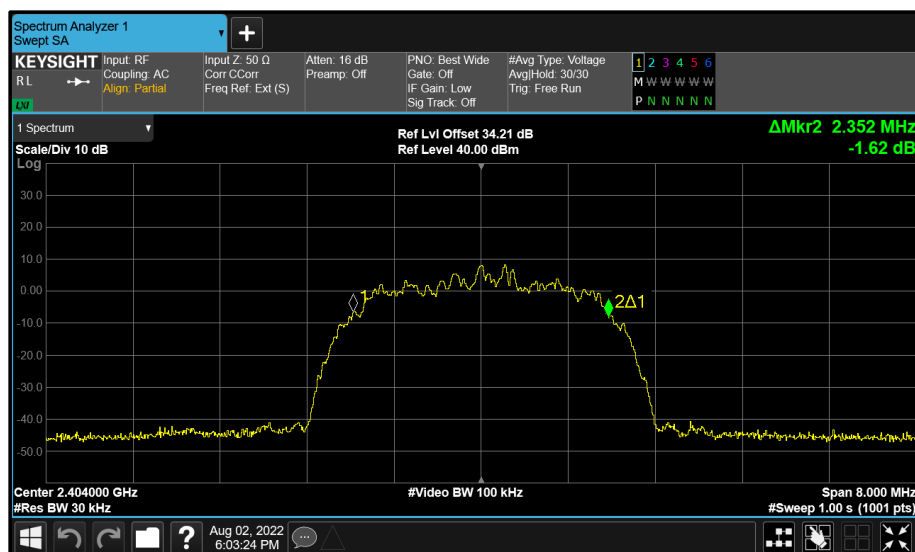
Figure 41 - BT Core 1 (B) 2404 MHz (CH2) 99% Bandwidth
