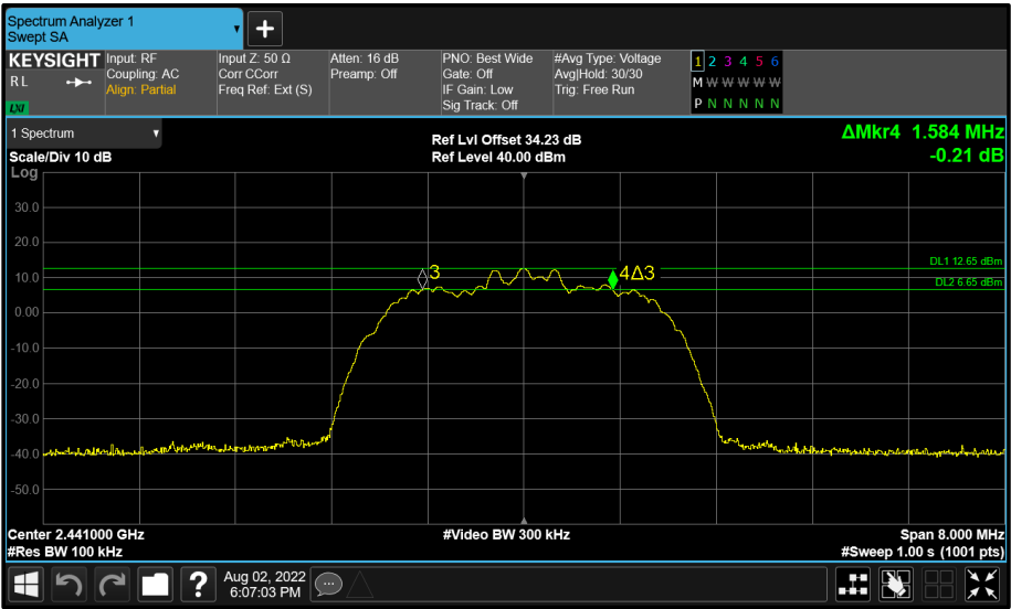
Figure 44 - BT Core 1 (B) 2441 MHz (CH39) 6 dB Bandwidth
