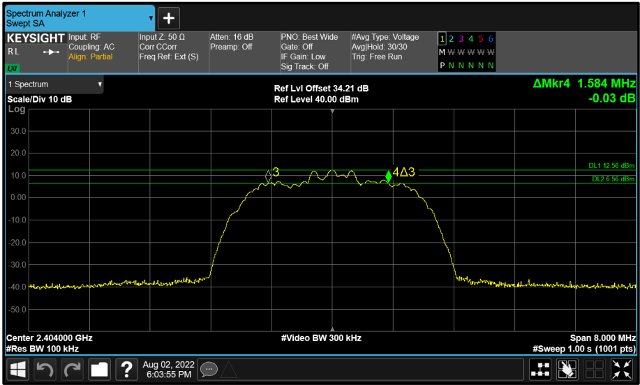
Figure 42 - BT Core 1 (B) 2404 MHz (CH2) 6 dB Bandwidth
