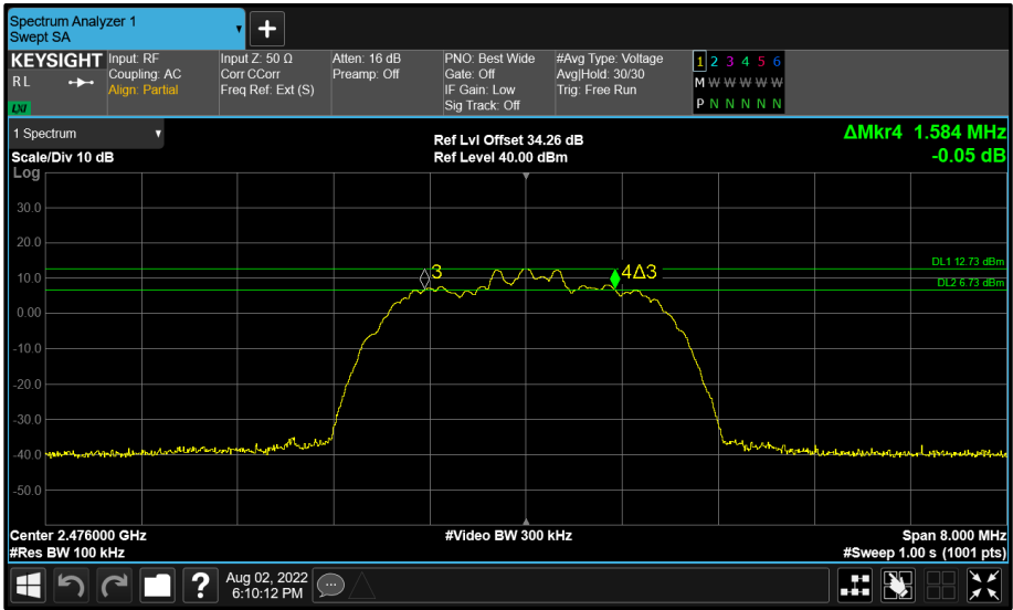
Figure 46 - BT Core 1 (B) 2476 MHz (CH74) 6 dB Bandwidth
