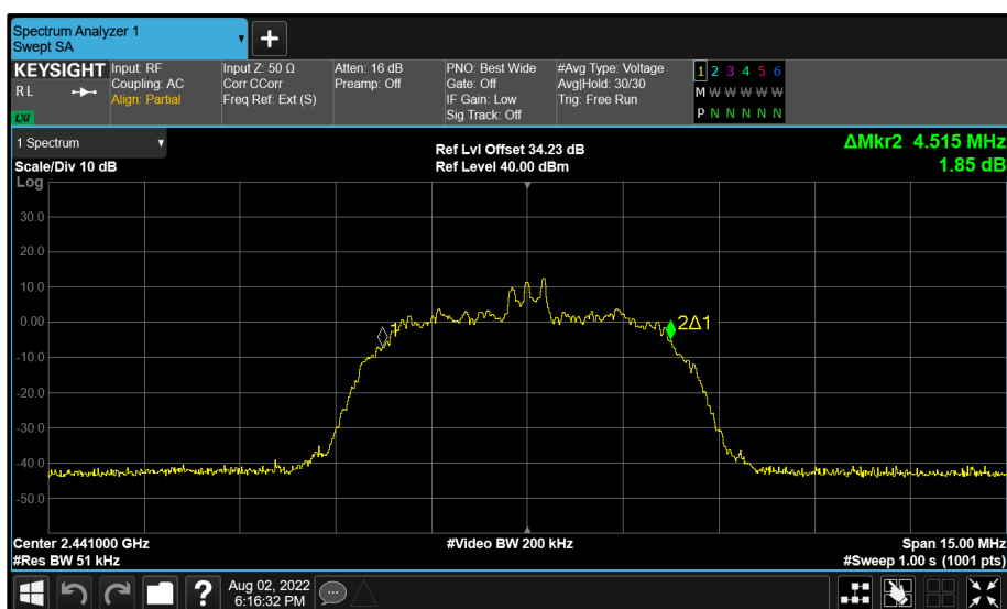
Figure 49 - BT Core 1 (B) 2441 MHz (CH39) 99% Bandwidth
