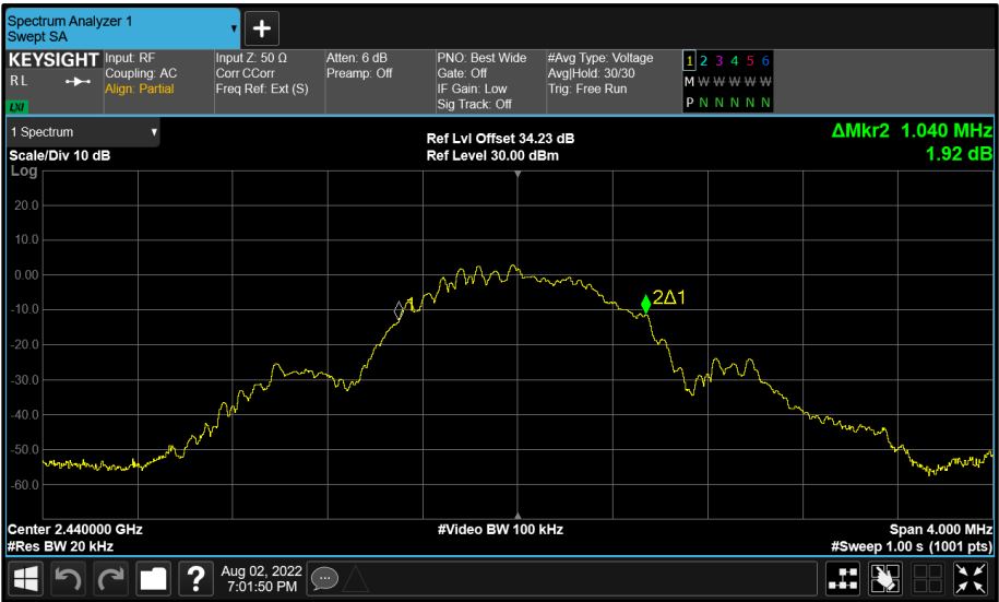
Figure 55 - BT Core 1 (B) 2440 MHz (CH17) 99% Bandwidth
