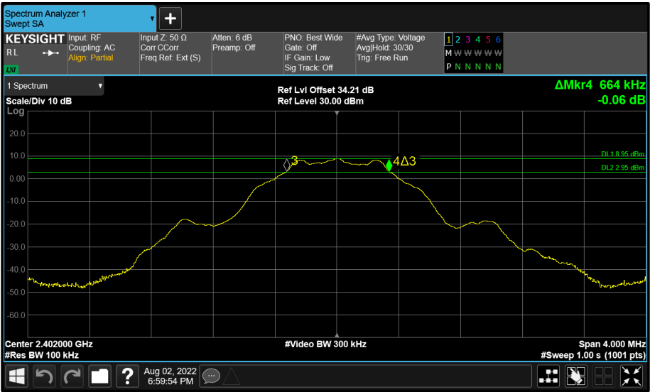
Figure 54 - BT Core 1 (B) 2402 MHz (CH37) 6 dB Bandwidth
