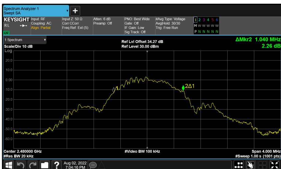
Figure 57 - BT Core 1 (B) 2480 MHz (CH39) 99% Bandwidth
