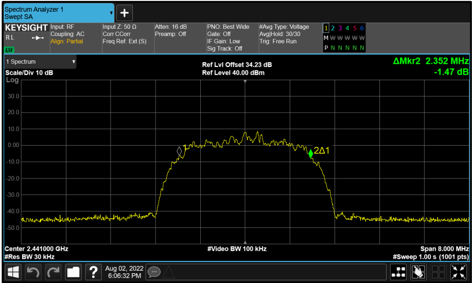
Figure 43 - BT Core 1 (B) 2441 MHz (CH39) 99% Bandwidth
