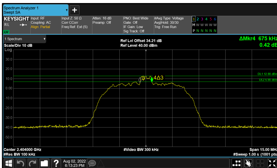
Figure 48 - BT Core 1 (B) 2404 MHz (CH2) 6 dB Bandwidth
