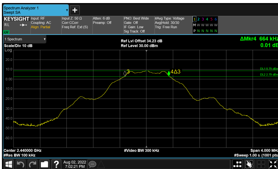
Figure 56 - BT Core 1 (B) 2440 MHz (CH17) 6 dB Bandwidth
