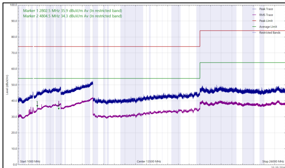
Figure 140 - 2402 MHz (CH0), DH5, iPA, Core 0 + Core 1, 1 GHz to 26 GHz, Horizontal
