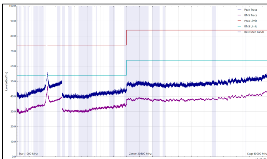
Figure 17 - 2472 MHz (CH13), HT20, Core 0 + Core 1 and U-NII-2C - 5680 MHz (CH136), VHT20, CDD, Core 0 + Core 1, 1 GHz to 40 GHz, Vertical
