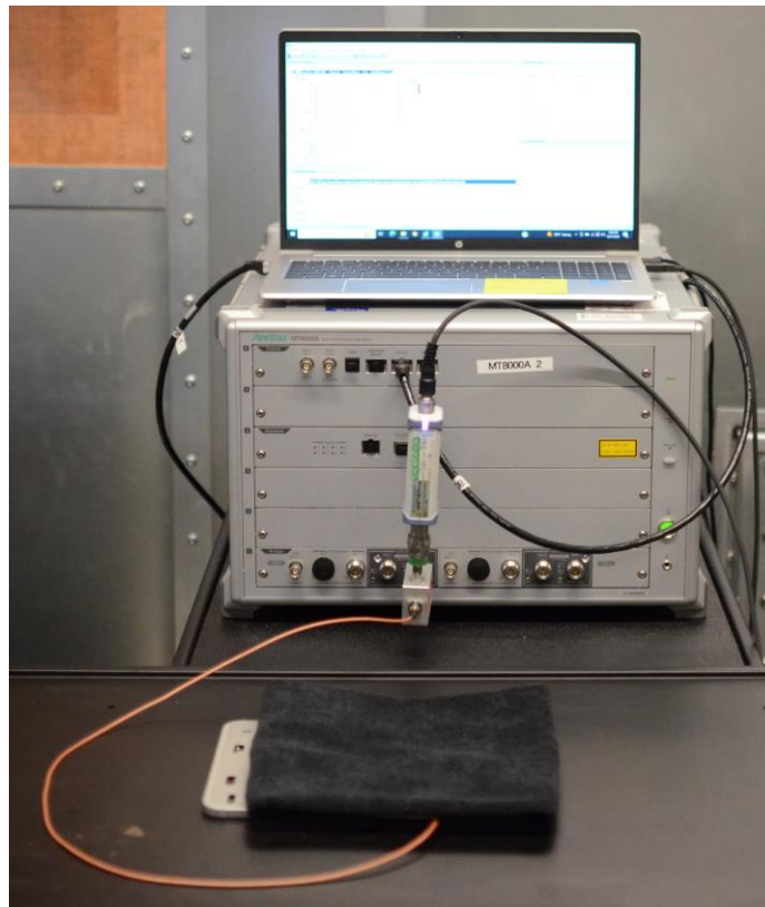
Test Setup Photo 2 – Conducted Test Setup (Figure 5-1a)
