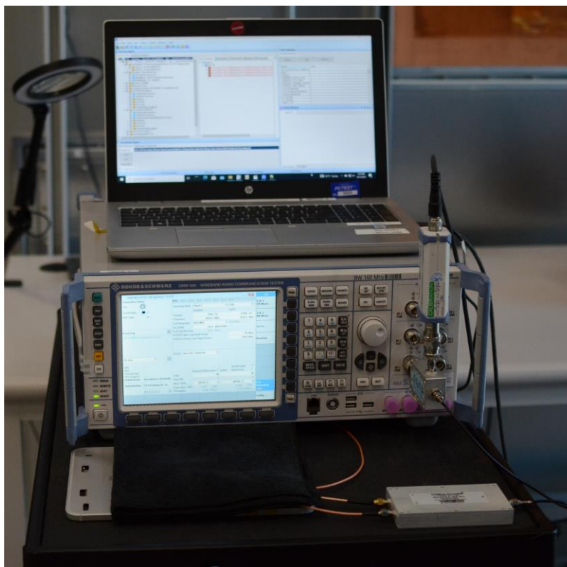
Test Setup Photo 6 – Conducted Test Setup (Figure 5-1d)
