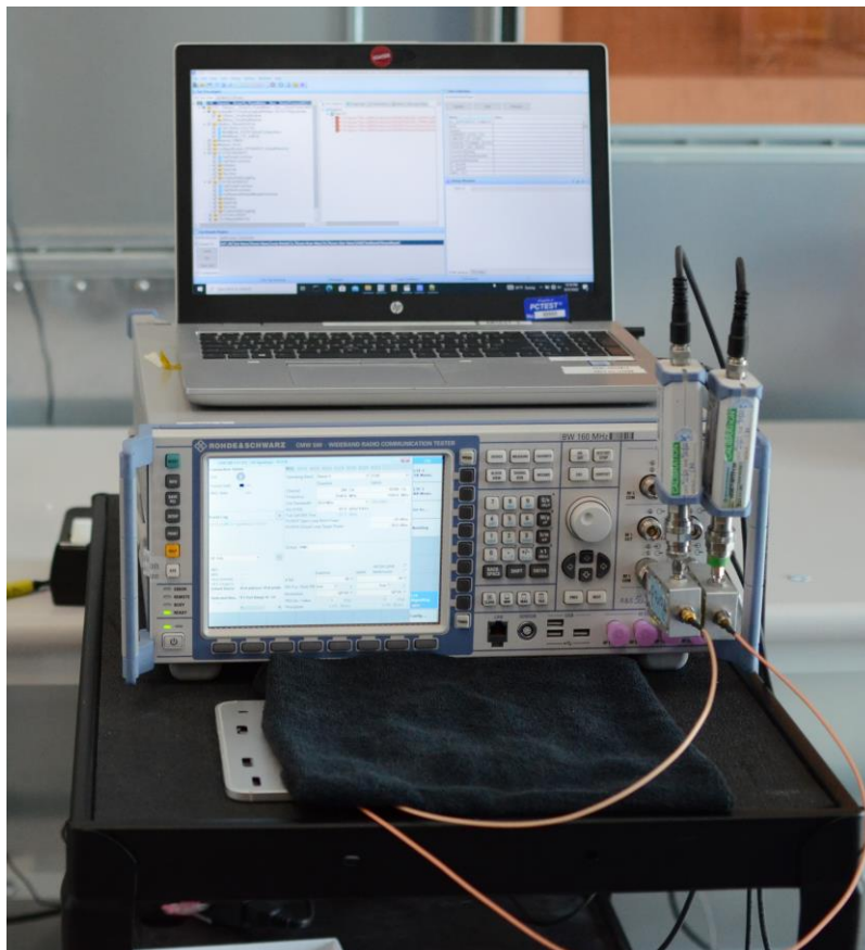
Test Setup Photo 4 – Conducted Test Setup (Figure 5-1b)
