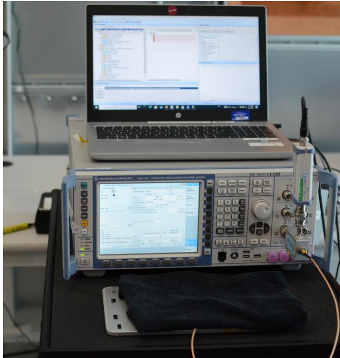
Test Setup Photo 1 – Conducted Test Setup (Figure 5-1a)
