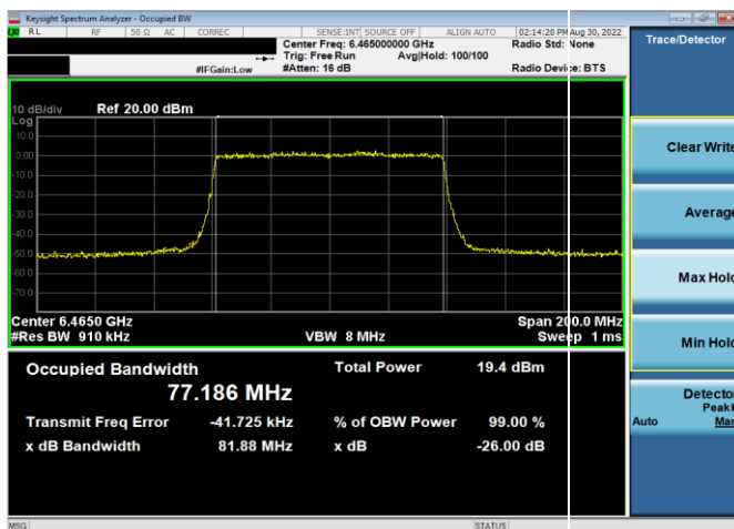
Plot 7-9. 26dB & 99% Bandwidth Plot Antenna WF5t (80MHz 802.11ax (UNII Band 6) – Ch. 103, MCS2)
