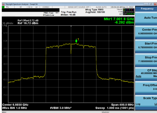
Plot 7-272. Power Spectral Density Plot SDM Antenna WF5b (160MHz 802.11ax (UNII Band 8) – Ch. 207, MCS2)
