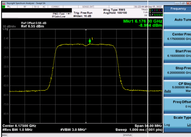
Plot 7-305. Power Spectral Density Plot SDM Antenna WF5t (20MHz 802.11ax (UNII Band 5) – Ch. 45, MCS11)
