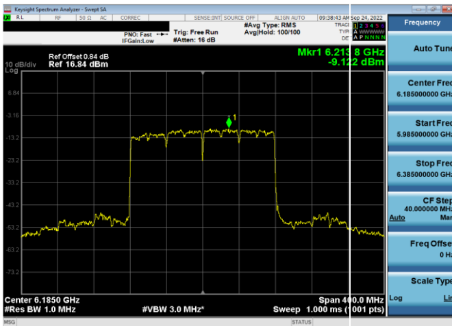
Plot 7-312. Power Spectral Density Plot SDM Antenna WF5b (160MHz 802.11ax (UNII Band 5) – Ch. 47, MCS11)
