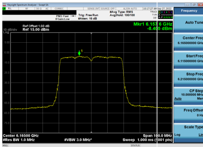
Plot 7-307. Power Spectral Density Plot SDM Antenna WF5t (40MHz 802.11ax (UNII Band 5) – Ch. 43, MCS11)
