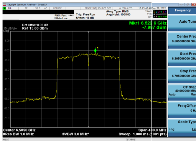
Plot 7-287. Power Spectral Density Plot SDM Antenna WF5t (160MHz 802.11ax (UNII Band 6) – Ch. 111, MCS4)
