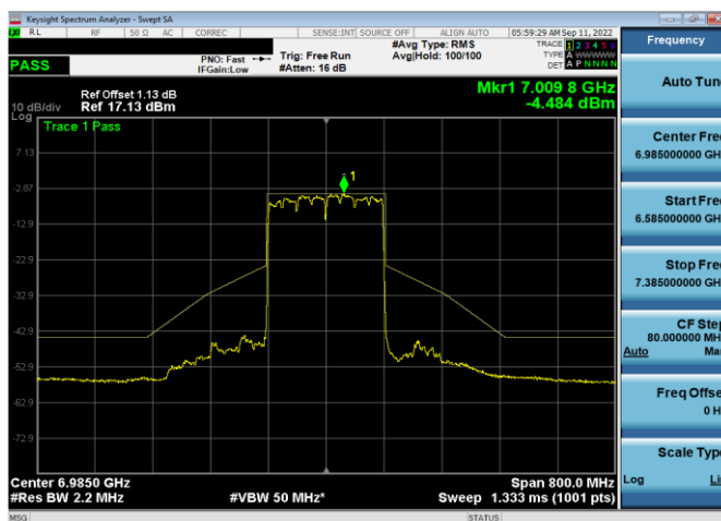
Plot 7-552. In-Band Emission Plot SDM Antenna WF5b (160MHz 802.11ax (UNII Band 8) – Ch. 207, MCS11)
