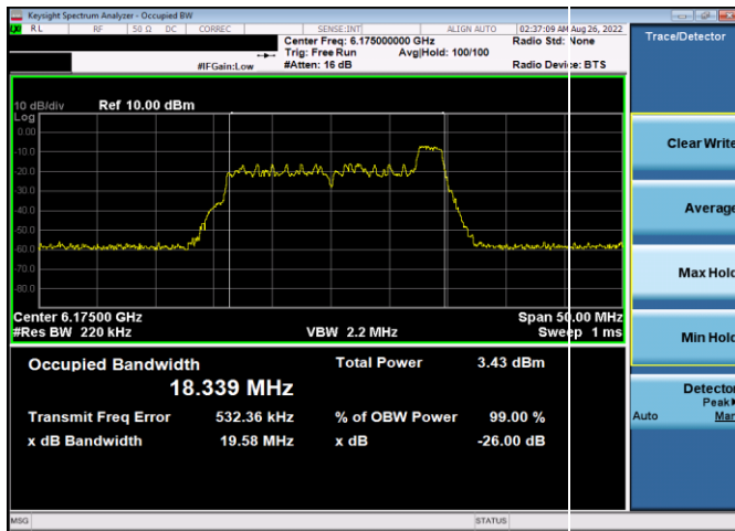
Plot 7-3. 26dB & 99% Bandwidth Plot Antenna WF5t (20MHz 802.11ax RU26 (UNII Band 5) – Ch. 45)
