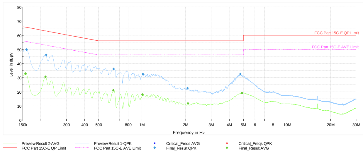
Plot 7-809. AC Line Conducted Plot with 11ax UNII Band 5 – RU26 – Ch.1 (L1) with AC/DC Adapter
