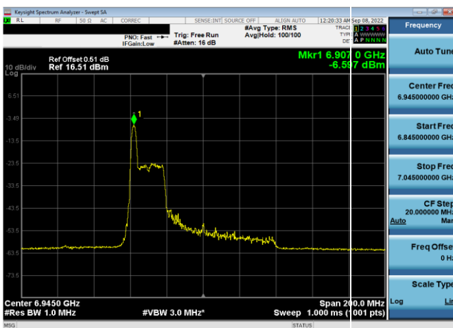
Plot 7-185. Power Spectral Density Plot Antenna WF5t (80MHz 802.11ax RU26 (UNII Band 8) - Ch. 199)
