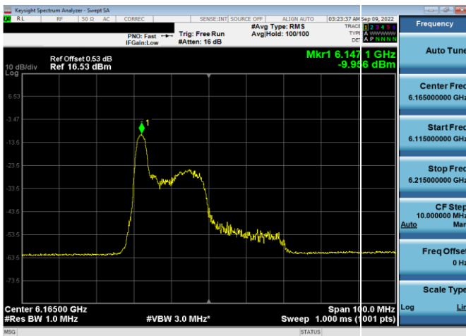
Plot 7-265. Power Spectral Density Plot SDM Antenna WF5t (40MHz 802.11ax RU26 (UNII Band 5) – Ch. 43)
