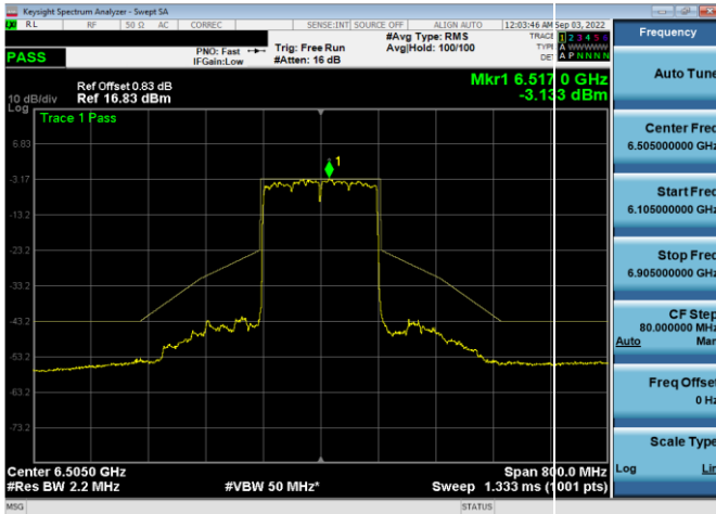
Plot 7-415. In-Band Emission Plot Antenna WF5t (160MHz 802.11ax RU484 (UNII Band 6) – Ch. 111)
