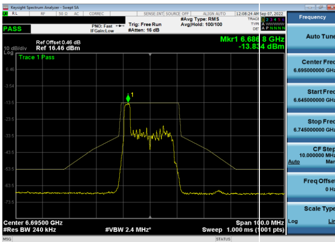
Plot 7-416. In-Band Emission Plot Antenna WF5t (20MHz 802.11ax RU26 (UNII Band 7) – Ch. 149)
