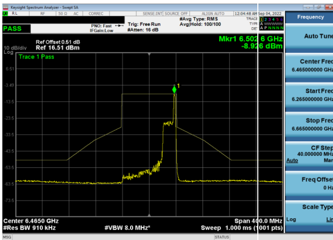
Plot 7-410. In-Band Emission Plot Antenna WF5t (80MHz 802.11ax RU26 (UNII Band 6) – Ch. 103)
