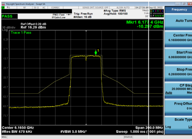
Plot 7-455. In-Band Emission Plot Antenna WF5b (40MHz 802.11ax RU484 (UNII Band 5) – Ch. 43)
