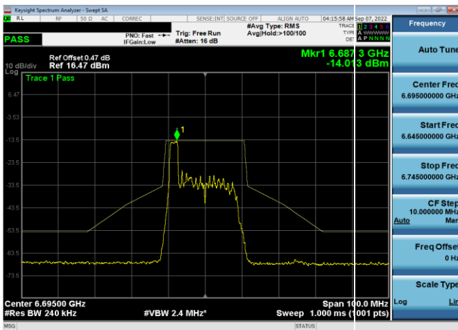
Plot 7-480. In-Band Emission Plot Antenna WF5b (20MHz 802.11ax RU26 (UNII Band 7) – Ch. 149)
