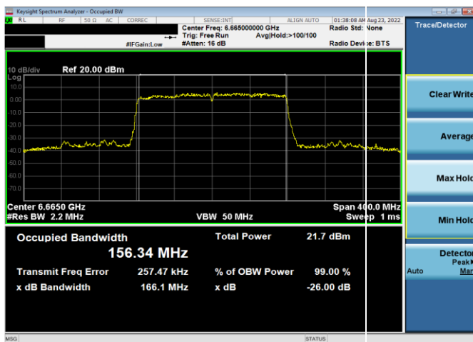
Plot 7-35. 26dB & 99% Bandwidth Plot Antenna 5b (160MHz 802.11ax (UNII Band 7) – Ch. 143, MCS4)
