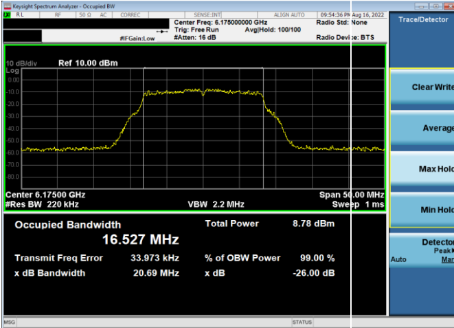
Plot 7-1. 26dB & 99% Bandwidth Plot Antenna 5b (20MHz 802.11a (UNII Band 5) – Ch. 45, 12Mbps)
