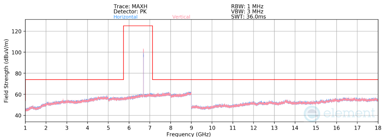
Plot 7-3. Radiated Spurious Emissions above 1GHz SDM (802.11ax – Ch. 149, MCS2)
