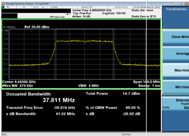
Plot 7-48. 26dB & 99% Bandwidth Plot Antenna 5b (40MHz 802.11ax (UNII Band 6) – Ch. 107, MCS11)
