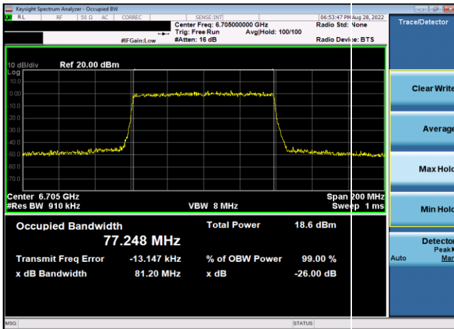
Plot 7-34. 26dB & 99% Bandwidth Plot Antenna 5b (80MHz 802.11ax (UNII Band 7) – Ch. 151, MCS4)
