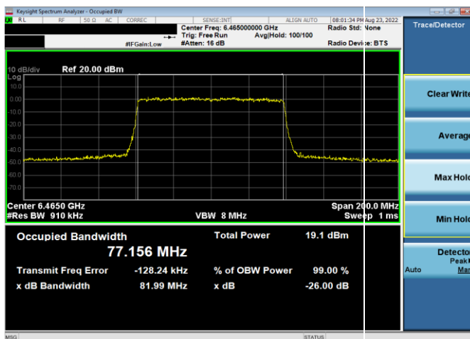
Plot 7-49. 26dB & 99% Bandwidth Plot Antenna 5b (80MHz) 802.11ax (UNII Band 6) – Ch. 103, MCS11)
