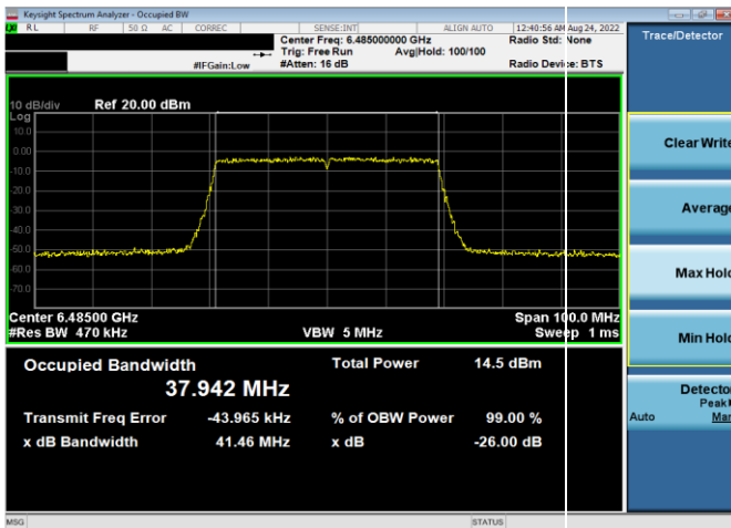
Plot 7-68. 26dB & 99% Bandwidth Plot Antenna 5b (40MHz 802.11ax (UNII Band 6) – Ch. 107, MCS2)
