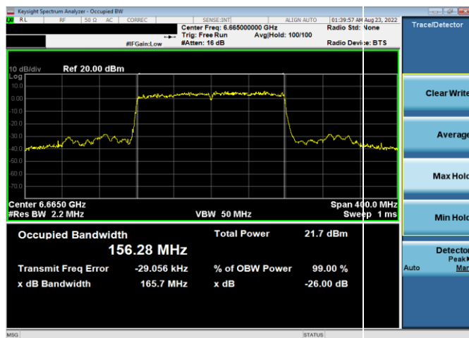
Plot 7-55. 26dB & 99% Bandwidth Plot Antenna 5b (160MHz 802.11ax (UNII Band 7) – Ch. 143, MCS11)
