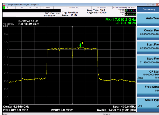
Plot 7-272. Power Spectral Density Plot SDM Antenna 4a (160MHz 802.11ax (UNII Band 8) – Ch. 207, MCS2)
