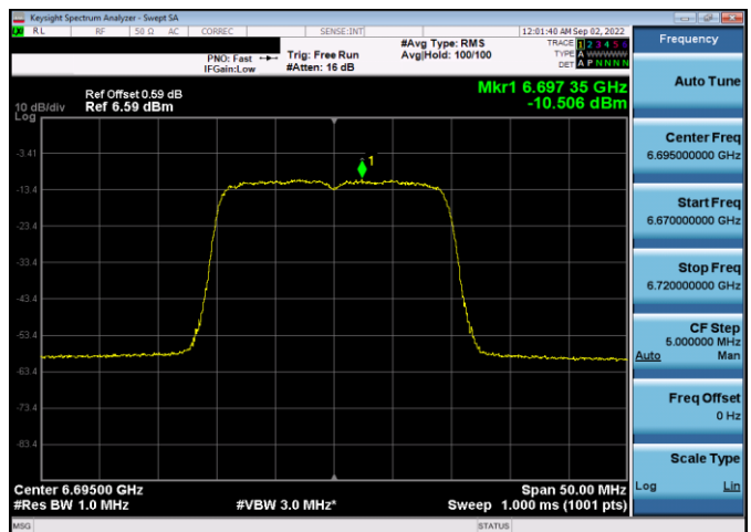
Plot 7-322. Power Spectral Density Plot SDM Antenna 4a (20MHz 802.11ax (UNII Band 7) – Ch. 149, MCS11)
