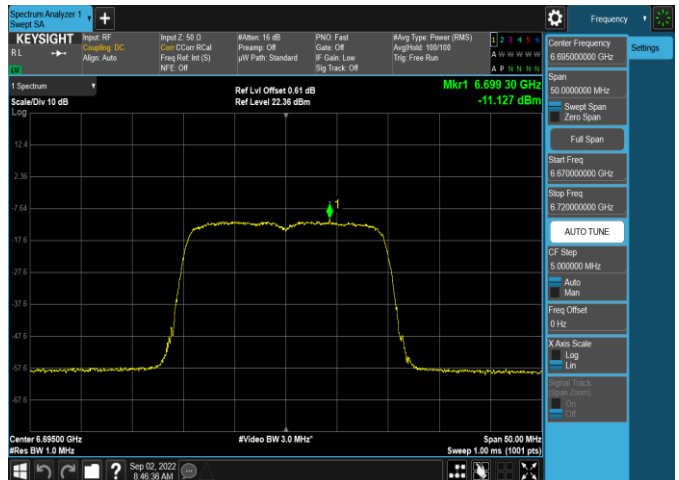
Plot 7-321. Power Spectral Density Plot SDM Antenna 5b (20MHz 802.11ax (UNII Band 7) – Ch. 149, MCS11)
