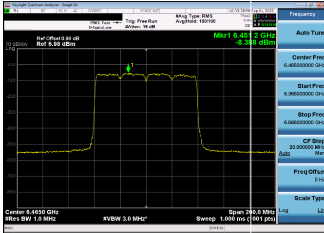
Plot 7-317. Power Spectral Density Plot SDM Antenna 5b (80MHz 802.11ax (UNII Band 6) – Ch. 103, MCS11)
