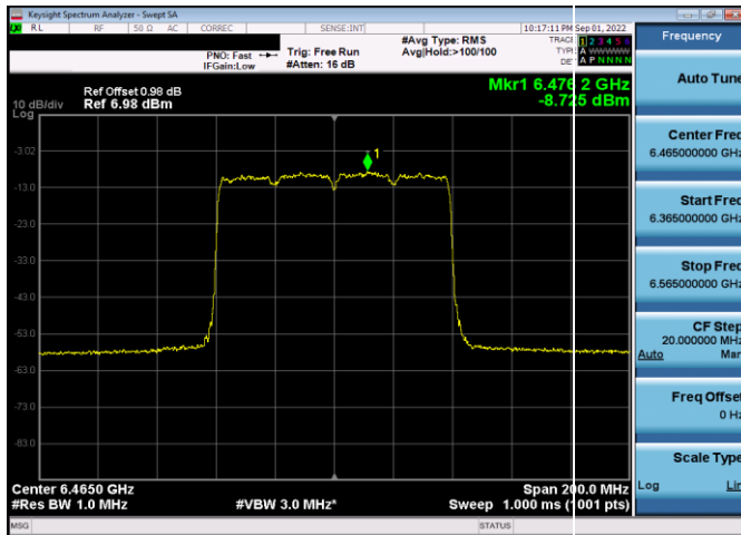
Plot 7-318. Power Spectral Density Plot SDM Antenna 4a (80MHz 802.11ax (UNII Band 6) – Ch. 103, MCS11)
