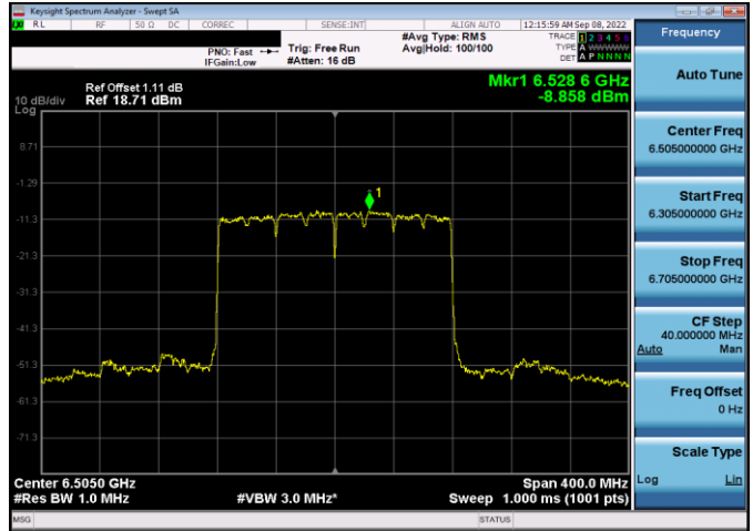
Plot 7-320. Power Spectral Density Plot SDM Antenna 4a (160MHz 802.11ax (UNII Band 6) – Ch. 111, MCS11)
