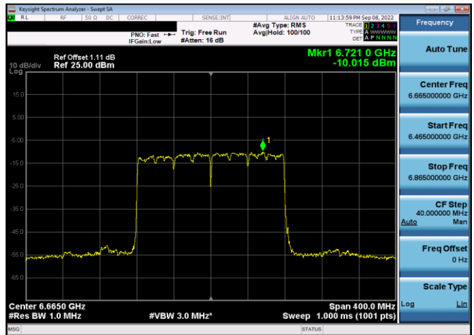
Plot 7-327. Power Spectral Density Plot SDM Antenna 5b (160MHz 802.11ax (UNII Band 7) – Ch. 143, MCS11)
