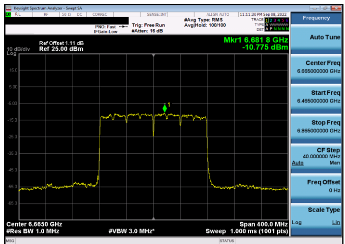
Plot 7-328. Power Spectral Density Plot SDM Antenna 4a (160MHz 802.11ax (UNII Band 7) – Ch. 143, MCS11)
