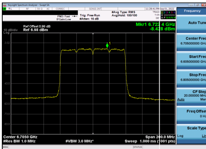
Plot 7-325. Power Spectral Density Plot SDM Antenna 5b (80MHz 802.11ax (UNII Band 7) – Ch. 151, MCS11)
