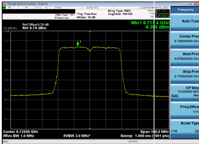
Plot 7-324. Power Spectral Density Plot SDM Antenna 4a (40MHz 802.11ax (UNII Band 7) – Ch. 155, MCS11)
