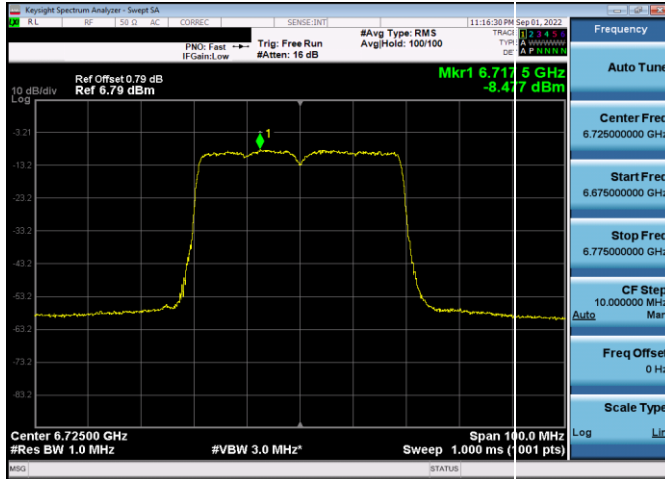
Plot 7-323. Power Spectral Density Plot SDM Antenna 5b (40MHz 802.11ax (UNII Band 7) – Ch. 155, MCS11)
