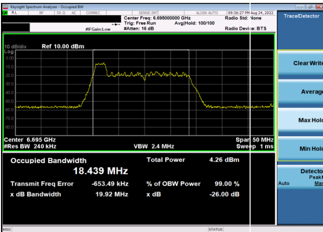
Plot 7-33. 26dB & 99% Bandwidth Plot Antenna 5b (20MHz 802.11ax RU26 (UNII Band 7) – Ch. 149)
