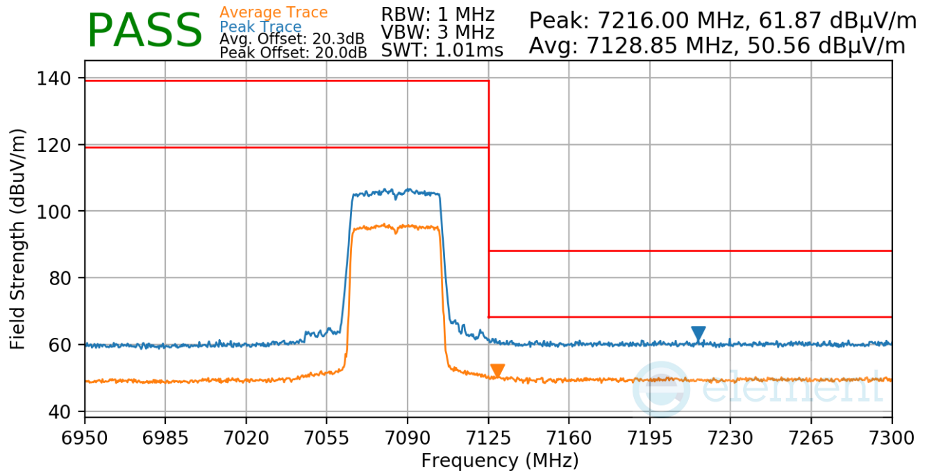
Plot 7-768. Antenna 5b Radiated Upper Band Edge (Peak & Average – UNII Band 8 – RU484)
