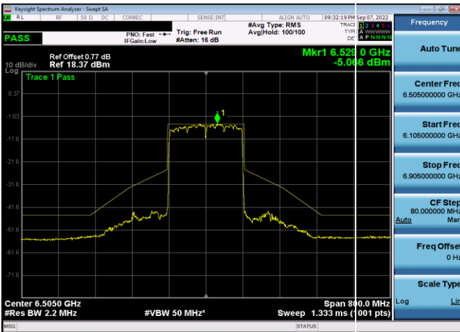
Plot 7-480. In-Band Emission Plot Antenna 4a (160MHz 802.11ax RU484 (UNII Band 6) – Ch. 111)
